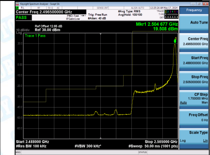
Band7_5MHz_16QAM_21425_1RB#0
