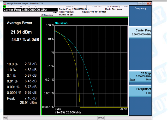
Band7-20MHz-16QAM-21350-27RB#0-PASS
