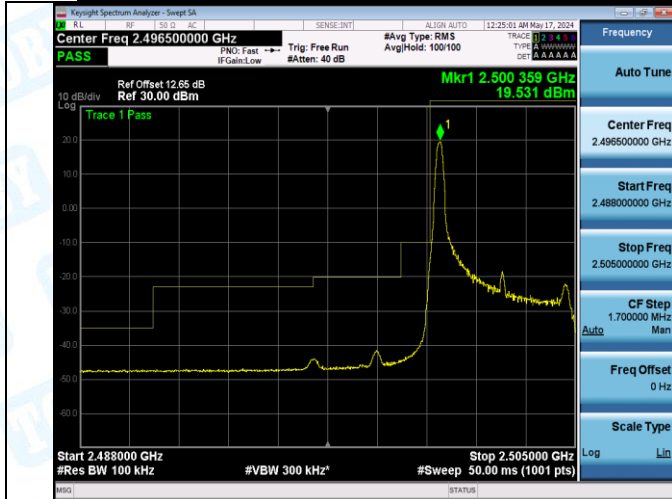
Band7_5MHz_16QAM_20775_25RB#0
