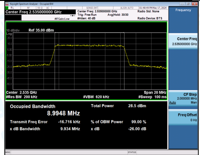
Band7-10MHz-16QAM-20800-27RB#0-PASS
