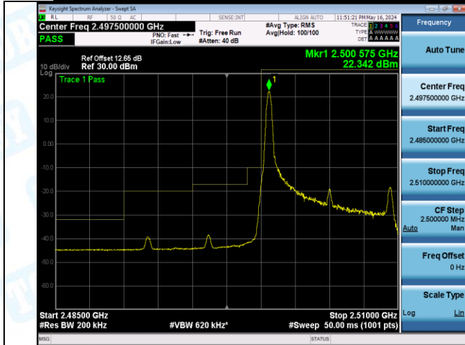
Band7_10MHz_QPSK_20800_50RB#0
