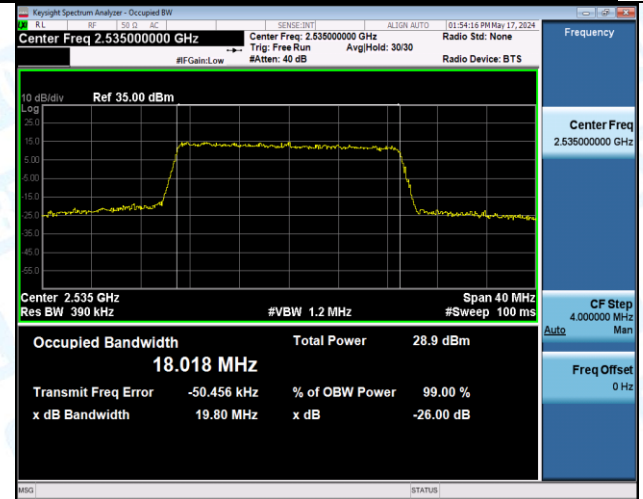
Band7-20MHz-16QAM-20850-27RB#0-PASS
