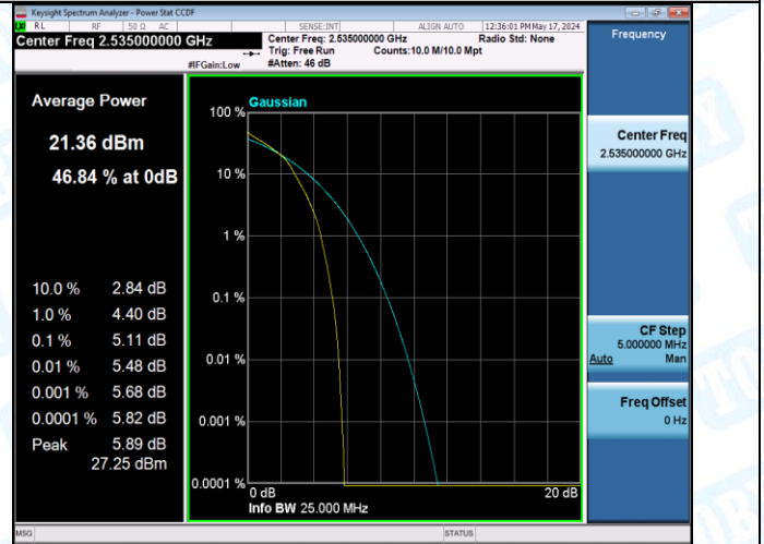
Band7-10MHz-16QAM-21400-27RB#0-PASS
