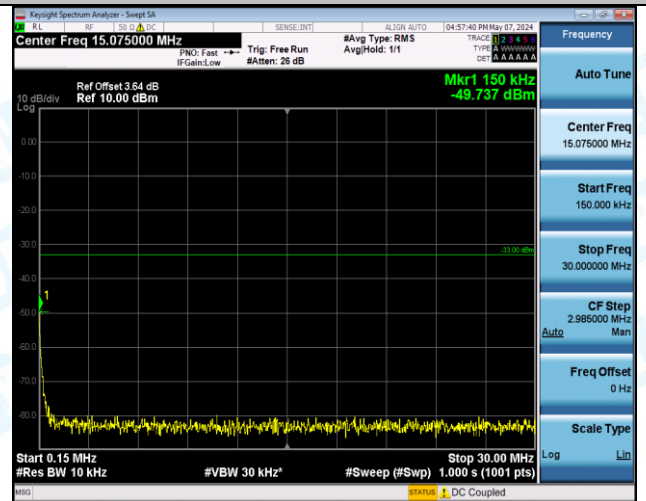
Band4_3MHz_16QAM_20175_15RB#0_1000~3000_1000~3000
