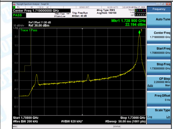
Band4_20MHz_QPSK_20050_100RB#99
