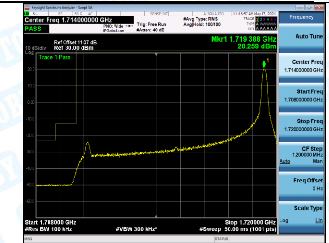
Band4_10MHz_16QAM_20350_1RB#49
