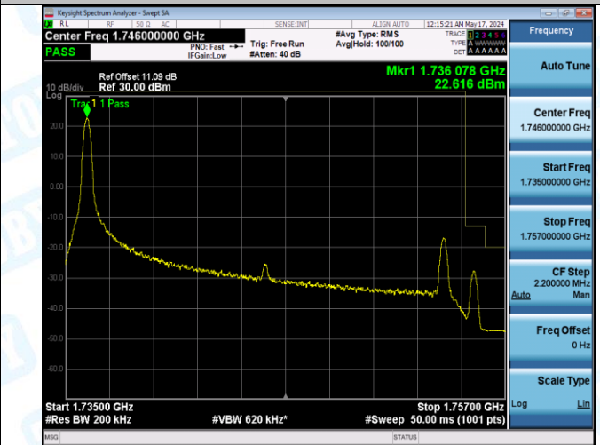
Band4_20MHz_QPSK_20300_1RB#99
