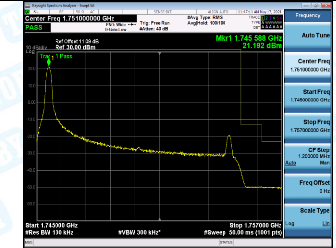
Band4_10MHz_QPSK_20350_50RB#0
