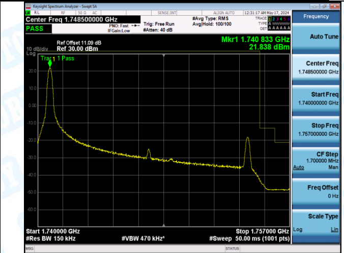
Band4_15MHz_QPSK_20325_75RB#0
