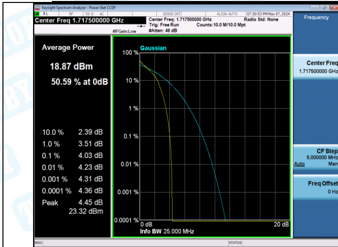
Band4-15MHz-QPSK-20175-1RB#0-PASS
