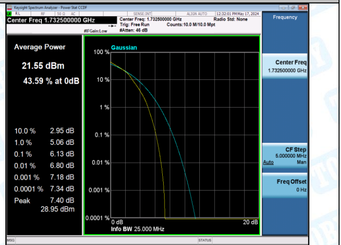
Band4-20MHz-16QAM-20300-27RB#0-PASS
