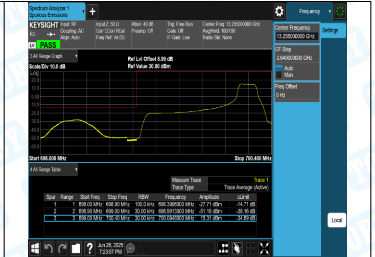
Band12-1.4MHz-QPSK-23017-1RB#5-PASS
