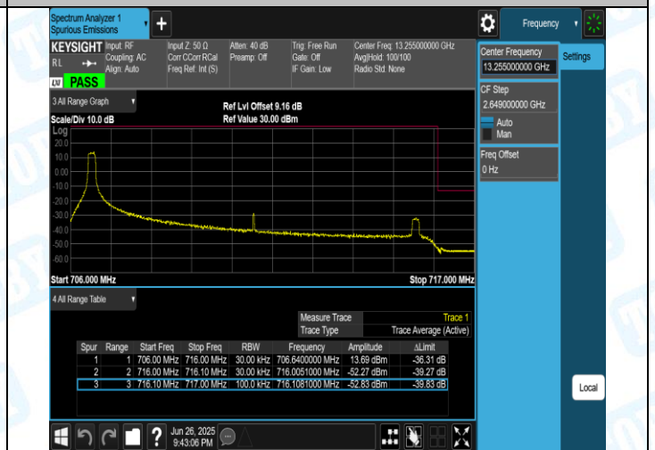
Band12-10MHz-16QAM-23130-1RB#0-PASS
