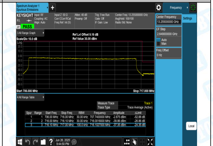
Band12-10MHz-16QAM-23130-50RB#0-PASS
