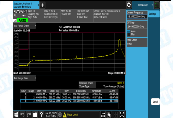
Band12-10MHz-16QAM-23060-1RB#49-PASS
