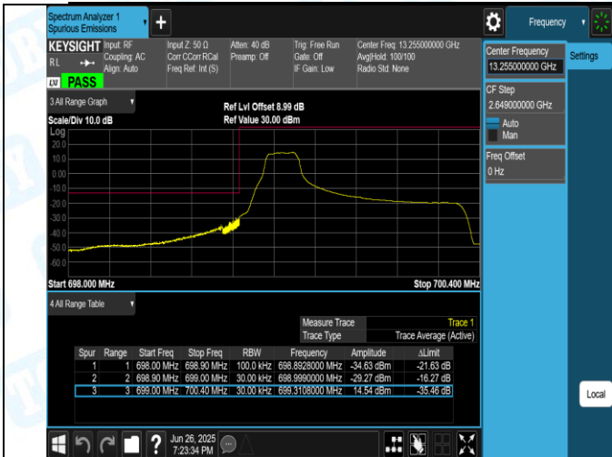
Band12-1.4MHz-16QAM-23017-1RB#0-PASS
