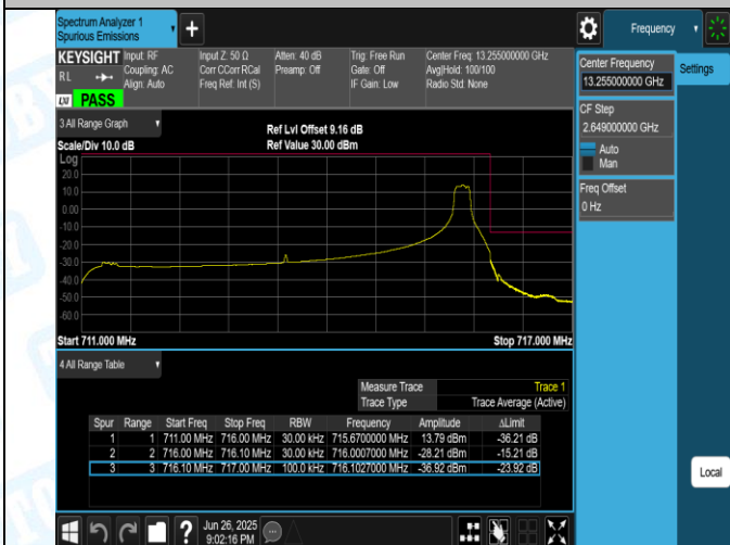
Band12-5MHz-16QAM-23155-1RB#24-PASS
