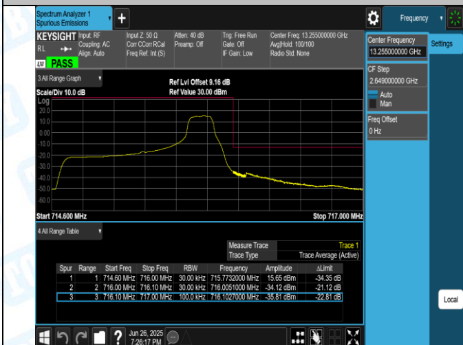
Band12-1.4MHz-QPSK-23173-1RB#5-PASS
