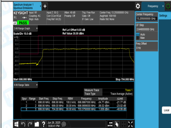
Band12-5MHz-16QAM-23035-25RB#0-PASS
