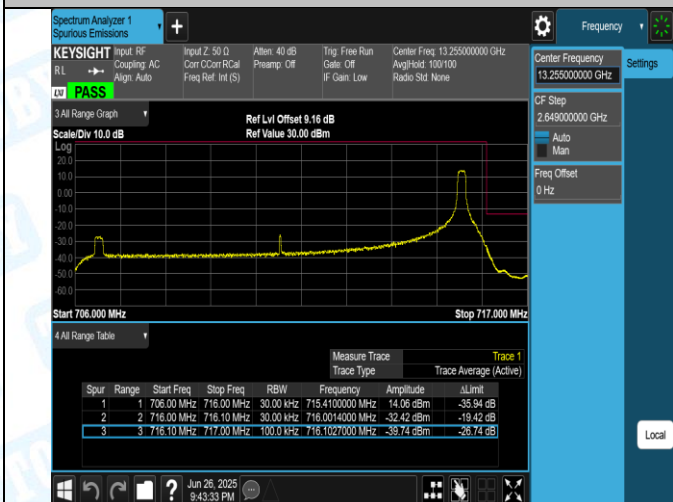
Band12-10MHz-QPSK-23130-1RB#49-PASS
