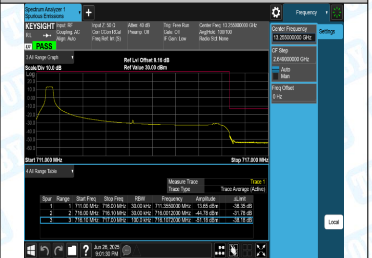
Band12-5MHz-16QAM-23155-1RB#0-PASS
