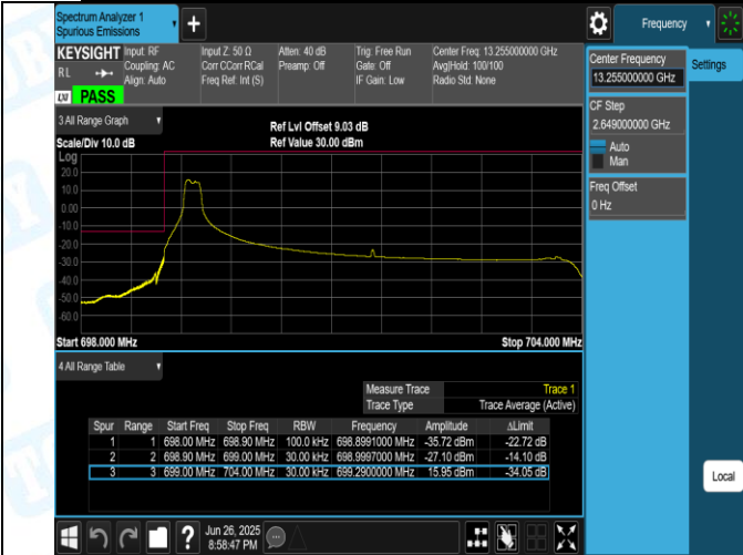
Band12-5MHz-QPSK-23035-1RB#0-PASS
