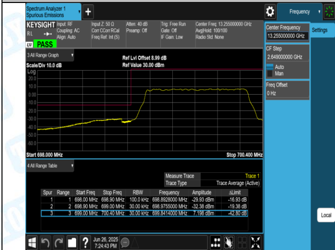
Band12-1.4MHz-QPSK-23017-6RB#0-PASS
