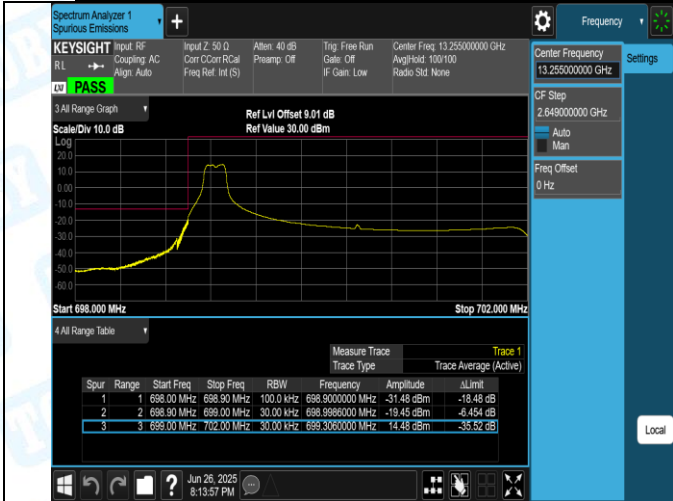
Band12-3MHz-16QAM-23025-1RB#0-PASS
