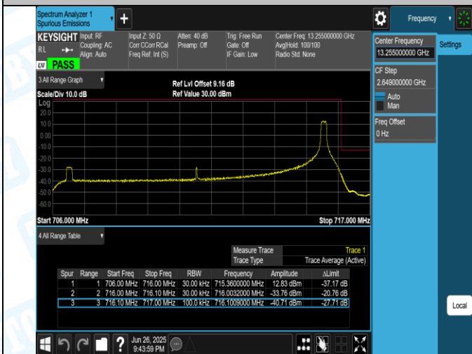
Band12-10MHz-16QAM-23130-1RB#49-PASS
