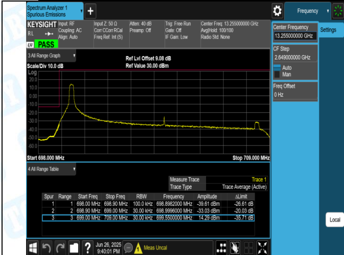
Band12-10MHz-QPSK-23060-1RB#0-PASS
