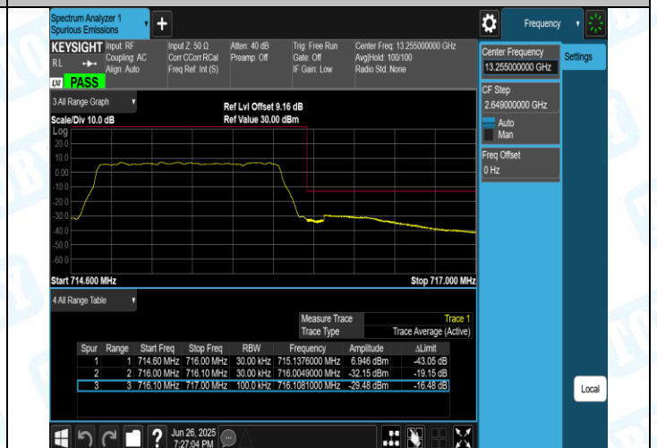
Band12-1.4MHz-QPSK-23173-6RB#0-PASS
