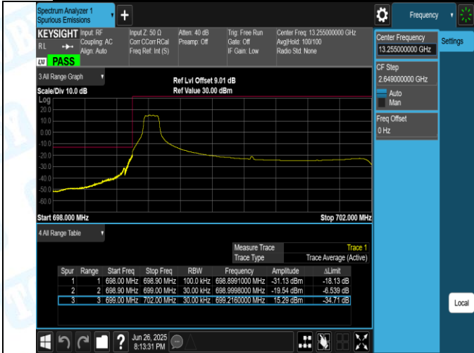
Band12-3MHz-QPSK-23025-1RB#0-PASS
