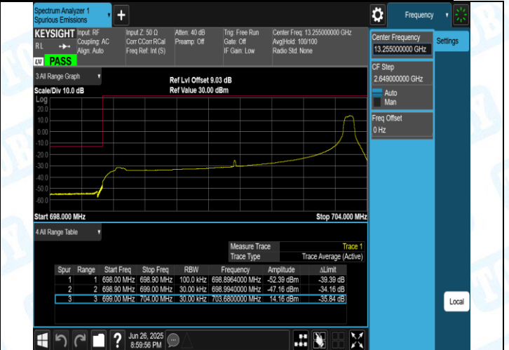
Band12-5MHz-16QAM-23035-1RB#24-PASS
