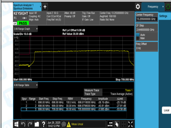
Band12-10MHz-16QAM-23060-50RB#0-PASS
