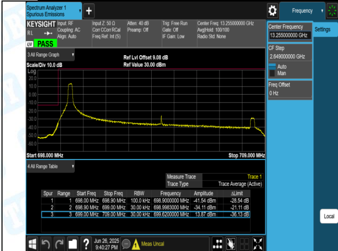
Band12-10MHz-16QAM-23060-1RB#0-PASS
