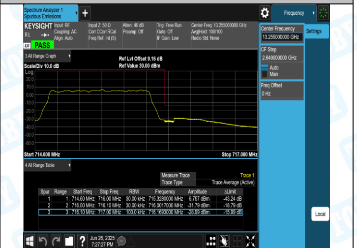
Band12-1.4MHz-16QAM-23173-6RB#0-PASS
