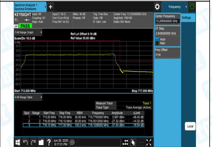
Band12-3MHz-QPSK-23165-15RB#0-PASS
