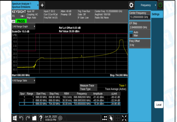
Band12-5MHz-QPSK-23035-1RB#24-PASS
