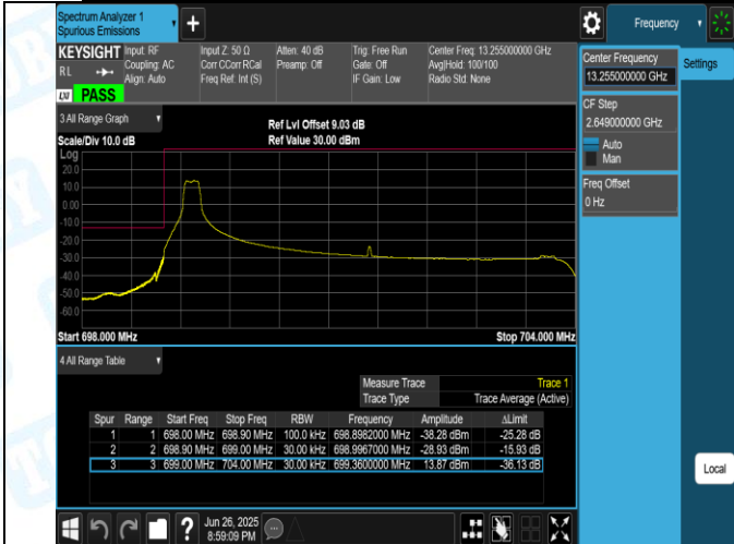
Band12-5MHz-16QAM-23035-1RB#0-PASS
