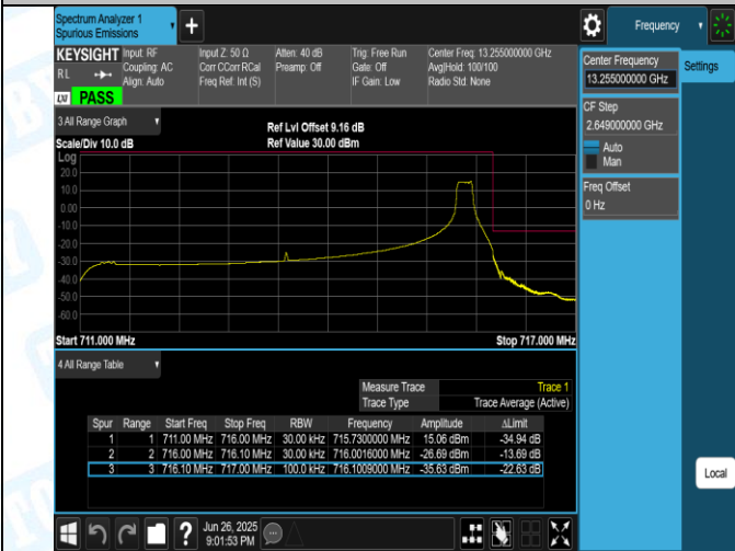
Band12-5MHz-QPSK-23155-1RB#24-PASS
