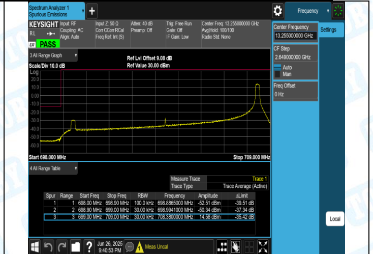
Band12-10MHz-QPSK-23060-1RB#49-PASS
