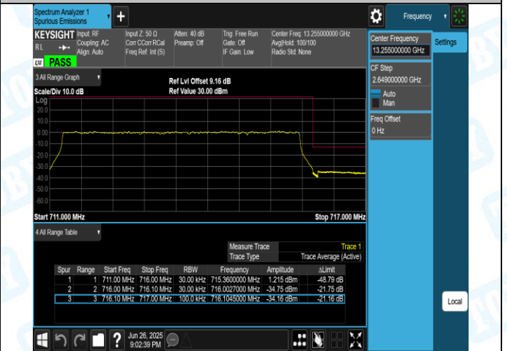
Band12-5MHz-QPSK-23155-25RB#0-PASS
