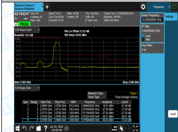
Band7-5MHz-QPSK-21425-1RB#0-PASS
