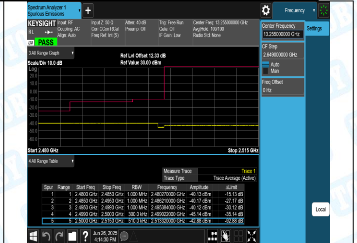
Band7-15MHz-QPSK-20825-1RB#74-PASS
