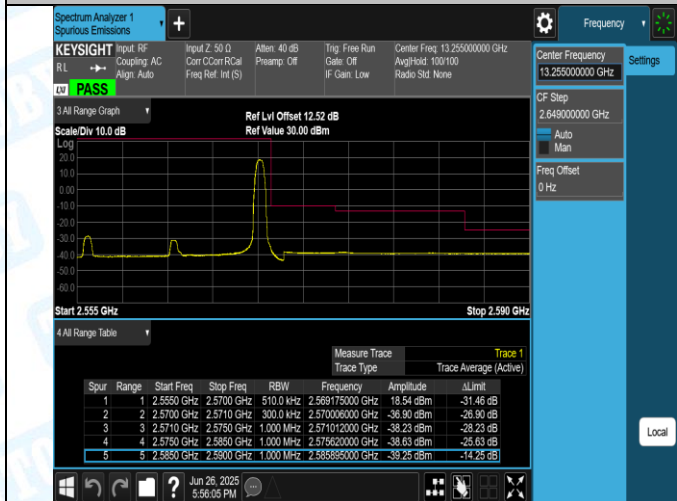
Band7-15MHz-QPSK-21375-1RB#74-PASS
