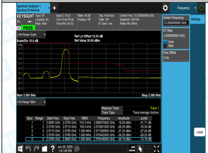
Band7-5MHz-16QAM-21425-1RB#24-PASS
