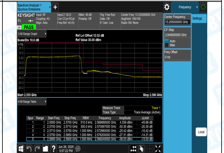
Band7-15MHz-QPSK-21375-75RB#0-PASS
