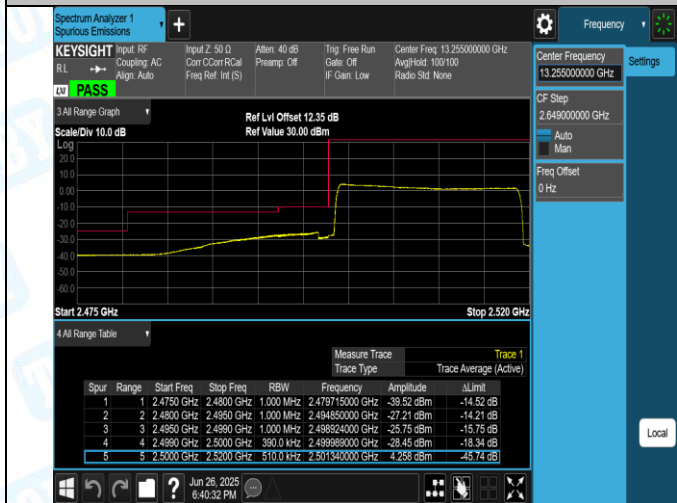
Band7-20MHz-16QAM-20850-100RB#0-PASS
