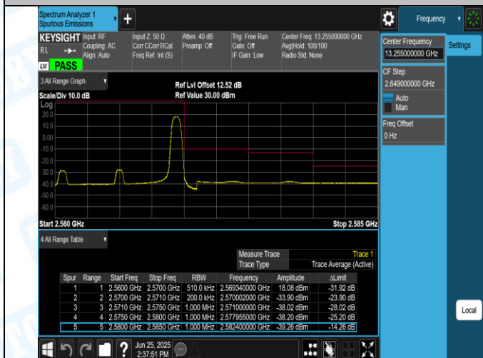
Band7-10MHz-16QAM-21400-1RB#49-PASS
