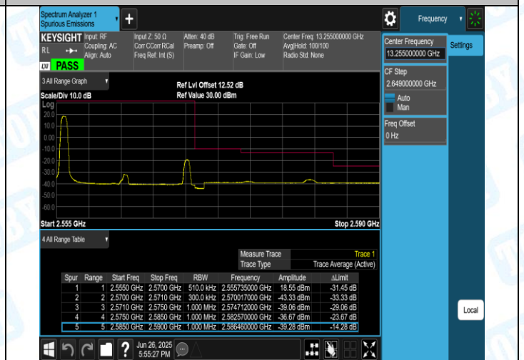
Band7-15MHz-16QAM-21375-1RB#0-PASS
