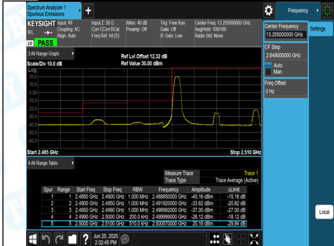
Band7-10MHz-16QAM-20800-1RB#0-PASS
