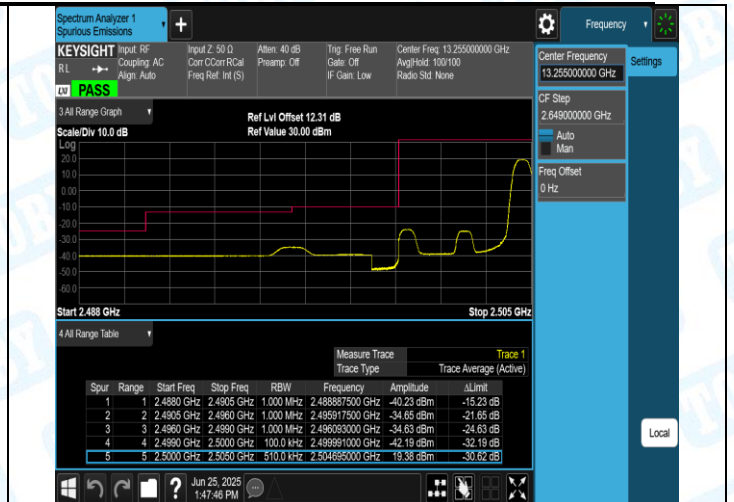
Band7-5MHz-16QAM-20775-1RB#24-PASS
