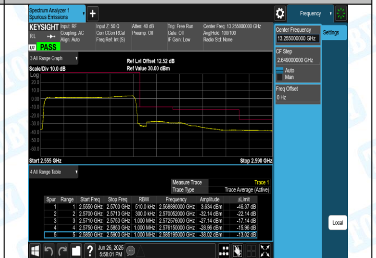
Band7-15MHz-16QAM-21375-75RB#0-PASS
