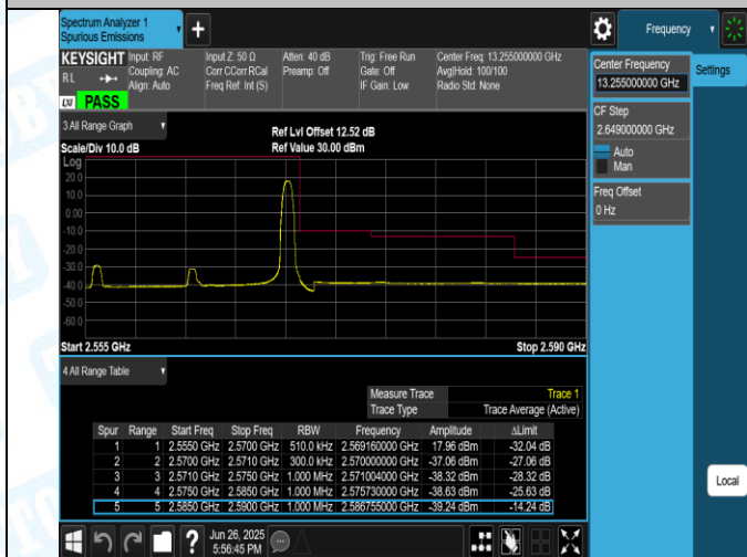
Band7-15MHz-16QAM-21375-1RB#74-PASS
