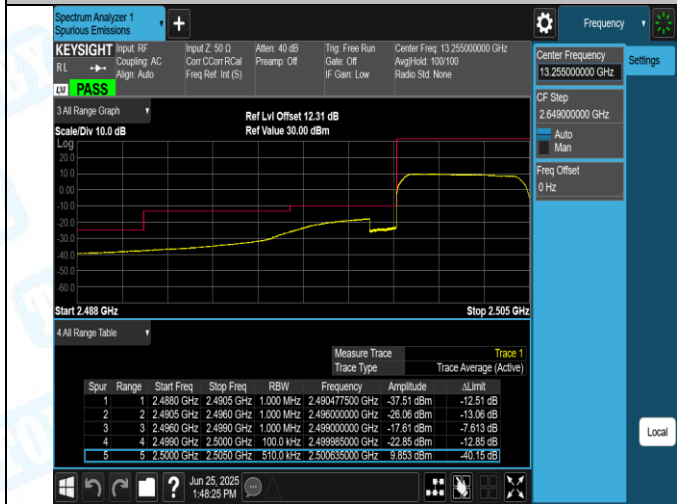
Band7-5MHz-QPSK-20775-25RB#0-PASS
