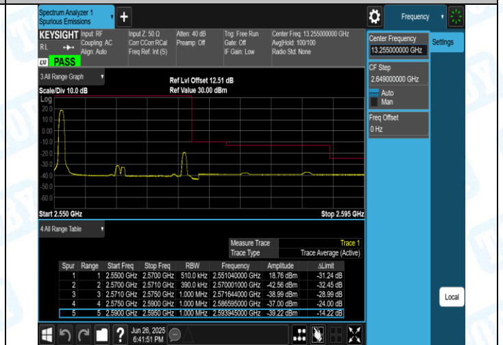
Band7-20MHz-16QAM-21350-1RB#0-PASS
