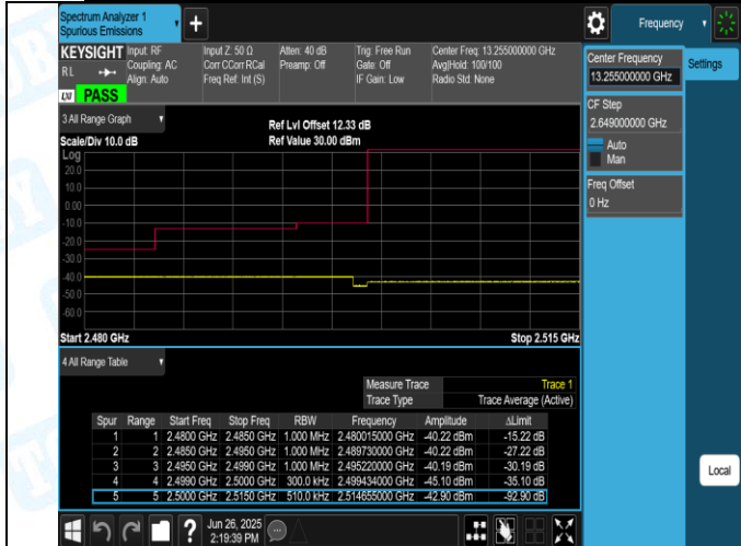
Band7-15MHz-QPSK-20825-1RB#0-PASS
