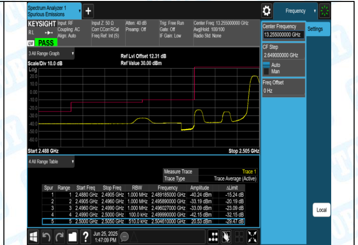
Band7-5MHz-QPSK-20775-1RB#24-PASS
