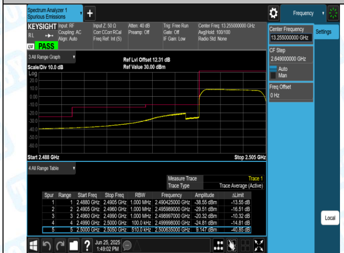
Band7-5MHz-16QAM-20775-25RB#0-PASS
