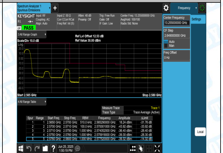
Band7-5MHz-16QAM-21425-1RB#0-PASS
