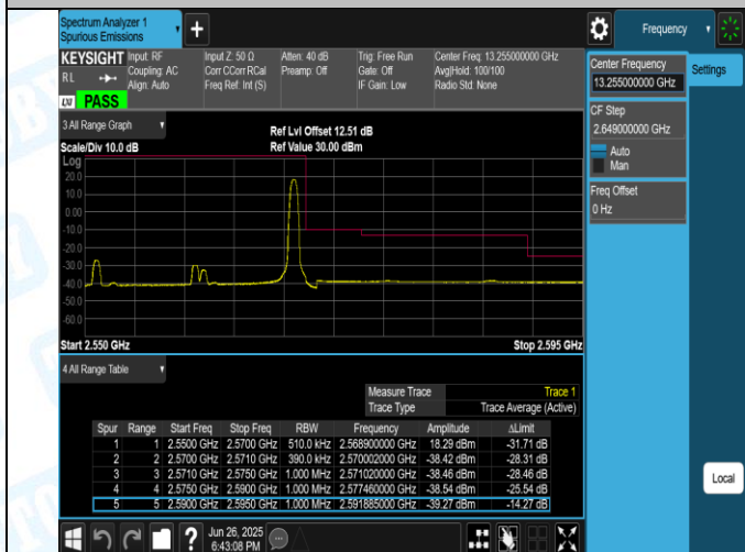
Band7-20MHz-16QAM-21350-1RB#99-PASS
