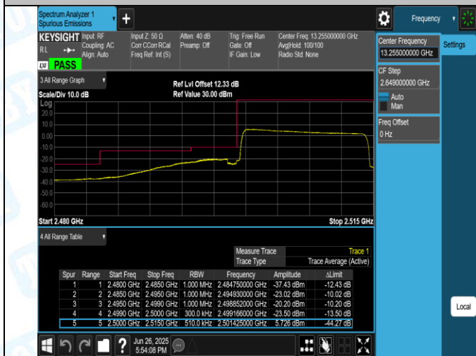
Band7-15MHz-16QAM-20825-75RB#0-PASS
