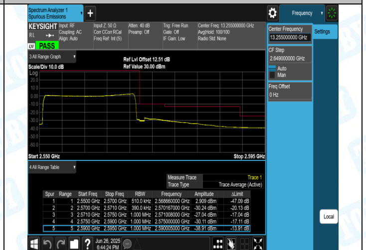
Band7-20MHz-16QAM-21350-100RB#0-PASS
