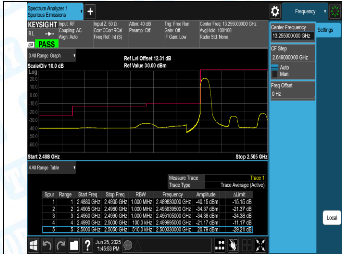
Band7-5MHz-QPSK-20775-1RB#0-PASS
