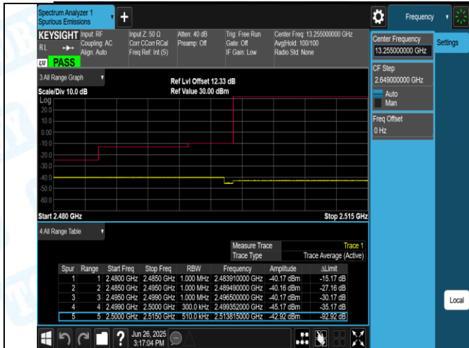
Band7-15MHz-16QAM-20825-1RB#0-PASS
