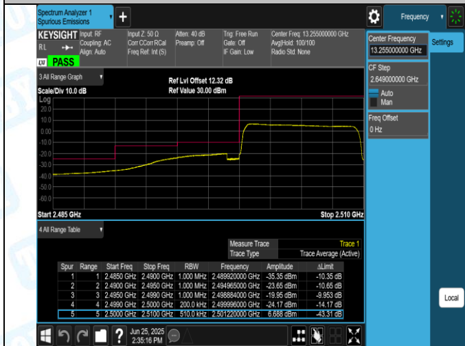
Band7-10MHz-16QAM-20800-50RB#0-PASS
