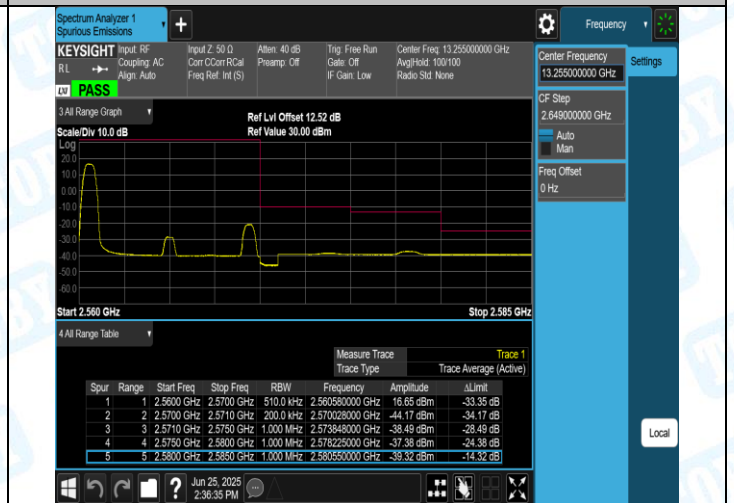
Band7-10MHz-16QAM-21400-1RB#0-PASS
