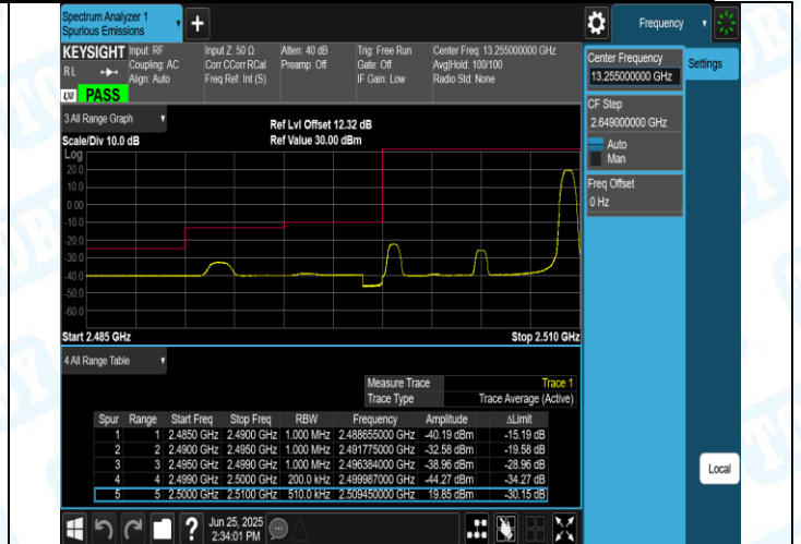
Band7-10MHz-16QAM-20800-1RB#49-PASS
