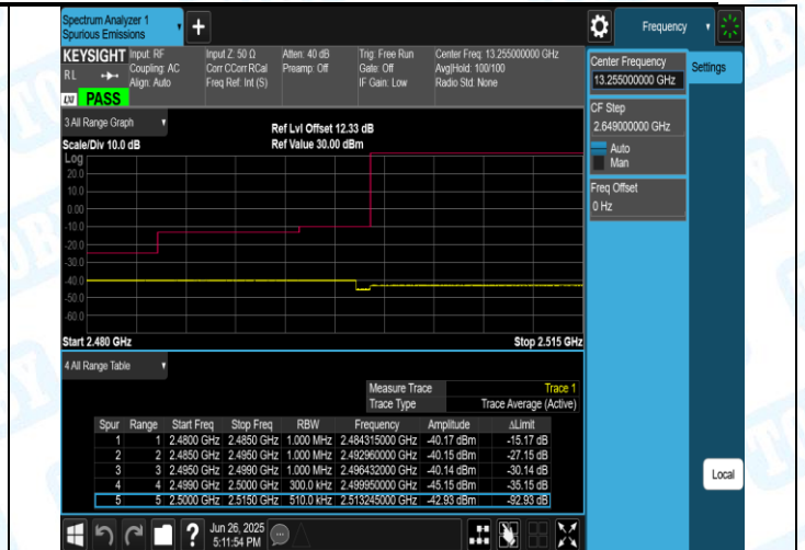
Band7-15MHz-16QAM-20825-1RB#74-PASS
