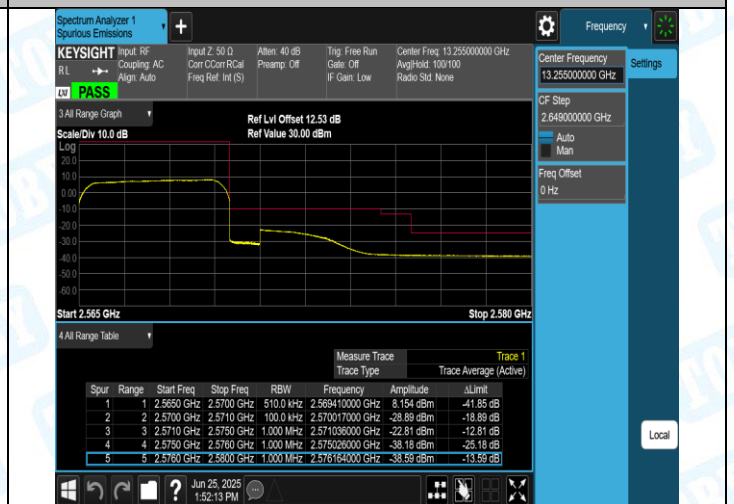
Band7-5MHz-QPSK-21425-1RB#24-PASS
