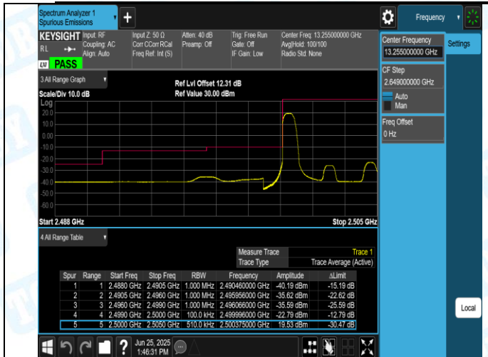
Band7-5MHz-16QAM-20775-1RB#0-PASS
