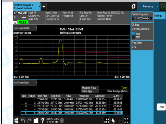
Band7-10MHz-QPSK-21400-1RB#49-PASS
