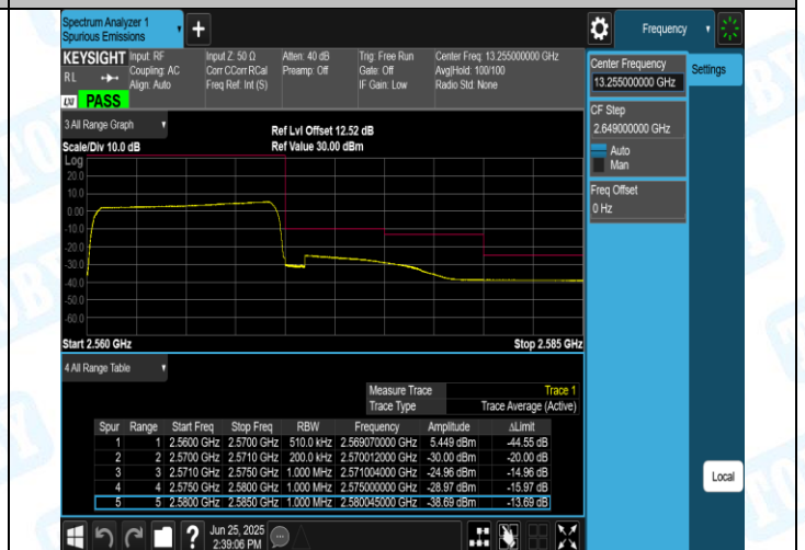
Band7-10MHz-16QAM-21400-50RB#0-PASS
