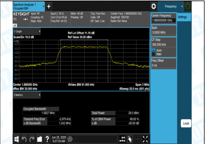
Band2-1.4MHz-QPSK-18900-6RB#0-PASS
