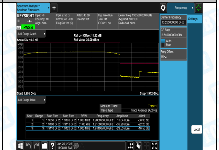
Band2-5MHz-QPSK-19175-25RB#0-PASS
