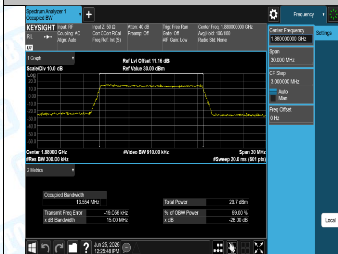
Band2-15MHz-16QAM-18900-75RB#0-PASS
