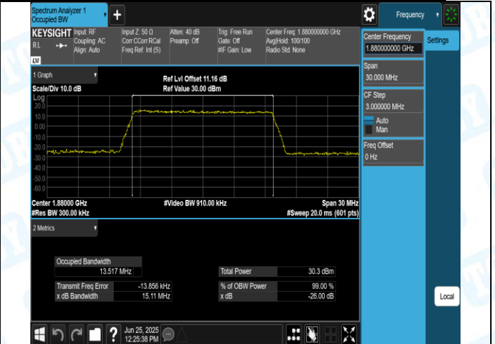
Band2-15MHz-QPSK-18900-75RB#0-PASS
