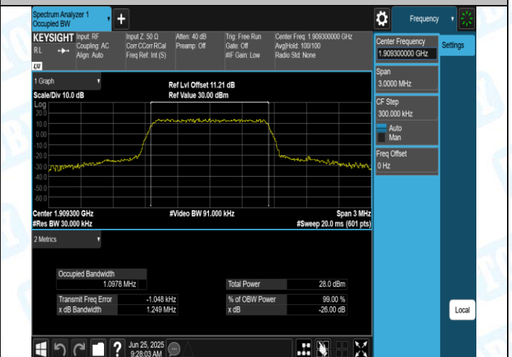
Band2-1.4MHz-16QAM-19193-6RB#0-PASS
