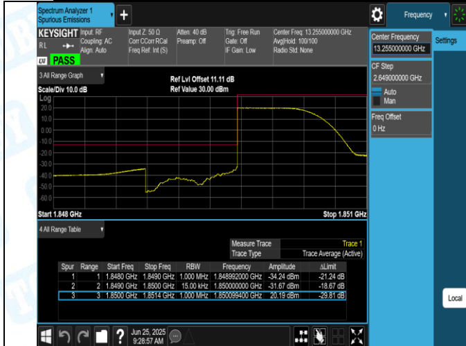
Band2-1.4MHz-16QAM-18607-1RB#0-PASS
