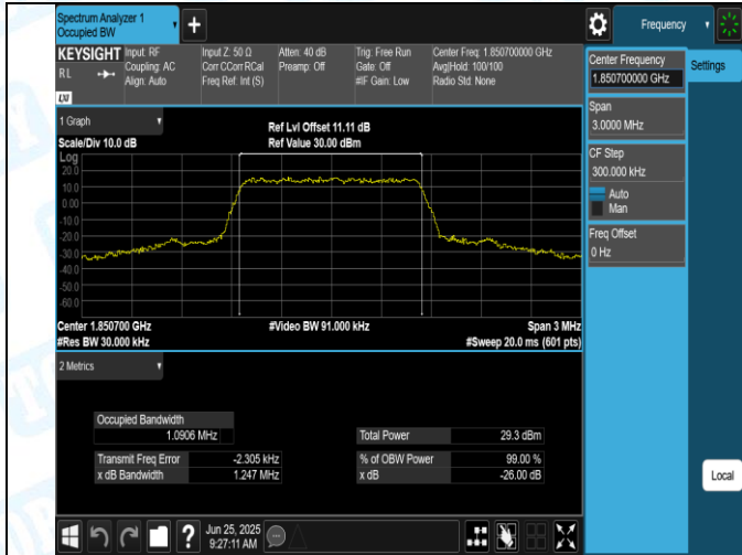
Band2-1.4MHz-QPSK-18607-6RB#0-PASS
