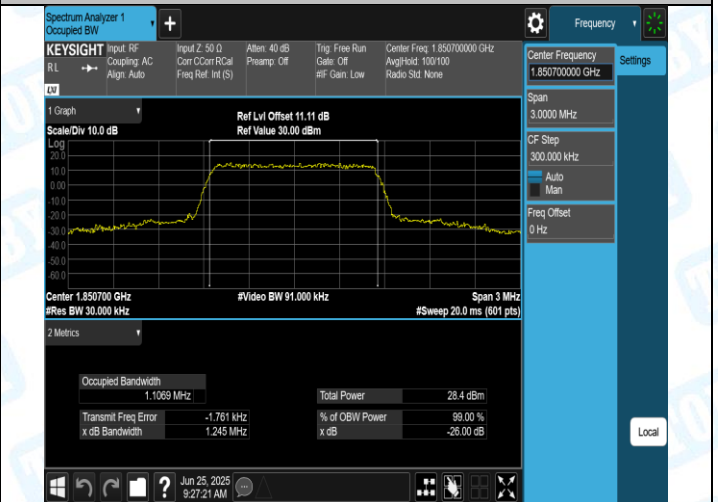
Band2-1.4MHz-16QAM-18607-6RB#0-PASS
