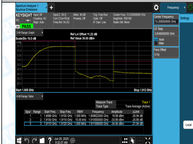
Band2-1.4MHz-16QAM-19193-1RB#5-PASS
