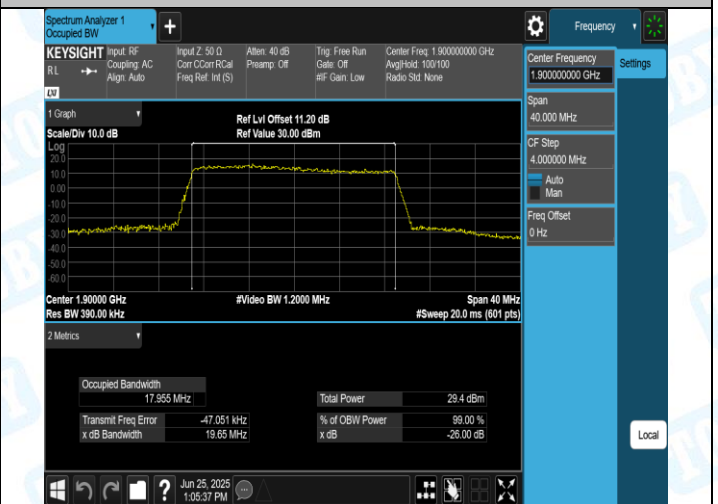
Band2-20MHz-16QAM-19100-100RB#0-PASS
