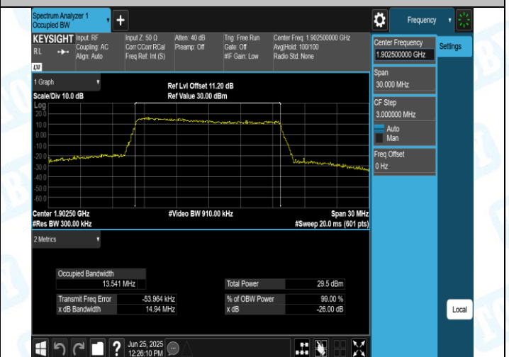
Band2-15MHz-16QAM-19125-75RB#0-PASS
