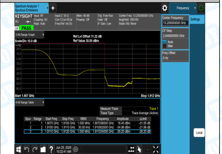
Band2-3MHz-QPSK-19185-1RB#0-PASS
