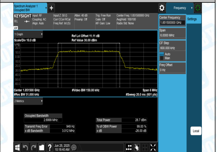
Band2-3MHz-16QAM-18615-15RB#0-PASS
