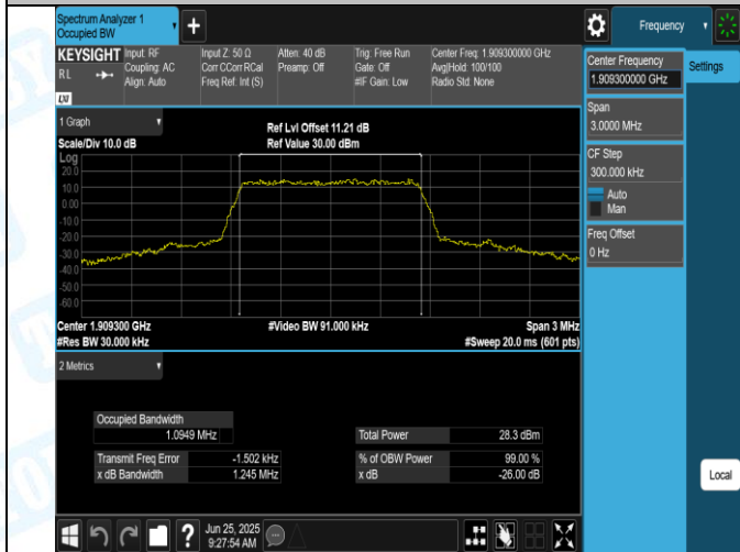
Band2-1.4MHz-QPSK-19193-6RB#0-PASS
