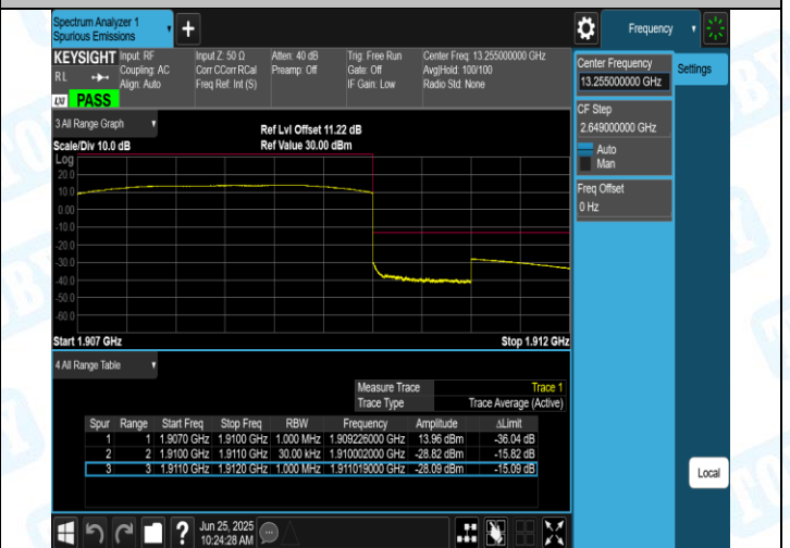
Band2-3MHz-QPSK-19185-15RB#0-PASS
