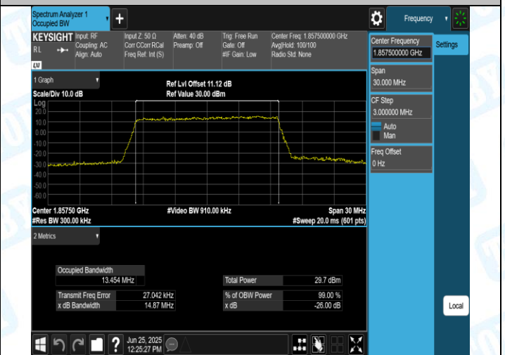
Band2-15MHz-16QAM-18675-75RB#0-PASS
