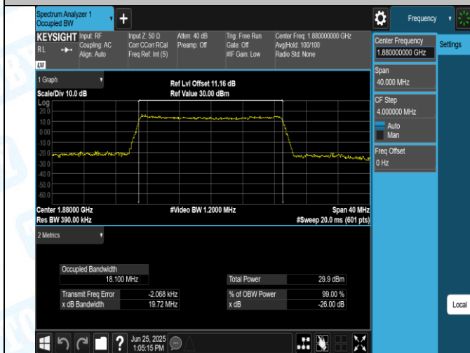
Band2-20MHz-16QAM-18900-100RB#0-PASS
