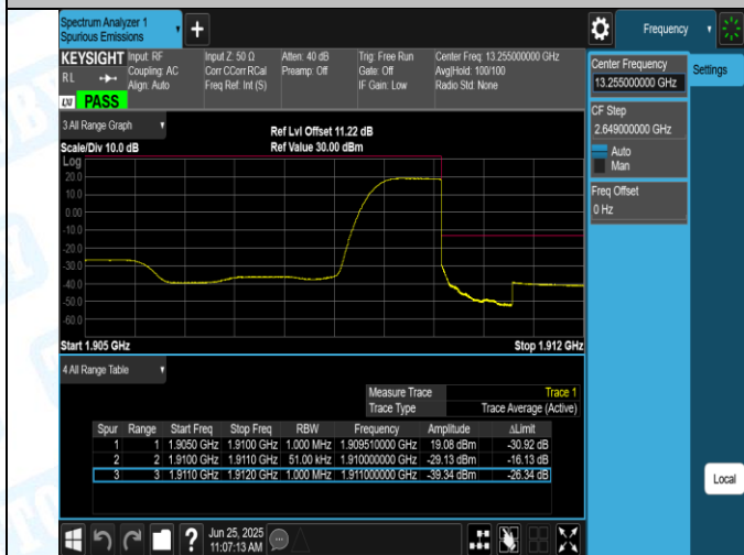
Band2-5MHz-QPSK-19175-1RB#24-PASS
