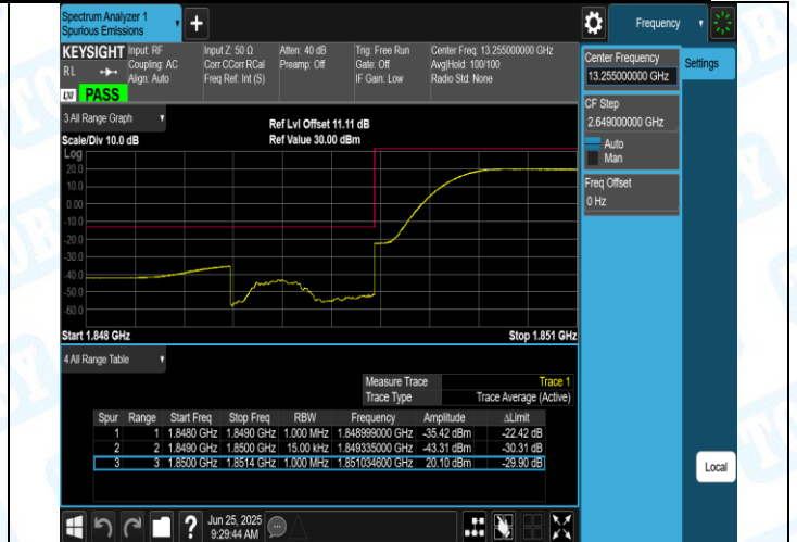
Band2-1.4MHz-16QAM-18607-1RB#5-PASS
