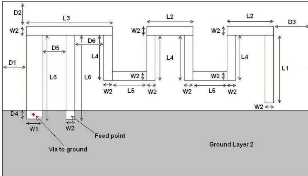
Figure 3: Antenna Dimensions
