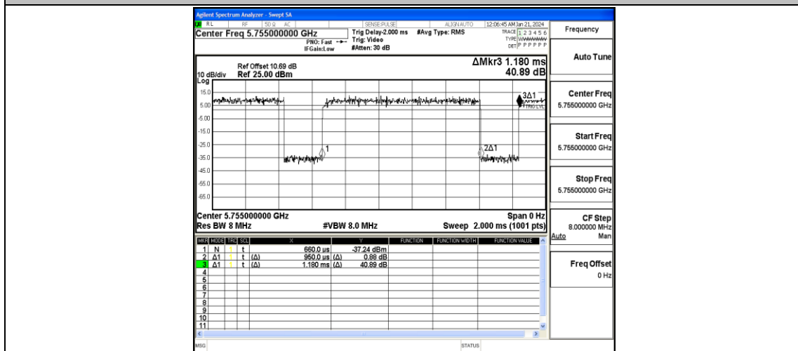
NTNV-11N40MIMO-Ant2-5755
