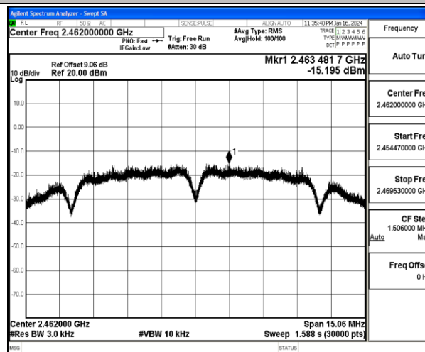
11B-Ant1-2462-PASS
