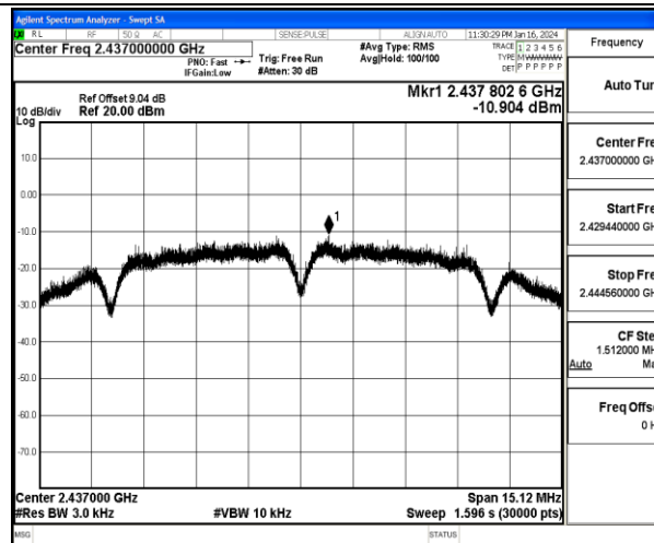
11B-Ant2-2437-PASS
