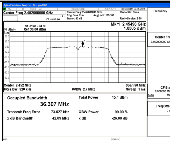
11N40MIMO-Ant2-2452
