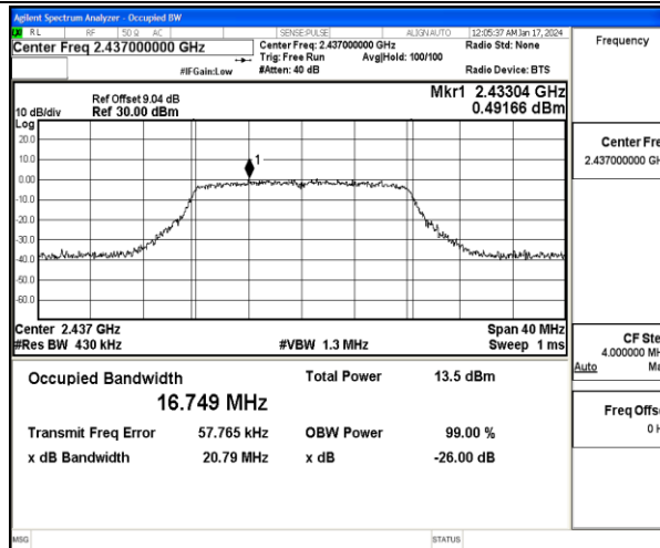
11G-Ant2-2437
