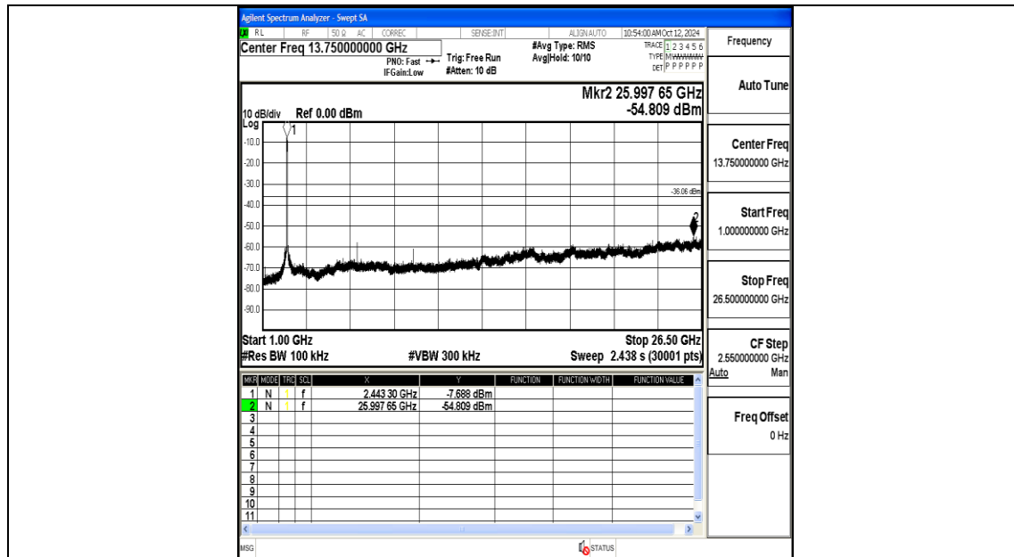
11N40MIMO-Ant2-2437-1000~26500-PASS
