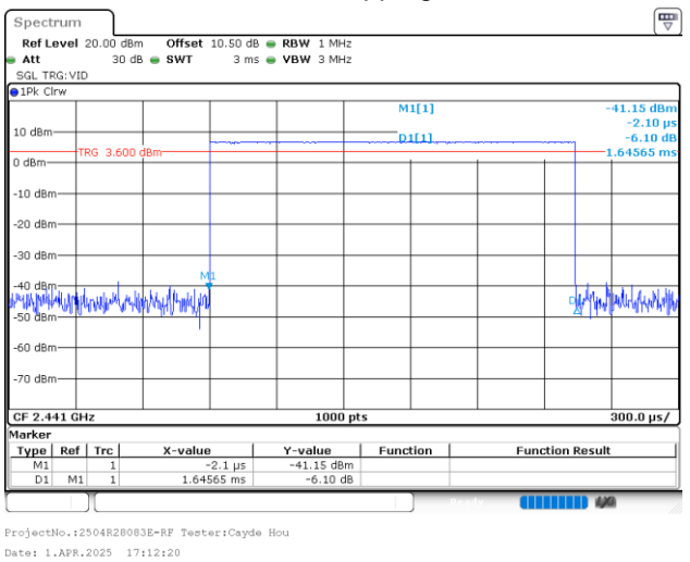
2DH1_Hopping
