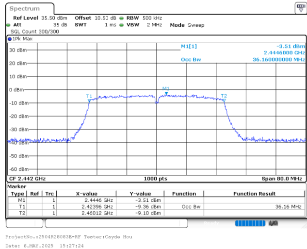
802.11n40_2442MHz_Chain 1
