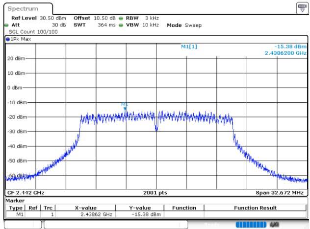
802.11g_2442MHz_Chain 0
