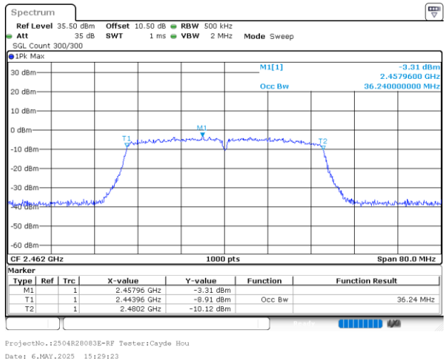
802.11n40_2462MHz_Chain 1
