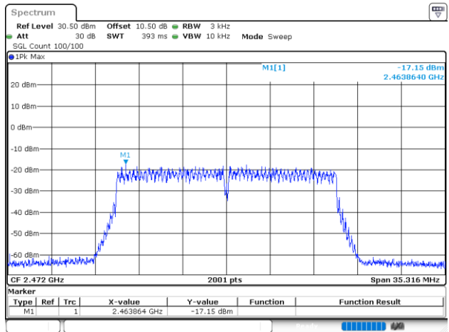
802.11n20_2472MHz_Chain 1
