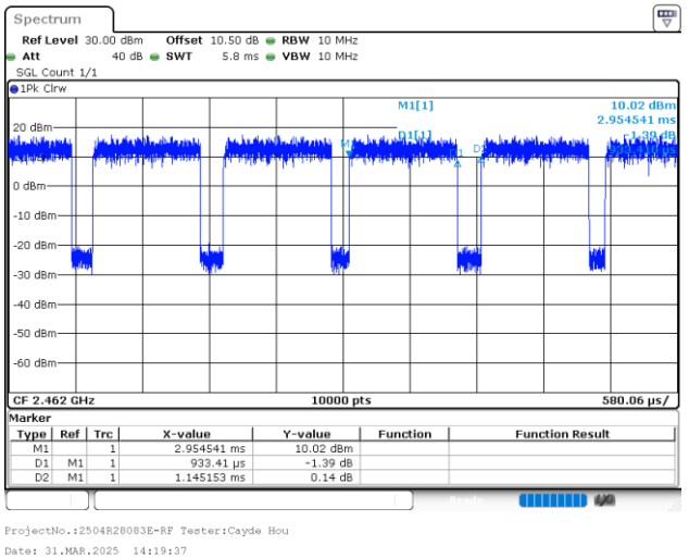
802.11n40_2462MHz_Chain 1
