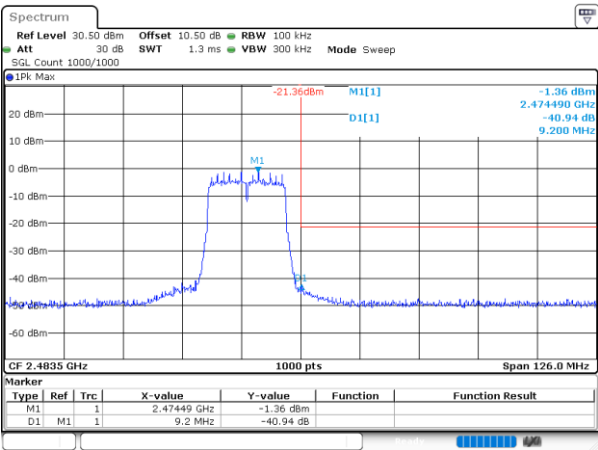
802.11g_2472MHz_Chain 0
