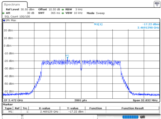
802.11g_2472MHz_Chain 1
