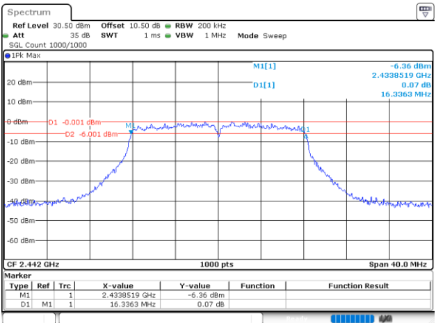
802.11g_2442MHz_Chain 0
