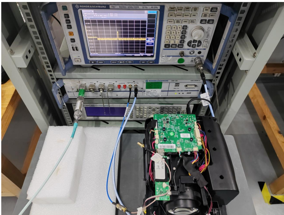
Photo of DFS Measurement
