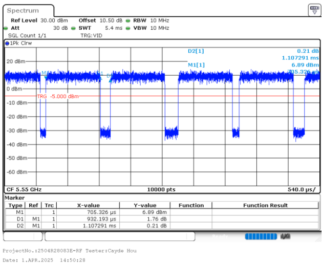
802.11n40_5550MHz_Chain 1
