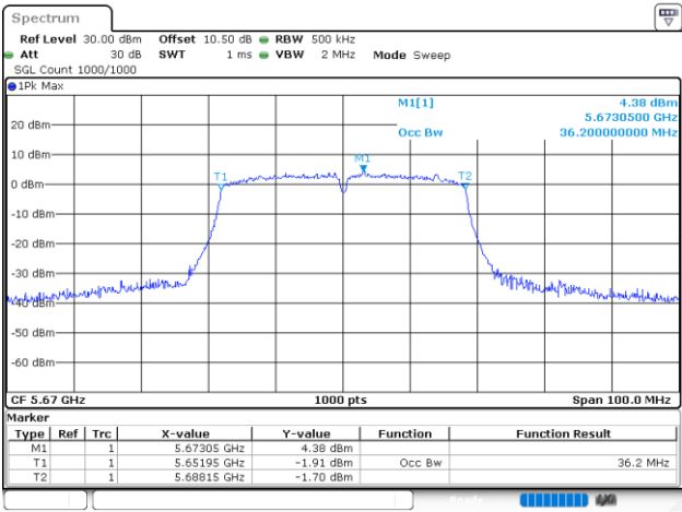
802.11n40_5670MHz_Chain 0
