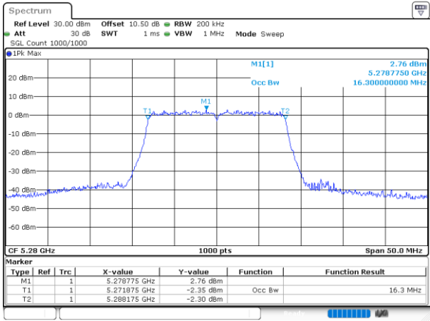
802.11a_5280MHz_Chain 0
