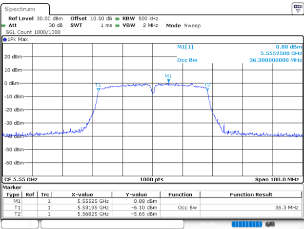
802.11n40_5550MHz_Chain 1
