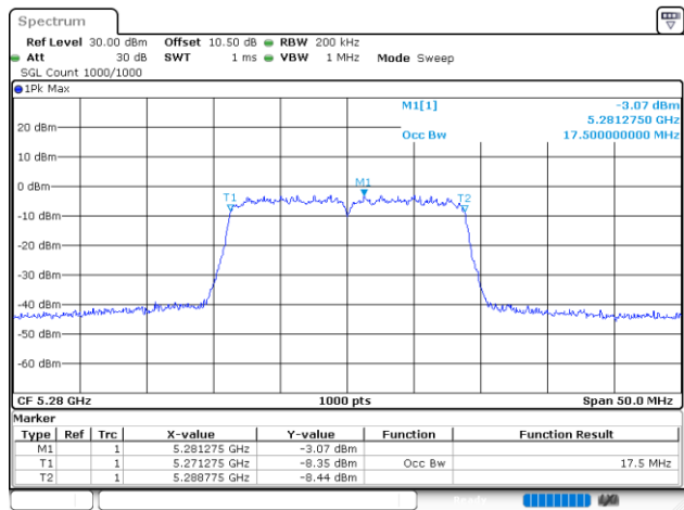
802.11n20_5280MHz_Chain 1
