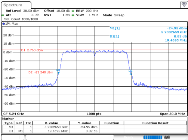
802.11n20_5240MHz_Chain 0
