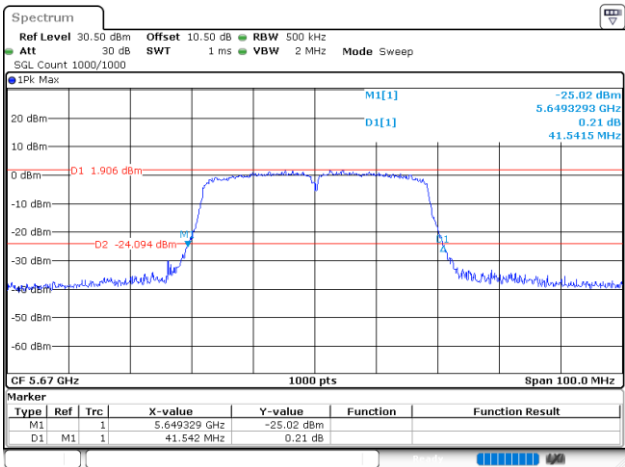
802.11n40_5670MHz_Chain 1
