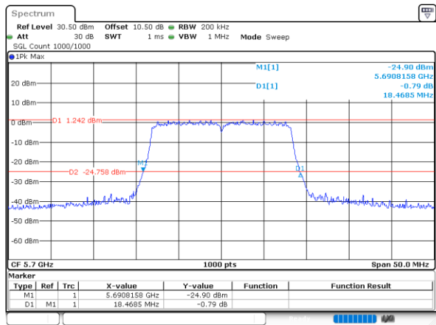
802.11a_5700MHz_Chain 1
