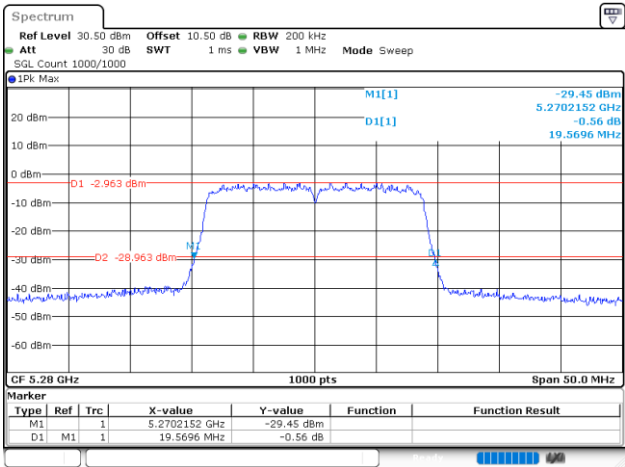
802.11n20_5280MHz_Chain 1
