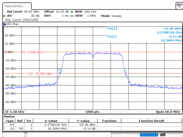
802.11a_5580MHz_Chain 1
