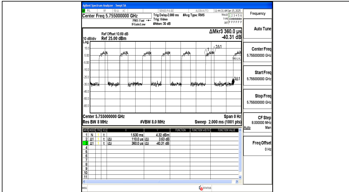
NTNV-11AC40MIMO-Ant2-5755
