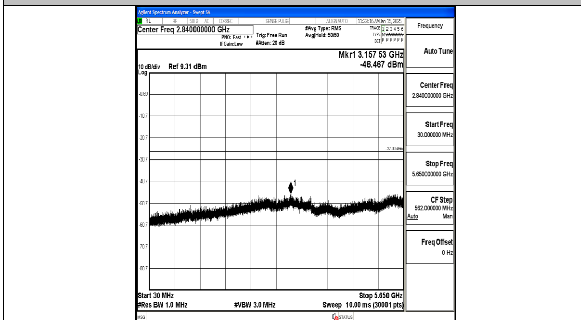
11AC20MIMO-Ant2-5745-30~5650-PASS
