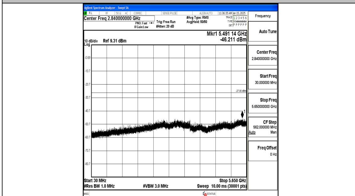
11AC20MIMO-Ant2-5785-30~5650-PASS
