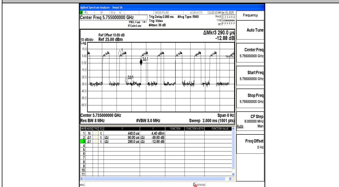
NTNV-11N40MIMO-Ant2-5755
