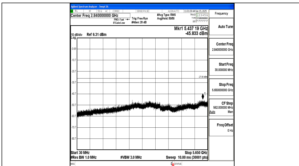
11A-Ant1-5825-30~5650-PASS
