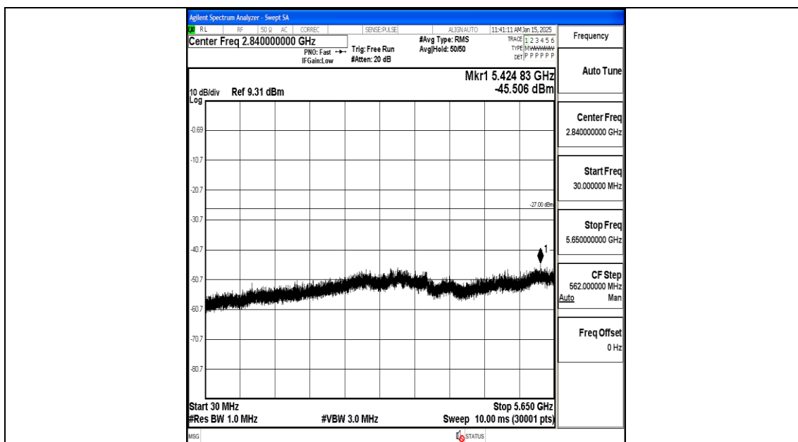
11AC20MIMO-Ant2-5825-30~5650-PASS
