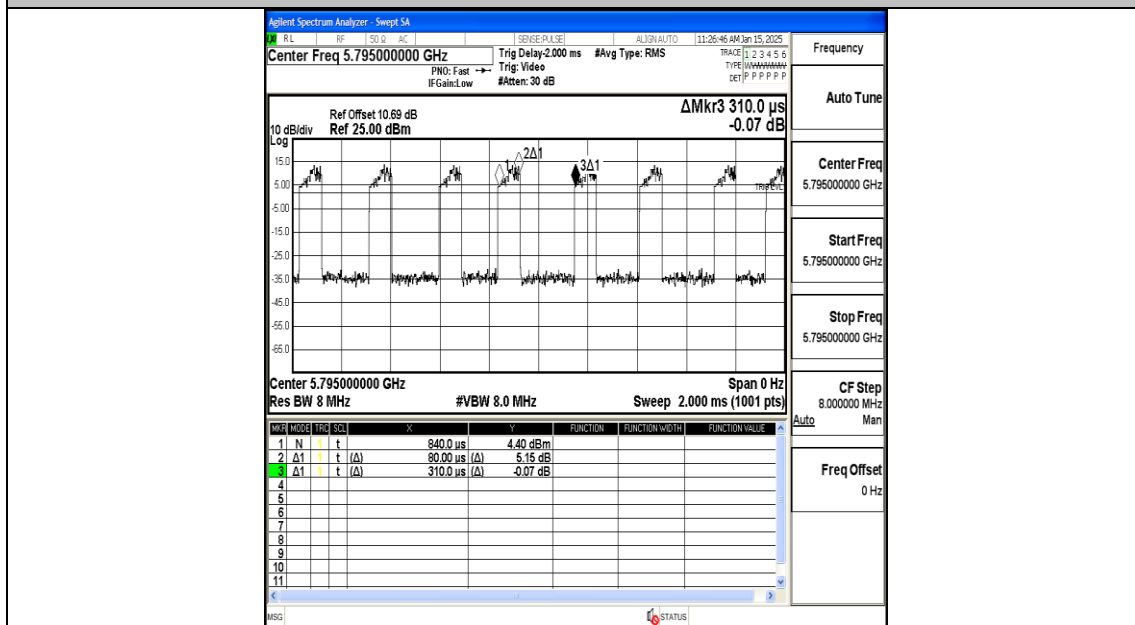
NTNV-11N40MIMO-Ant2-5795
