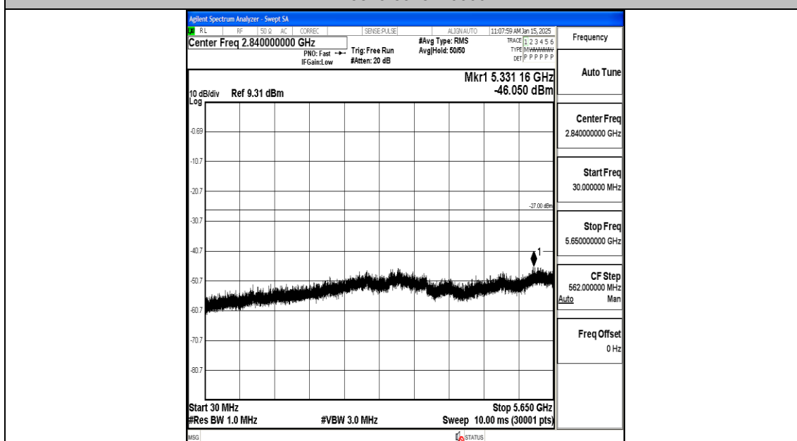
11N20MIMO-Ant1-5745-30~5650-PASS
