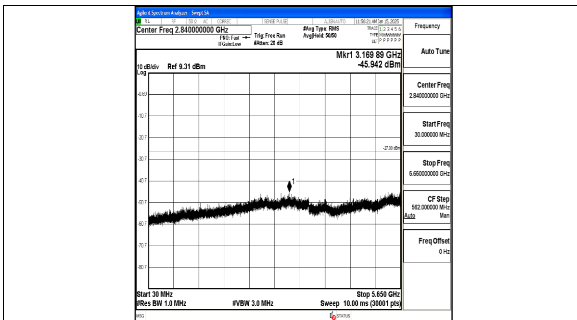
11AC80MIMO-Ant2-5775-30~5650-PASS
