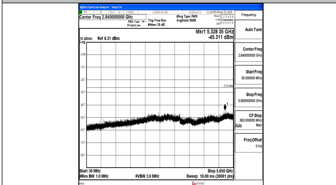
11AC20MIMO-Ant1-5785-30~5650-PASS
