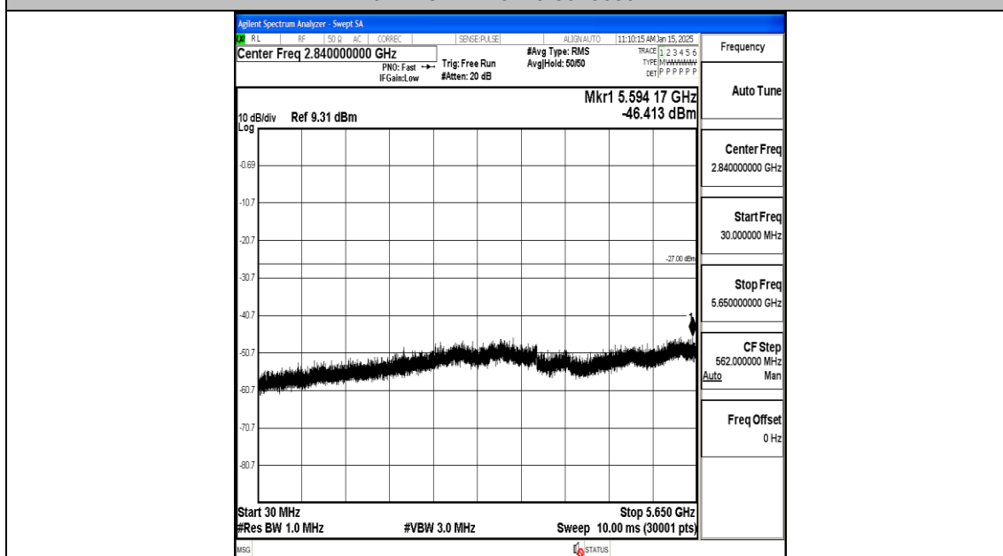
11N20MIMO-Ant2-5745-30~5650-PASS
