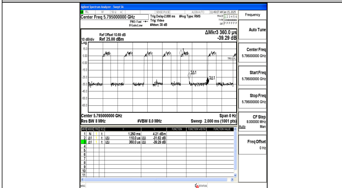
NTNV-11AC40MIMO-Ant2-5795
