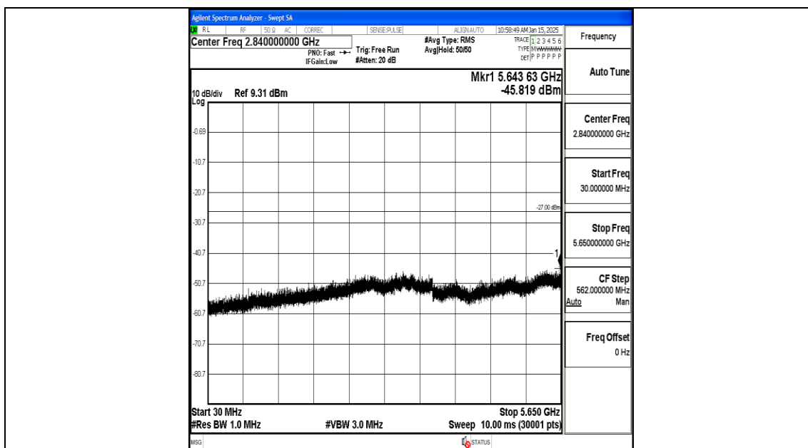
11A-Ant2-5785-30~5650-PASS
