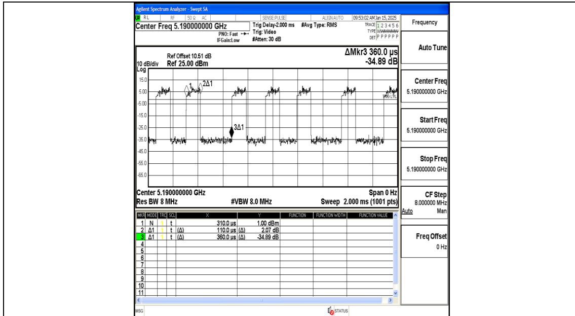
NTNV-11AC40MIMO-Ant2-5190
