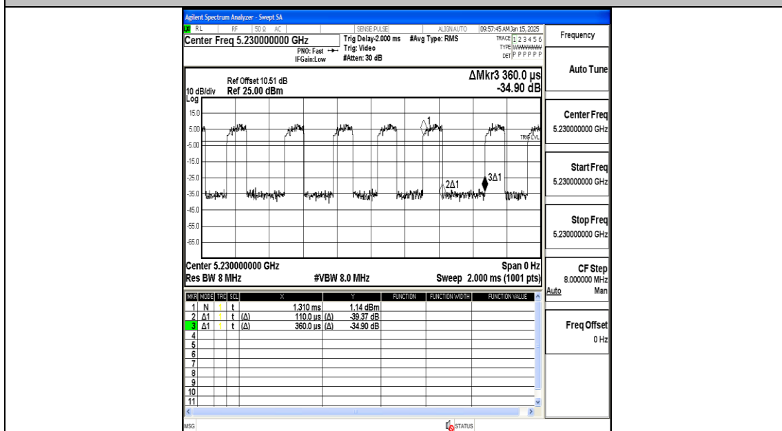
NTNV-11AC40MIMO-Ant2-5230
