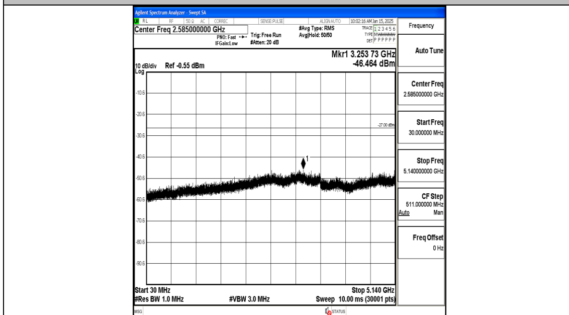
11AC80MIMO-Ant1-5210-30~5140-PASS
