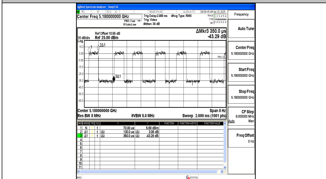
NTNV-11N20MIMO-Ant1-5180
