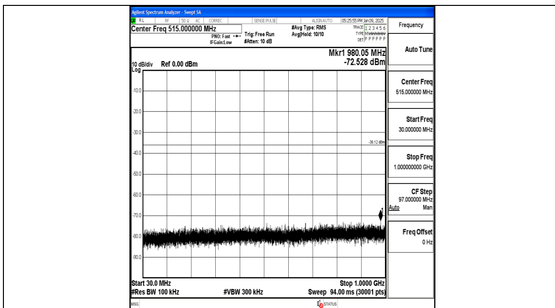
11N40MIMO-Ant1-2422-30~1000-PASS
