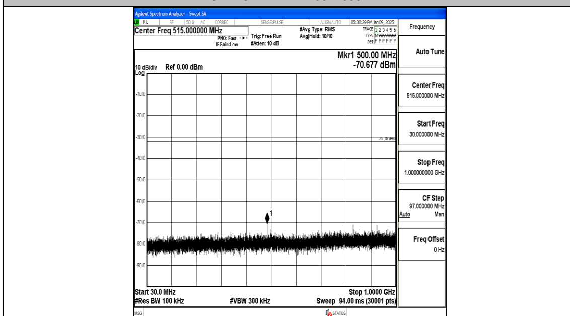
11N40MIMO-Ant2-2422-30~1000-PASS
