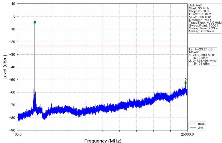
1M_HCH_2480MHz_Ant1_NTNV
