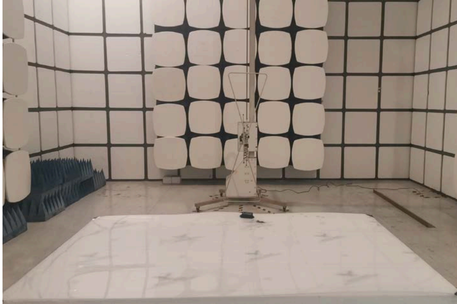
Spurious Emission Test Setup (Below 1GHz)
