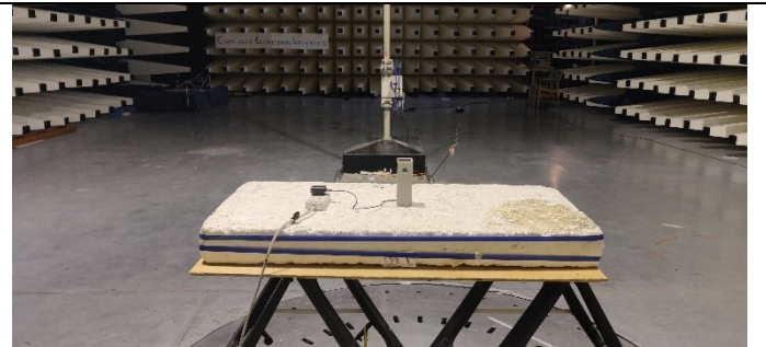
Fig B4: Radiated Emissions
