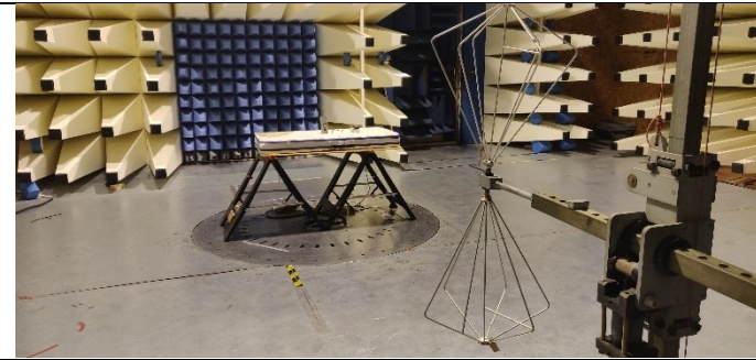
Fig B1: Radiated Emissions
