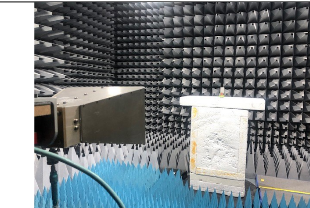
Fig B5: Radiated Emissions
