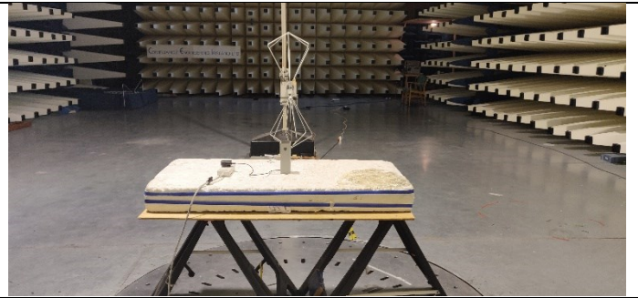
Fig B2: Radiated Emissions
