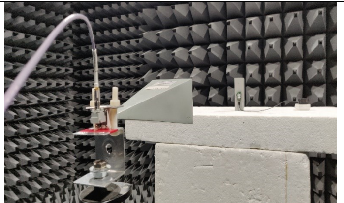
Fig B6: Radiated Emissions
