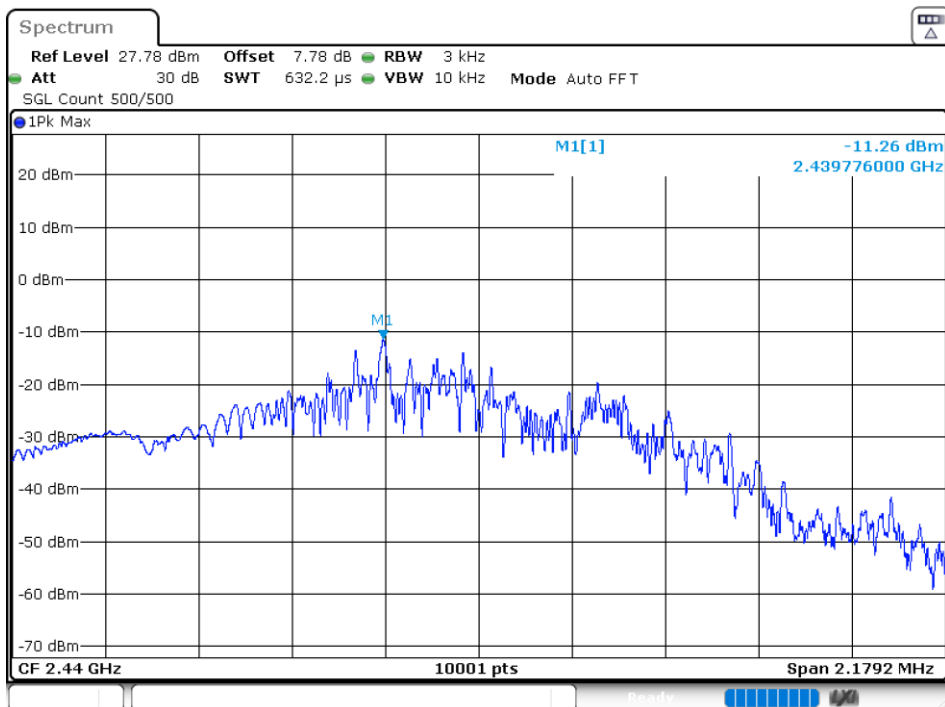
PSD NVNT 2440MHz Ant1
