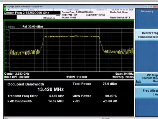
Band41-15MHz-QPSK-41515-75RB#0-PASS
