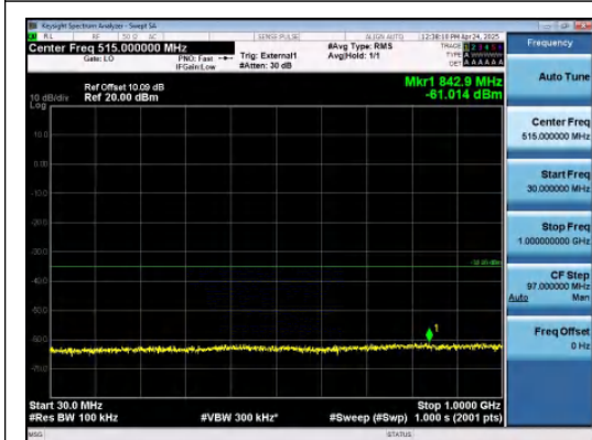
Band41-5MHz-16QAM-40620-1RB#24-30~1000-PASS
