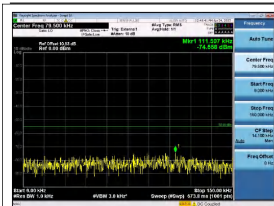
Band41-5MHz-QPSK-41565-1RB#24-0.009~0.1 5-PASS
