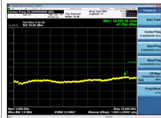
Band41-5MHz-QPSK-39675-25RB#0-3000~180 00-PASS
