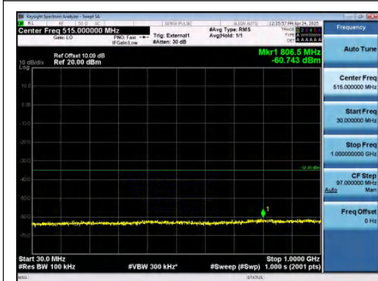
Band41-5MHz-QPSK-40620-1RB#24-30~1000-P ASS
