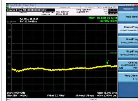
Band41-10MHz-QPSK-39700-1RB#49-3000~18000-PASS
