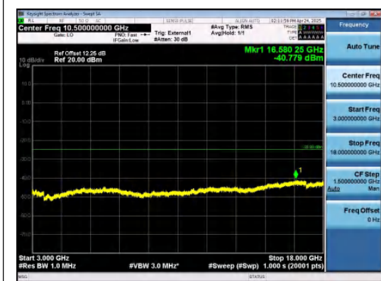
Band41-10MHz-QPSK-39700-50RB#0-3000~18000-PASS
