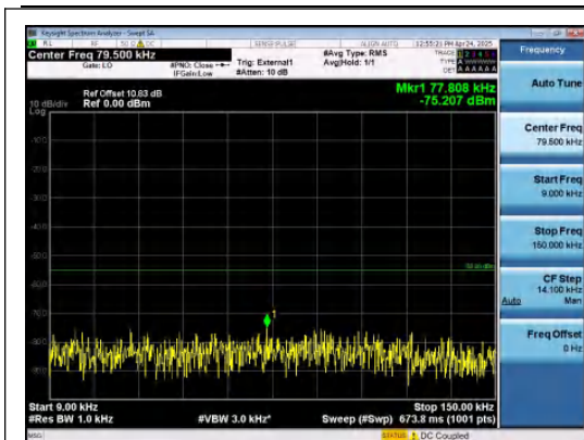
Band41-5MHz-16QAM-41565-25RB#0-0.009~0.15-PASS
