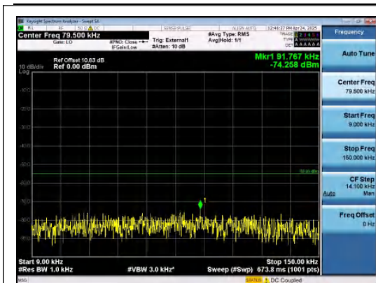
Band41-5MHz-16QAM-41565-1RB#0-0.009~0.1 5-PASS
