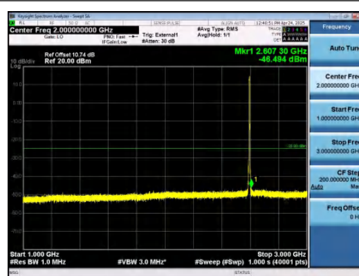
Band41-5MHz-QPSK-40620-25RB#0-1000~300 0-PASS
