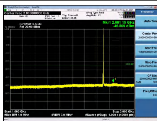
Band41-10MHz-16QAM-39700-1RB#49-1000~3000-PASS
