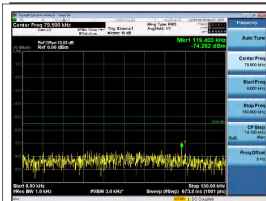
Band41-10MHz-QPSK-39700-1RB#49-0.009~0.15-PASS
