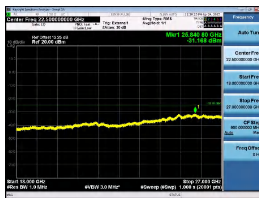
Band41-5MHz-16QAM-40620-1RB#24-18000~27000-PASS
