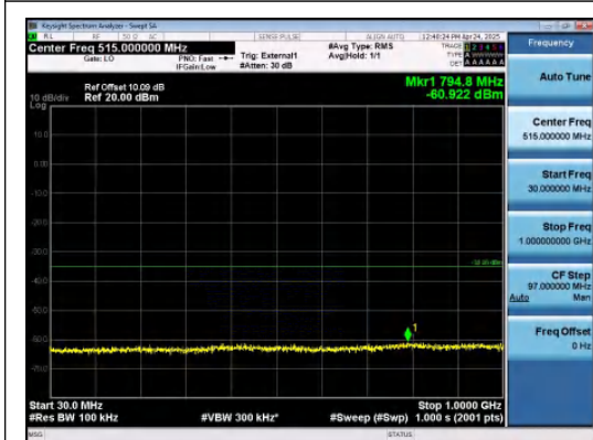
Band41-5MHz-QPSK-40620-25RB#0-30~1000-P ASS
