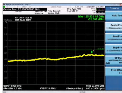
Band41-5MHz-QPSK-39675-25RB#0-18000~27 000-PASS
