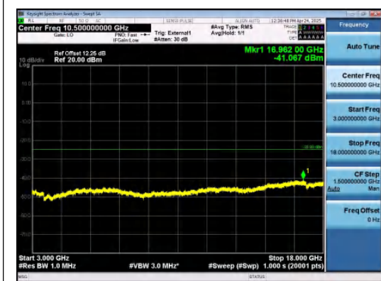
Band41-5MHz-QPSK-40620-1RB#24-3000~180 00-PASS
