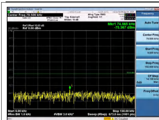
Band41-5MHz-QPSK-39675-1RB#24-0.009~0.1 5-PASS
