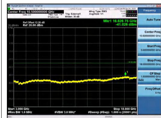
Band41-5MHz-16QAM-40620-25RB#0-3000~18000-PASS
