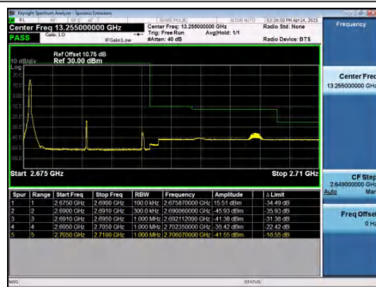
Band41-15MHz-QPSK-41515-1RB#0-PASS
