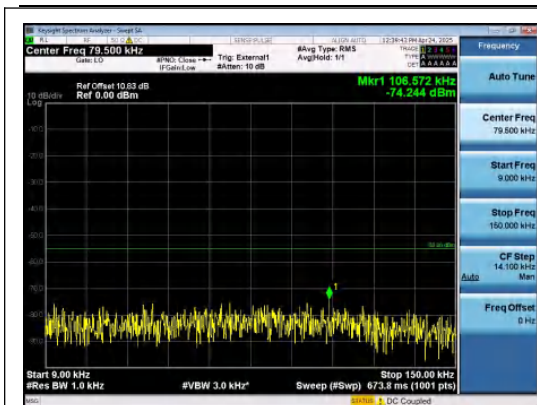
Band41-5MHz-QPSK-40620-25RB#0-0.009~0.1 5-PASS
