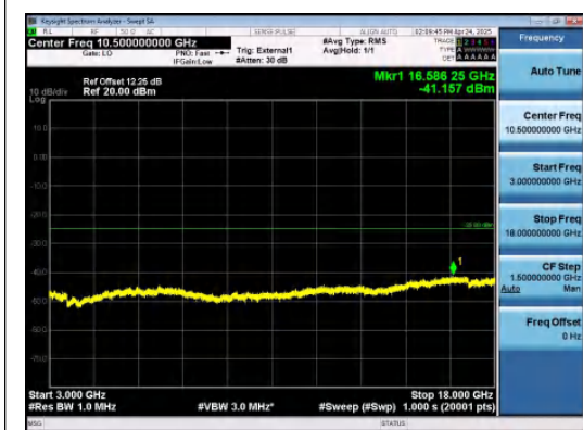
Band41-10MHz-16QAM-39700-1RB#49-3000~18000-PASS
