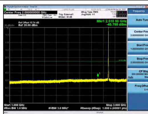
Band41-5MHz-QPSK-41565-1RB#24-1000~300 0-PASS
