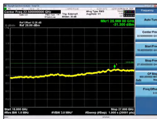
Band41-5MHz-16QAM-41565-25RB#0-18000~27000-PASS
