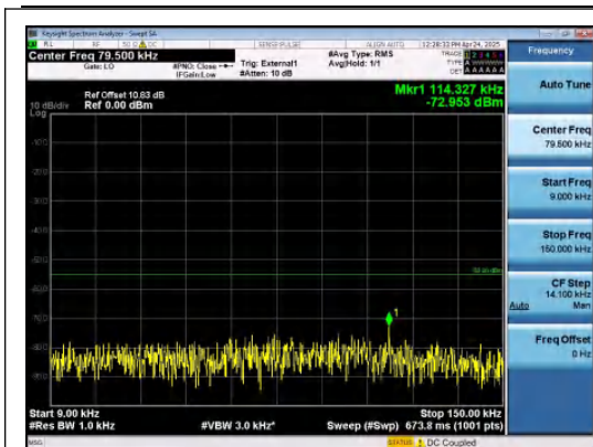
Band41-5MHz-16QAM-39675-25RB#0-0.009~0.15-PASS
