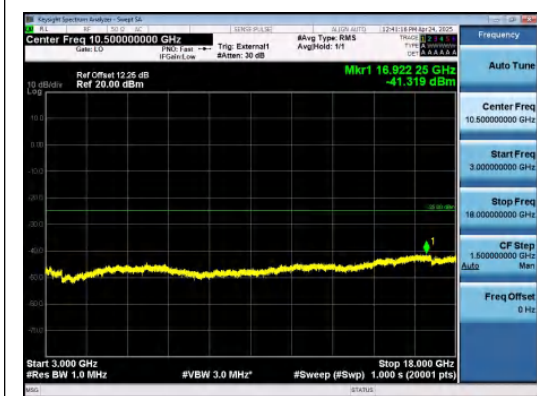
Band41-5MHz-QPSK-40620-25RB#0-3000~180 00-PASS
