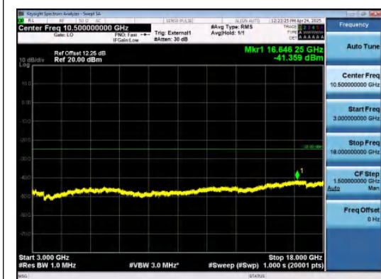
Band41-5MHz-QPSK-39675-1RB#24-3000~180 00-PASS
