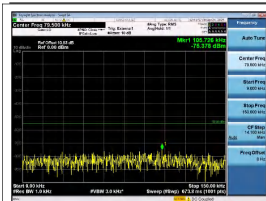
Band41-5MHz-16QAM-40620-25RB#0-0.009~0.15-PASS
