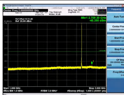
Band41-5MHz-QPSK-39675-1RB#24-1000~300 0-PASS
