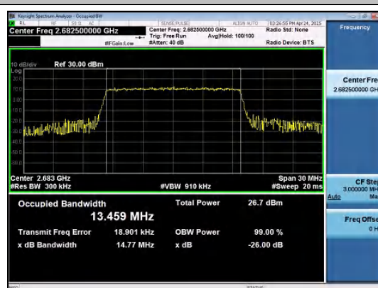
Band41-15MHz-16QAM-41515-75RB#0-PASS
