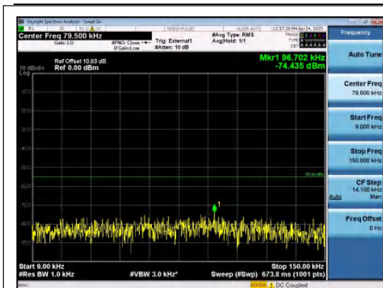
Band41-5MHz-16QAM-40620-1RB#24-0.009~0.15-PASS
