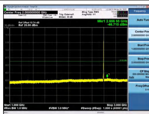
Band41-5MHz-16QAM-40620-1RB#24-1000~3000-PASS
