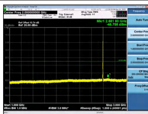
Band41-5MHz-QPSK-40620-1RB#24-1000~300 0-PASS
