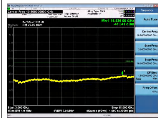
Band41-5MHz-16QAM-39675-25RB#0-3000~18000-PASS
