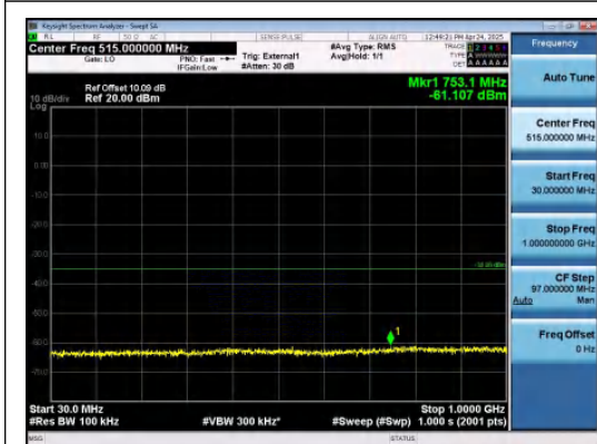
Band41-5MHz-QPSK-41565-1RB#24-30~1000-P ASS
