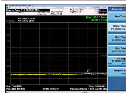
Band41-5MHz-16QAM-40620-25RB#0-30~1000-PASS
