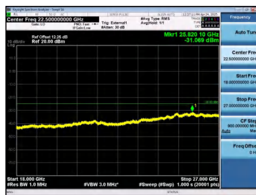
Band41-5MHz-QPSK-40620-1RB#24-18000~27 000-PASS
