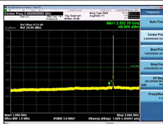
Band41-5MHz-16QAM-40620-25RB#0-1000~3000-PASS
