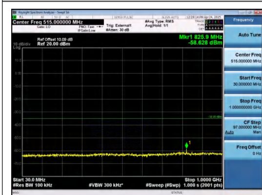
Band41-5MHz-16QAM-39675-25RB#0-30~1000-PASS
