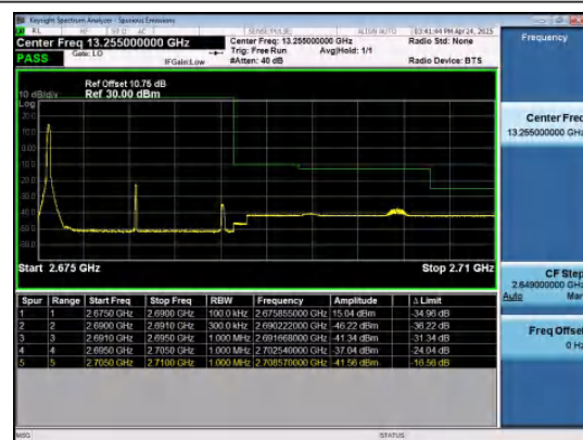
Band41-15MHz-16QAM-41515-1RB#0-PASS
