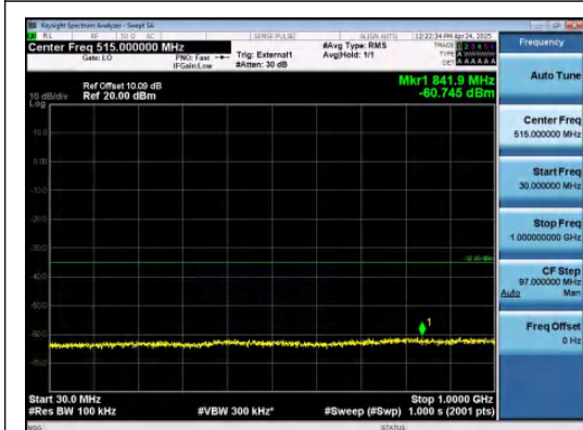
Band41-5MHz-QPSK-39675-1RB#24-30~1000-P ASS
