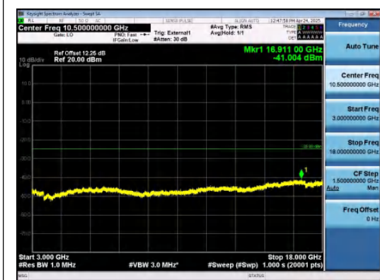
Band41-5MHz-16QAM-41565-1RB#0-3000~180 00-PASS
