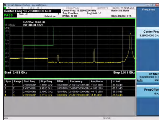
Band41-15MHz-16QAM-39725-1RB#74-PASS
