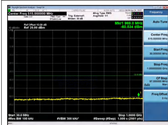
Band41-10MHz-QPSK-39700-50RB#0-30~1000-PASS
