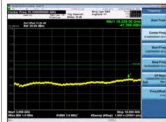
Band41-5MHz-16QAM-41565-25RB#0-3000~18000-PASS
