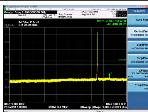
Band41-5MHz-QPSK-39675-25RB#0-1000~300 0-PASS
