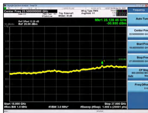
Band41-10MHz-QPSK-39700-1RB#49-18000~27000-PASS
