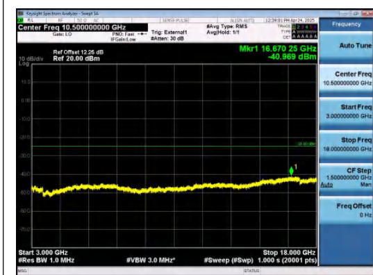
Band41-5MHz-16QAM-40620-1RB#24-3000~18000-PASS
