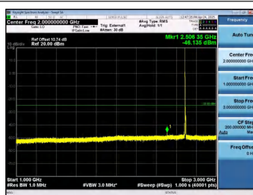
Band41-5MHz-16QAM-41565-1RB#0-1000~300 0-PASS
