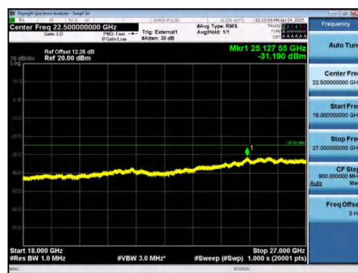
Band41-10MHz-16QAM-39700-1RB#49-18000~27000-PASS
