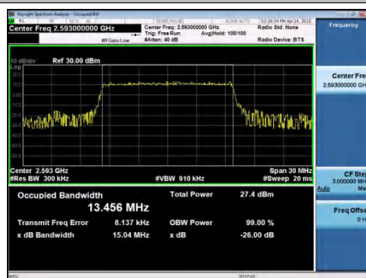
Band41-15MHz-16QAM-40620-75RB#0-PASS
