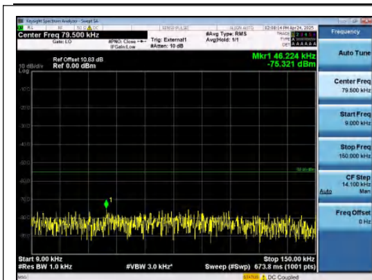
Band41-10MHz-16QAM-39700-1RB#49-0.009~0.15-PASS
