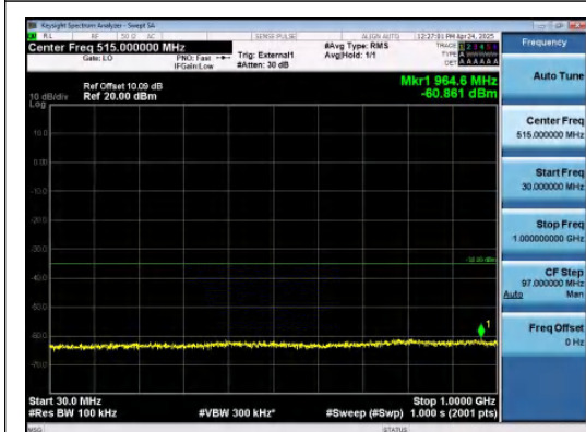
Band41-5MHz-QPSK-39675-25RB#0-30~1000-P ASS
