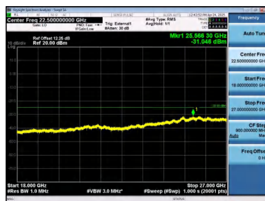
Band41-5MHz-16QAM-40620-25RB#0-18000~27000-PASS
