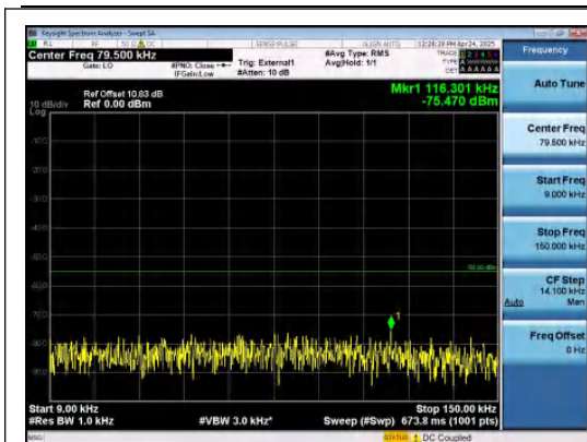
Band41-5MHz-QPSK-39675-25RB#0-0.009~0.1 5-PASS
