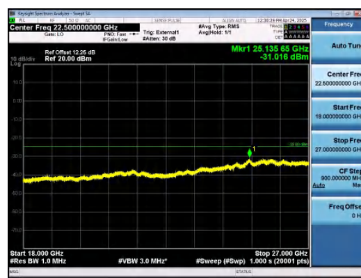
Band41-5MHz-16QAM-39675-25RB#0-18000~27000-PASS
