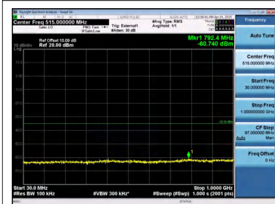
Band41-10MHz-QPSK-39700-1RB#49-30~1000-PASS
