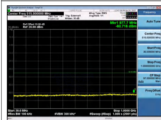
Band41-5MHz-16QAM-41565-1RB#0-30~1000-P ASS
