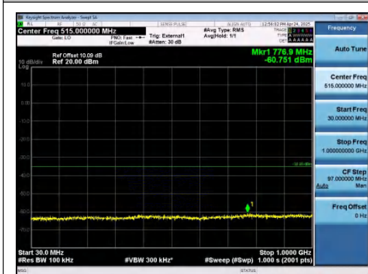
Band41-5MHz-16QAM-41565-25RB#0-30~1000-PASS
