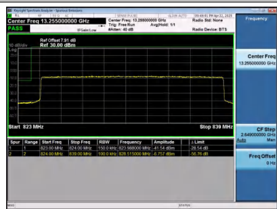
Band26(824-849)-15MHz-16QAM-26865-75RB#0-P
