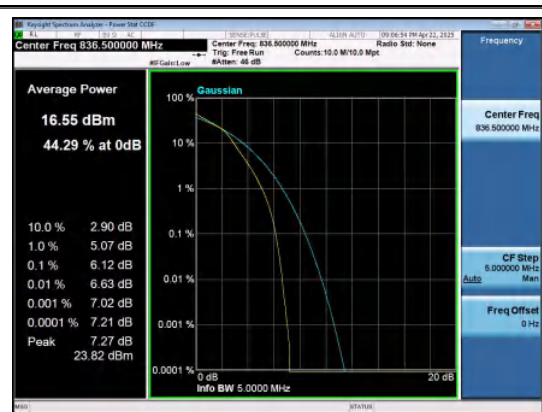
Band26(824-849)-5MHz-16QAM-26915-25RB#0-P ASS
