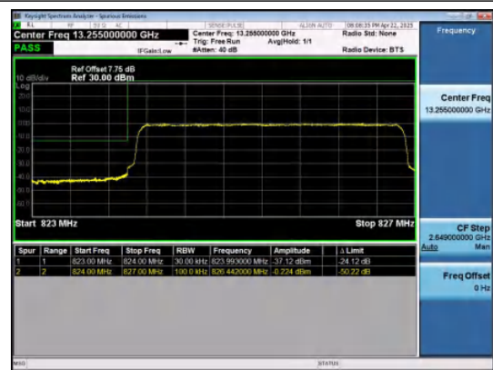
Band26(824-849)-3MHz-16QAM-26805-15RB#0-P ASS
