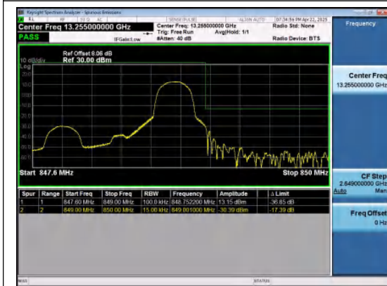
Band26(824-849)-1.4MHz-16QAM-27033-1RB#5- PASS
