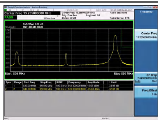
Band26(824-849)-10MHz-QPSK-26990-1RB#49-P
