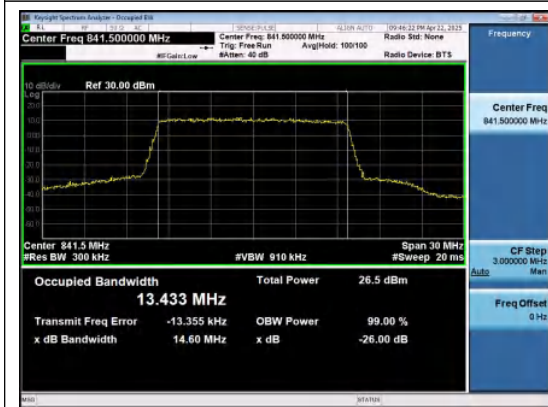
Band26(824-849)-15MHz-QPSK-26965-75RB#0-PASS
