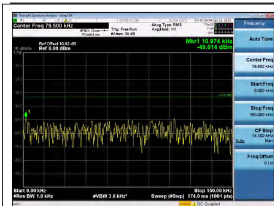
Band26(824-849)-1.4MHz-QPSK-26915-1RB#0- 0.009~0.15-PASS
