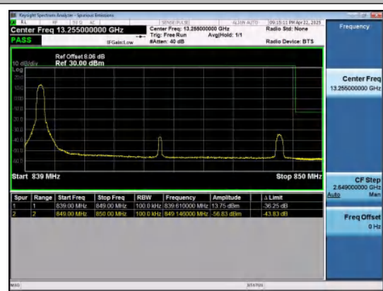
Band26(824-849)-10MHz-16QAM-26990-1RB#0-P
