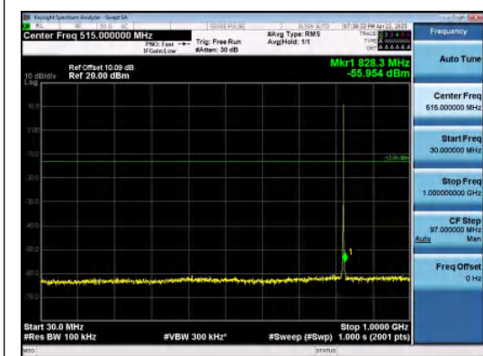
Band26(824-849)-1.4MHz-16QAM-26797-1RB#5 -30~1000-PASS
