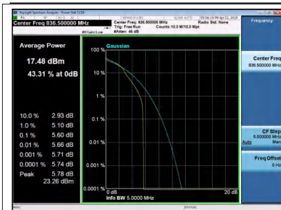
Band26(824-849)-5MHz-16QAM-26915-1RB#0-P ASS
