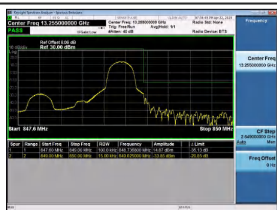
Band26(824-849)-1.4MHz-QPSK-27033-1RB#5-P ASS
