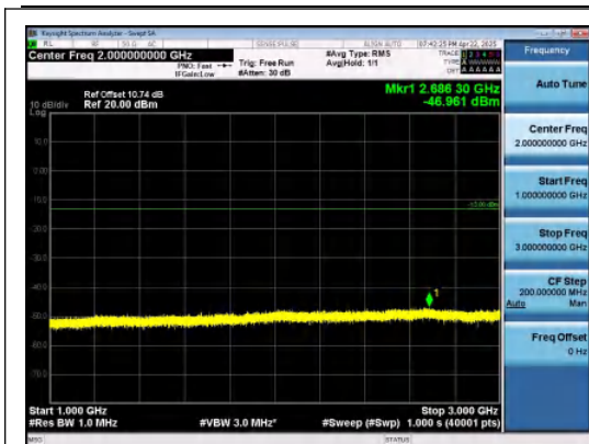
Band26(824-849)-1.4MHz-16QAM-26915-1RB#0 -1000~3000-PASS
