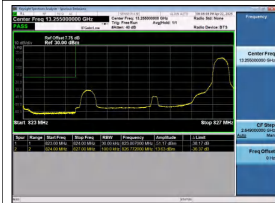
Band26(824-849)-3MHz-16QAM-26805-1RB#14-P ASS
