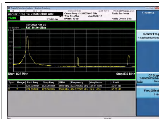
Band26(824-849)-15MHz-QPSK-26865-1RB#0-P
