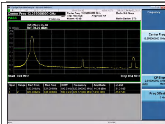
Band26(824-849)-10MHz-QPSK-26840-1RB#0-P
