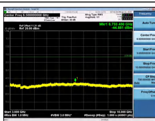
Band26(824-849)-1.4MHz-16QAM-26915-1RB#0 -3000~10000-PASS
