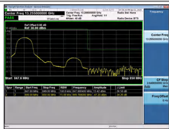
Band26(824-849)-1.4MHz-16QAM-27033-1RB#0- PASS
