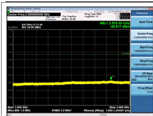
Band26(824-849)-1.4MHz-16QAM-26797-1RB#0 -1000~3000-PASS
