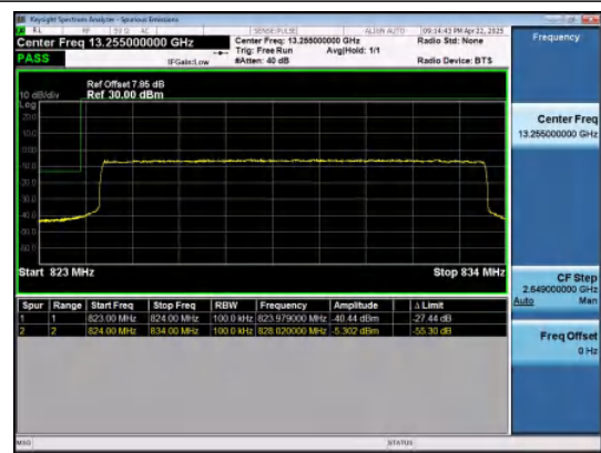
Band26(824-849)-10MHz-16QAM-26840-50RB#0-P
