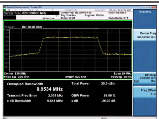
Band26(824-849)-10MHz-16QAM-26840-50RB#0-PASS
