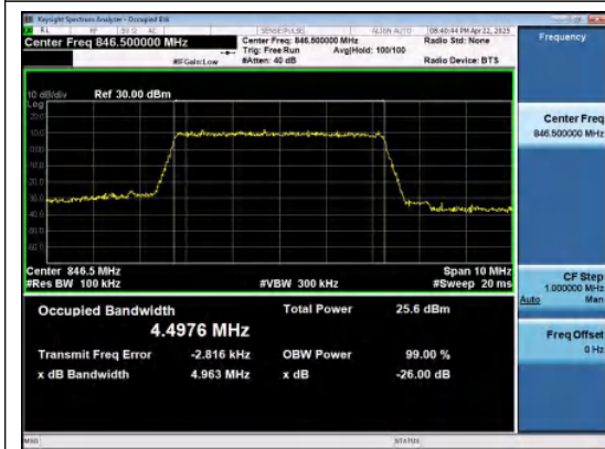
Band26(824-849)-5MHz-QPSK-27015-25RB#0-P ASS
