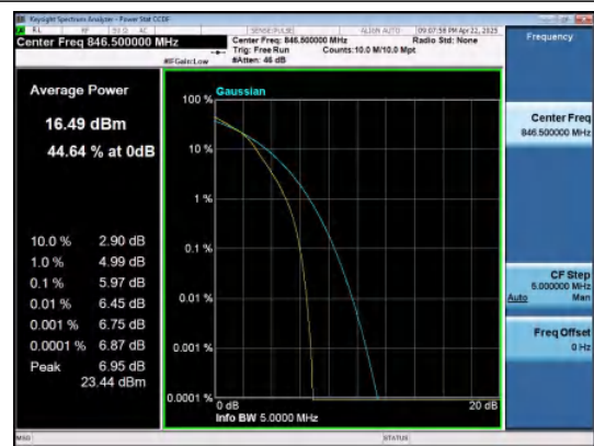
Band26(824-849)-5MHz-16QAM-27015-25RB#0-P ASS
