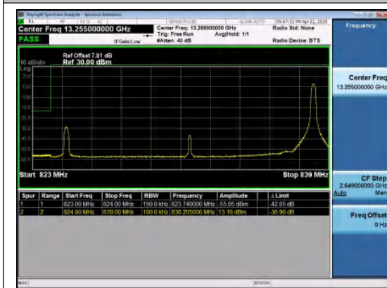
Band26(824-849)-15MHz-16QAM-26865-1RB#74-P
