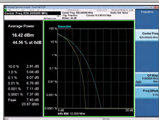
Band26(824-849)-10MHz-16QAM-26840-50RB#0-P PASS
