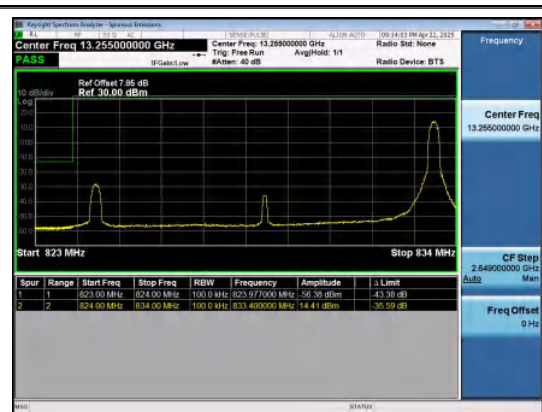
Band26(824-849)-10MHz-QPSK-26840-1RB#49-P
