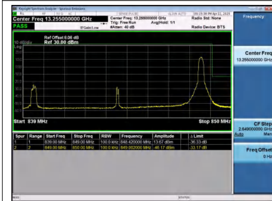
Band26(824-849)-10MHz-16QAM-26990-1RB#49-
