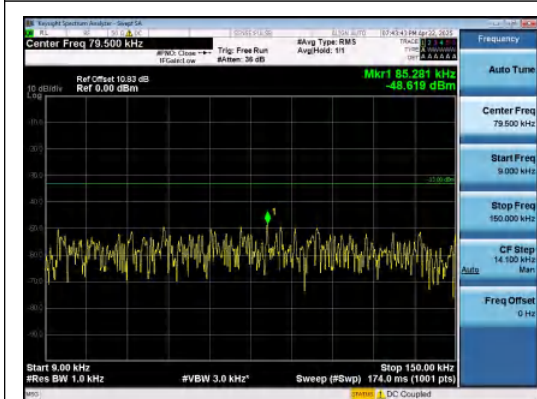
Band26(824-849)-1.4MHz-16QAM-26915-1RB#5 -0.009~0.15-PASS
