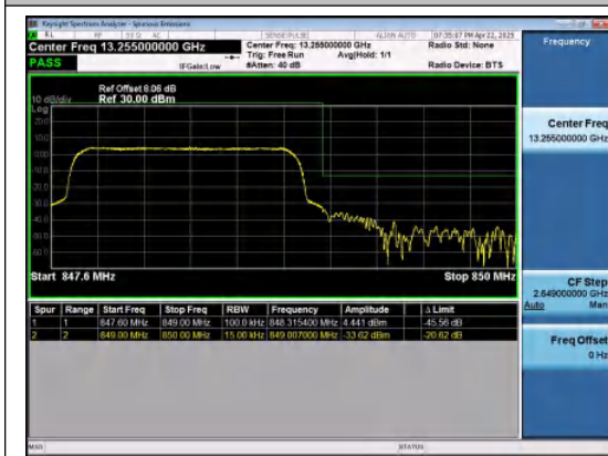
Band26(824-849)-1.4MHz-QPSK-27033-6RB#0-P ASS
