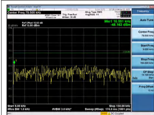
Band26(824-849)-1.4MHz-16QAM-26797-1RB#5 -0.009~0.15-PASS
