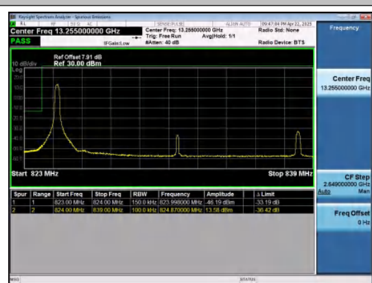
Band26(824-849)-15MHz-16QAM-26865-1RB#0-P
