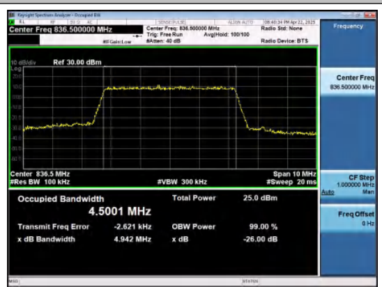
Band26(824-849)-5MHz-16QAM-26915-25RB#0-P ASS
