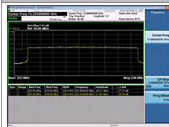
Band26(824-849)-15MHz-QPSK-26865-75RB#0-P
