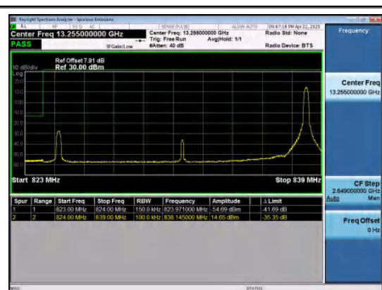
Band26(824-849)-15MHz-QPSK-26865-1RB#74-P
