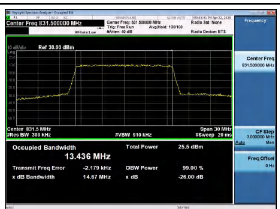
Band26(824-849)-15MHz-16QAM-26865-75RB#0-PASS
