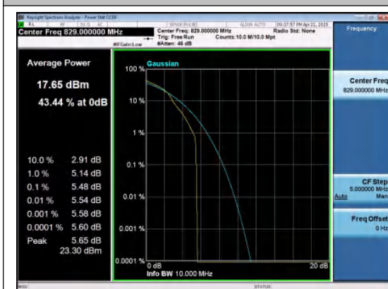
Band26(824-849)-10MHz-16QAM-26840-1RB#0-P ASS
