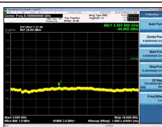
Band26(824-849)-1.4MHz-16QAM-26797-1RB#0 -3000~10000-PASS
