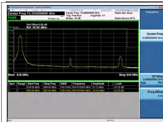
Band26(824-849)-10MHz-QPSK-26990-1RB#0-P
