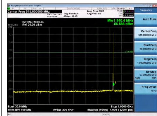
Band26(824-849)-1.4MHz-16QAM-26915-1RB#5 -30~1000-PASS
