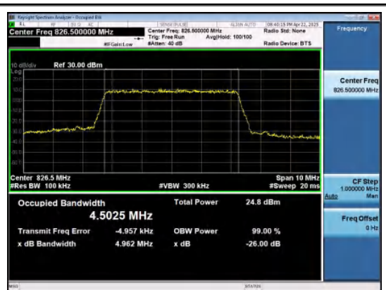
Band26(824-849)-5MHz-16QAM-26815-25RB#0-P ASS
