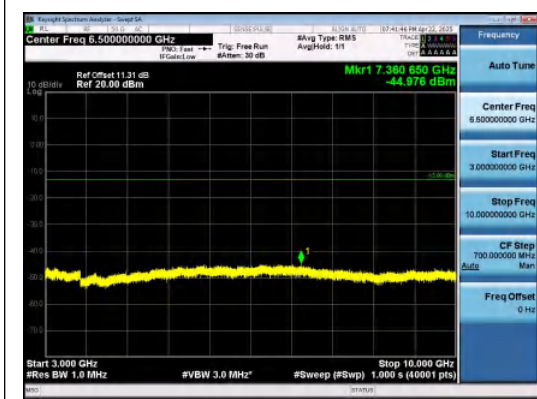
Band26(824-849)-1.4MHz-QPSK-26915-1RB#0- 3000~10000-PASS
