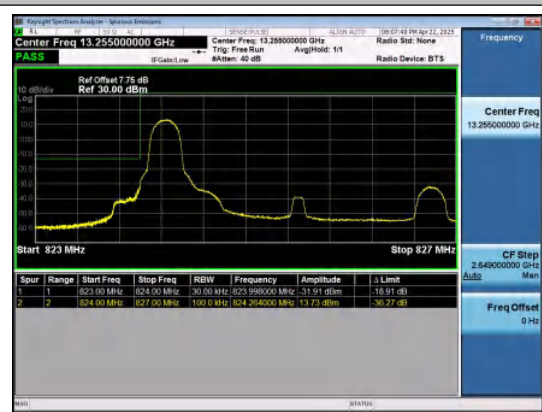
Band26(824-849)-3MHz-16QAM-26805-1RB#0-P ASS
