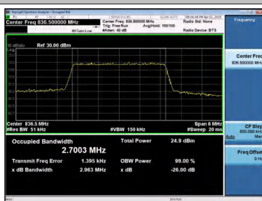
Band26(824-849)-3MHz-16QAM-26915-15RB#0-P
