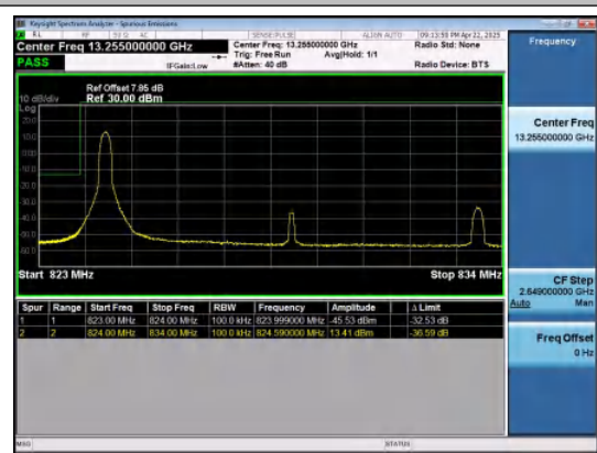
Band26(824-849)-10MHz-16QAM-26840-1RB#0-P
