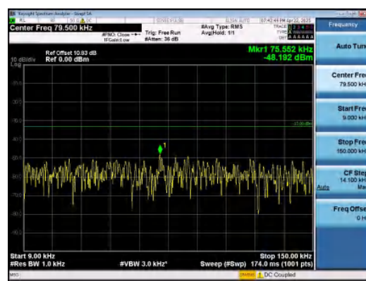
Band26(824-849)-1.4MHz-QPSK-26915-1RB#5- 0.009~0.15-PASS
