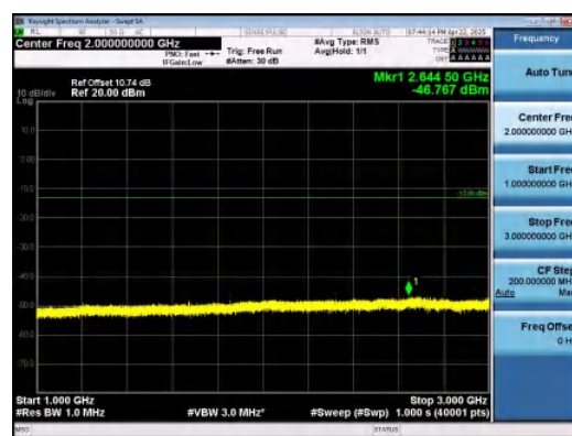
Band26(824-849)-1.4MHz-16QAM-26915-1RB#5 -1000~3000-PASS
