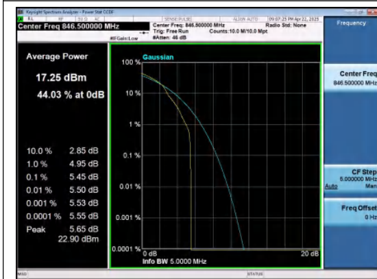
Band26(824-849)-5MHz-16QAM-27015-1RB#0-P ASS
