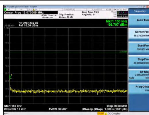
Band26(824-849)-1.4MHz-16QAM-26797-1RB#5 -0.15~30-PASS
