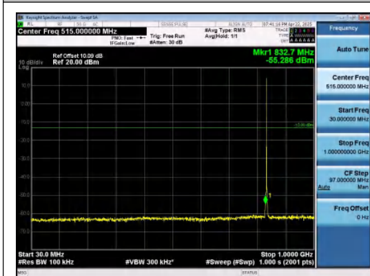
Band26(824-849)-1.4MHz-QPSK-26915-1RB#0- 30~1000-PASS
