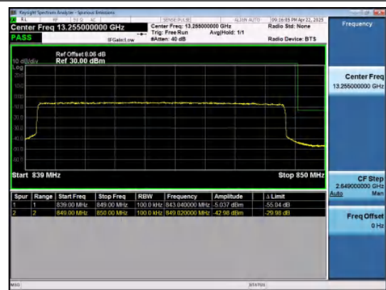
Band26(824-849)-10MHz-16QAM-26990-50RB#0-
