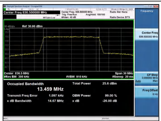
Band26(824-849)-15MHz-16QAM-26915-75RB#0-PASS
