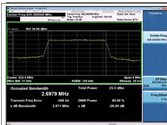
Band26(824-849)-3MHz-QPSK-26805-15RB#0-P
