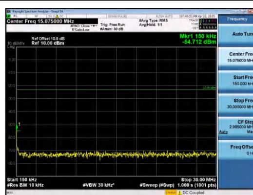
Band26(824-849)-1.4MHz-16QAM-26915-1RB#5 -0.15~30-PASS
