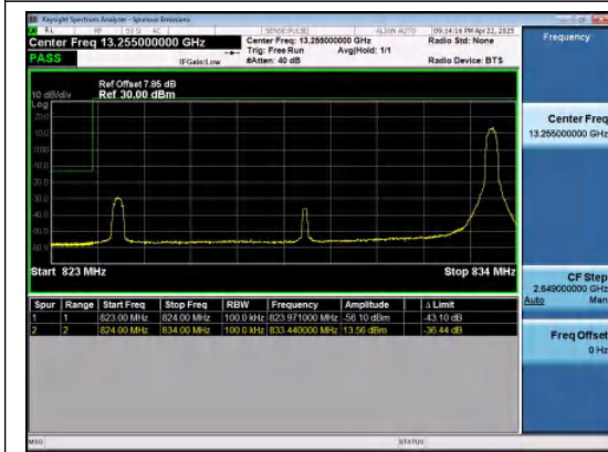
Band26(824-849)-10MHz-16QAM-26840-1RB#49-P
