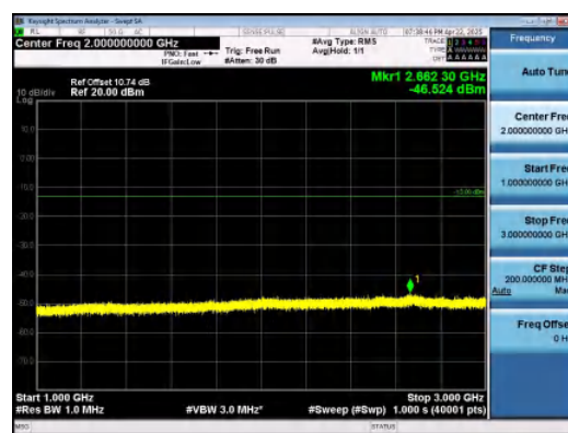
Band26(824-849)-1.4MHz-16QAM-26797-1RB#5 -1000~3000-PASS
