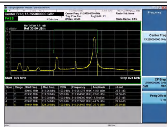
Band26(814-824)-5MHz-QPSK-26715-1RB#24-P
