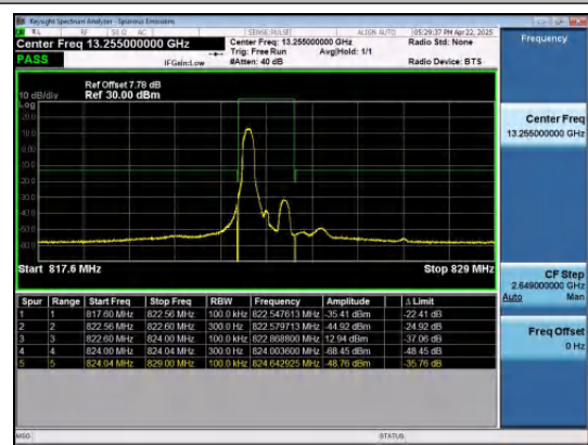
Band26(814-824)-1.4MHz-16QAM-26783-1RB#0- PASS
