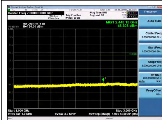
Band26(814-824)-1.4MHz-QPSK-26697-1RB#5- 1000~3000-PASS
