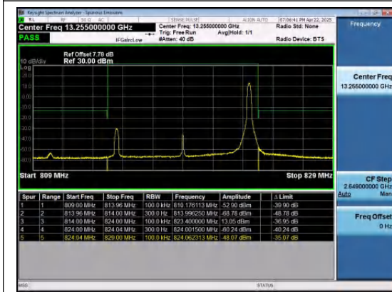
Band26(814-824)-10MHz-16QAM-26740-1RB#49-P
