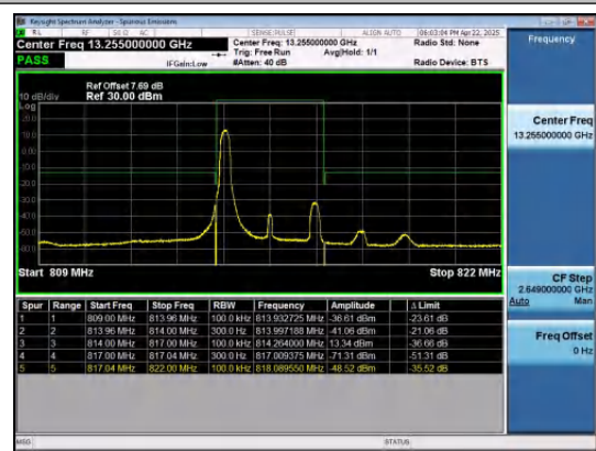
Band26(814-824)-3MHz-16QAM-26705-1RB#0-P
