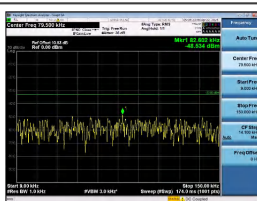
Band26(814-824)-1.4MHz-16QAM-26697-6RB#0 -0.009~0.15-PASS
