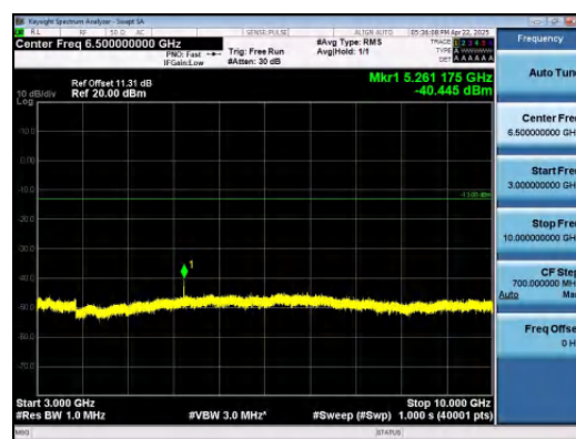
Band26(814-824)-1.4MHz-16QAM-26697-6RB#0 -3000~10000-PASS
