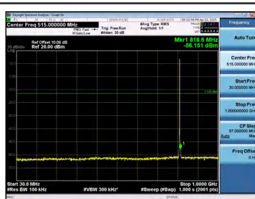
Band26(814-824)-1.4MHz-QPSK-26697-1RB#5- 30~1000-PASS
