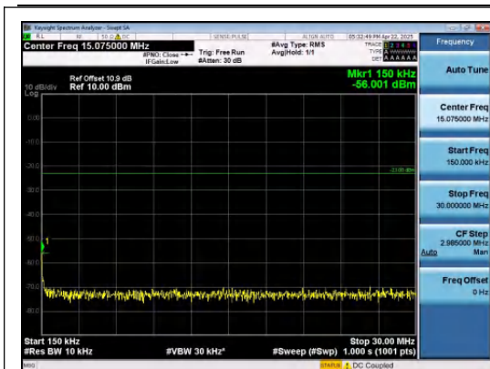
Band26(814-824)-1.4MHz-QPSK-26697-1RB#5- 0.15~30-PASS
