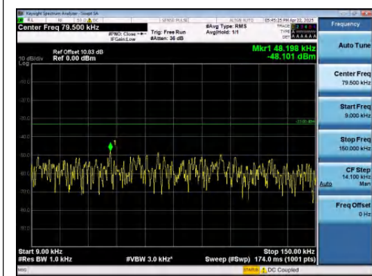
Band26(814-824)-1.4MHz-QPSK-26783-6RB#0- 0.009~0.15-PASS
