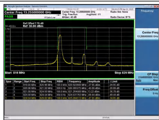
Band26(814-824)-3MHz-16QAM-26775-1RB#0-P
