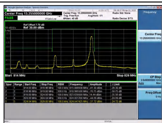
Band26(814-824)-5MHz-QPSK-26765-1RB#24-P
