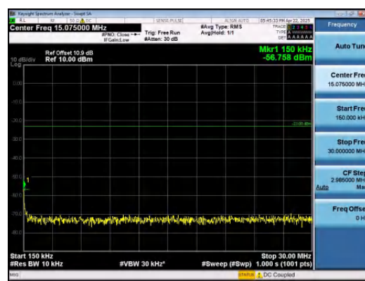
Band26(814-824)-1.4MHz-QPSK-26783-6RB#0- 0.15~30-PASS
