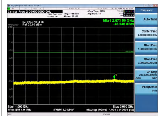
Band26(814-824)-1.4MHz-16QAM-26697-6RB#0 -1000~3000-PASS
