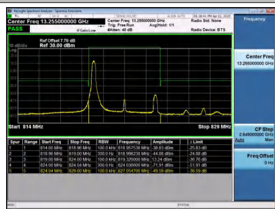
Band26(814-824)-5MHz-16QAM-26765-1RB#0-P
