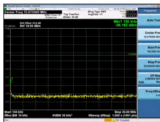
Band26(814-824)-1.4MHz-QPSK-26697-6RB#0- 0.15~30-PASS
