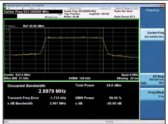
Band26(814-824)-3MHz-16QAM-26775-15RB#0-P ASS
