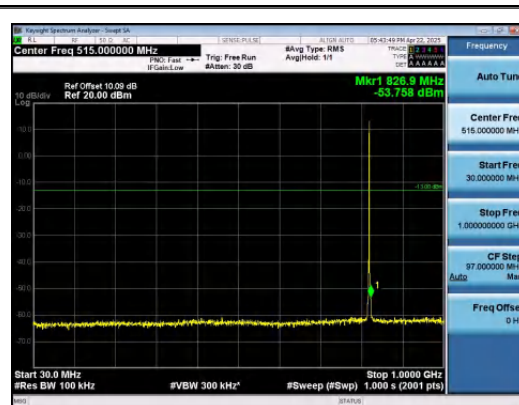
Band26(814-824)-1.4MHz-QPSK-26783-1RB#5- 30~1000-PASS
