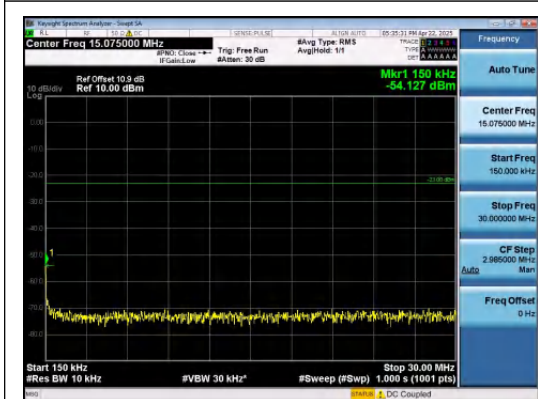
Band26(814-824)-1.4MHz-16QAM-26697-6RB#0 -0.15~30-PASS
