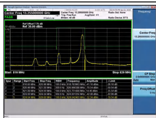
Band26(814-824)-3MHz-QPSK-26775-1RB#14-P
