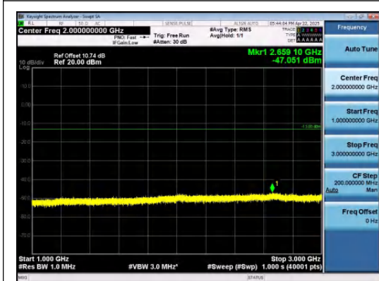
Band26(814-824)-1.4MHz-QPSK-26783-1RB#5- 1000~3000-PASS
