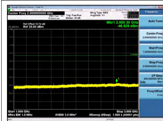
Band26(814-824)-1.4MHz-QPSK-26740-1RB#5- 1000~3000-PASS
