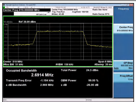
Band26(814-824)-3MHz-16QAM-26740-15RB#0-P ASS
