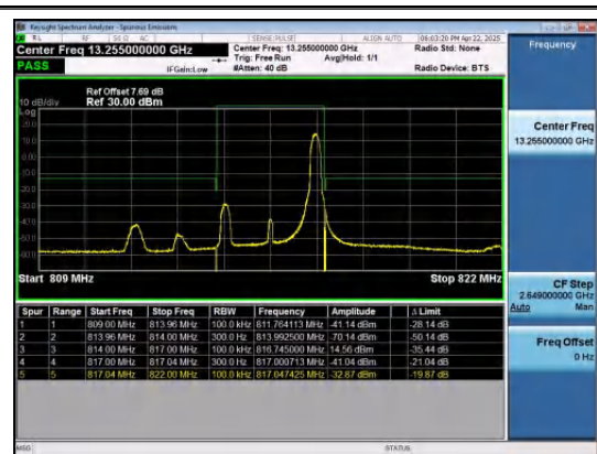
Band26(814-824)-3MHz-QPSK-26705-1RB#14-P
