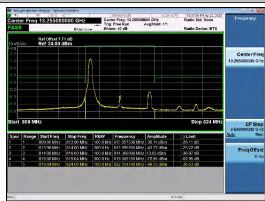
Band26(814-824)-5MHz-16QAM-26715-1RB#0-P
