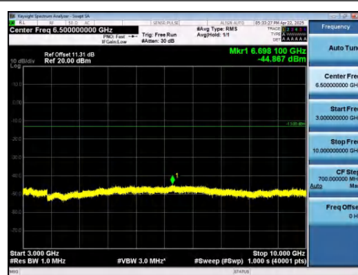
Band26(814-824)-1.4MHz-QPSK-26697-1RB#5- 3000~10000-PASS
