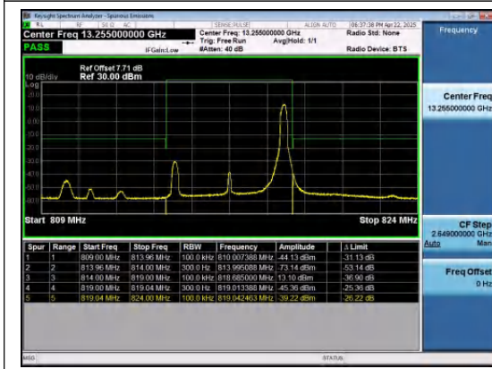
Band26(814-824)-5MHz-16QAM-26715-1RB#24-P
