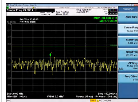
Band26(814-824)-1.4MHz-QPSK-26740-6RB#0- 0.009~0.15-PASS
