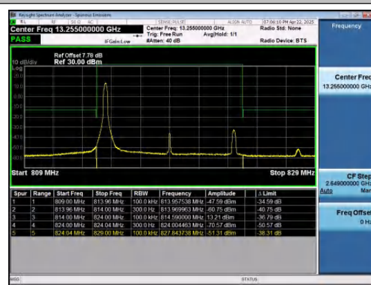
Band26(814-824)-10MHz-16QAM-26740-1RB#0-P
