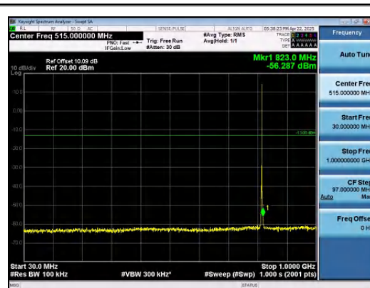
Band26(814-824)-1.4MHz-QPSK-26740-1RB#5- 30~1000-PASS
