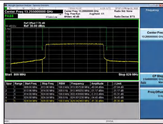
Band26(814-824)-10MHz-16QAM-26740-50RB#0-P
