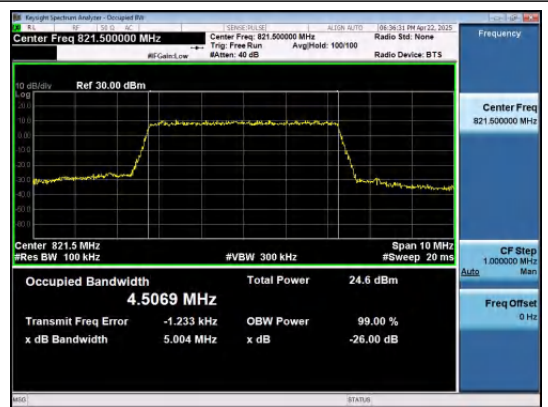
Band26(814-824)-5MHz-16QAM-26765-25RB#0-P ASS
