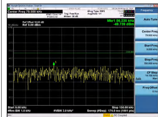
Band26(814-824)-1.4MHz-QPSK-26697-6RB#0- 0.009~0.15-PASS
