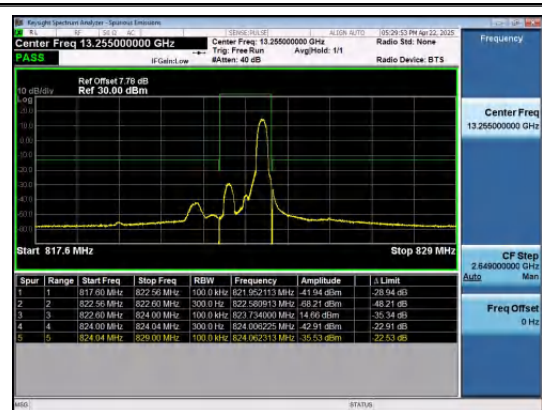
Band26(814-824)-1.4MHz-QPSK-26783-1RB#5-P ASS
