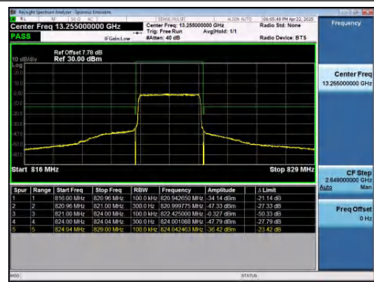
Band26(814-824)-3MHz-16QAM-26775-15RB#0-P
