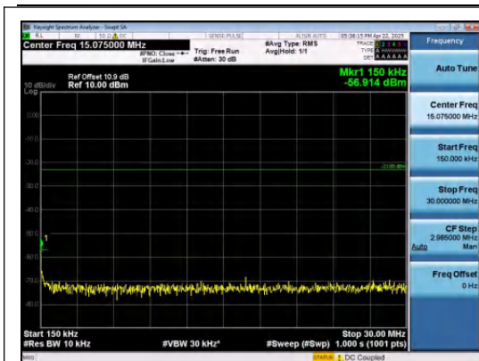
Band26(814-824)-1.4MHz-QPSK-26740-1RB#5- 0.15~30-PASS
