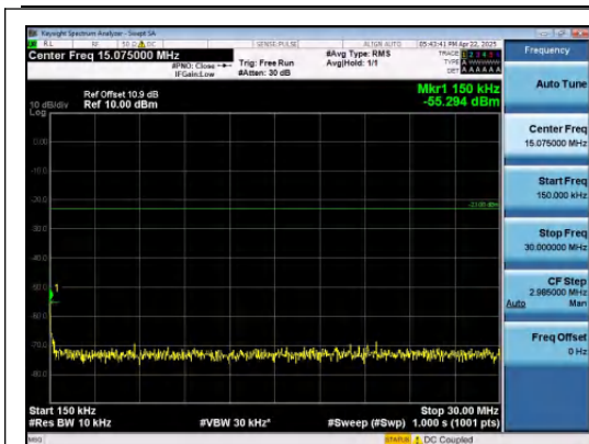
Band26(814-824)-1.4MHz-QPSK-26783-1RB#5- 0.15~30-PASS
