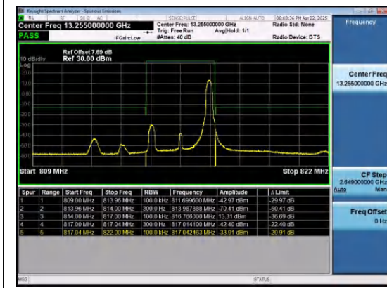
Band26(814-824)-3MHz-16QAM-26705-1RB#14-P
