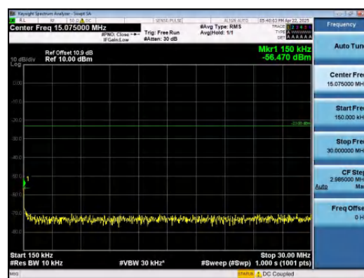
Band26(814-824)-1.4MHz-QPSK-26740-6RB#0- 0.15~30-PASS
