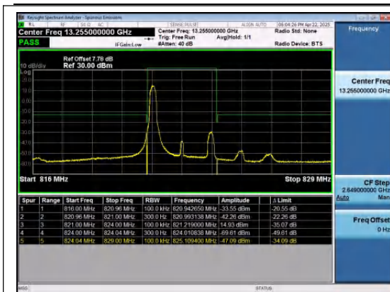
Band26(814-824)-3MHz-QPSK-26775-1RB#0-PA
