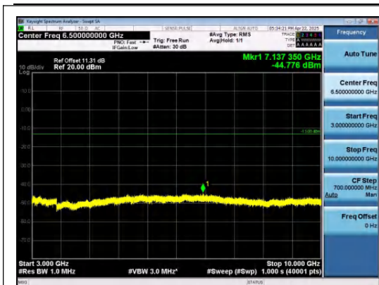
Band26(814-824)-1.4MHz-16QAM-26697-1RB#5 -3000~10000-PASS
