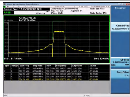
Band26(814-824)-1.4MHz-16QAM-26783-6RB#0- PASS
