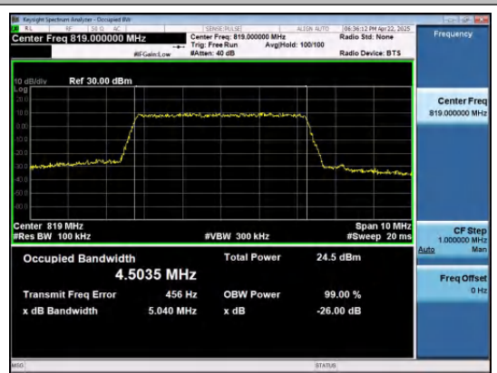
Band26(814-824)-5MHz-16QAM-26740-25RB#0-P ASS
