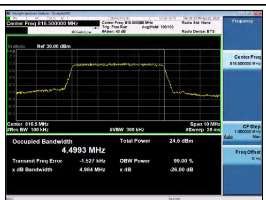
Band26(814-824)-5MHz-16QAM-26715-25RB#0-P ASS
