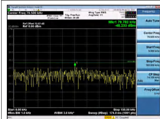
Band25-20MHz-16QAM-26140-1RB#99-0.009~0 .15-PASS
