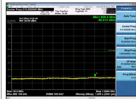
Band25-15MHz-16QAM-26365-1RB#74-30~100 0-PASS
