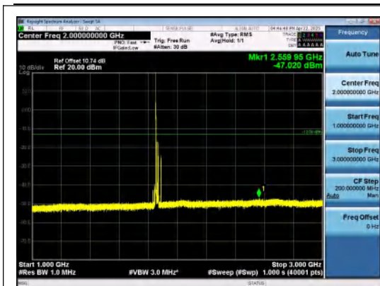
Band25-20MHz-16QAM-26140-1RB#0-1000~30 00-PASS
