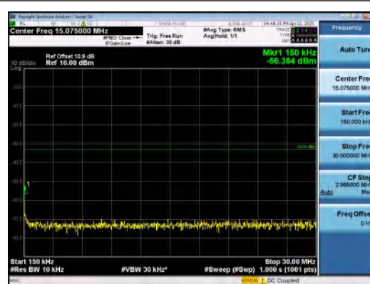
Band25-20MHz-16QAM-26140-1RB#99-0.15~30 -PASS
