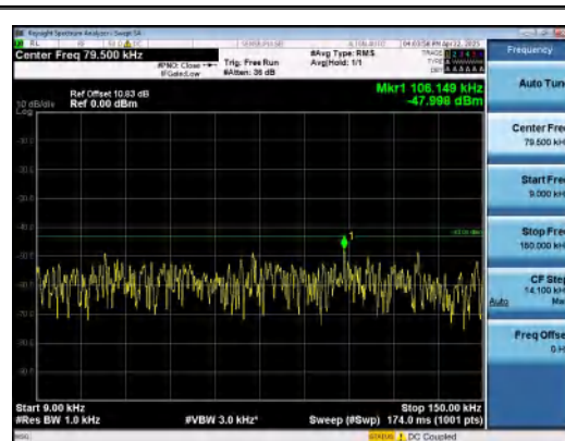
Band25-15MHz-16QAM-26115-75RB#0-0.009~0.15-PASS
