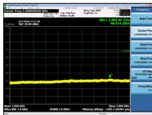
Band25-15MHz-16QAM-26365-1RB#74-1000~3 000-PASS
