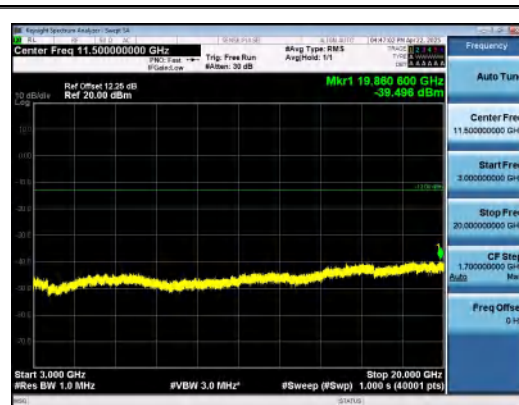
Band25-20MHz-16QAM-26140-1RB#0-3000~20 000-PASS
