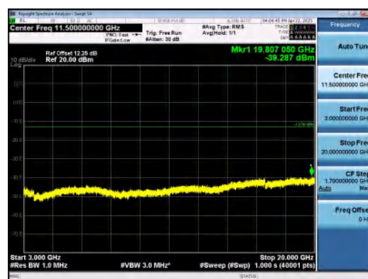
Band25-15MHz-16QAM-26115-75RB#0-3000~20000-PASS
