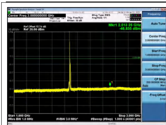
Band25-15MHz-16QAM-26365-1RB#0-1000~30 00-PASS
