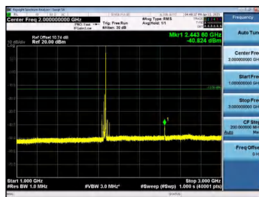
Band25-20MHz-16QAM-26140-1RB#99-1000~3 000-PASS
