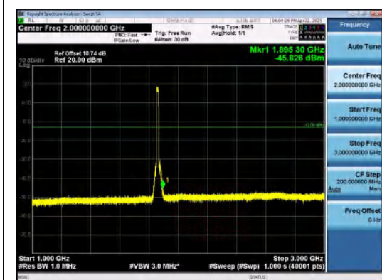
Band25-15MHz-16QAM-26115-75RB#0-1000~3000-PASS
