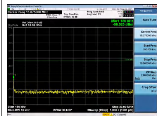
Band25-15MHz-16QAM-26115-75RB#0-0.15~30-PASS
