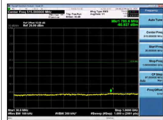
Band25-20MHz-16QAM-26140-1RB#99-30~100 0-PASS
