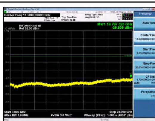
Band25-15MHz-16QAM-26365-1RB#0-3000~20 000-PASS
