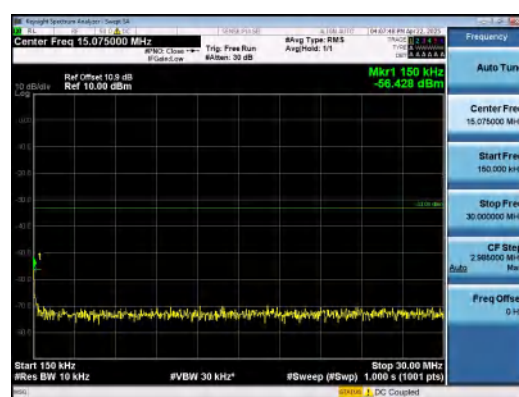
Band25-15MHz-16QAM-26365-1RB#74-0.15~30 -PASS
