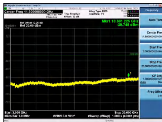
Band4-10MHz-16QAM-20175-50RB#0-3000~20000-PASS
