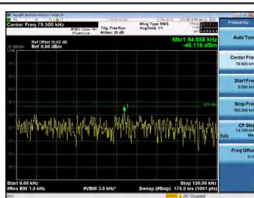
Band4-15MHz-16QAM-20025-75RB#0-0.009~0.15-PASS
