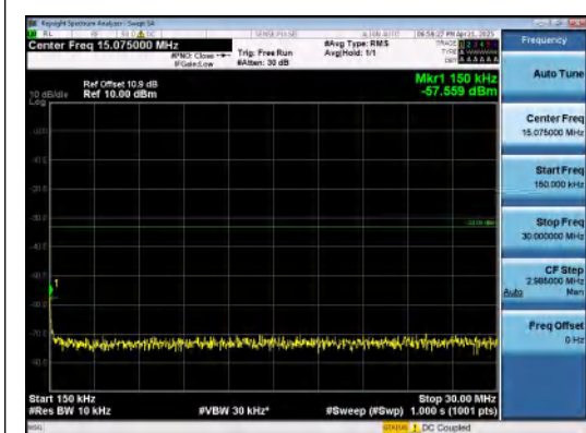
Band4-10MHz-16QAM-20175-50RB#0-0.15~30-PASS
