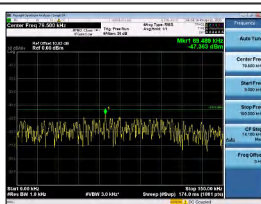
Band4-10MHz-16QAM-20175-50RB#0-0.009~0.15-PASS
