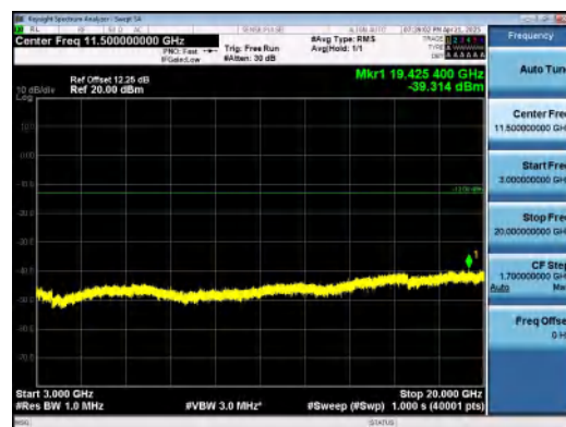
Band4-15MHz-16QAM-20025-75RB#0-3000~20000-PASS
