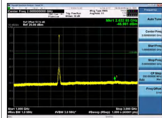
Band4-10MHz-16QAM-20175-50RB#0-1000~3000-PASS
