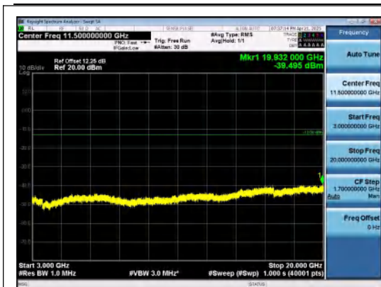
Band4-15MHz-16QAM-20025-1RB#74-3000~20000-PASS
