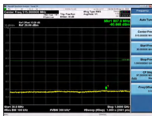
Band4-10MHz-16QAM-20175-50RB#0-30~1000-PASS
