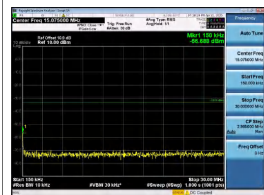
Band4-15MHz-16QAM-20025-75RB#0-0.15~30-PASS
