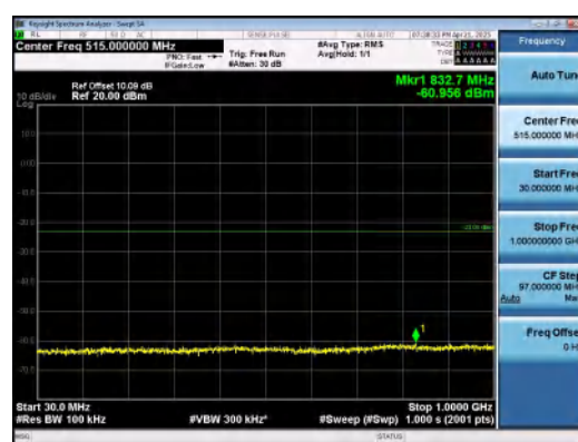
Band4-15MHz-16QAM-20025-75RB#0-30~1000-PASS
