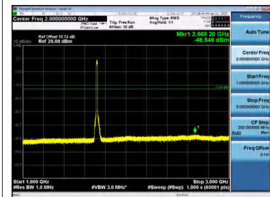
Band4-15MHz-16QAM-20025-75RB#0-1000~3000-PASS
