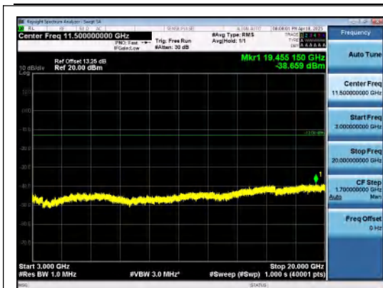
Band2-5MHz-16QAM-18625-1RB#24-3000~200 00-PASS
