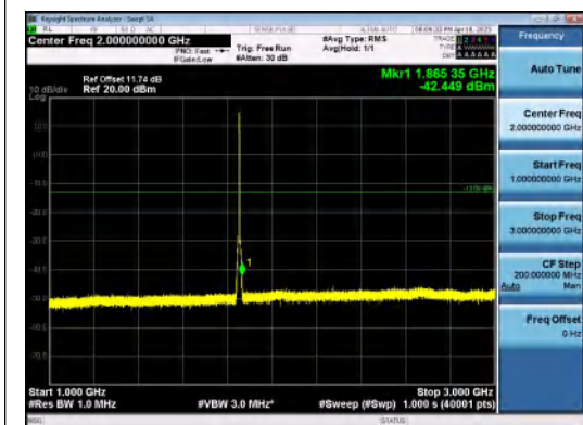
Band2-5MHz-16QAM-18625-25RB#0-1000~300 0-PASS
