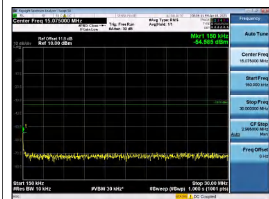
Band2-5MHz-16QAM-18625-25RB#0-0.15~30-P ASS
