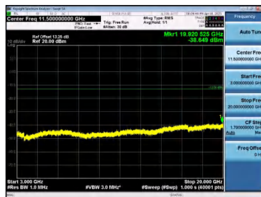
Band2-5MHz-16QAM-18625-25RB#0-3000~200 00-PASS
