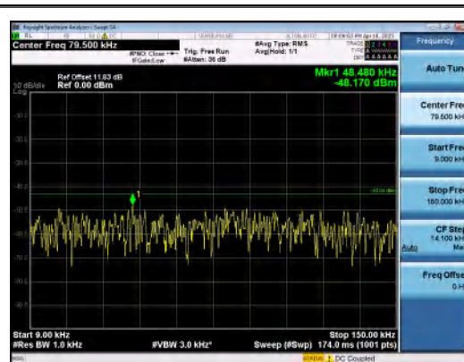
Band2-5MHz-16QAM-18625-25RB#0-0.009~0.1 5-PASS
