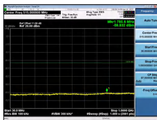
Band2-5MHz-16QAM-18625-25RB#0-30~1000-P ASS
