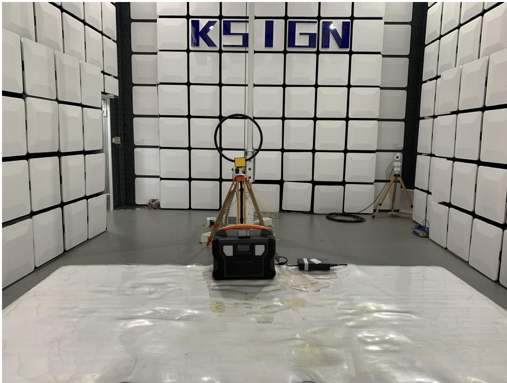
Radiated Measurement (Below 30MHz)
