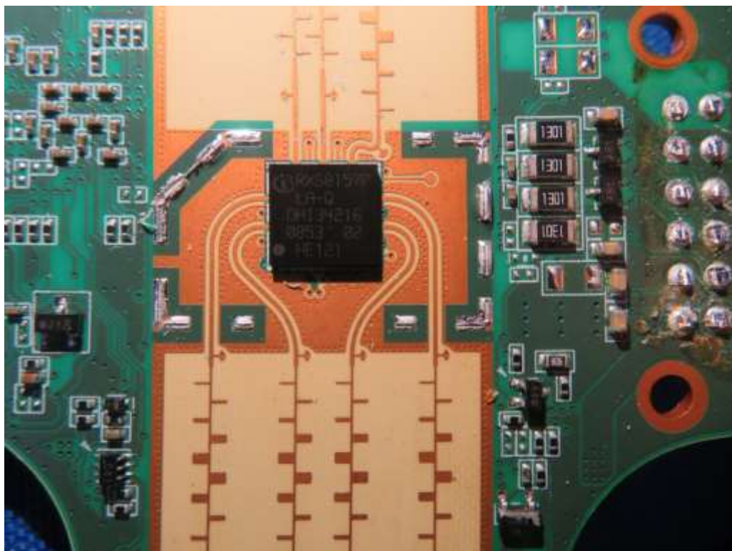
PCB bottom side without shielding
