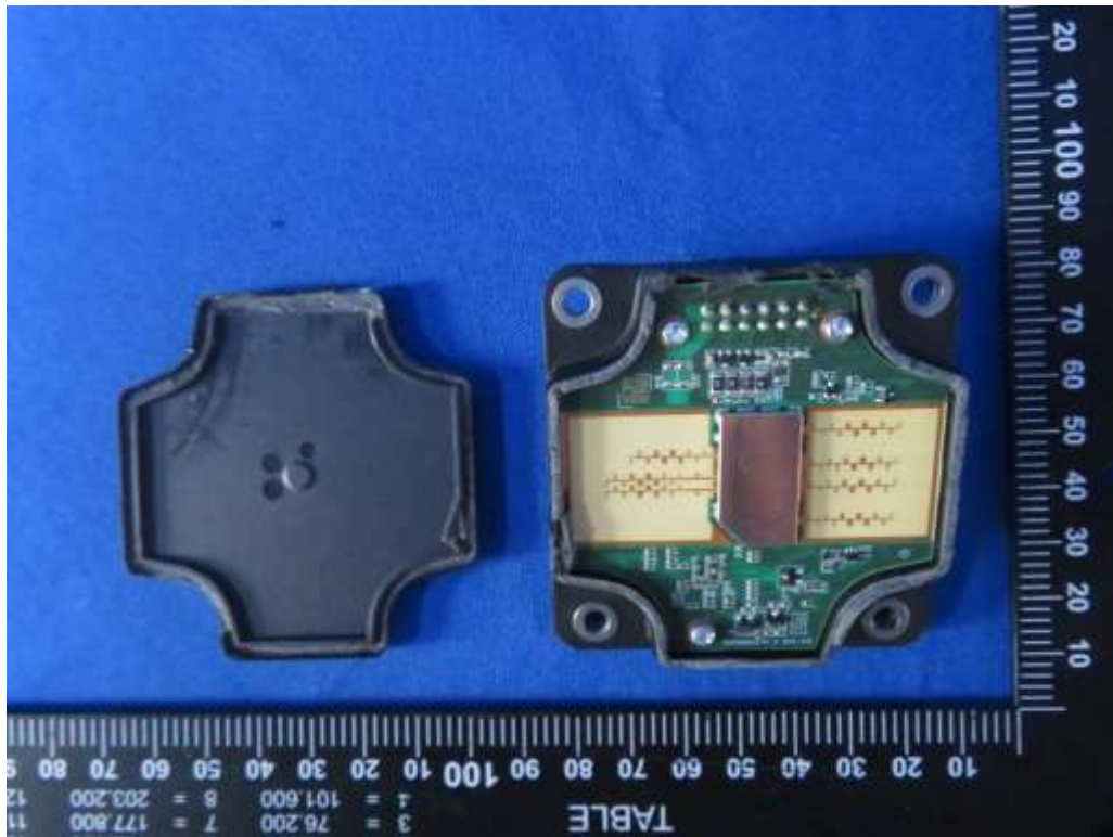
Disassembly view
