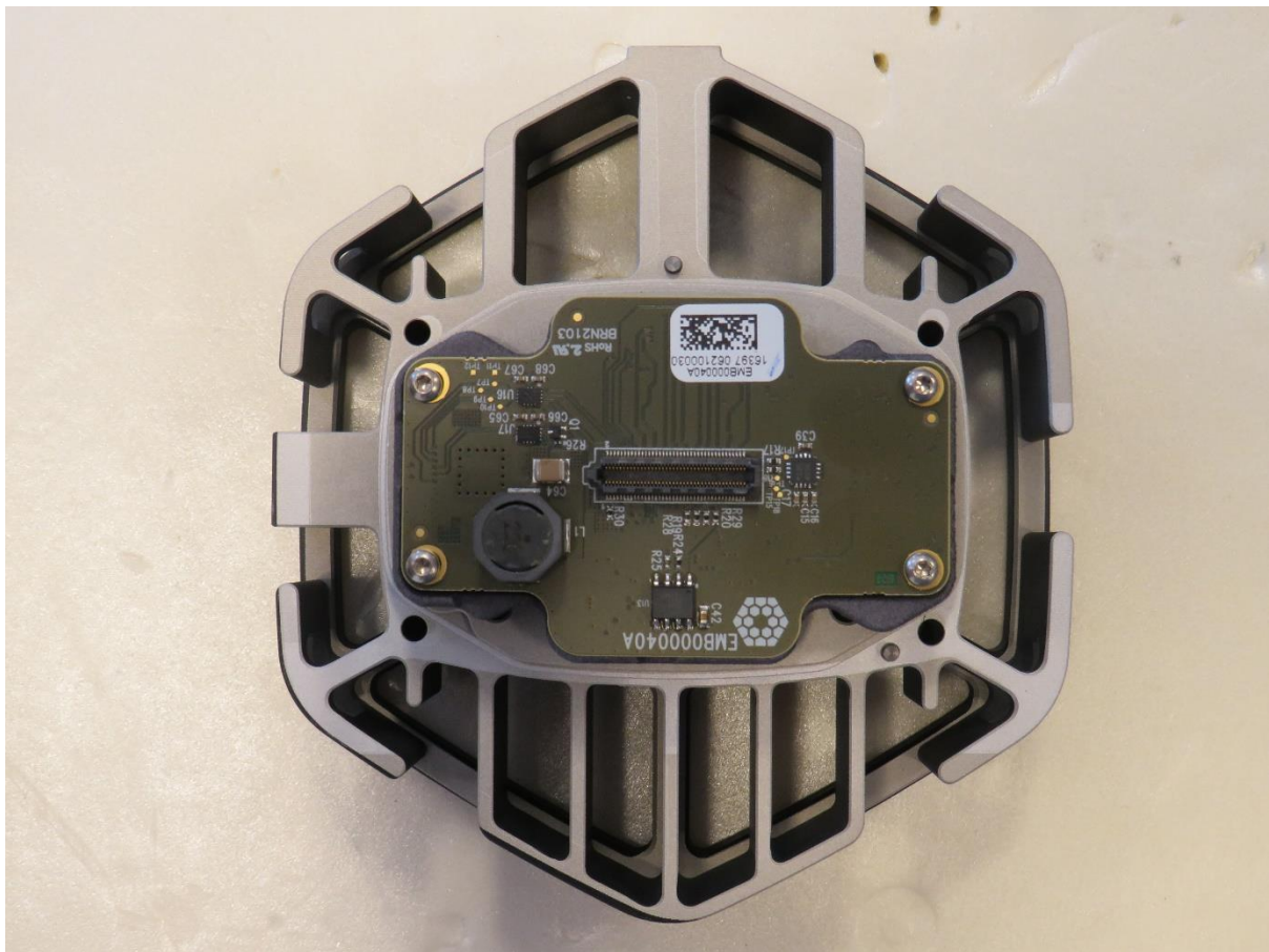
Sensor PCB:
