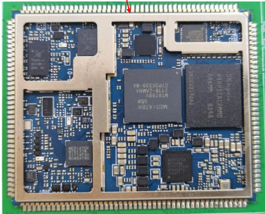
Internal 4 (WIFI chip)
