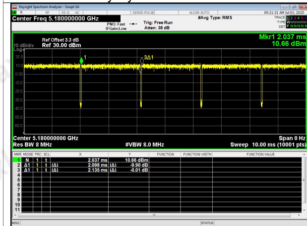
Duty Cycle NVNT n20 5180MHz
