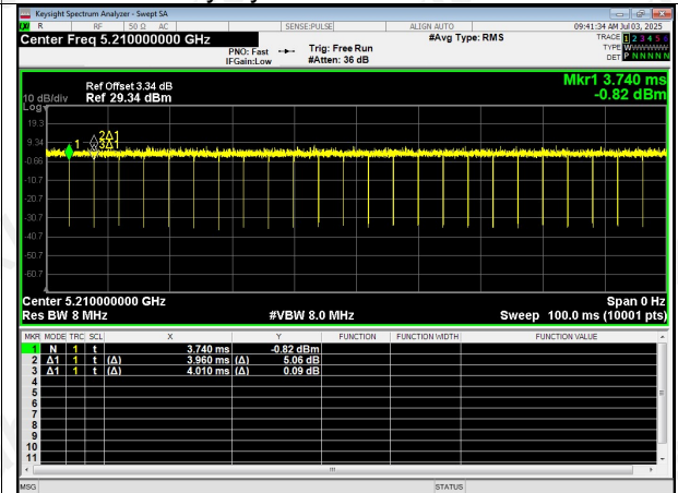
Duty Cycle NVNT ac80 5210MHz
