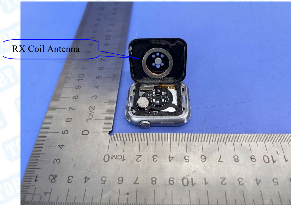
Photo 6 Internal of EUT
