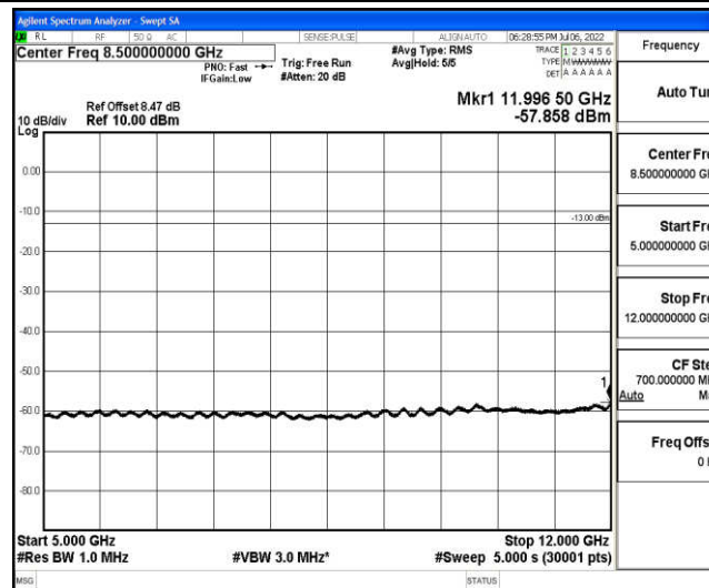
Band66-15MHz-16QAM-132322-1-0-Low-5000-12000--57.86-PASS
