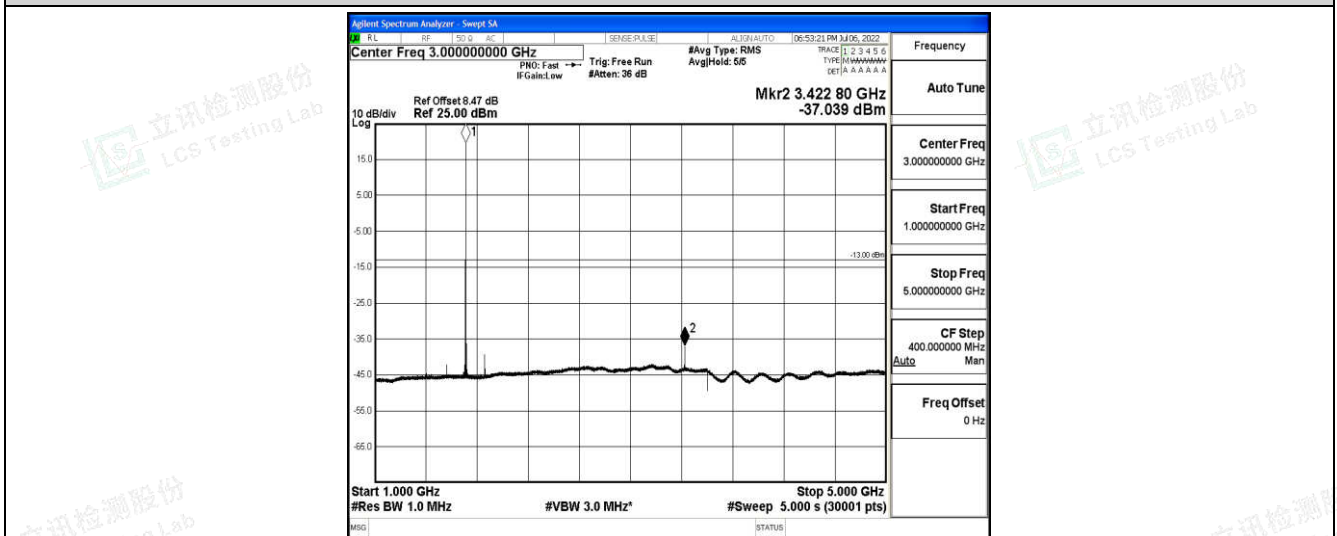
Band66-20MHz-16QAM-132072-1-0-Low-1000-5000--37.04-PASS
