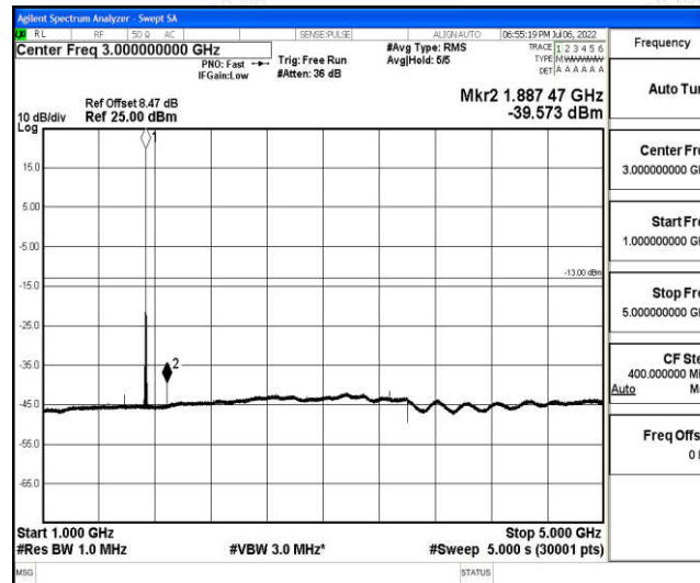
Band66-20MHz-QPSK-132322-1-0-Low-1000-5000--39.57-PASS
