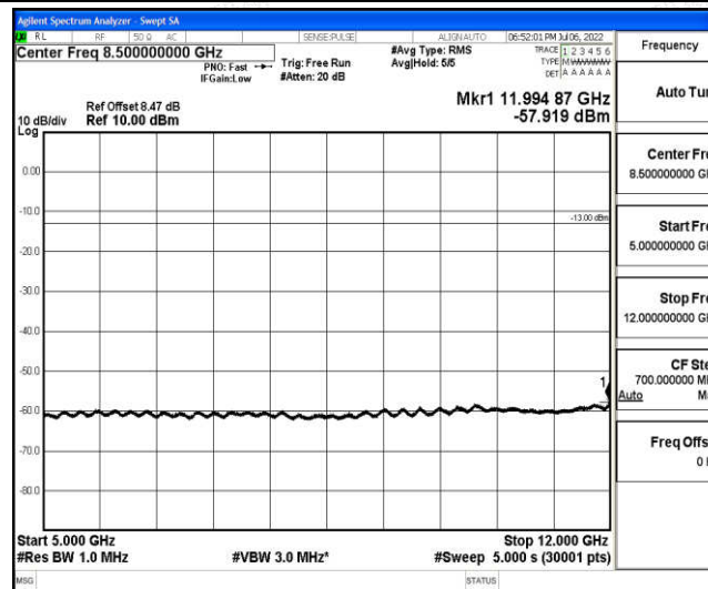
Band66-20MHz-QPSK-132072-1-0-Low-5000-12000--57.92-PASS
