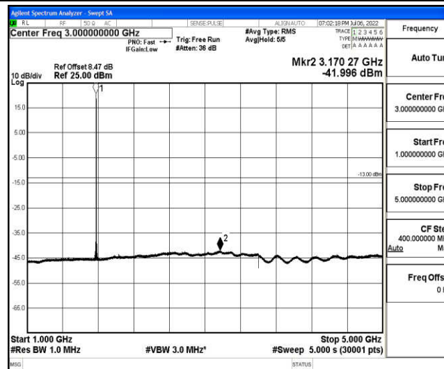
Band66-20MHz-QPSK-132572-1-0-High-1000-5000--42-PASS
