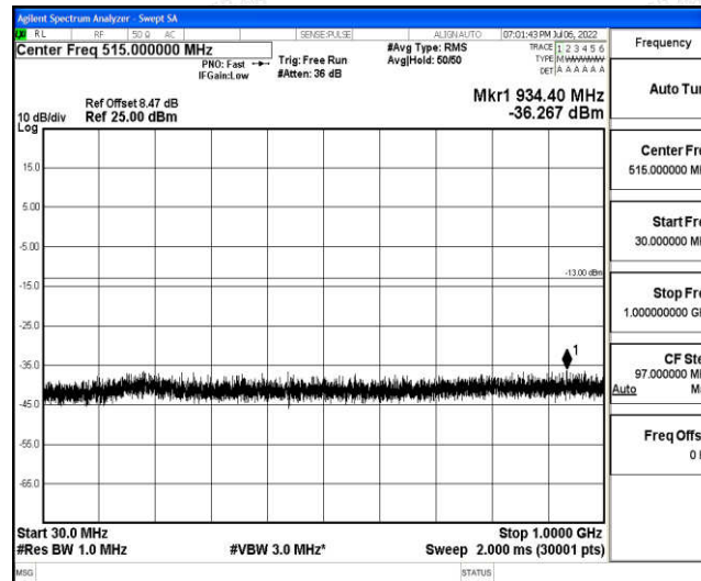
Band66-20MHz-QPSK-132572-1-0-High-30-1000--36.27-PASS
