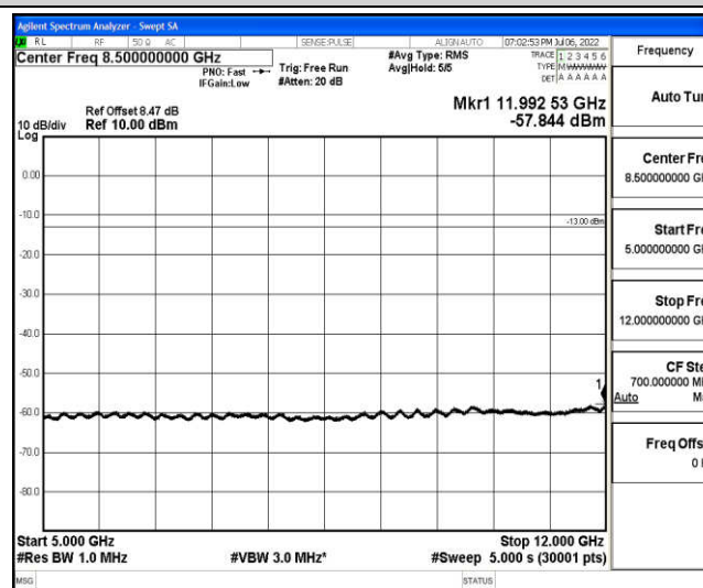
Band66-20MHz-QPSK-132572-1-0-High-5000-12000--57.84-PASS
