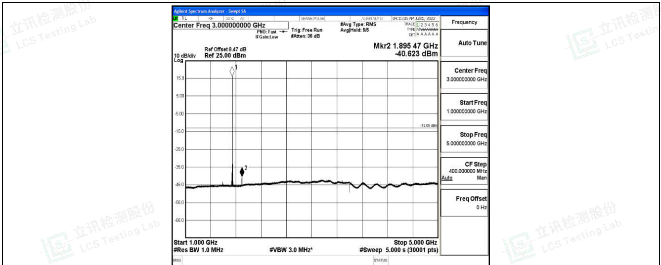
Band66-3MHz-16QAM-132322-1-0-Low-1000-5000--40.62-PASS
