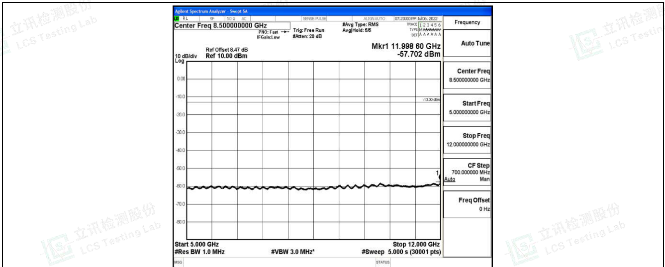
Band66-10MHz-16QAM-132022-1-0-Low-5000-12000--57.7-PASS
