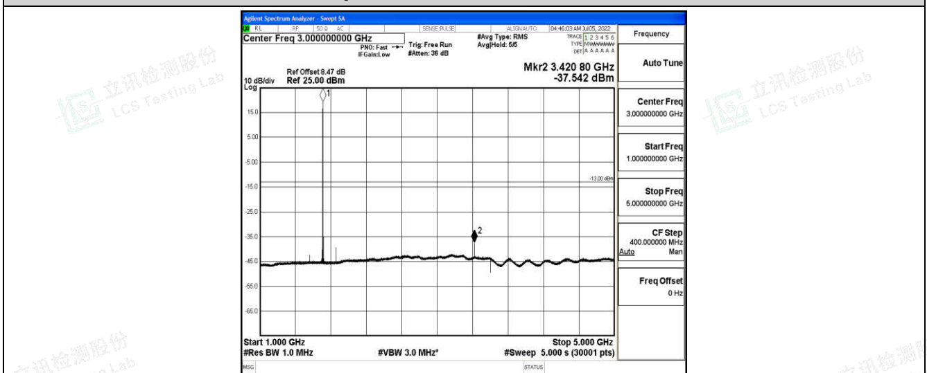
Band66-5MHz-QPSK-131997-1-0-Low-1000-5000--37.54-PASS
