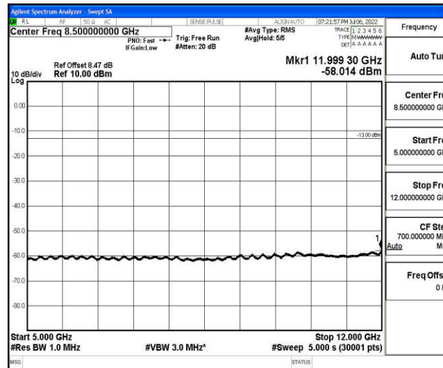
Band66-10MHz-QPSK-132322-1-0-Low-5000-12000--58.01-PASS
