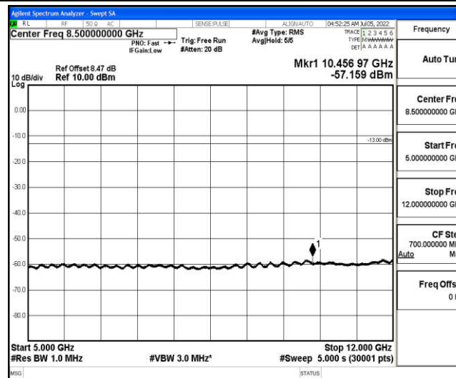
Band66-5MHz-16QAM-132322-1-0-Low-5000-12000--57.16-PASS
