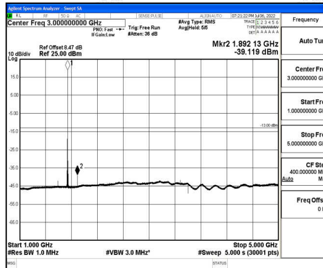
Band66-10MHz-QPSK-132322-1-0-Low-1000-5000--39.12-PASS
