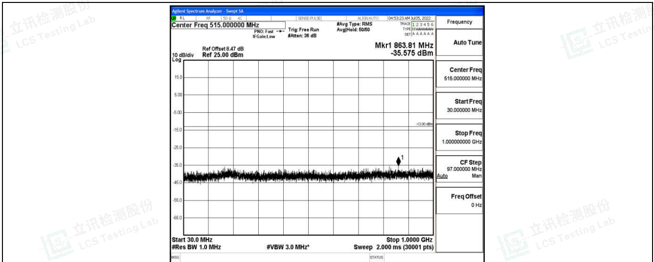
Band66-5MHz-QPSK-132647-1-0-High-30-1000--35.58-PASS
