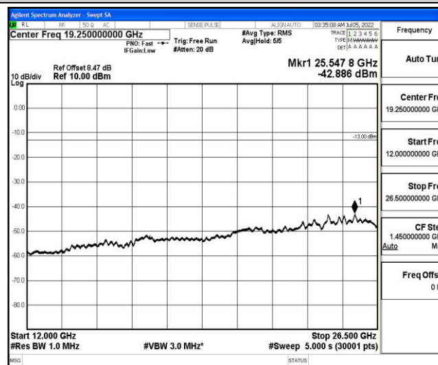
Band66-1.4MHz-QPSK-132322-1-0-Low-12000-26500--42.89-PASS
