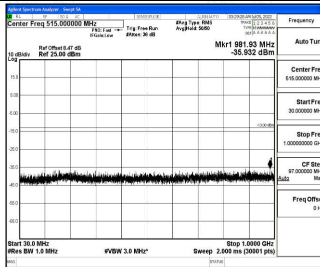
Band66-1.4MHz-QPSK-131979-1-0-Low-30-1000--35.93-PASS
