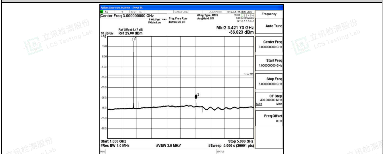
Band66-10MHz-16QAM-132022-1-0-Low-1000-5000--36.82-PASS
