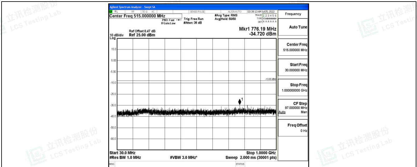
Band66-1.4MHz-16QAM-132665-1-0-High-30-1000--34.72-PASS
