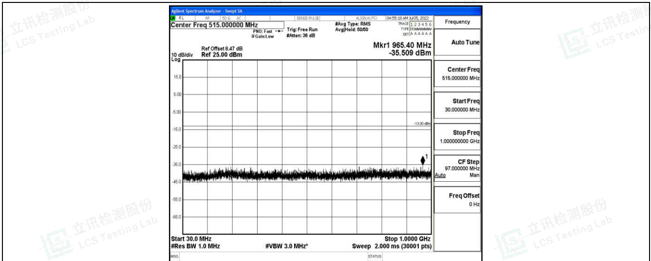
Band66-5MHz-16QAM-132647-1-0-High-30-1000--35.51-PASS
