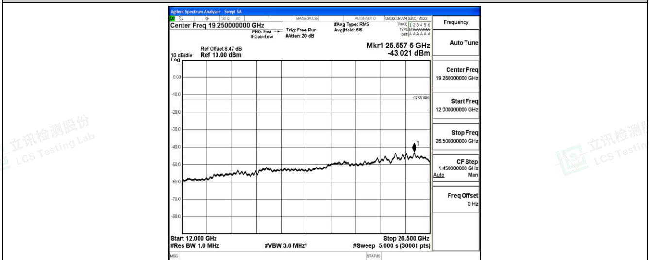
Band66-1.4MHz-16QAM-131979-1-0-Low-12000-26500--43.02-PASS
