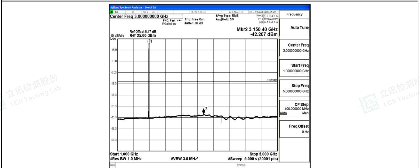
Band66-3MHz-16QAM-132657-1-0-High-1000-5000--42.21-PASS
