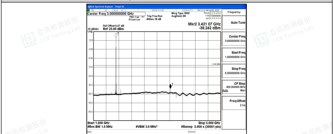
Band66-3MHz-16QAM-131987-1-0-Low-1000-5000--39.24-PASS
