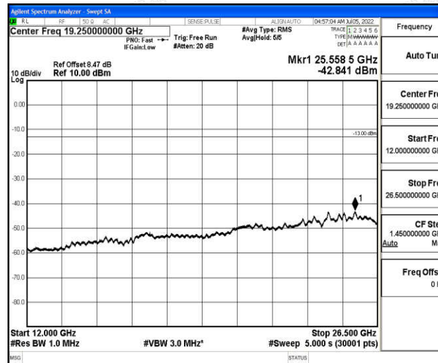
Band66-5MHz-16QAM-132647-1-0-High-12000-26500--42.84-PASS
