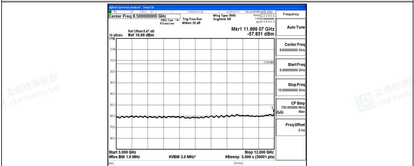
Band66-3MHz-QPSK-132322-1-0-Low-5000-12000--57.83-PASS
