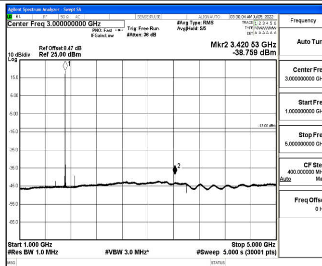
Band66-1.4MHz-QPSK-131979-1-0-Low-1000-5000--38.76-PASS
