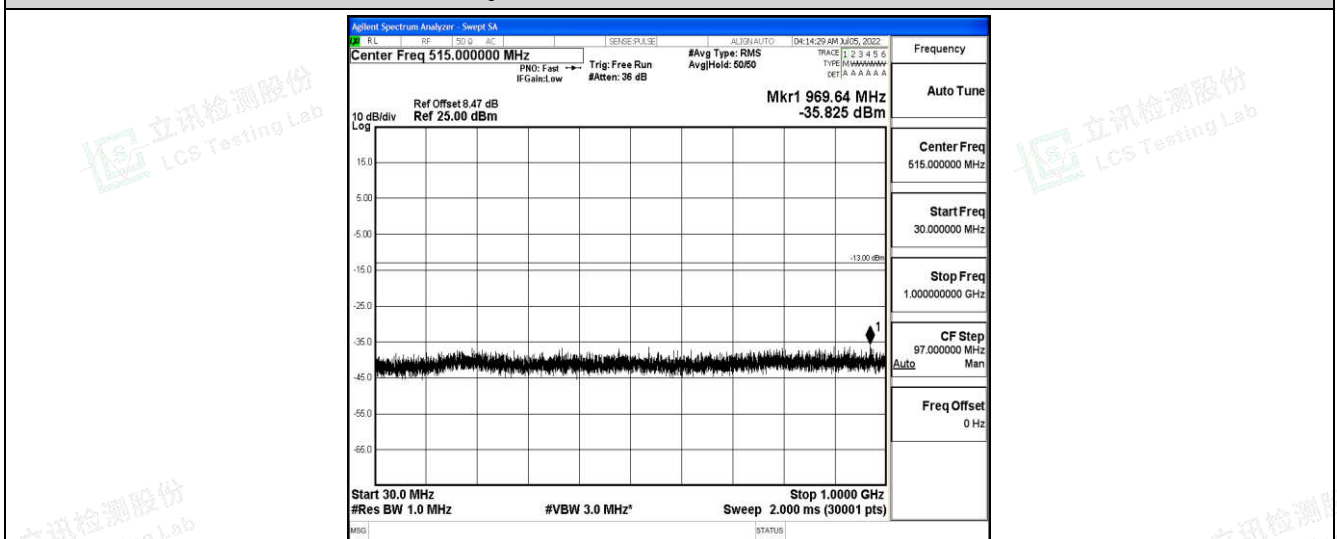
Band66-3MHz-16QAM-132322-1-0-Low-30-1000--35.83-PASS
