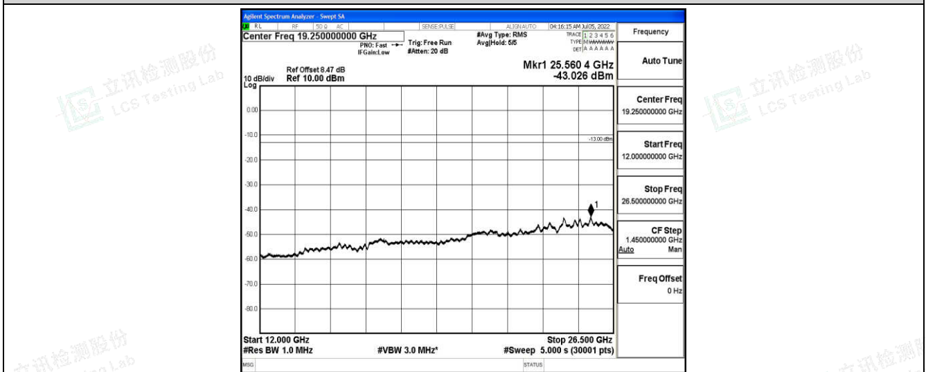
Band66-3MHz-16QAM-132322-1-0-Low-12000-26500--43.03-PASS
