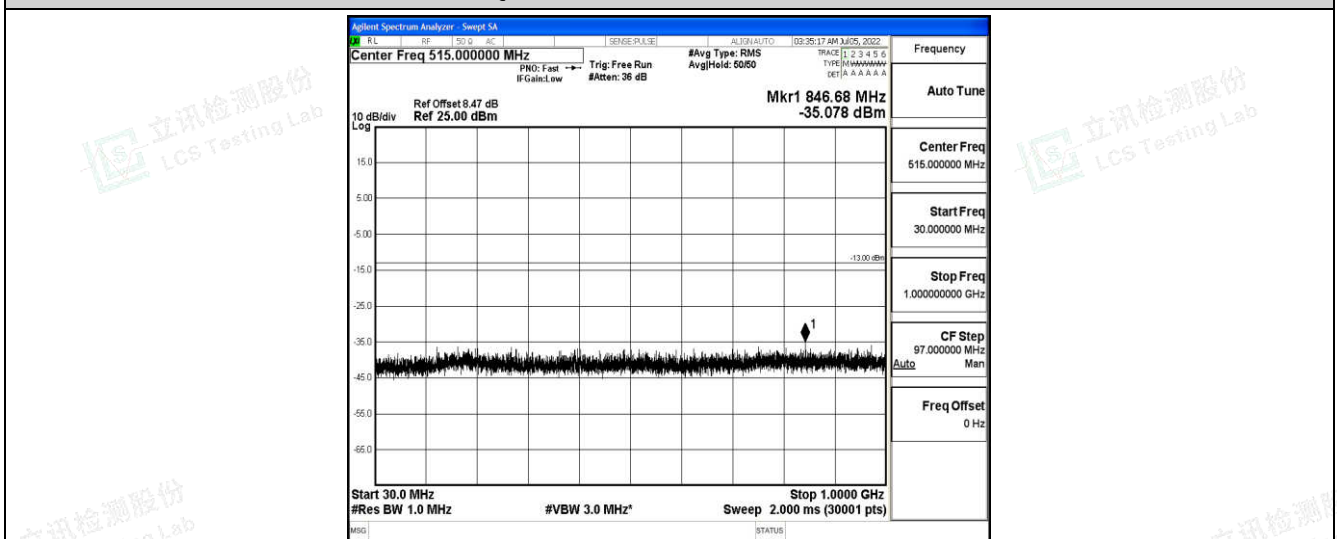
Band66-1.4MHz-16QAM-132322-1-0-Low-30-1000--35.08-PASS
