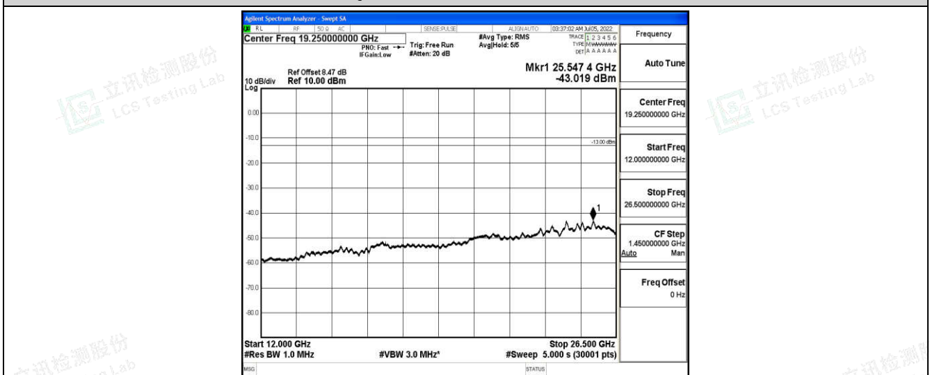
Band66-1.4MHz-16QAM-132322-1-0-Low-12000-26500--43.02-PASS
