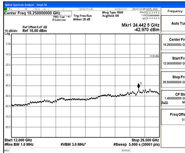
Band66-5MHz-QPSK-131997-1-0-Low-12000-26500--42.97-PASS
