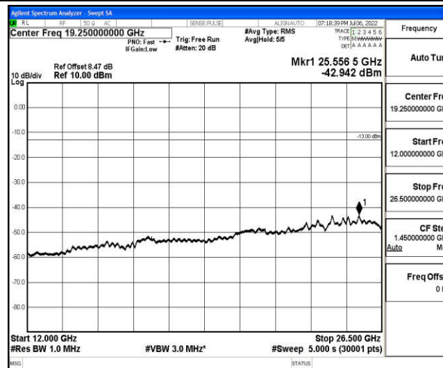
Band66-10MHz-QPSK-132022-1-0-Low-12000-26500--42.94-PASS
