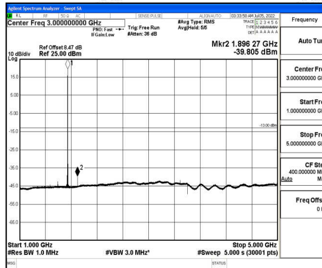
Band66-1.4MHz-QPSK-132322-1-0-Low-1000-5000--39.81-PASS
