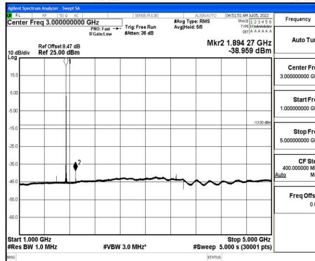
Band66-5MHz-16QAM-132322-1-0-Low-1000-5000--38.96-PASS
