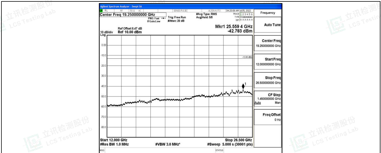
Band66-3MHz-16QAM-132657-1-0-High-12000-26500--42.78-PASS
