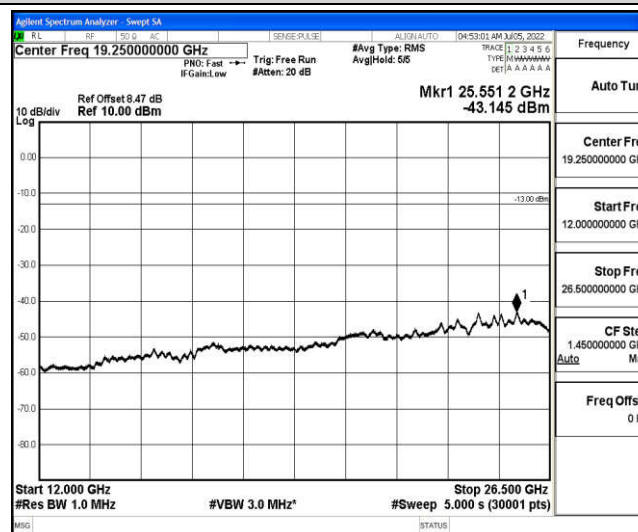
Band66-5MHz-16QAM-132322-1-0-Low-12000-26500--43.15-PASS
