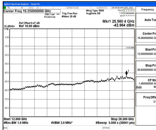
Band66-5MHz-16QAM-131997-1-0-Low-12000-26500--42.96-PASS
