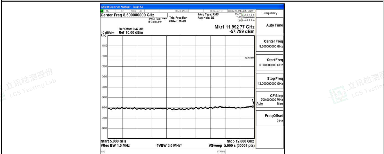
Band66-1.4MHz-16QAM-132322-1-0-Low-5000-12000--57.8-PASS
