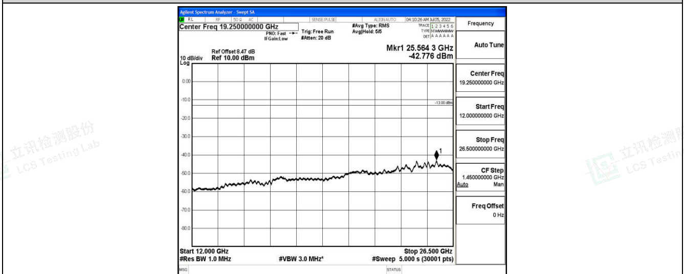
Band66-3MHz-QPSK-131987-1-0-Low-12000-26500--42.78-PASS
