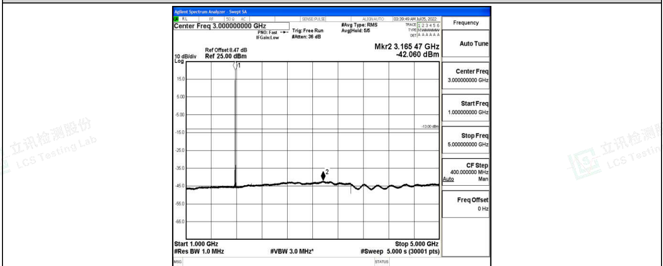
Band66-1.4MHz-16QAM-132665-1-0-High-1000-5000--42.06-PASS
