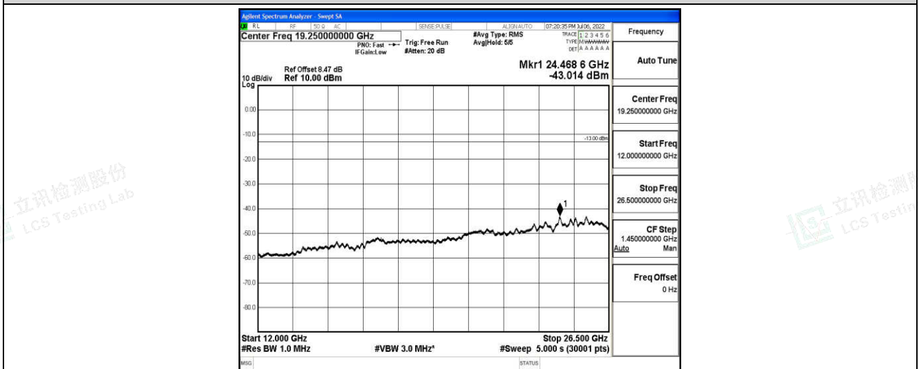
Band66-10MHz-16QAM-132022-1-0-Low-12000-26500--43.01-PASS
