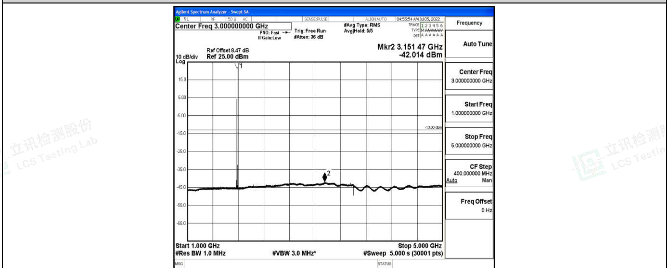
Band66-5MHz-16QAM-132647-1-0-High-1000-5000--42.01-PASS
