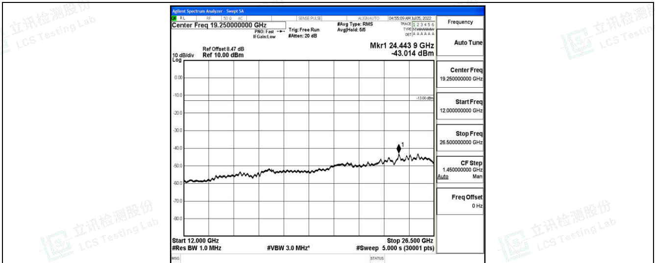
Band66-5MHz-QPSK-132647-1-0-High-12000-26500--43.01-PASS
