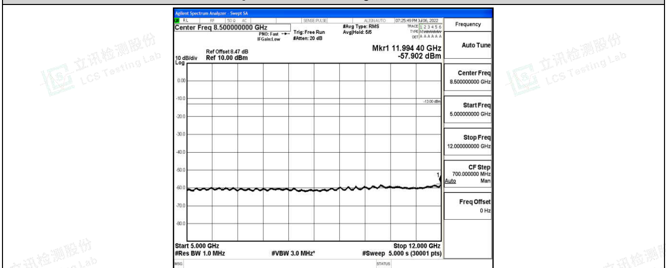
Band66-10MHz-QPSK-132622-1-0-High-5000-12000--57.9-PASS
