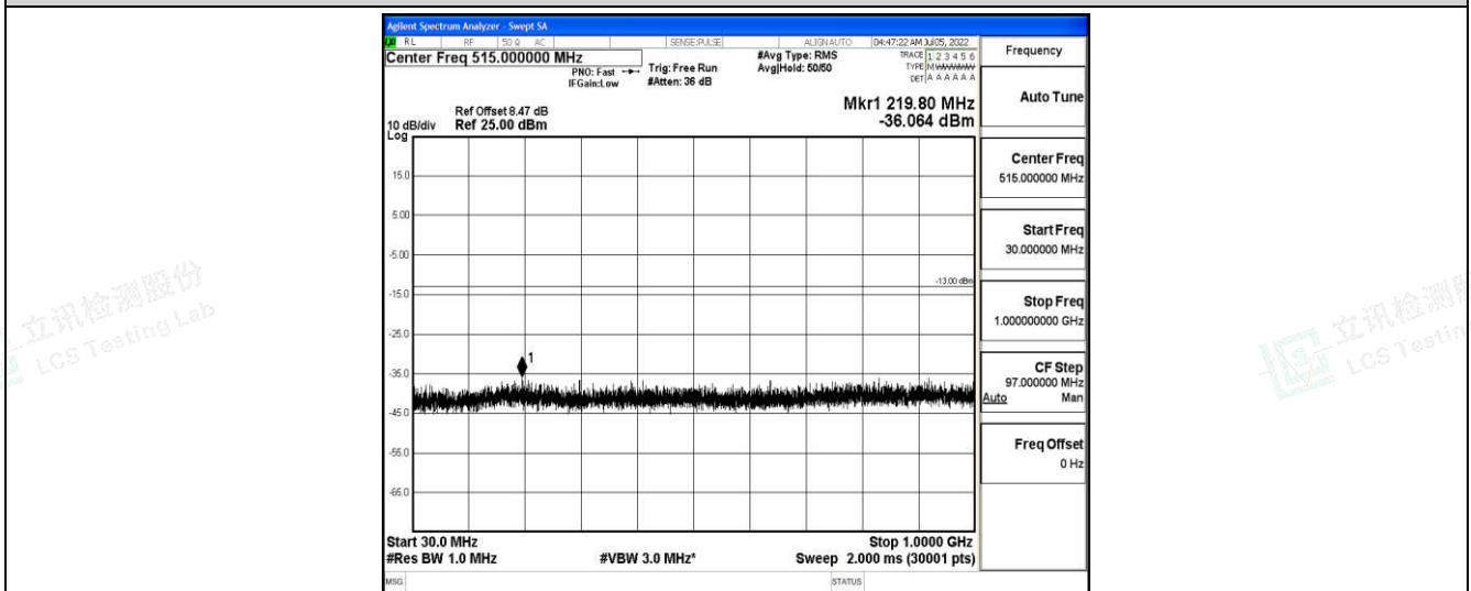
Band66-5MHz-16QAM-131997-1-0-Low-30-1000--36.06-PASS
