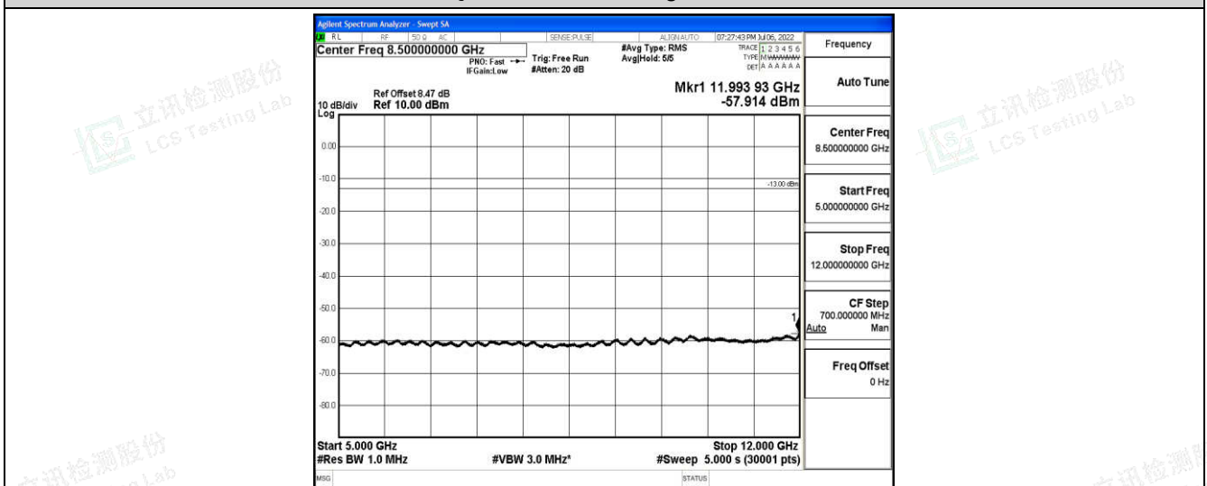
Band66-10MHz-16QAM-132622-1-0-High-5000-12000--57.91-PASS
