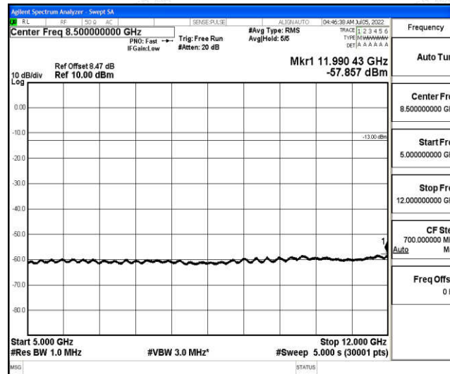
Band66-5MHz-QPSK-131997-1-0-Low-5000-12000--57.86-PASS
