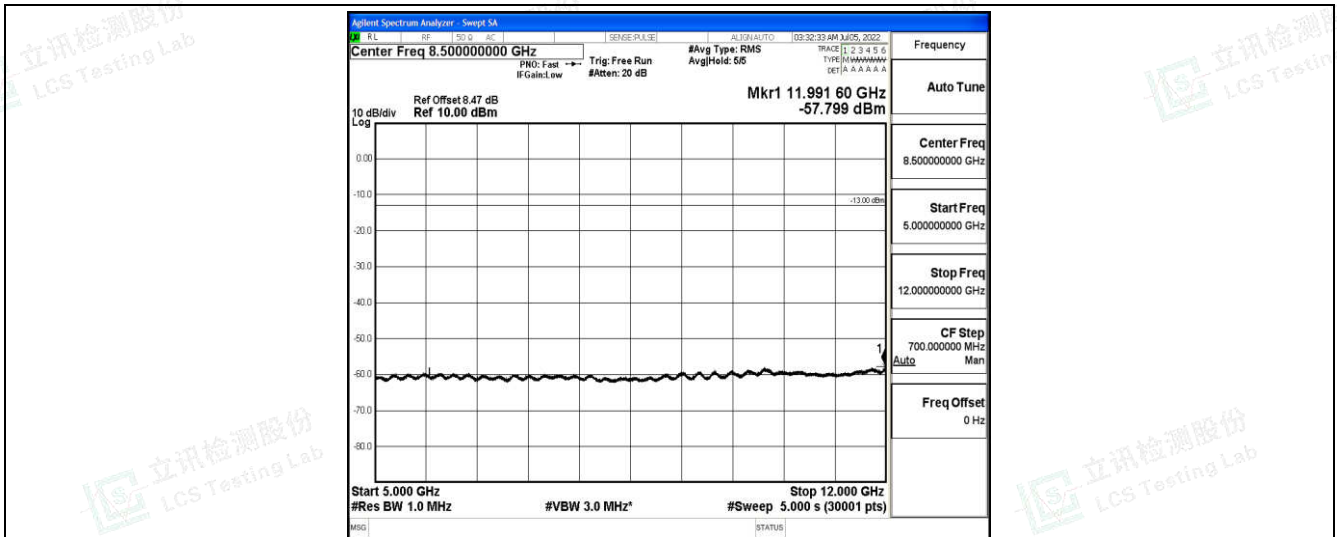
Band66-1.4MHz-16QAM-131979-1-0-Low-5000-12000--57.8-PASS
