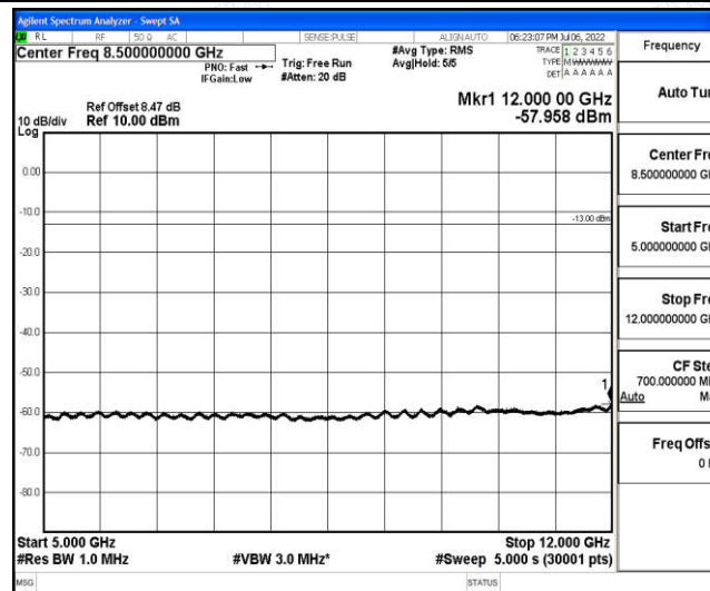
Band66-15MHz-QPSK-132047-1-0-Low-5000-12000--57.96-PASS
