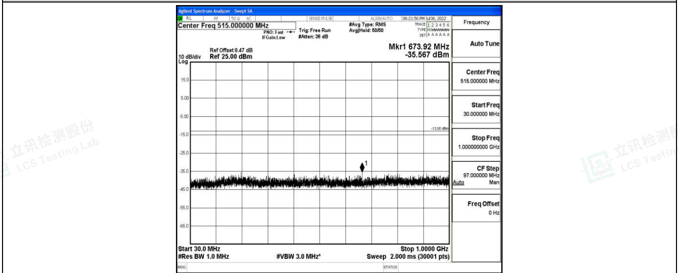
Band66-15MHz-QPSK-132047-1-0-Low-30-1000--35.57-PASS
