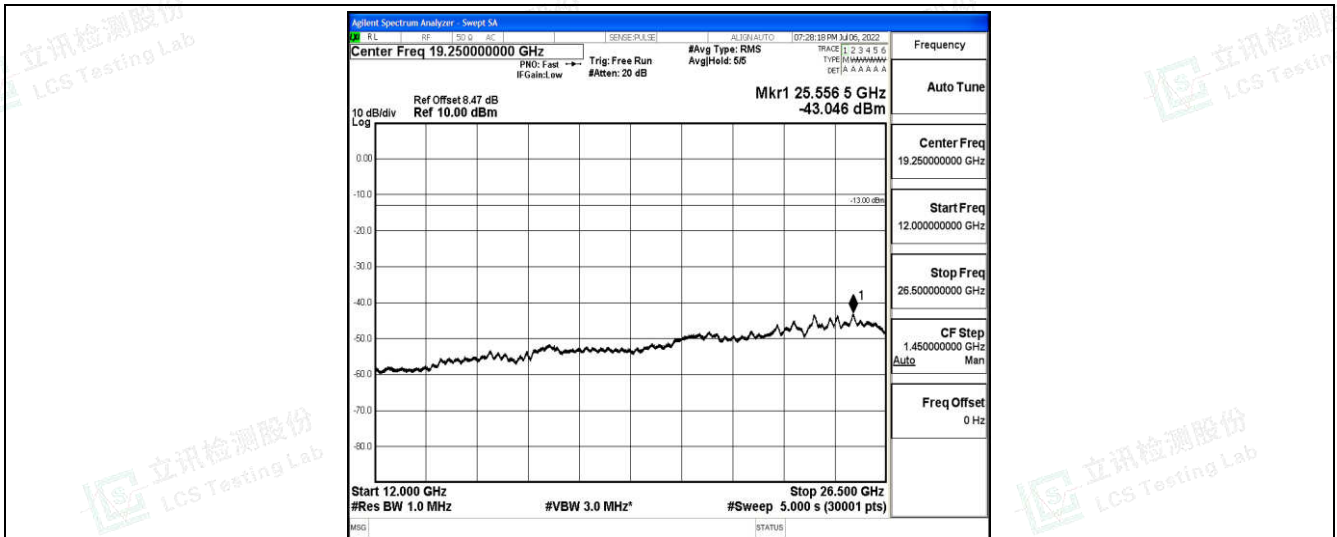
Band66-10MHz-16QAM-132622-1-0-High-12000-26500--43.05-PASS
