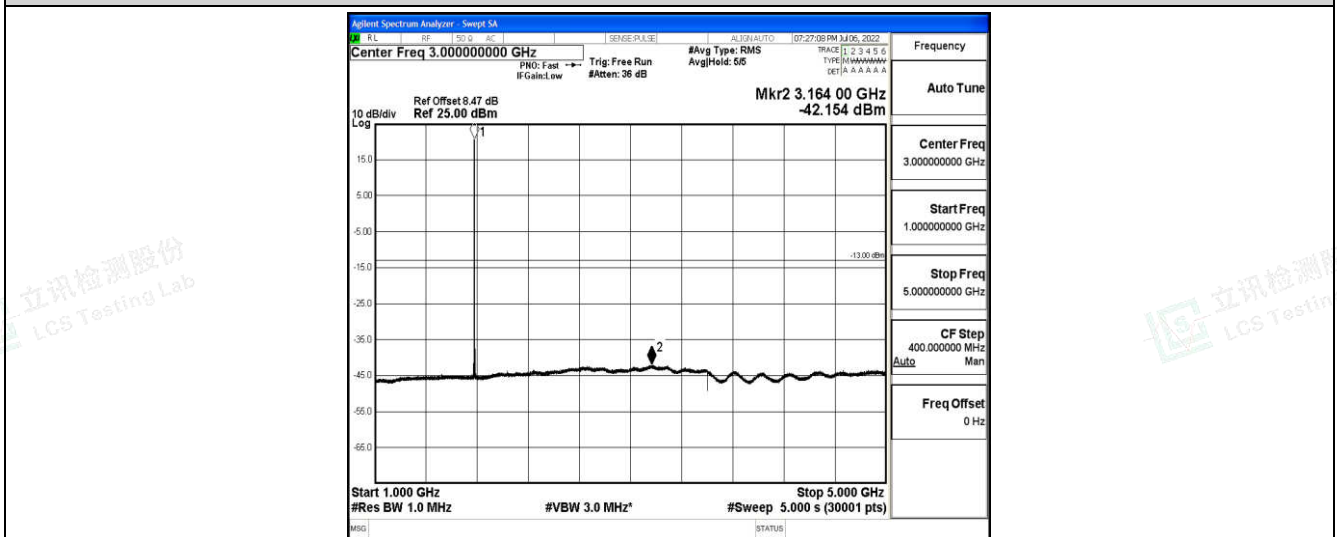
Band66-10MHz-16QAM-132622-1-0-High-1000-5000--42.15-PASS
