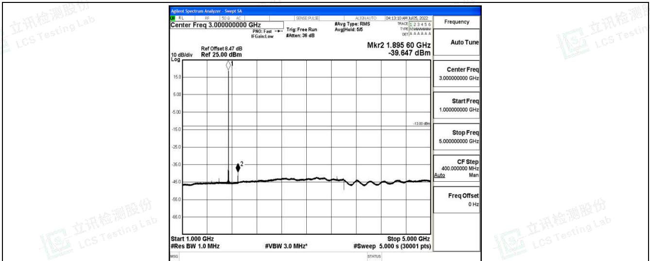
Band66-3MHz-QPSK-132322-1-0-Low-1000-5000--39.65-PASS
