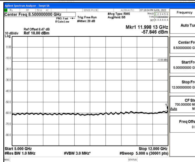
Band66-10MHz-QPSK-132022-1-0-Low-5000-12000--57.85-PASS
