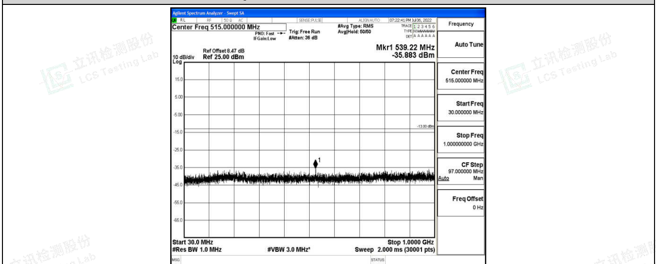
Band66-10MHz-16QAM-132322-1-0-Low-30-1000--35.88-PASS
