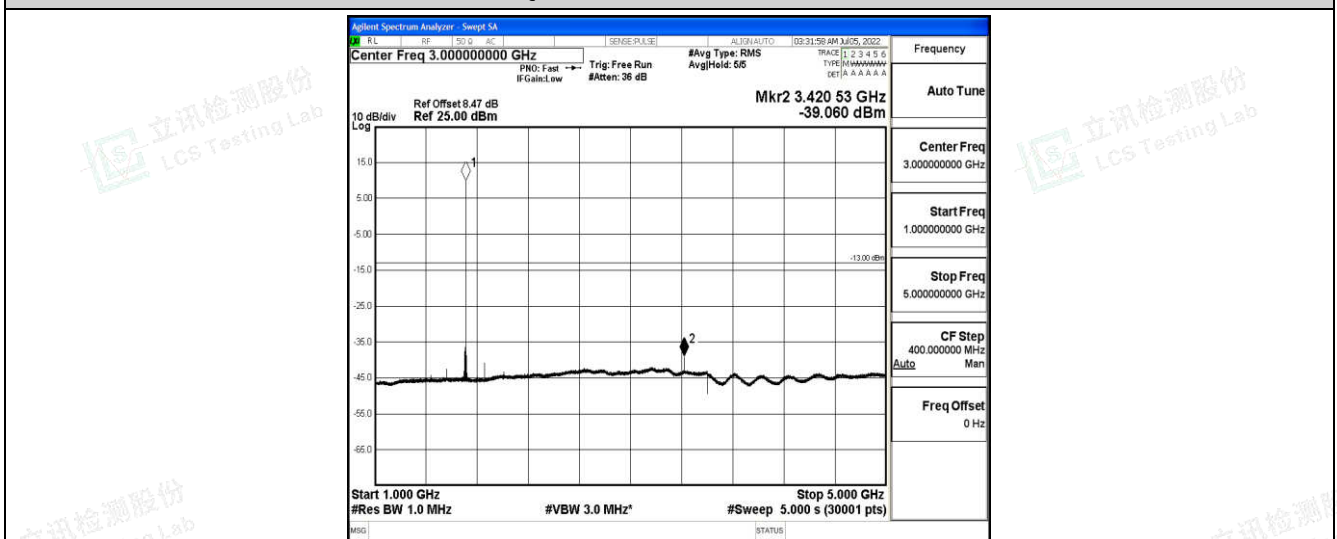
Band66-1.4MHz-16QAM-131979-1-0-Low-1000-5000--39.06-PASS
