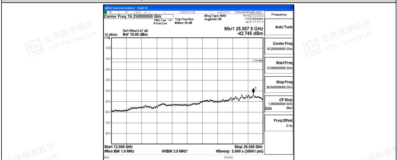
Band66-5MHz-QPSK-132322-1-0-Low-12000-26500--42.75-PASS
