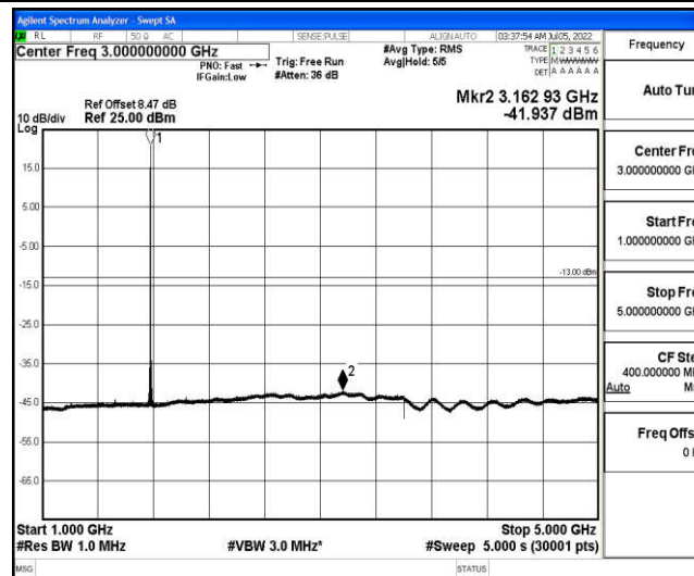
Band66-1.4MHz-QPSK-132665-1-0-High-1000-5000--41.94-PASS
