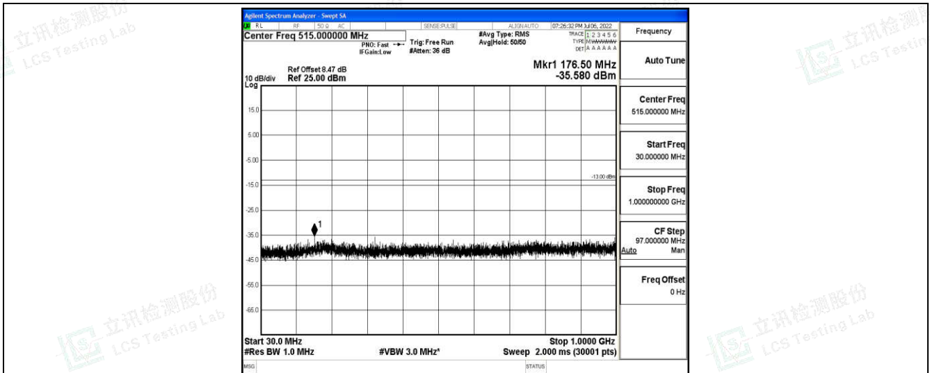
Band66-10MHz-16QAM-132622-1-0-High-30-1000--35.58-PASS
