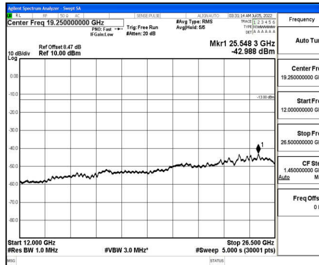
Band66-1.4MHz-QPSK-131979-1-0-Low-12000-26500--42.99-PASS
