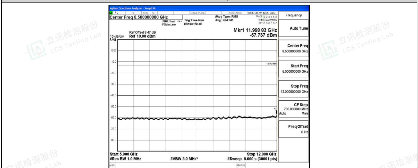
Band66-3MHz-QPSK-132657-1-0-High-5000-12000--57.74-PASS
