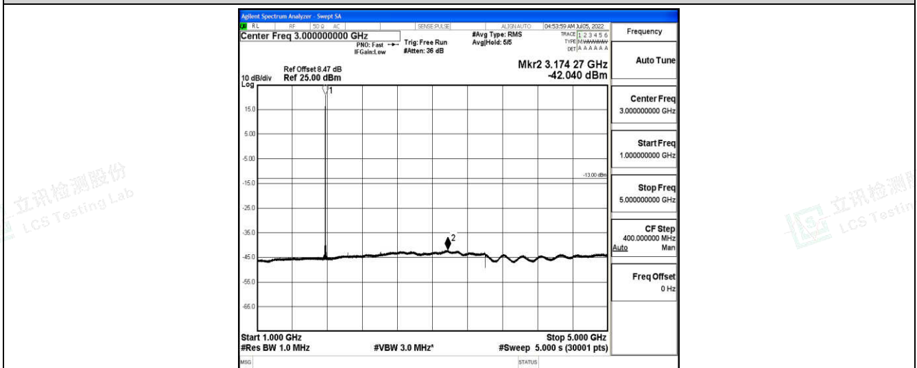
Band66-5MHz-QPSK-132647-1-0-High-1000-5000--42.04-PASS
