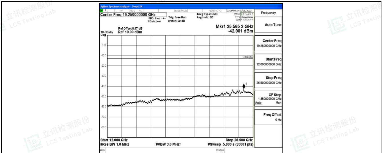
Band66-1.4MHz-QPSK-132665-1-0-High-12000-26500--42.9-PASS
