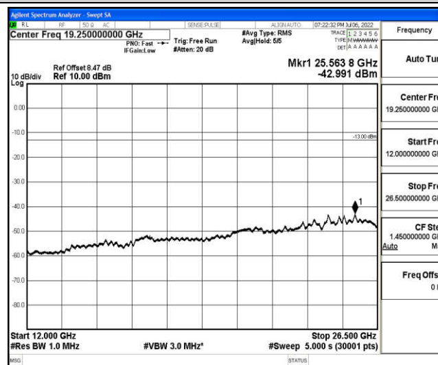
Band66-10MHz-QPSK-132322-1-0-Low-12000-26500--42.99-PASS
