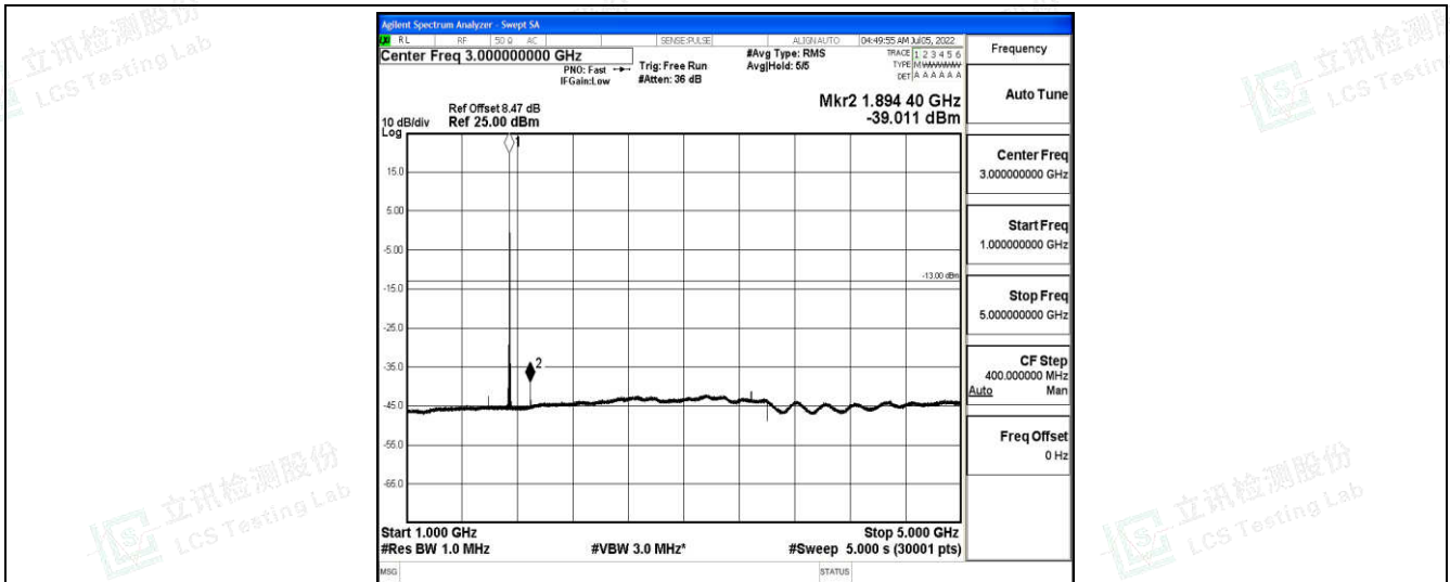
Band66-5MHz-QPSK-132322-1-0-Low-1000-5000--39.01-PASS
