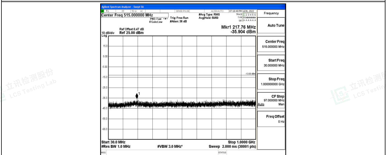
Band66-10MHz-16QAM-132022-1-0-Low-30-1000--35.9-PASS
