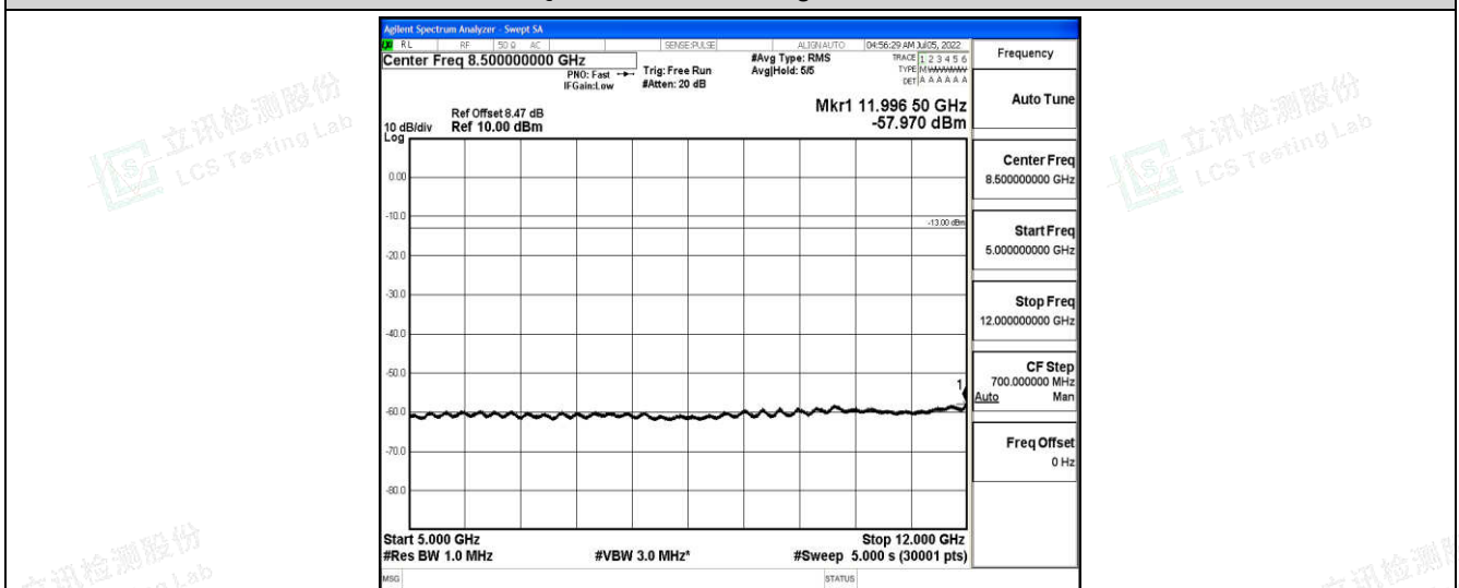
Band66-5MHz-16QAM-132647-1-0-High-5000-12000--57.97-PASS
