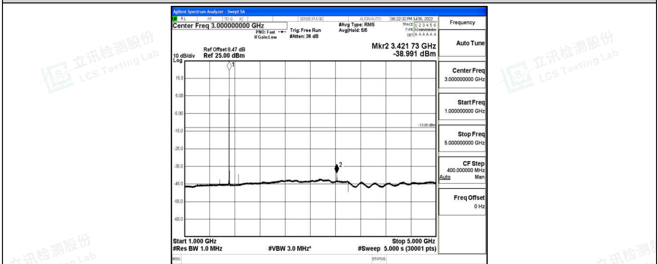
Band66-15MHz-QPSK-132047-1-0-Low-1000-5000--38.99-PASS
