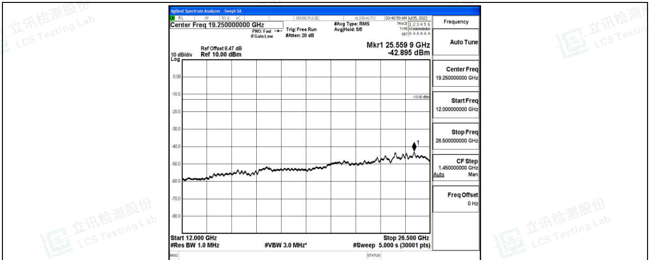
Band66-1.4MHz-16QAM-132665-1-0-High-12000-26500--42.9-PASS
