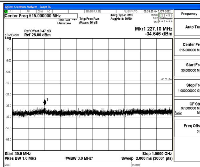
Band66-1.4MHz-QPSK-132322-1-0-Low-30-1000--34.65-PASS
