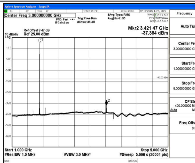
Band66-10MHz-QPSK-132022-1-0-Low-1000-5000--37.38-PASS
