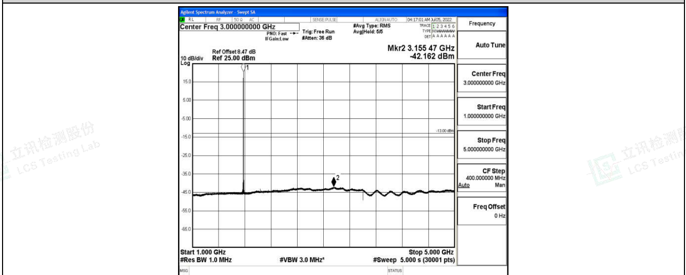
Band66-3MHz-QPSK-132657-1-0-High-1000-5000--42.16-PASS
