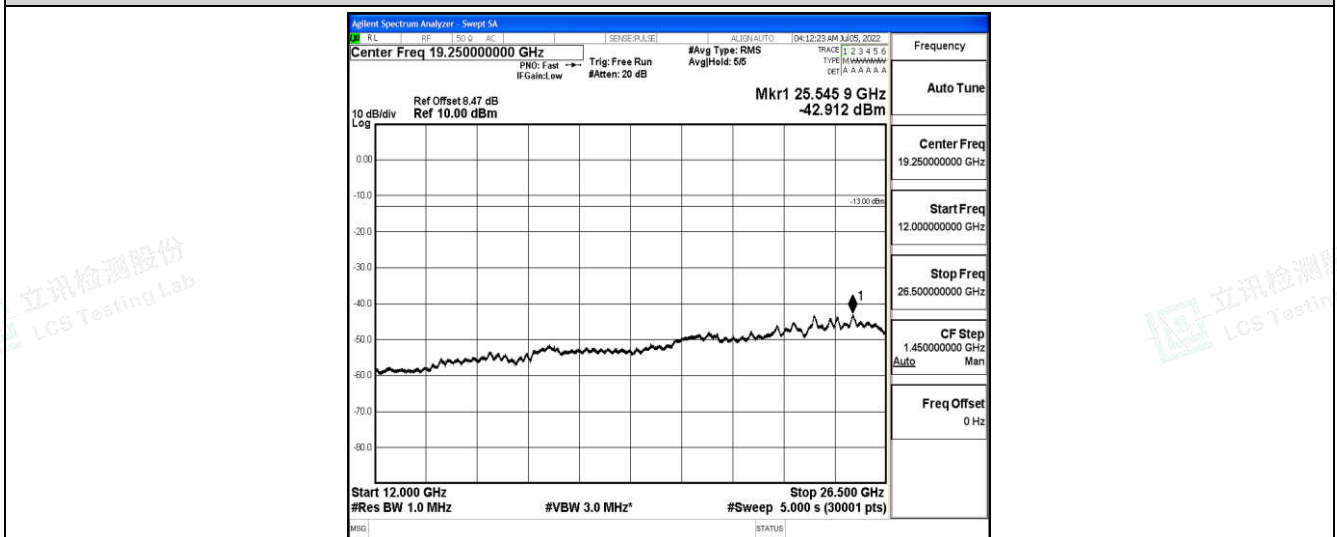
Band66-3MHz-16QAM-131987-1-0-Low-12000-26500--42.91-PASS
