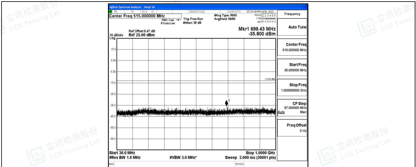
Band66-10MHz-QPSK-132622-1-0-High-30-1000--35.8-PASS
