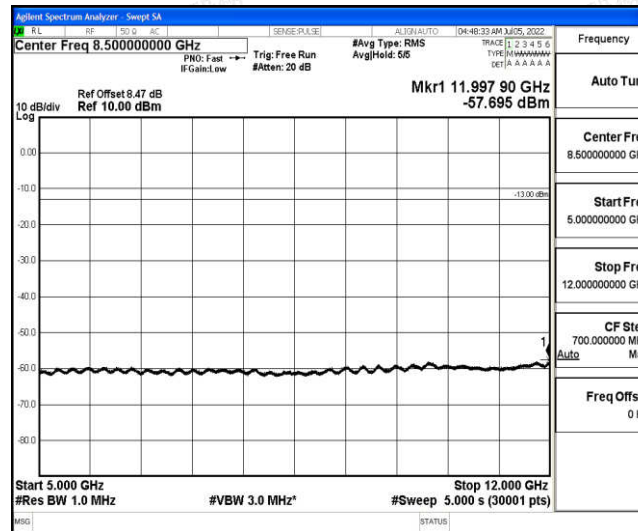
Band66-5MHz-16QAM-131997-1-0-Low-5000-12000--57.7-PASS
