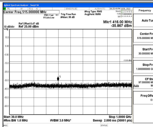
Band66-15MHz-QPSK-132322-1-0-Low-30-1000--35.87-PASS
