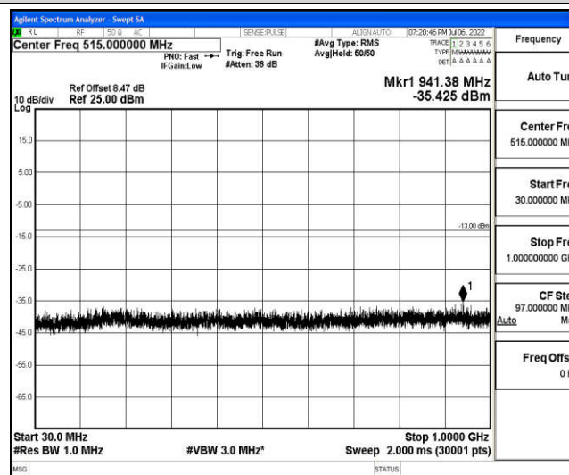
Band66-10MHz-QPSK-132322-1-0-Low-30-1000--35.43-PASS
