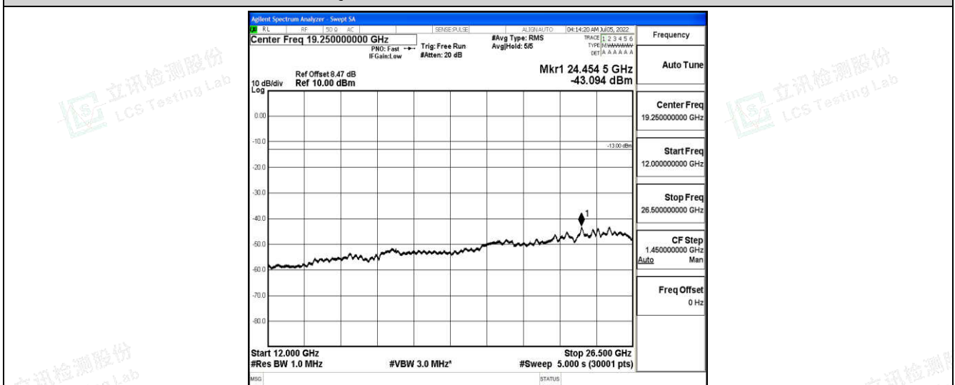
Band66-3MHz-QPSK-132322-1-0-Low-12000-26500--43.09-PASS
