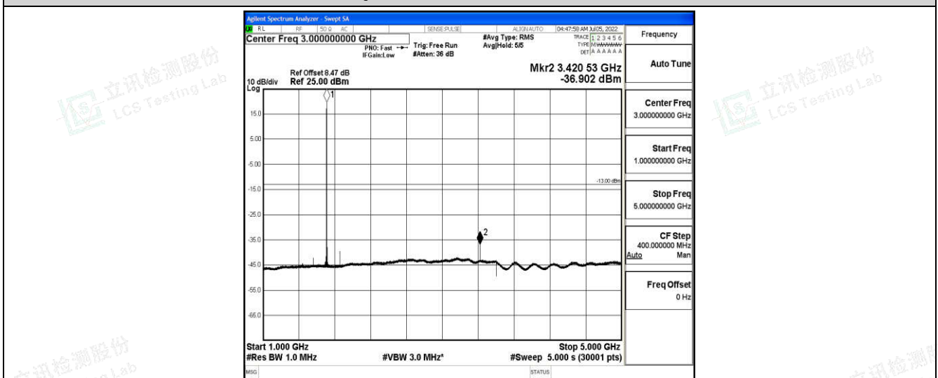
Band66-5MHz-16QAM-131997-1-0-Low-1000-5000--36.9-PASS
