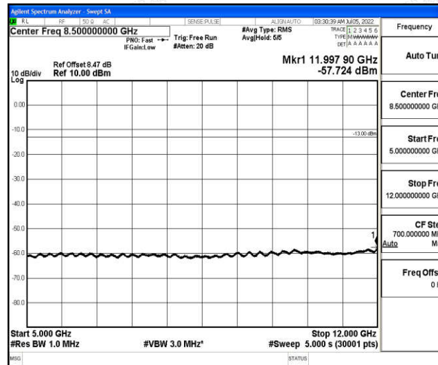
Band66-1.4MHz-QPSK-131979-1-0-Low-5000-12000--57.72-PASS
