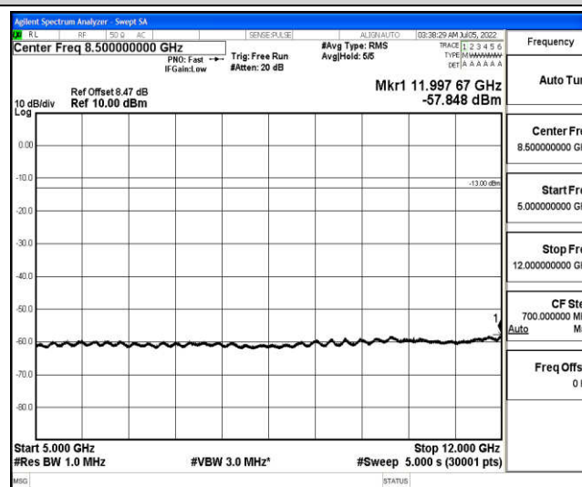
Band66-1.4MHz-QPSK-132665-1-0-High-5000-12000--57.85-PASS
