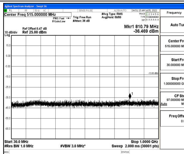
Band66-5MHz-16QAM-132322-1-0-Low-30-1000--36.47-PASS
