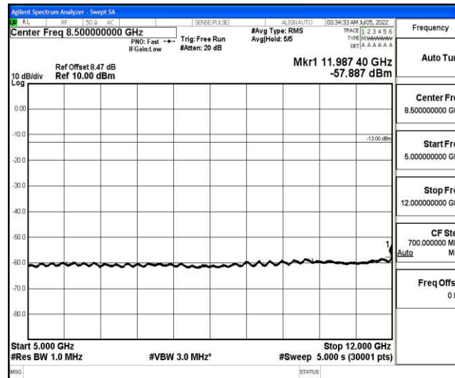
Band66-1.4MHz-QPSK-132322-1-0-Low-5000-12000--57.89-PASS
