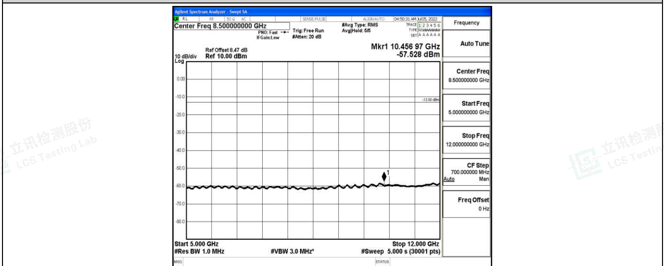
Band66-5MHz-QPSK-132322-1-0-Low-5000-12000--57.53-PASS
