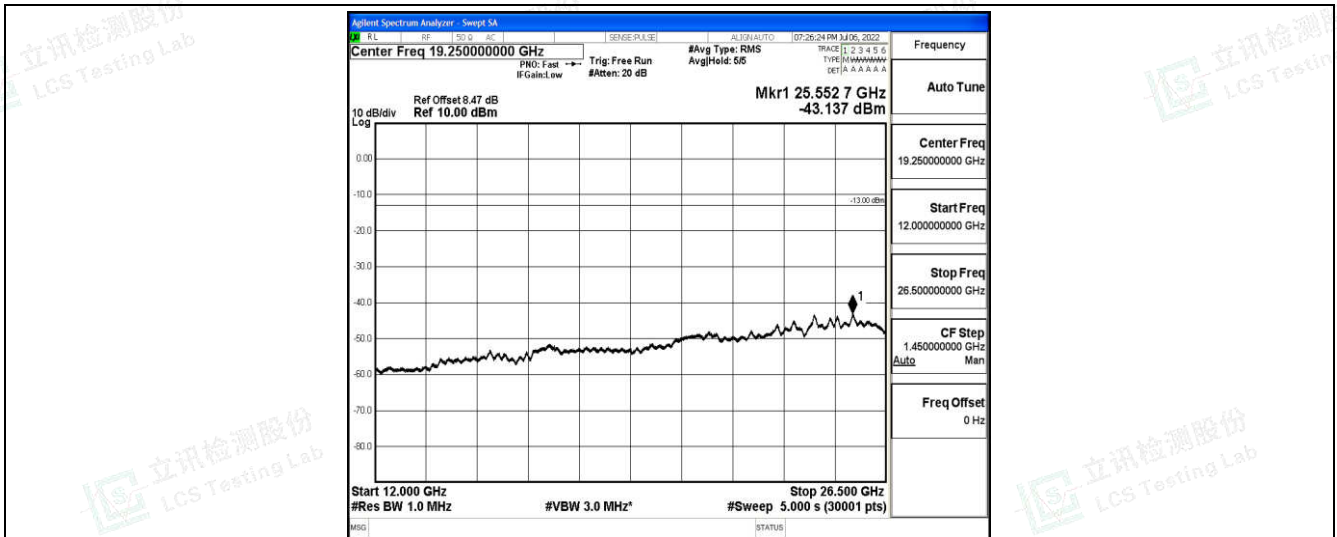
Band66-10MHz-QPSK-132622-1-0-High-12000-26500--43.14-PASS
