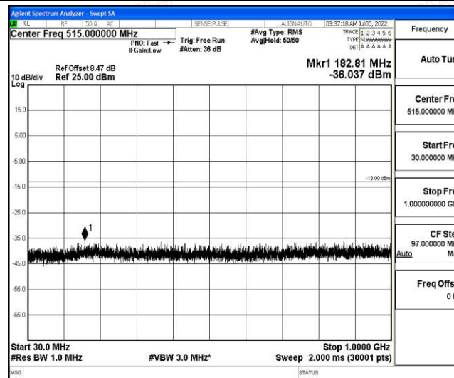
Band66-1.4MHz-QPSK-132665-1-0-High-30-1000--36.04-PASS
