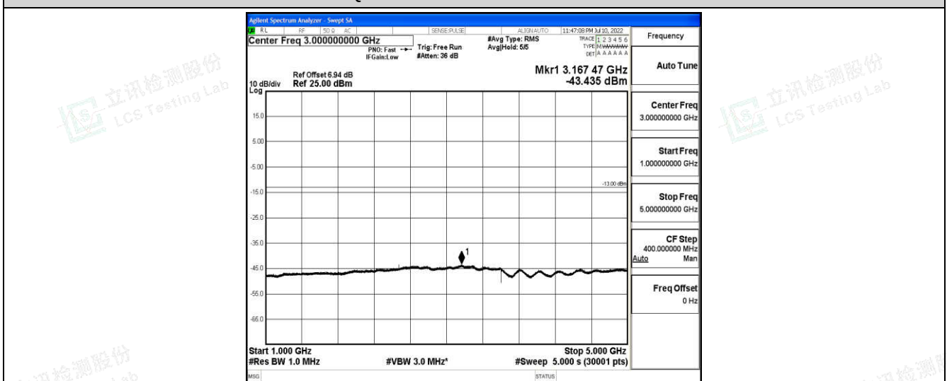
Band26-3MHz-QPSK-26805-1-0-Low-1000-5000--43.44-PASS
