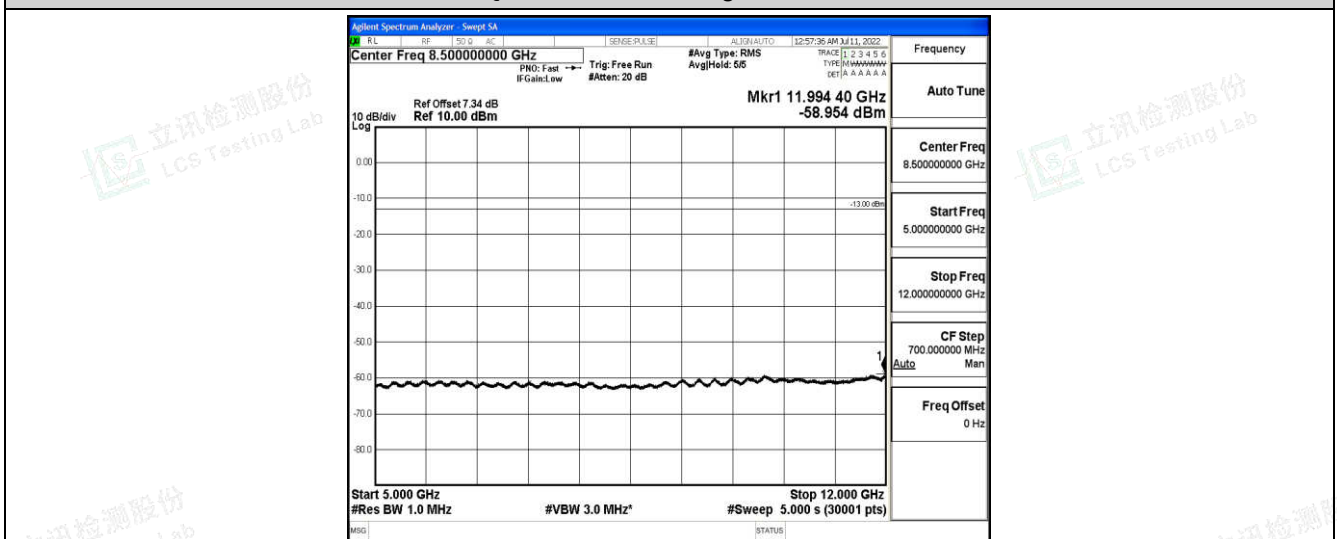
Band26-15MHz-QPSK-26965-1-0-High-5000-12000--58.95-PASS
