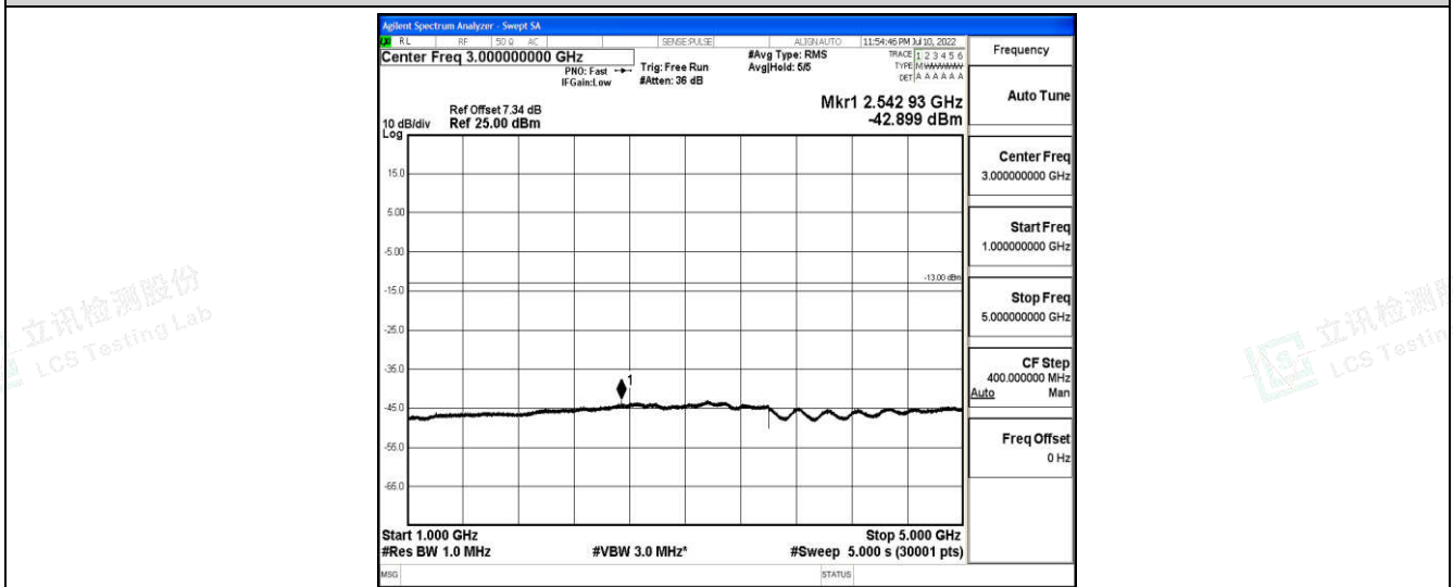
Band26-3MHz-QPSK-27025-1-0-High-1000-5000--42.9-PASS
