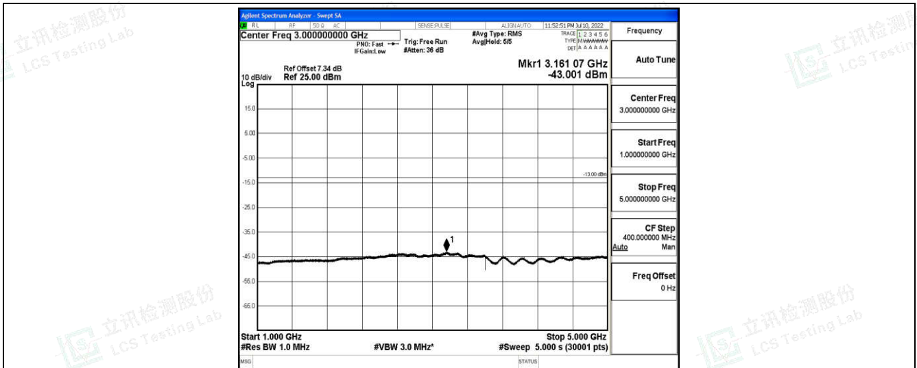
Band26-3MHz-16QAM-26915-1-0-Low-1000-5000--43-PASS
