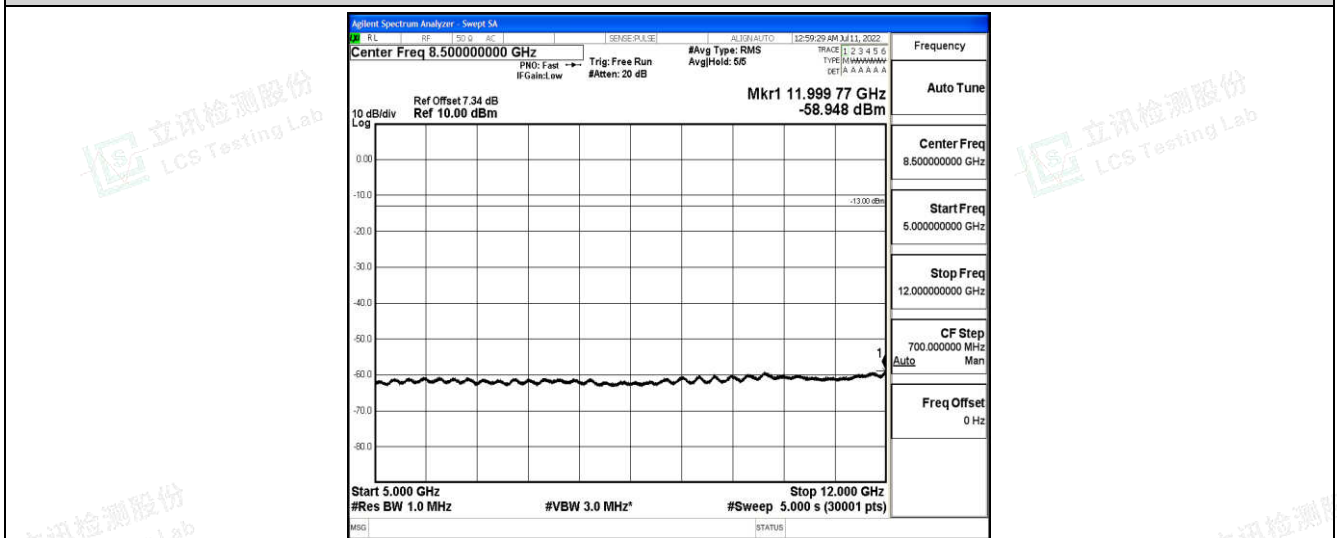
Band26-15MHz-16QAM-26965-1-0-High-5000-12000--58.95-PASS
