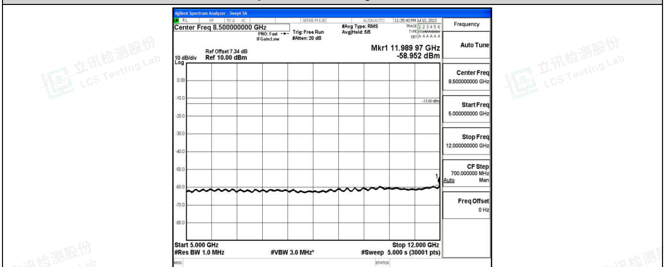
Band26-1.4MHz-16QAM-27033-1-0-High-5000-12000--58.95-PASS
