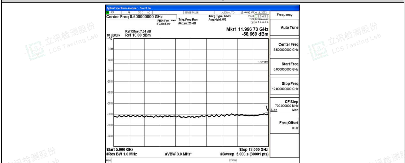
Band26-10MHz-16QAM-26990-1-0-High-5000-12000--58.67-PASS
