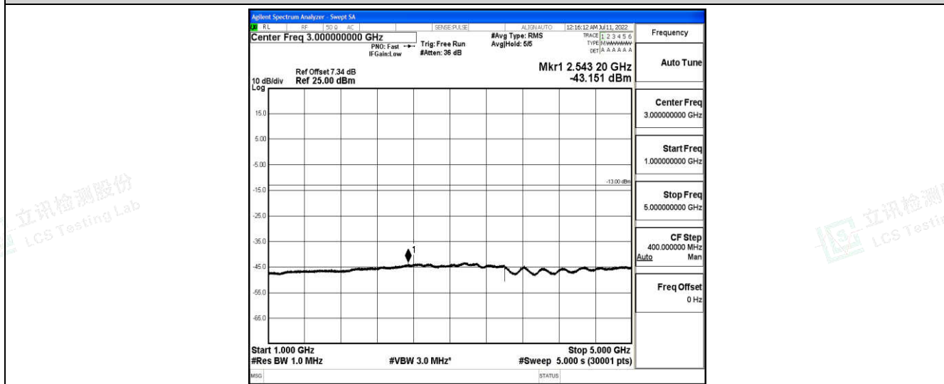
Band26-5MHz-QPSK-27015-1-0-High-1000-5000--43.15-PASS
