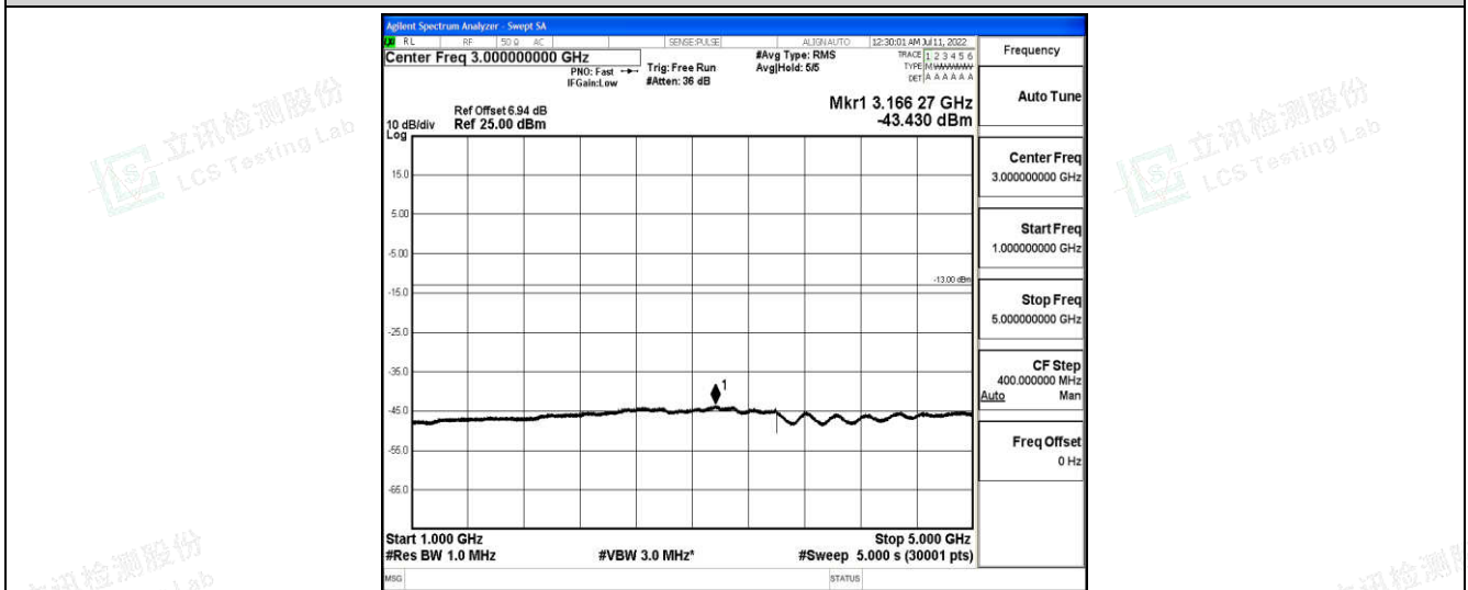
Band26-10MHz-QPSK-26840-1-0-Low-1000-5000--43.43-PASS
