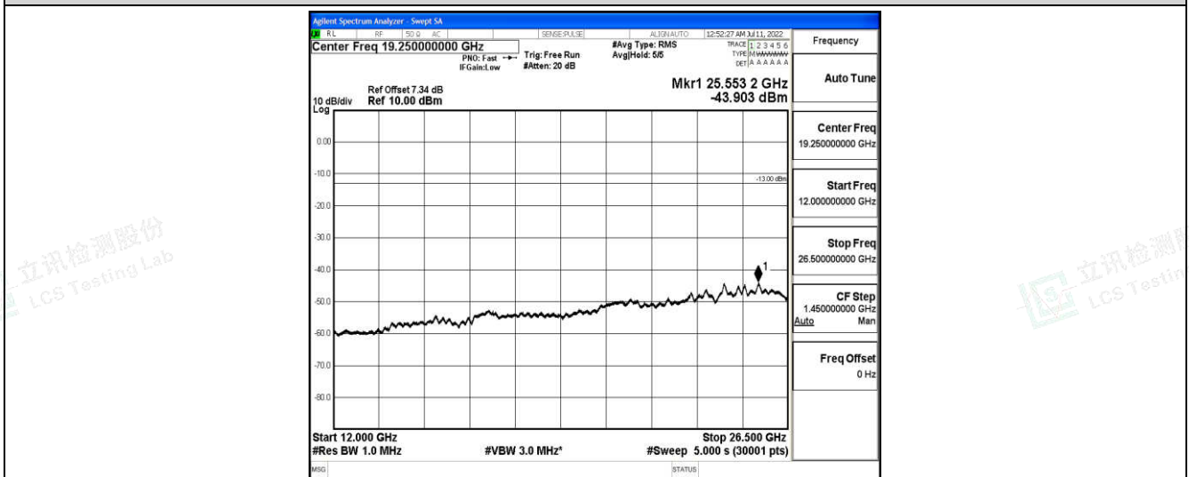
Band26-15MHz-16QAM-26865-1-0-Low-12000-26500--43.9-PASS
