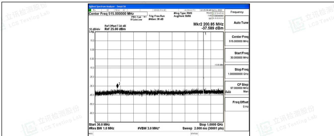
Band26-5MHz-QPSK-27015-1-0-High-30-1000--37.59-PASS
