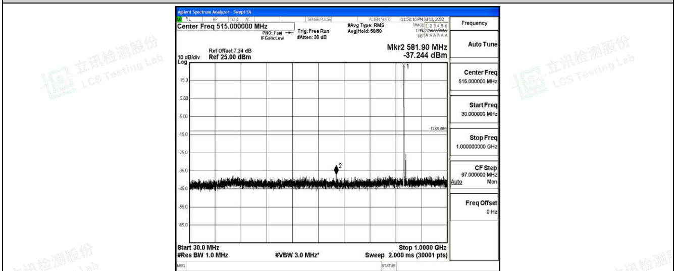
Band26-3MHz-16QAM-26915-1-0-Low-30-1000--37.24-PASS
