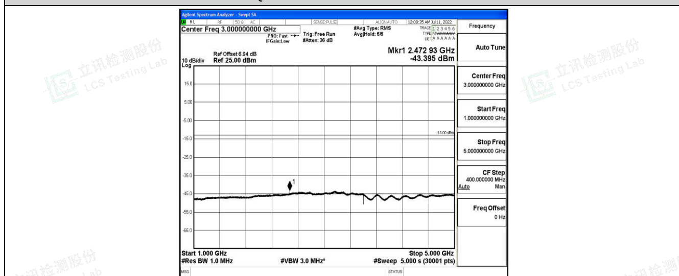
Band26-5MHz-QPSK-26815-1-0-Low-1000-5000--43.4-PASS
