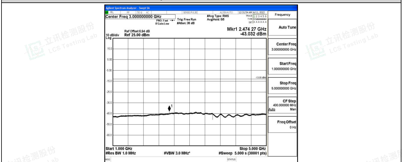
Band26-10MHz-16QAM-26840-1-0-Low-1000-5000--43.03-PASS
