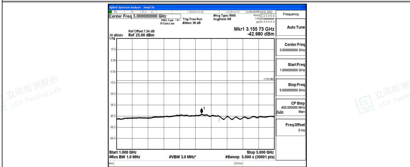
Band26-3MHz-16QAM-27025-1-0-High-1000-5000--42.98-PASS
