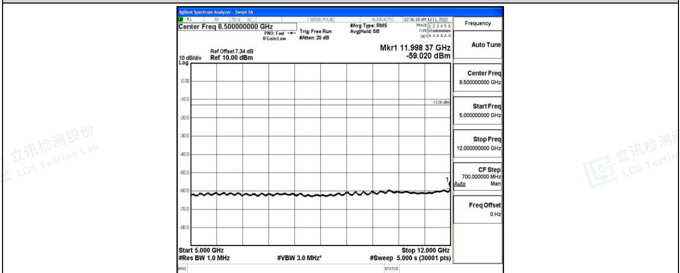
Band26-10MHz-16QAM-26915-1-0-Low-5000-12000--59.02-PASS
