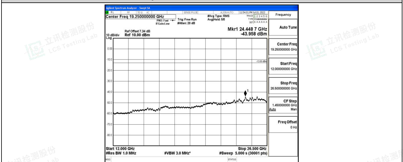
Band26-3MHz-16QAM-26915-1-0-Low-12000-26500--43.96-PASS
