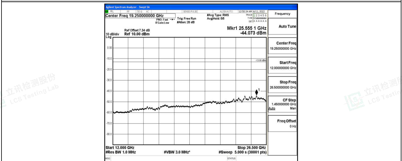
Band26-15MHz-QPSK-26865-1-0-Low-12000-26500--44.07-PASS
