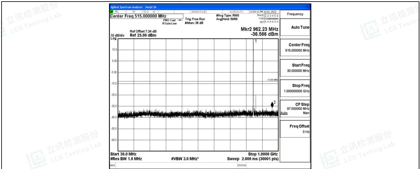
Band26-3MHz-QPSK-27025-1-0-High-30-1000--36.57-PASS
