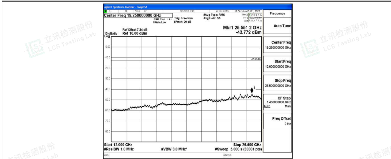
Band26-15MHz-16QAM-26915-1-0-Low-12000-26500--43.77-PASS
