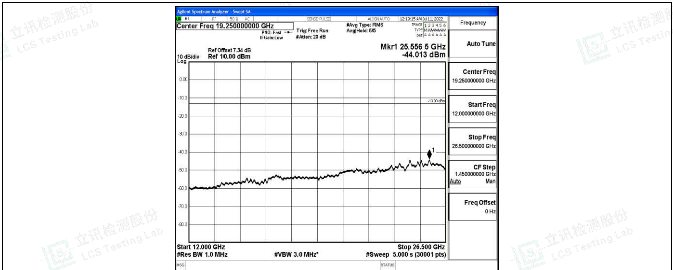
Band26-5MHz-16QAM-27015-1-0-High-12000-26500--44.01-PASS
