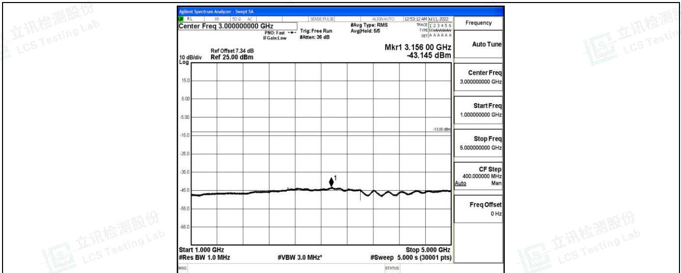
Band26-15MHz-QPSK-26915-1-0-Low-1000-5000--43.15-PASS
