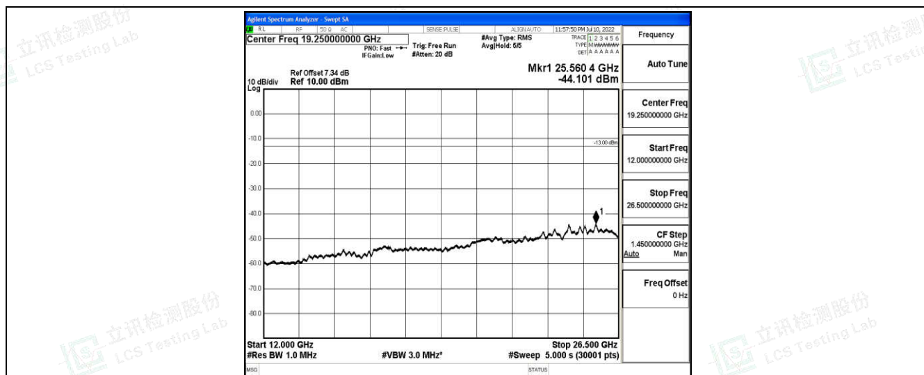
Band26-3MHz-16QAM-27025-1-0-High-12000-26500--44.1-PASS
