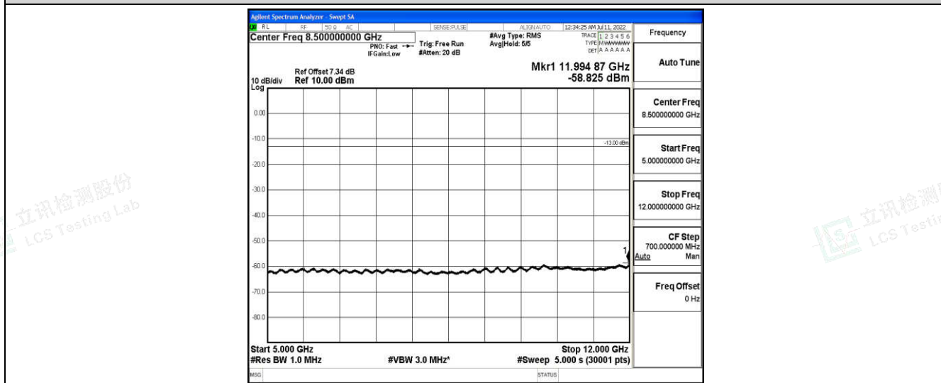
Band26-10MHz-QPSK-26915-1-0-Low-5000-12000--58.83-PASS
