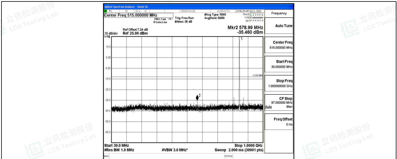
Band26-15MHz-QPSK-26965-1-0-High-30-1000--35.46-PASS
