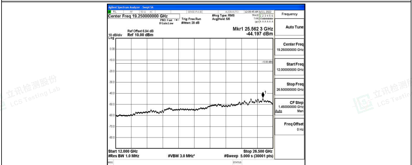
Band26-5MHz-QPSK-26815-1-0-Low-12000-26500--44.2-PASS
