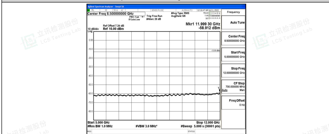
Band26-5MHz-QPSK-27015-1-0-High-5000-12000--58.91-PASS
