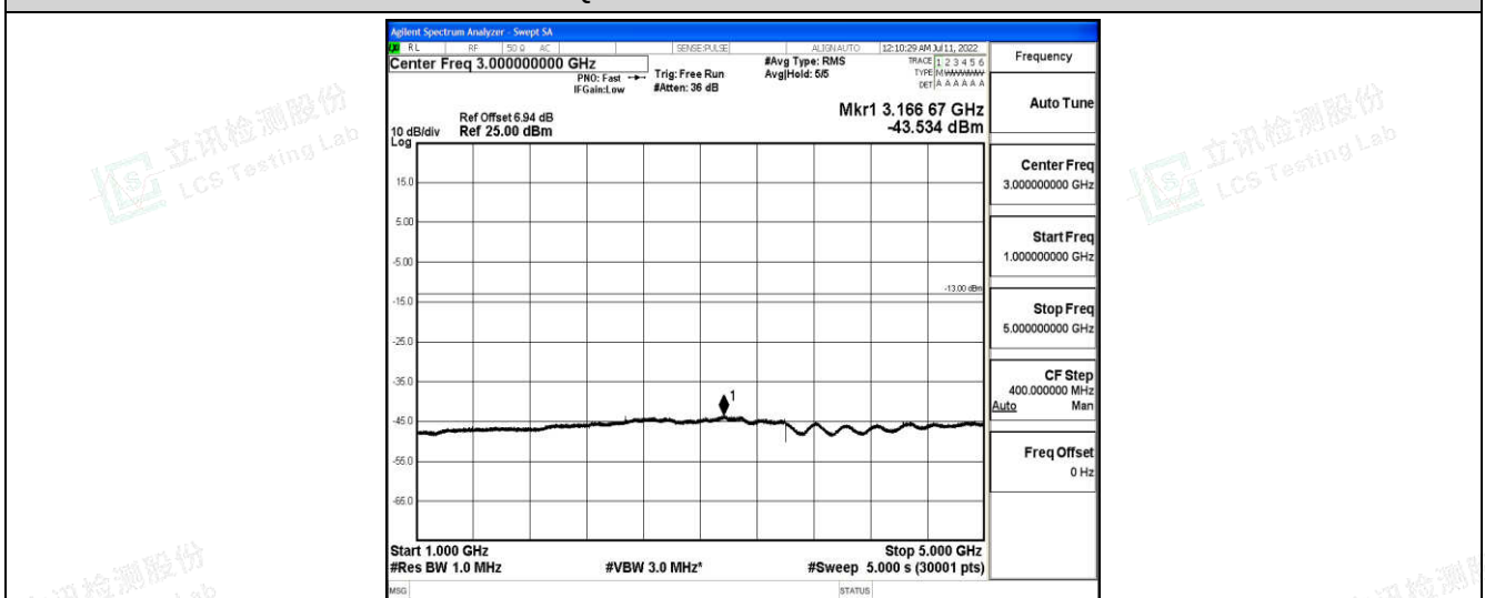
Band26-5MHz-16QAM-26815-1-0-Low-1000-5000--43.53-PASS
