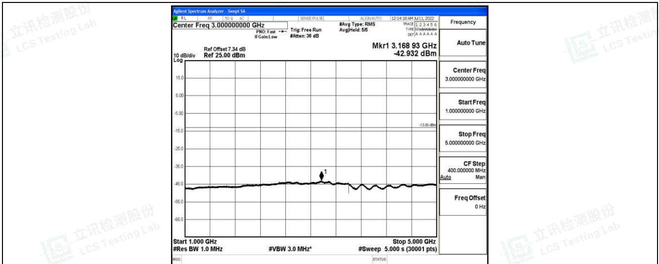
Band26-5MHz-16QAM-26915-1-0-Low-1000-5000--42.93-PASS
