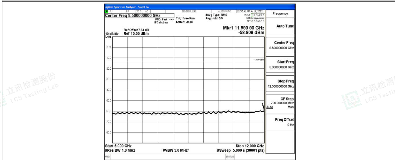
Band26-15MHz-16QAM-26915-1-0-Low-5000-12000--58.81-PASS
