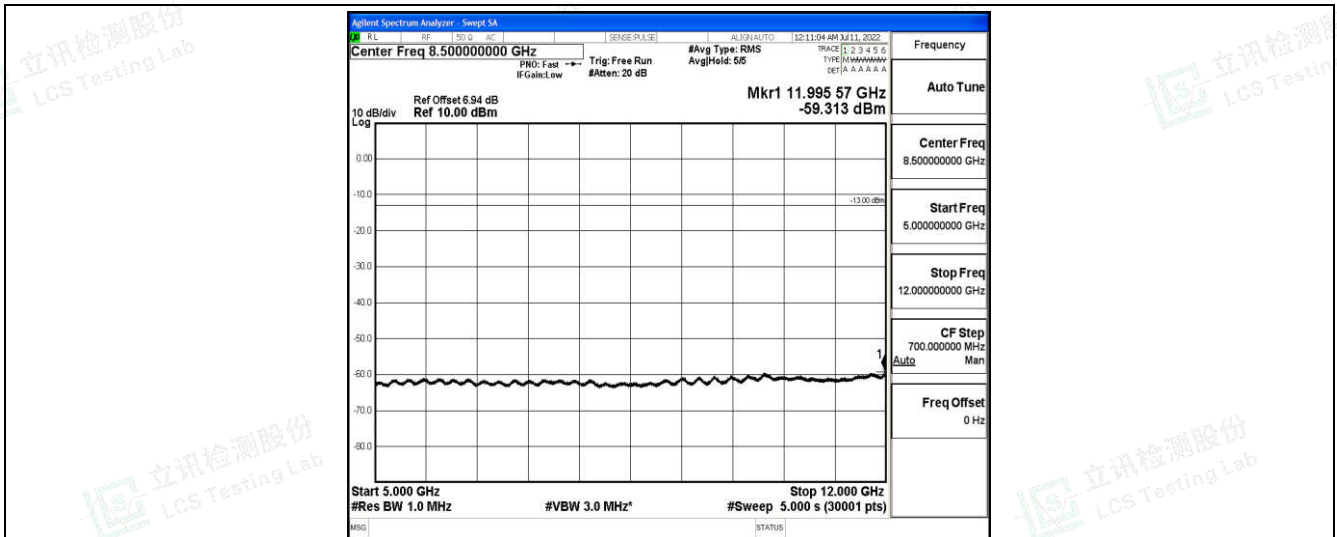
Band26-5MHz-16QAM-26815-1-0-Low-5000-12000--59.31-PASS
