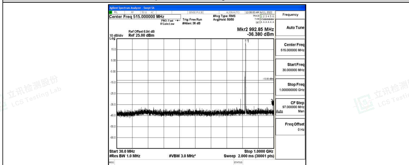
Band26-5MHz-QPSK-26815-1-0-Low-30-1000--36.38-PASS
