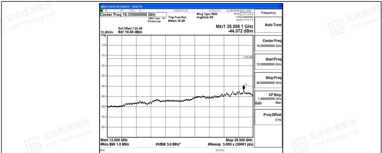
Band26-10MHz-QPSK-26990-1-0-High-12000-26500--44.07-PASS
