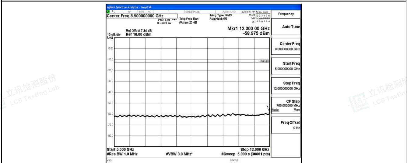
Band26-15MHz-QPSK-26915-1-0-Low-5000-12000--58.98-PASS
