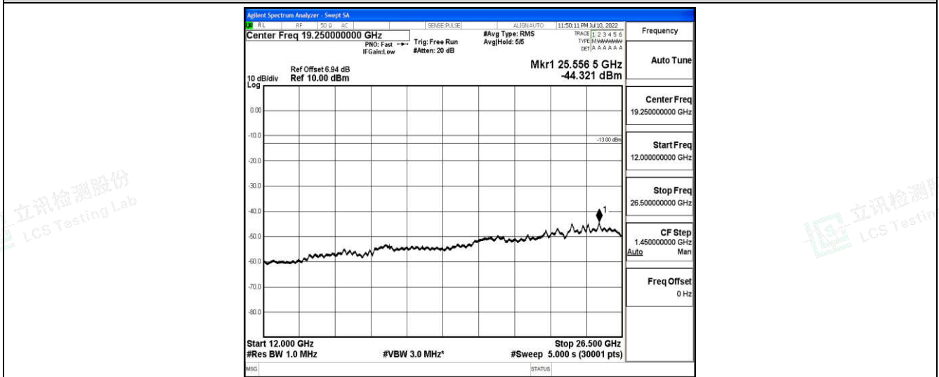
Band26-3MHz-16QAM-26805-1-0-Low-12000-26500--44.32-PASS
