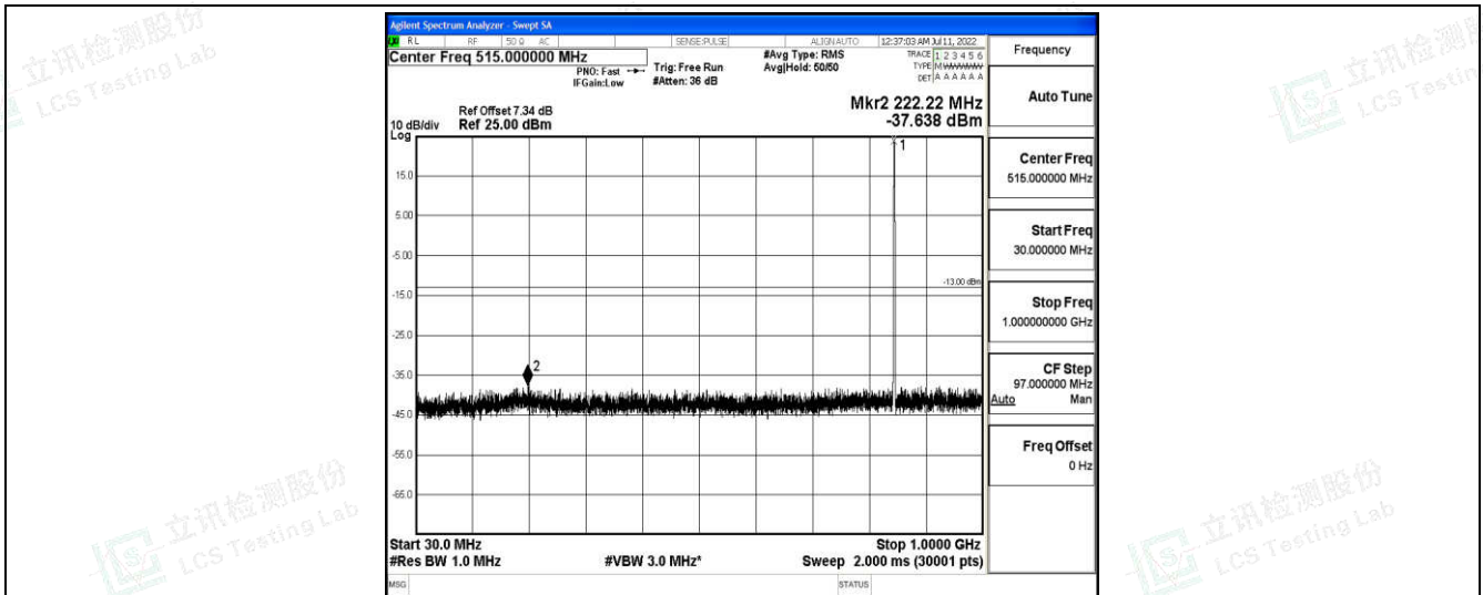
Band26-10MHz-QPSK-26990-1-0-High-30-1000--37.64-PASS
