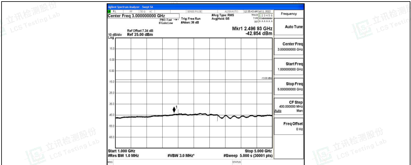
Band26-10MHz-16QAM-26915-1-0-Low-1000-5000--42.85-PASS
