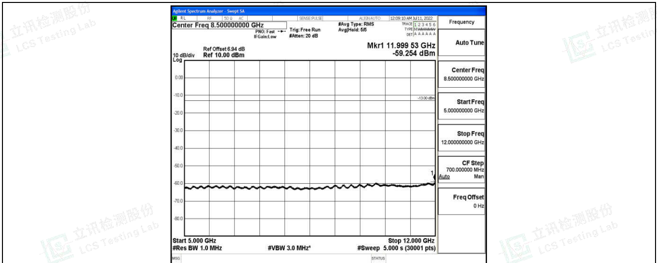
Band26-5MHz-QPSK-26815-1-0-Low-5000-12000--59.25-PASS
