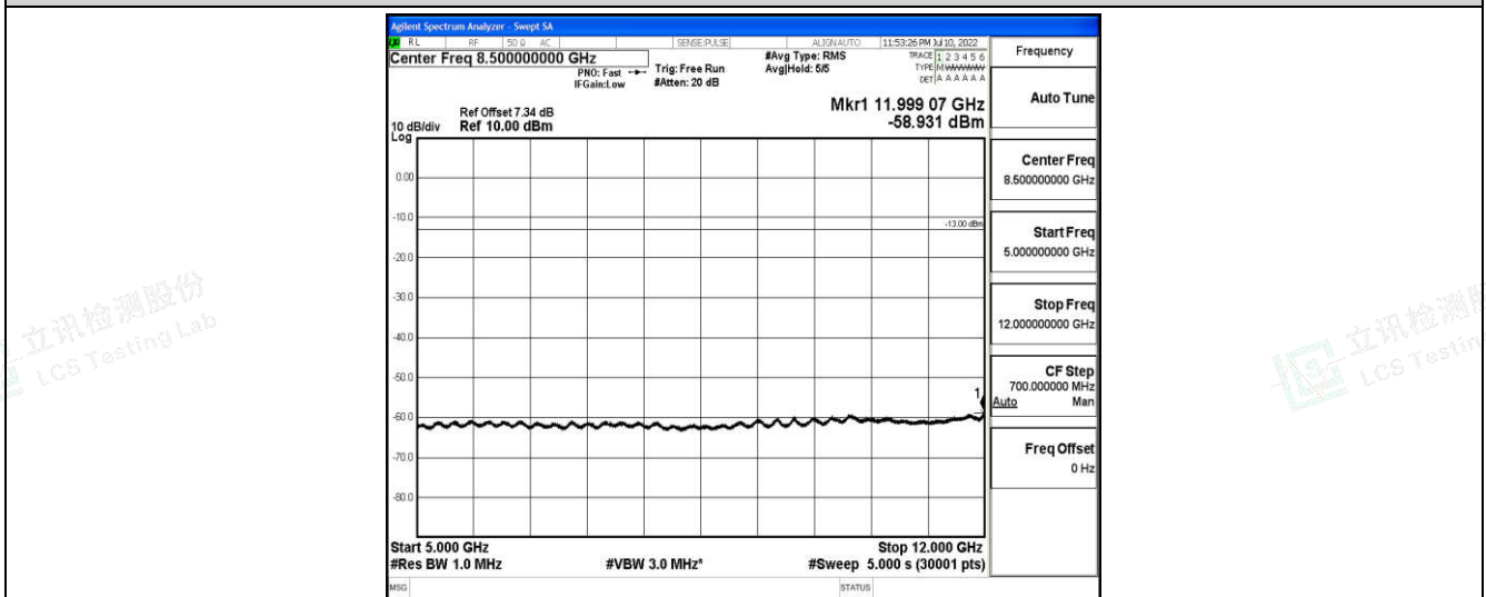
Band26-3MHz-16QAM-26915-1-0-Low-5000-12000--58.93-PASS
