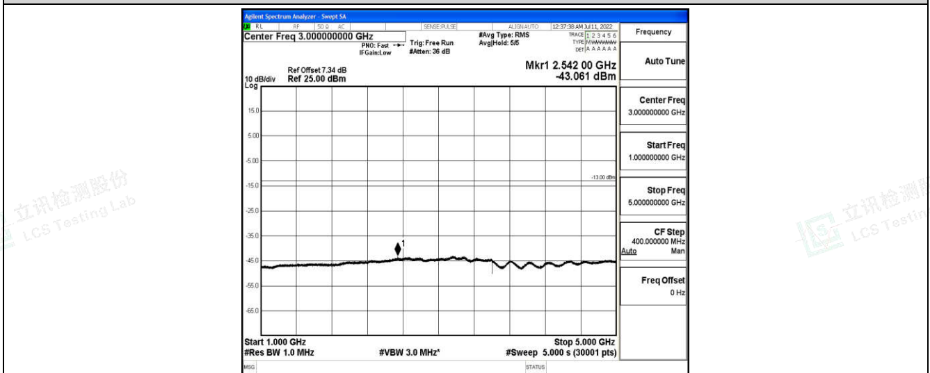
Band26-10MHz-QPSK-26990-1-0-High-1000-5000--43.06-PASS
