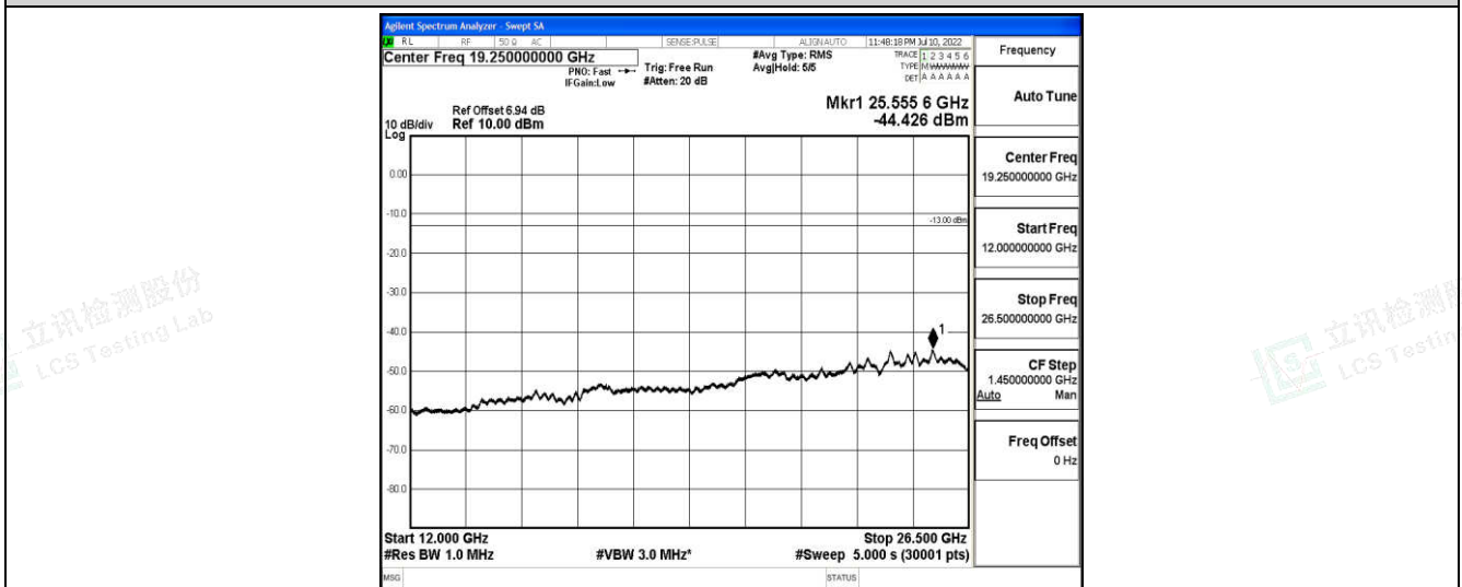
Band26-3MHz-QPSK-26805-1-0-Low-12000-26500--44.43-PASS
