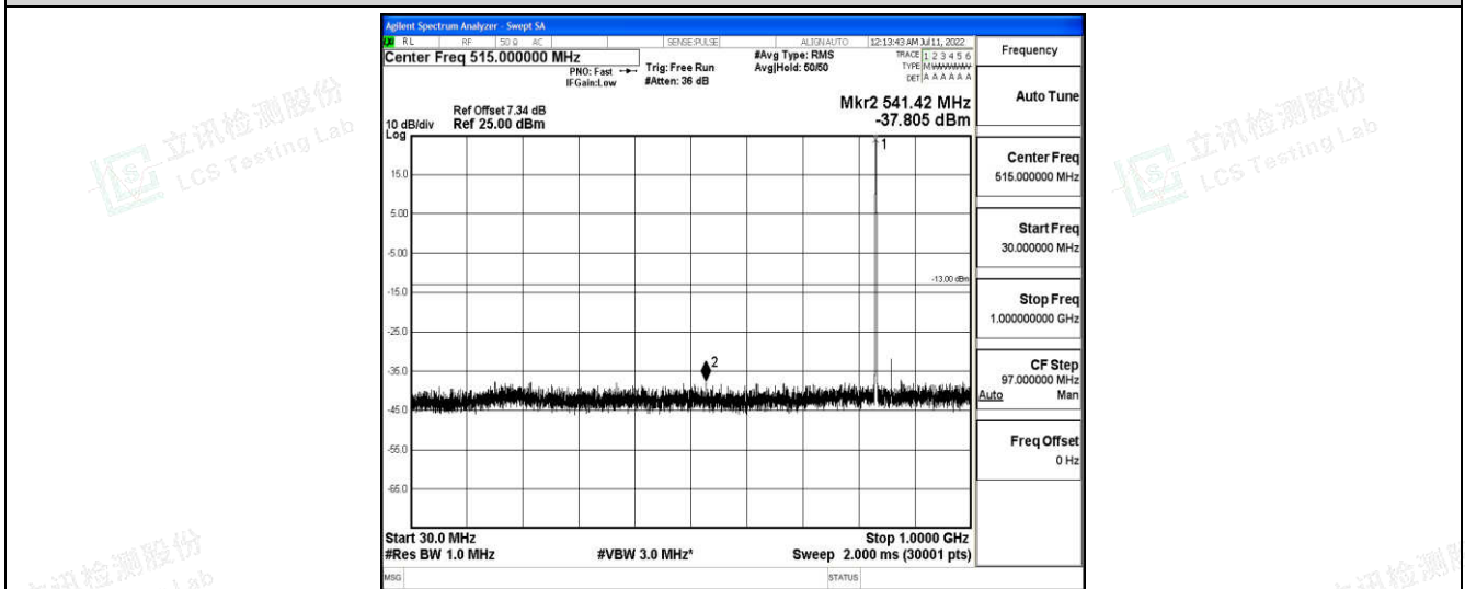
Band26-5MHz-16QAM-26915-1-0-Low-30-1000--37.81-PASS
