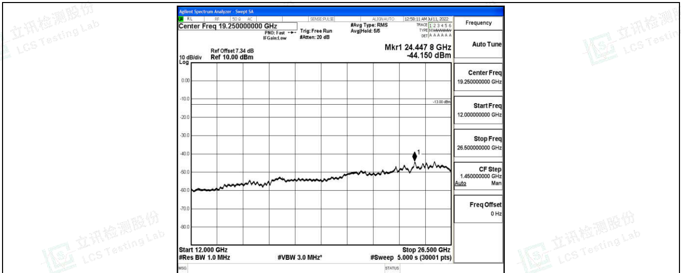
Band26-15MHz-QPSK-26965-1-0-High-12000-26500--44.15-PASS
