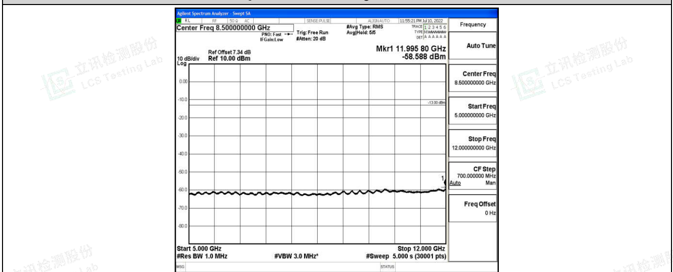
Band26-3MHz-QPSK-27025-1-0-High-5000-12000--58.59-PASS
