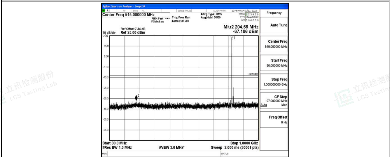
Band26-15MHz-QPSK-26865-1-0-Low-30-1000--37.11-PASS
