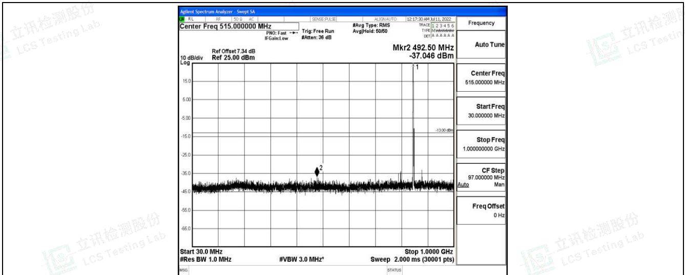
Band26-5MHz-16QAM-27015-1-0-High-30-1000--37.05-PASS
