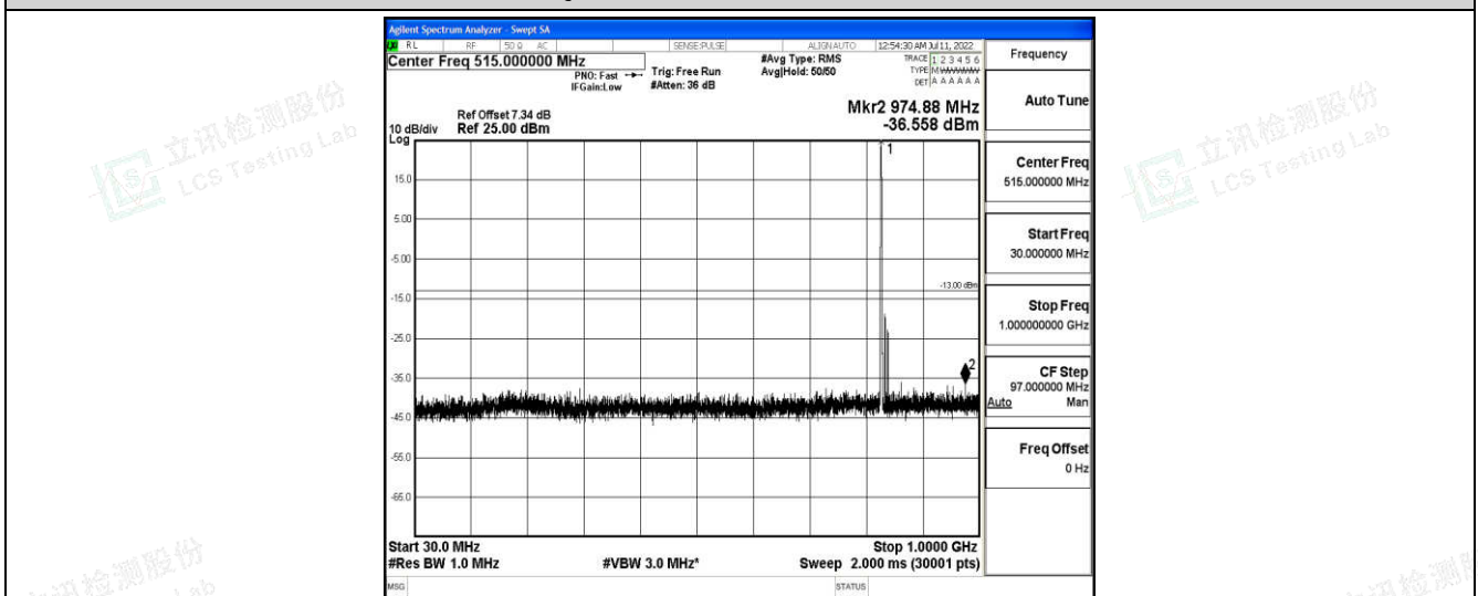
Band26-15MHz-16QAM-26915-1-0-Low-30-1000--36.56-PASS
