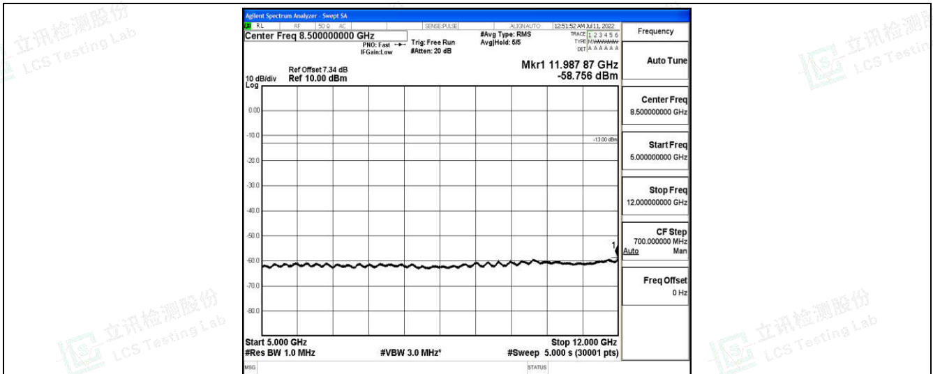
Band26-15MHz-16QAM-26865-1-0-Low-5000-12000--58.76-PASS
