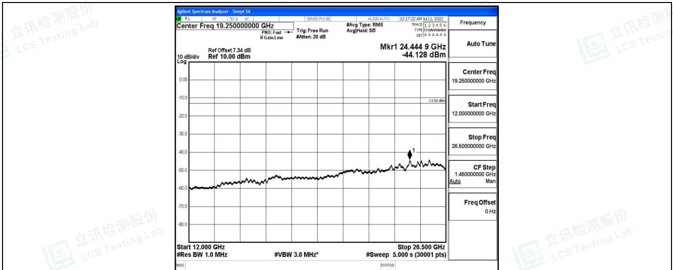
Band26-5MHz-QPSK-27015-1-0-High-12000-26500--44.13-PASS
