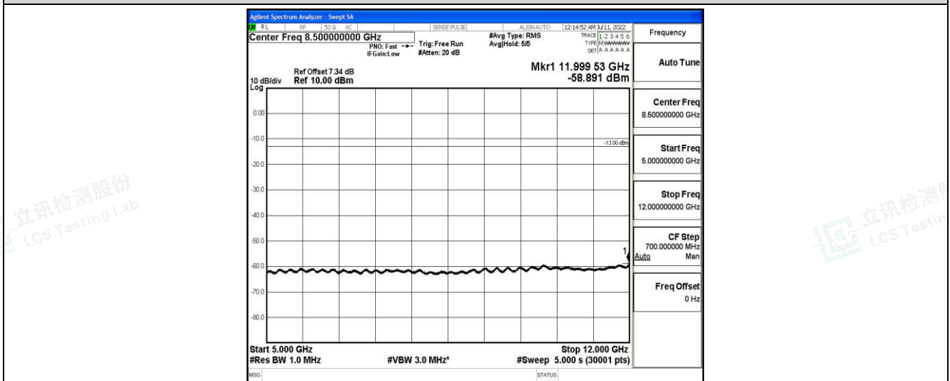
Band26-5MHz-16QAM-26915-1-0-Low-5000-12000--58.89-PASS
