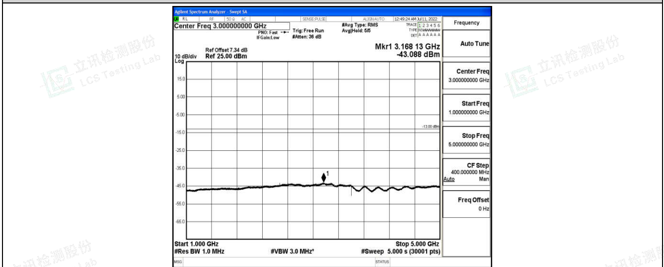
Band26-15MHz-QPSK-26865-1-0-Low-1000-5000--43.09-PASS
