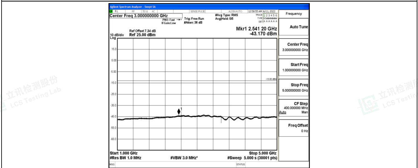
Band26-15MHz-16QAM-26965-1-0-High-1000-5000--43.17-PASS
