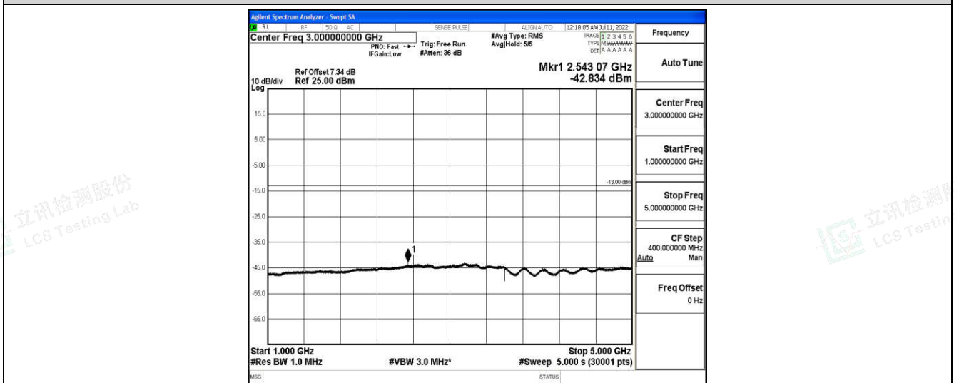
Band26-5MHz-16QAM-27015-1-0-High-1000-5000--42.83-PASS
