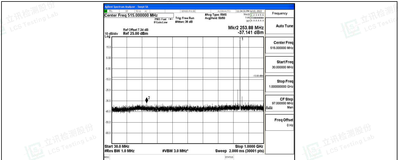
Band26-1.4MHz-16QAM-27033-1-0-High-30-1000--37.14-PASS
