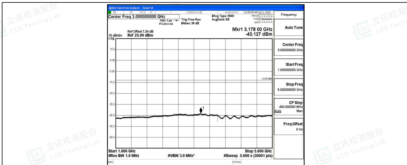
Band26-15MHz-16QAM-26915-1-0-Low-1000-5000--43.13-PASS
