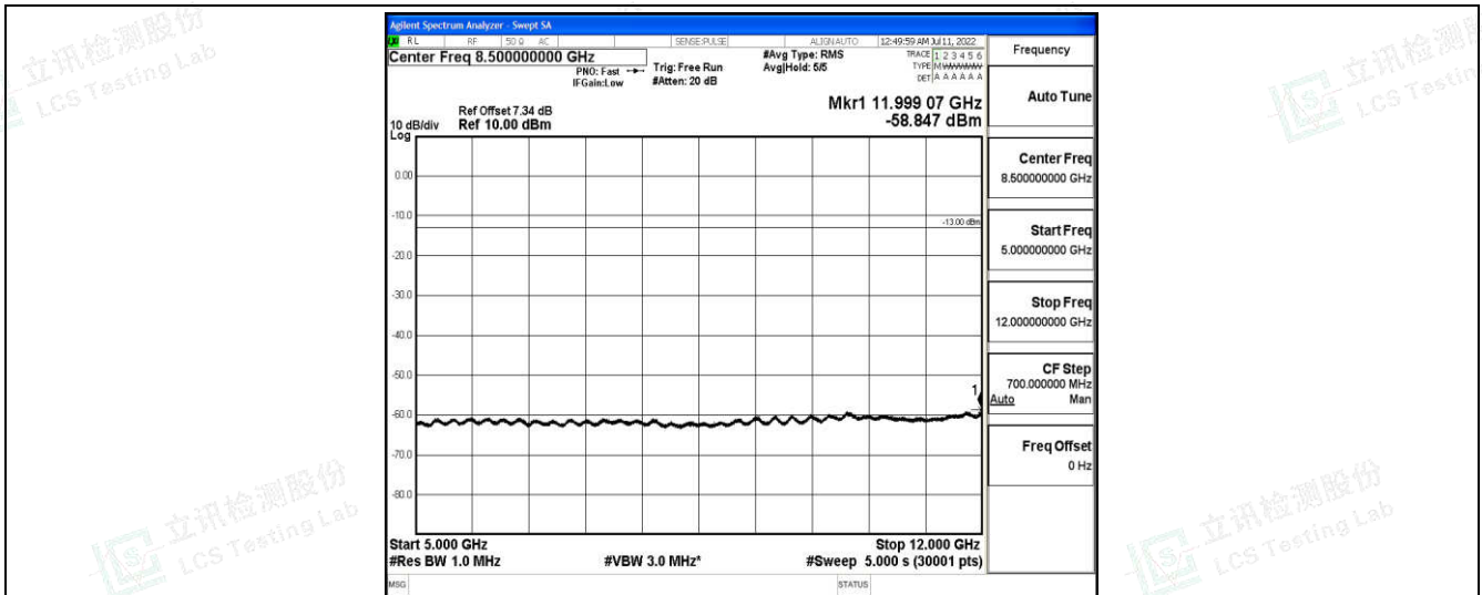
Band26-15MHz-QPSK-26865-1-0-Low-5000-12000--58.85-PASS
