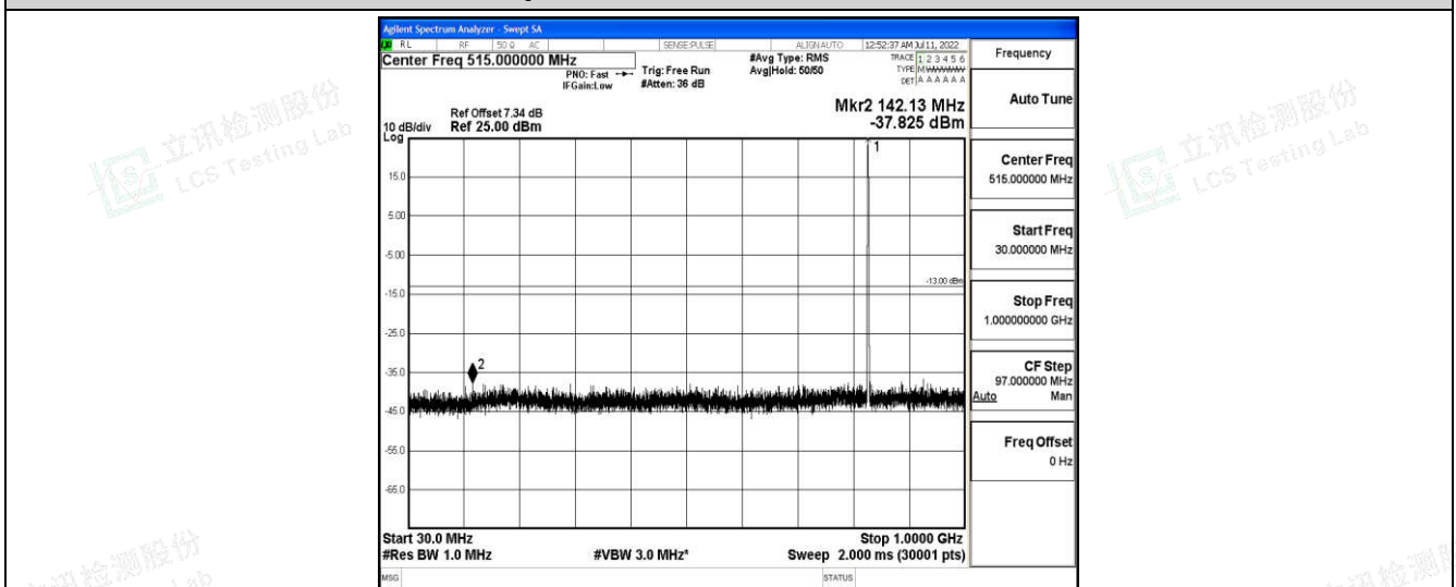
Band26-15MHz-QPSK-26915-1-0-Low-30-1000--37.83-PASS
