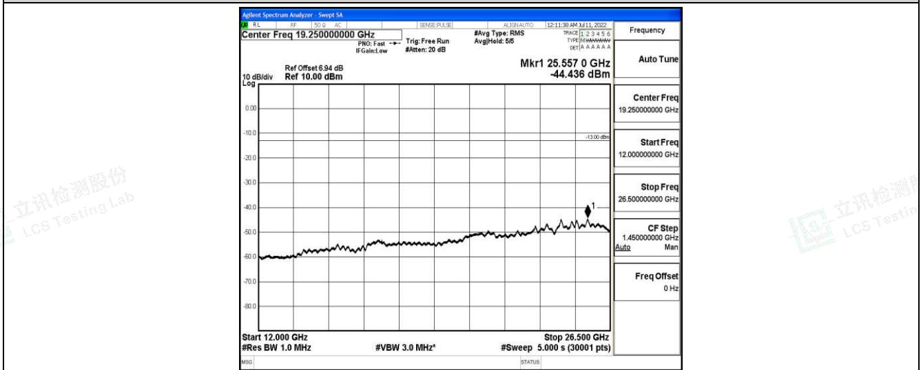
Band26-5MHz-16QAM-26815-1-0-Low-12000-26500--44.44-PASS
