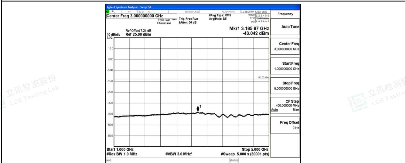
Band26-1.4MHz-16QAM-27033-1-0-High-1000-5000--43.04-PASS
