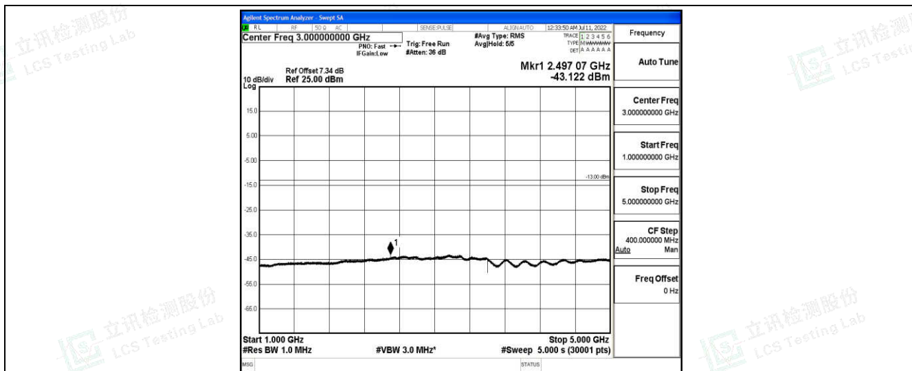
Band26-10MHz-QPSK-26915-1-0-Low-1000-5000--43.12-PASS
