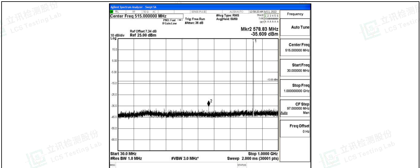
Band26-15MHz-16QAM-26965-1-0-High-30-1000--35.61-PASS
