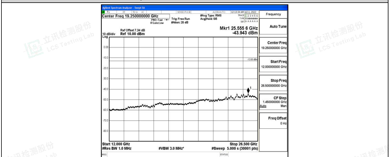
Band26-5MHz-QPSK-26915-1-0-Low-12000-26500--43.94-PASS
