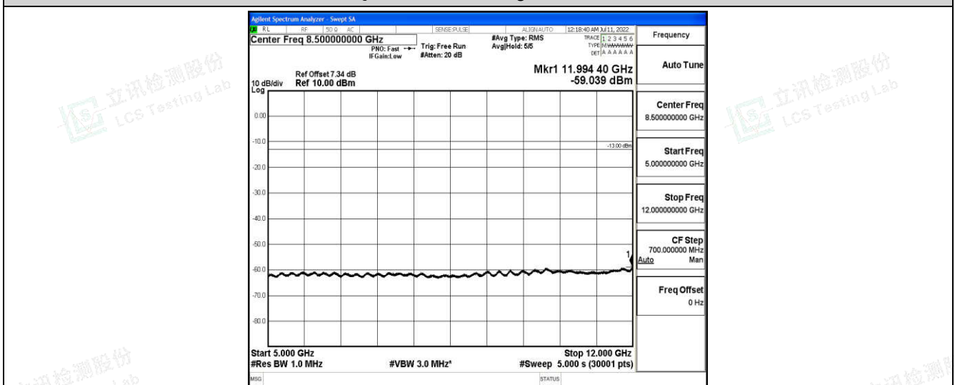
Band26-5MHz-16QAM-27015-1-0-High-5000-12000--59.04-PASS
