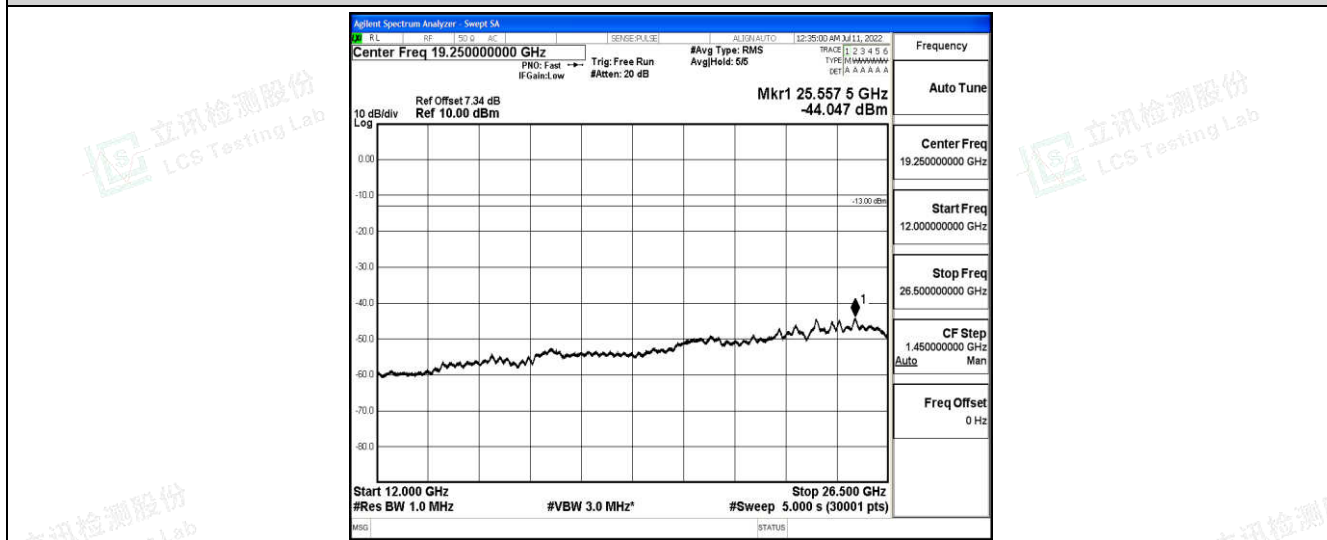
Band26-10MHz-QPSK-26915-1-0-Low-12000-26500--44.05-PASS
