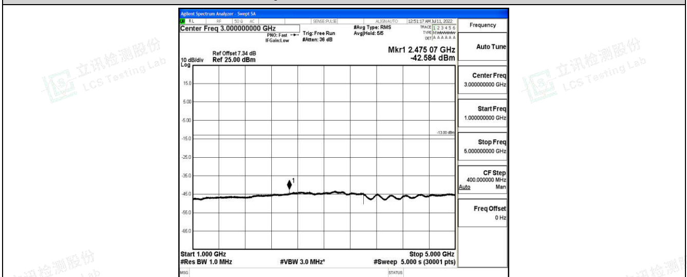
Band26-15MHz-16QAM-26865-1-0-Low-1000-5000--42.58-PASS
