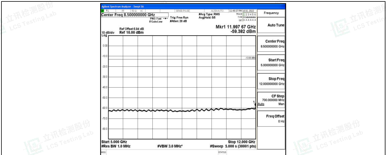
Band26-3MHz-16QAM-26805-1-0-Low-5000-12000--59.38-PASS
