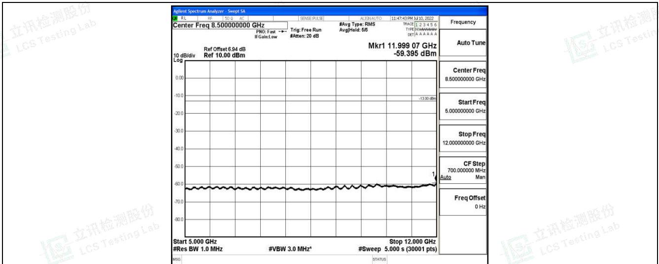
Band26-3MHz-QPSK-26805-1-0-Low-5000-12000--59.4-PASS
