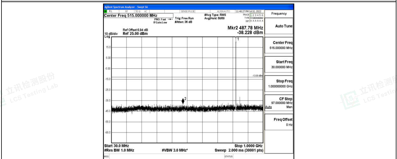
Band26-3MHz-16QAM-26805-1-0-Low-30-1000--38.23-PASS
