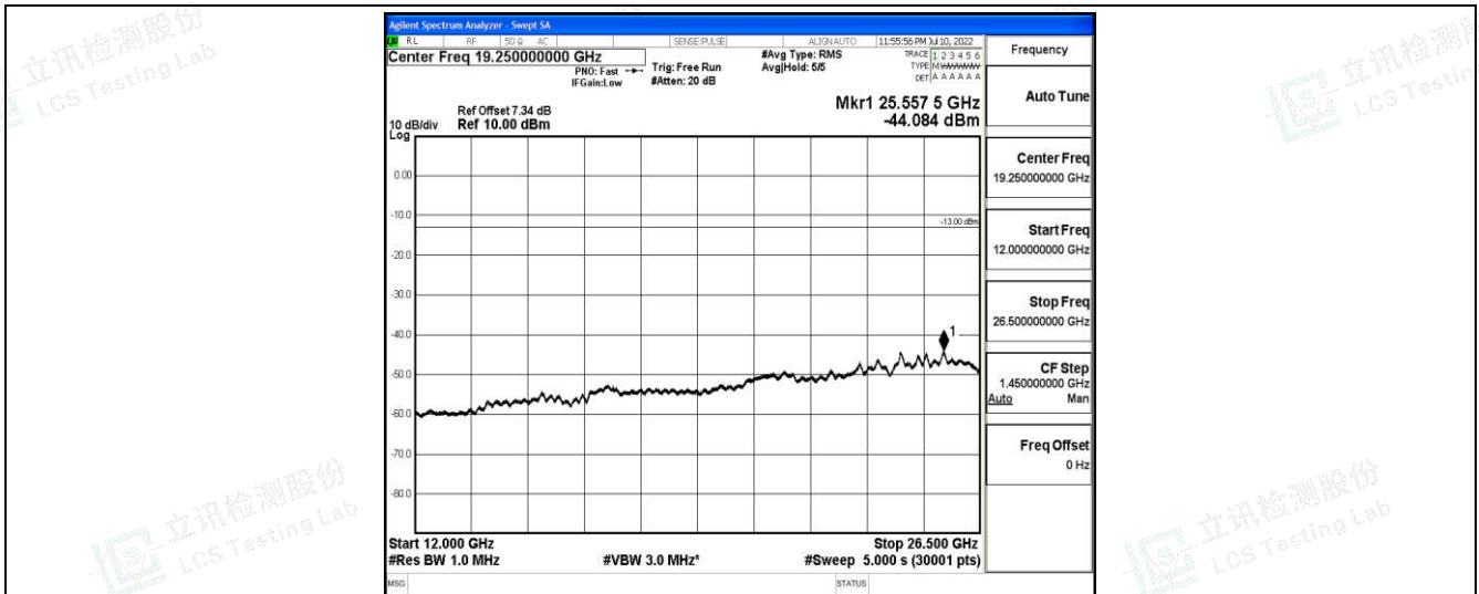
Band26-3MHz-QPSK-27025-1-0-High-12000-26500--44.08-PASS
