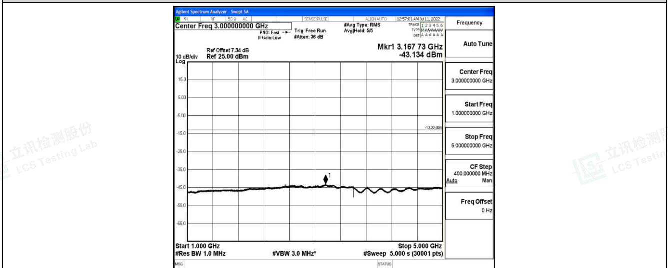
Band26-15MHz-QPSK-26965-1-0-High-1000-5000--43.13-PASS
