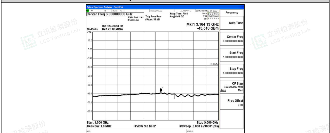
Band26-3MHz-16QAM-26805-1-0-Low-1000-5000--43.51-PASS
