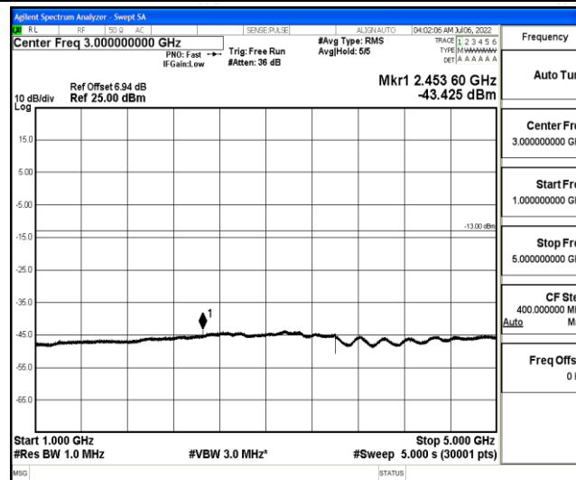
Band26-3MHz-QPSK-26740-1-0-Low-1000-5000--43.43-PASS
