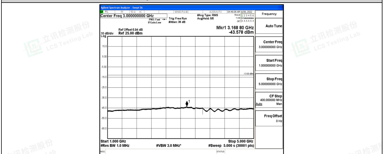
Band26-10MHz-QPSK-26740-1-0-Low-1000-5000--43.58-PASS
