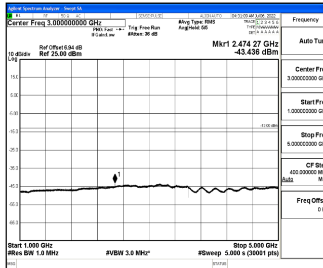
Band26-5MHz-QPSK-26785-1-0-High-1000-5000--43.44-PASS
