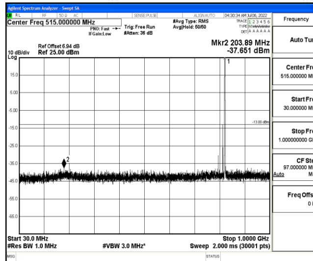
Band26-5MHz-QPSK-26785-1-0-High-30-1000--37.65-PASS
