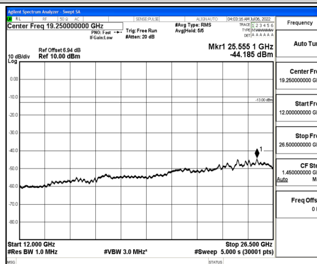
Band26-3MHz-QPSK-26740-1-0-Low-12000-26500--44.19-PASS
