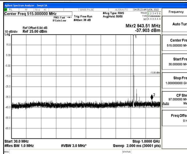
Band26-3MHz-QPSK-26775-1-0-High-30-1000--37.9-PASS
