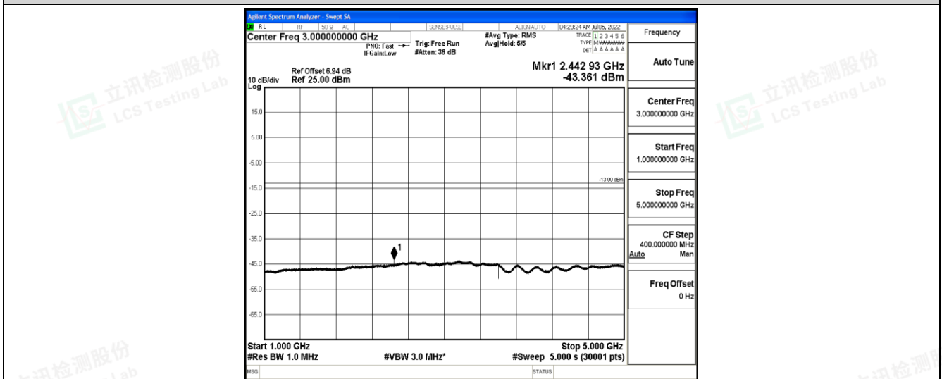
Band26-5MHz-QPSK-26715-1-0-Low-1000-5000--43.36-PASS
