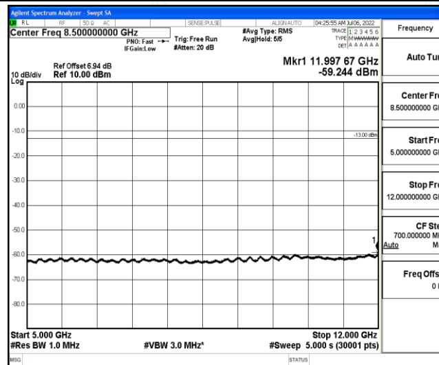
Band26-5MHz-16QAM-26715-1-0-Low-5000-12000--59.24-PASS
