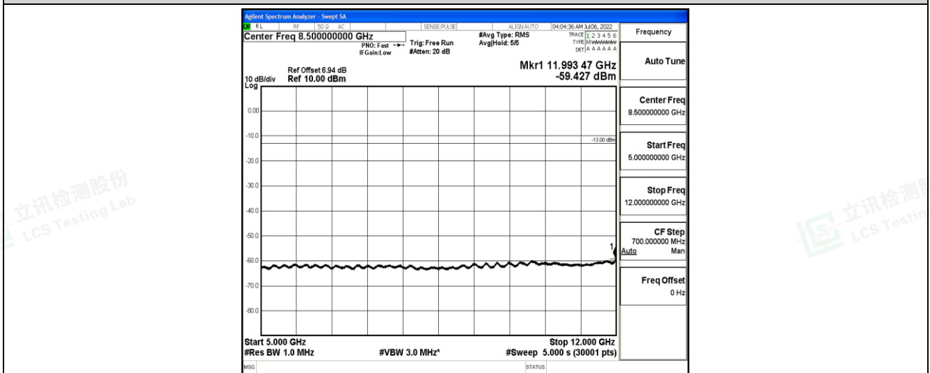
Band26-3MHz-16QAM-26740-1-0-Low-5000-12000--59.43-PASS
