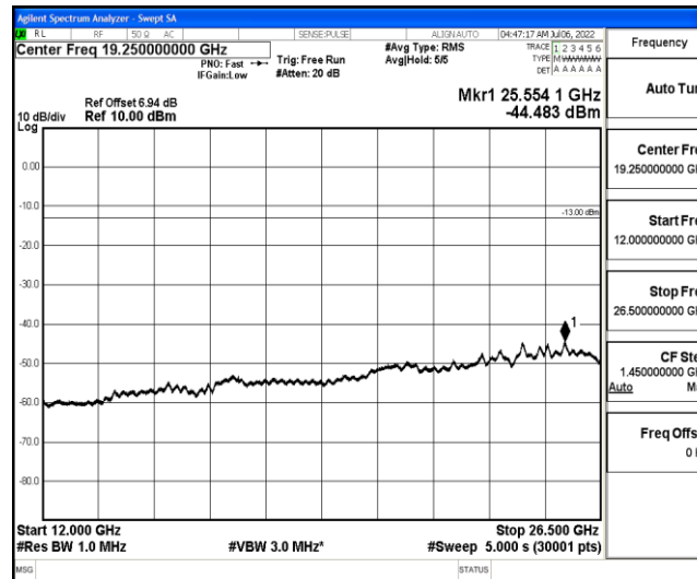
Band26-10MHz-QPSK-26740-1-0-Low-12000-26500--44.48-PASS
