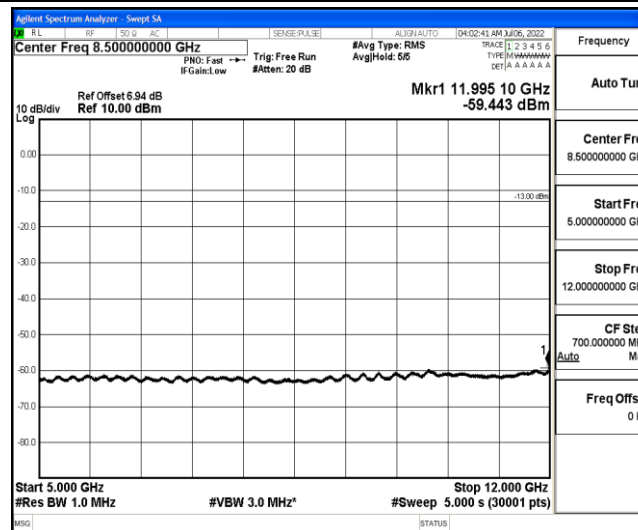
Band26-3MHz-QPSK-26740-1-0-Low-5000-12000--59.44-PASS
