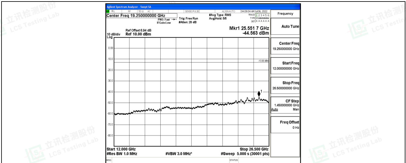
Band26-3MHz-16QAM-26775-1-0-High-12000-26500--44.56-PASS
