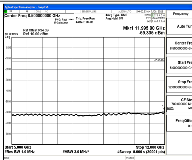
Band26-3MHz-QPSK-26775-1-0-High-5000-12000--59.31-PASS
