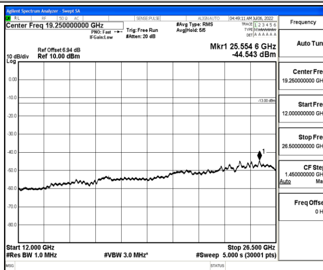
Band26-10MHz-16QAM-26740-1-0-Low-12000-26500--44.54-PASS
