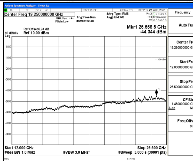
Band26-5MHz-QPSK-26785-1-0-High-12000-26500--44.34-PASS
