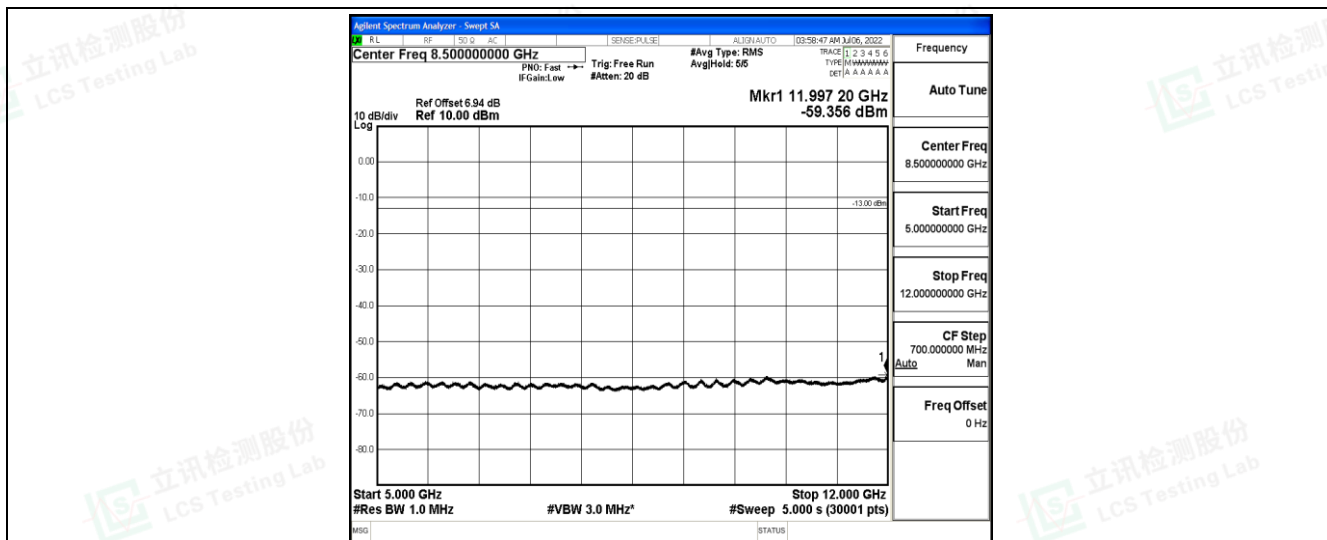
Band26-3MHz-QPSK-26705-1-0-Low-5000-12000--59.36-PASS
