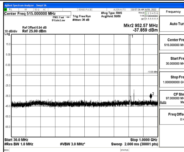
Band26-3MHz-QPSK-26705-1-0-Low-30-1000--37.86-PASS
