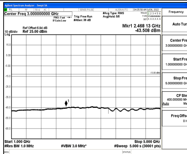
Band26-3MHz-QPSK-26775-1-0-High-1000-5000--43.51-PASS
