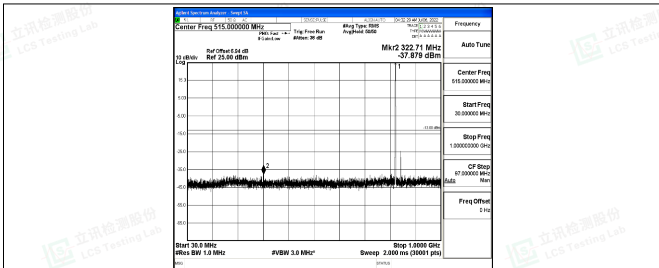
Band26-5MHz-16QAM-26785-1-0-High-30-1000--37.88-PASS
