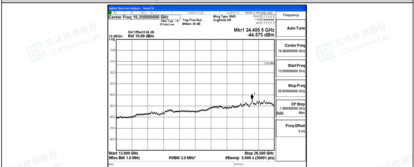
Band26-3MHz-16QAM-26740-1-0-Low-12000-26500--44.57-PASS
