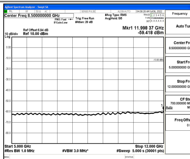
Band26-3MHz-16QAM-26775-1-0-High-5000-12000--59.42-PASS
