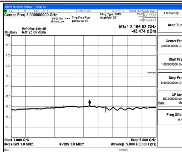
Band26-3MHz-QPSK-26705-1-0-Low-1000-5000--43.47-PASS
