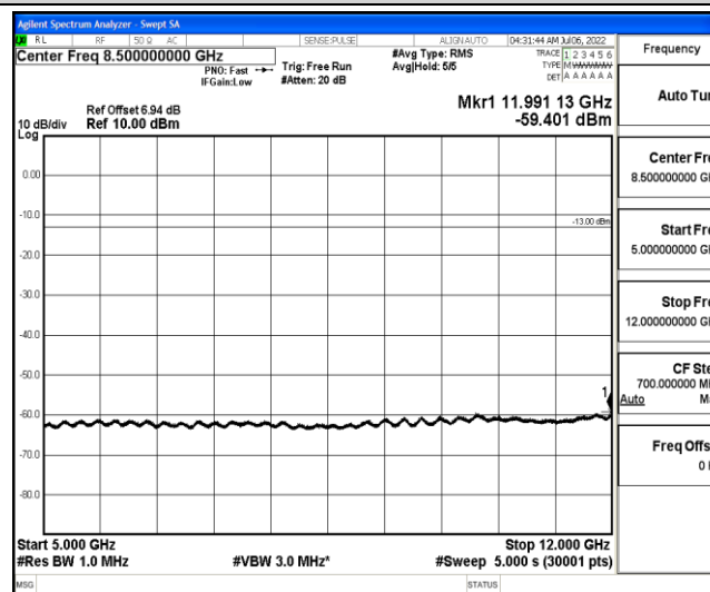
Band26-5MHz-QPSK-26785-1-0-High-5000-12000--59.4-PASS
