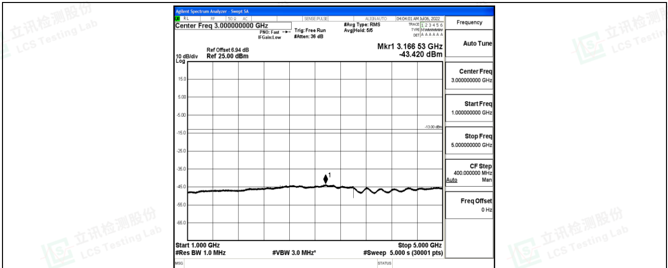
Band26-3MHz-16QAM-26740-1-0-Low-1000-5000--43.42-PASS
