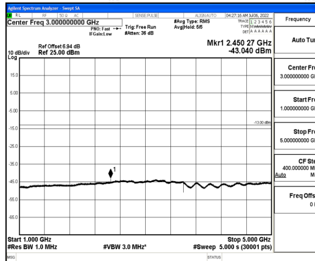
Band26-5MHz-QPSK-26740-1-0-Low-1000-5000--43.04-PASS
