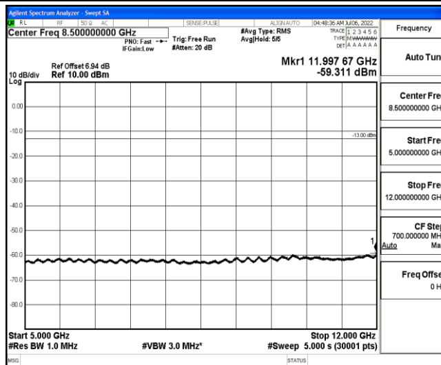
Band26-10MHz-16QAM-26740-1-0-Low-5000-12000--59.31-PASS
