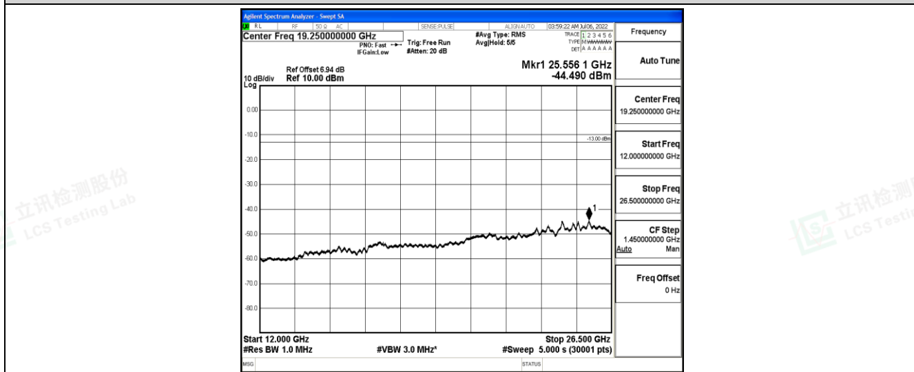
Band26-3MHz-QPSK-26705-1-0-Low-12000-26500--44.49-PASS
