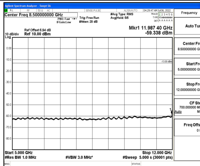
Band26-5MHz-16QAM-26740-1-0-Low-5000-12000--59.34-PASS
