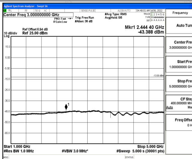
Band26-10MHz-16QAM-26740-1-0-Low-1000-5000--43.39-PASS
