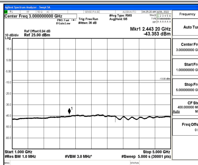
Band26-5MHz-16QAM-26715-1-0-Low-1000-5000--43.35-PASS
