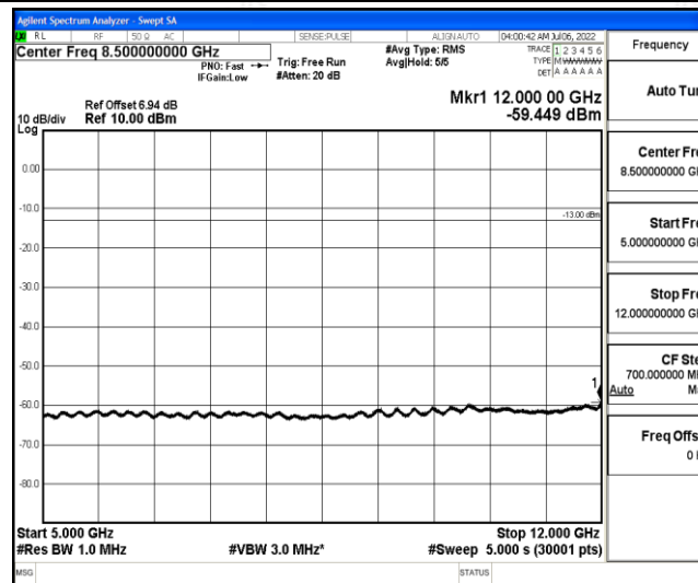
Band26-3MHz-16QAM-26705-1-0-Low-5000-12000--59.45-PASS
