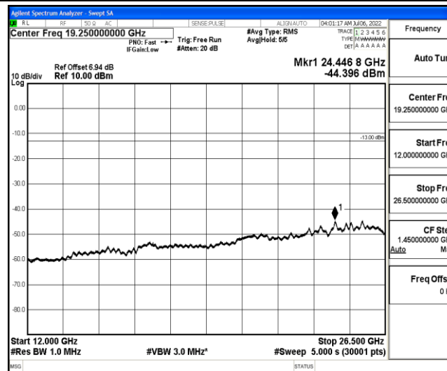
Band26-3MHz-16QAM-26705-1-0-Low-12000-26500--44.4-PASS
