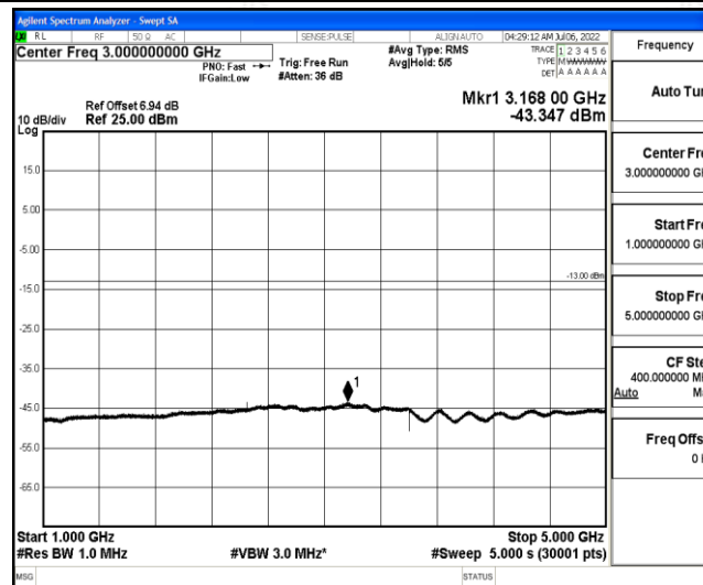
Band26-5MHz-16QAM-26740-1-0-Low-1000-5000--43.35-PASS
