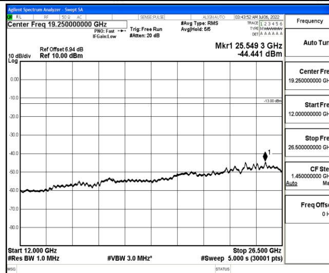
Band26-1.4MHz-16QAM-26783-1-0-High-12000-26500--44.44-PASS
