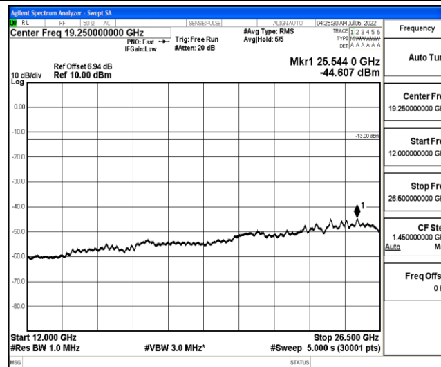
Band26-5MHz-16QAM-26715-1-0-Low-12000-26500--44.61-PASS
