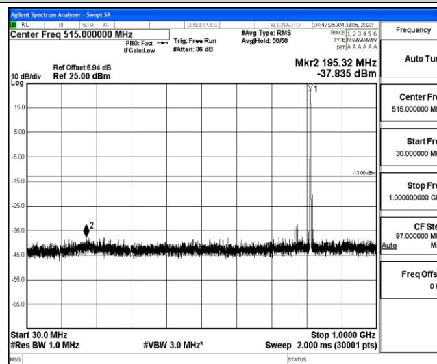
Band26-10MHz-16QAM-26740-1-0-Low-30-1000--37.84-PASS
