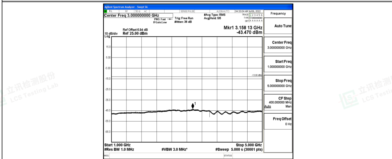
Band26-5MHz-16QAM-26785-1-0-High-1000-5000--43.47-PASS
