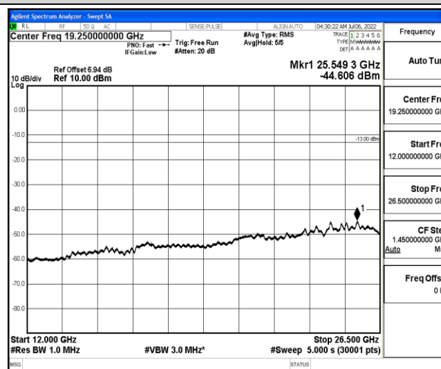
Band26-5MHz-16QAM-26740-1-0-Low-12000-26500--44.61-PASS
