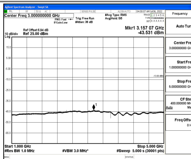
Band26-3MHz-16QAM-26705-1-0-Low-1000-5000--43.53-PASS
