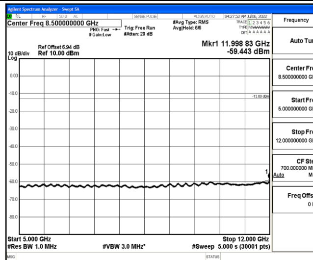
Band26-5MHz-QPSK-26740-1-0-Low-5000-12000--59.44-PASS
