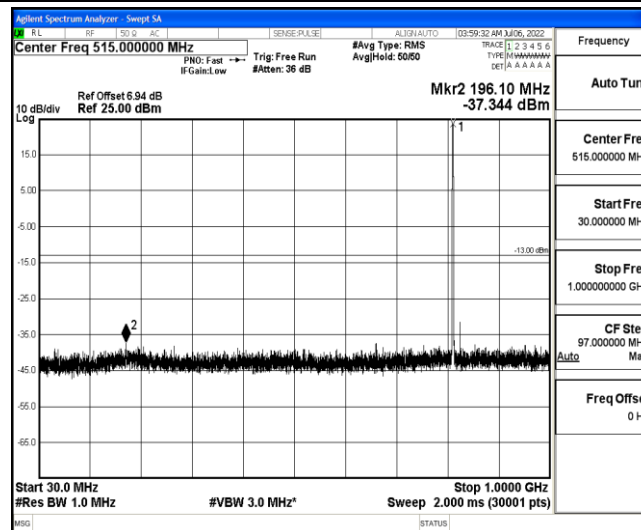
Band26-3MHz-16QAM-26705-1-0-Low-30-1000--37.34-PASS
