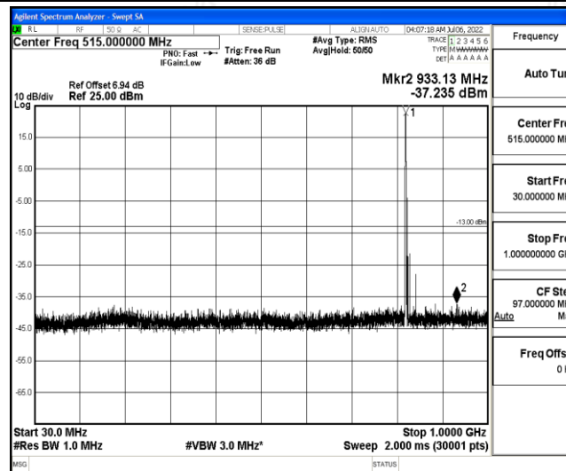
Band26-3MHz-16QAM-26775-1-0-High-30-1000--37.24-PASS
