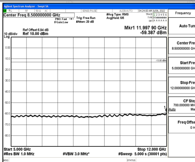
Band26-5MHz-QPSK-26715-1-0-Low-5000-12000--59.39-PASS
