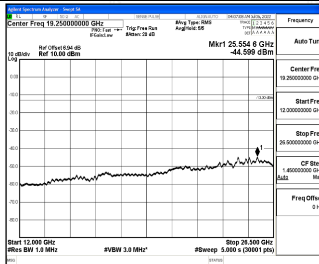
Band26-3MHz-QPSK-26775-1-0-High-12000-26500--44.6-PASS
