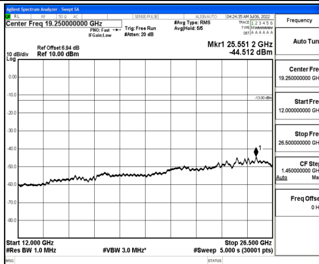
Band26-5MHz-QPSK-26715-1-0-Low-12000-26500--44.51-PASS
