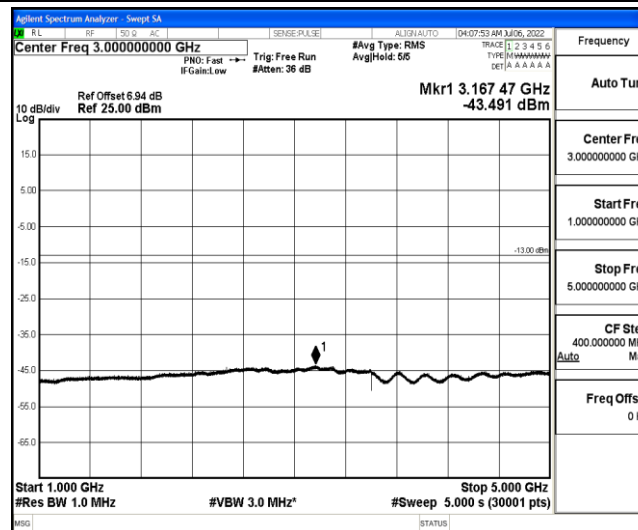
Band26-3MHz-16QAM-26775-1-0-High-1000-5000--43.49-PASS
