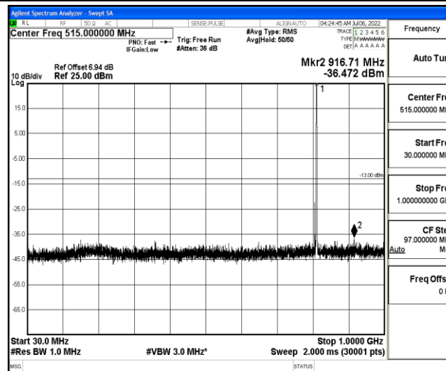
Band26-5MHz-16QAM-26715-1-0-Low-30-1000--36.47-PASS
