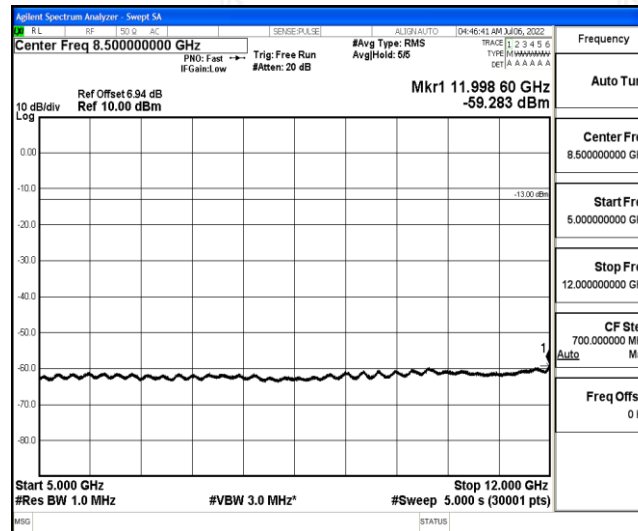
Band26-10MHz-QPSK-26740-1-0-Low-5000-12000--59.28-PASS
