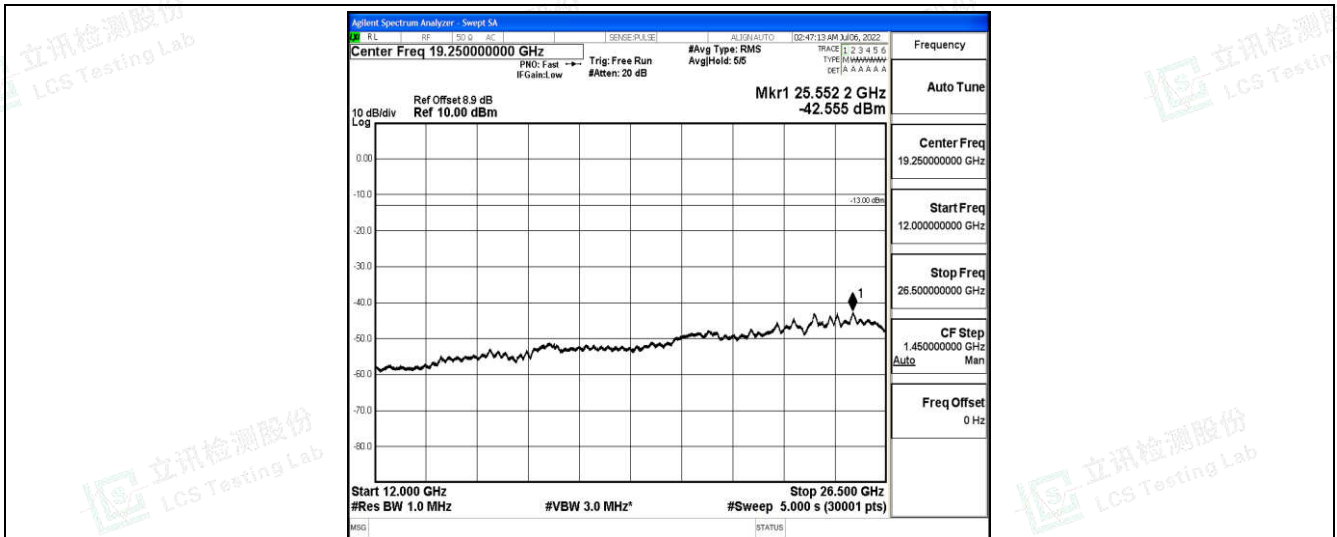
Band25-15MHz-QPSK-26615-1-0-High-12000-26500--42.56-PASS
