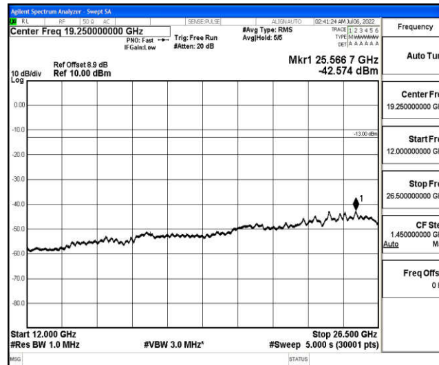
Band25-15MHz-16QAM-26115-1-0-Low-12000-26500--42.57-PASS
