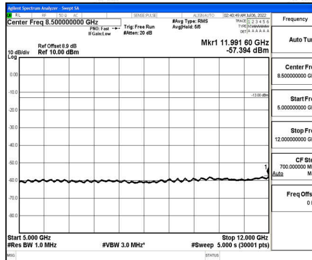
Band25-15MHz-16QAM-26115-1-0-Low-5000-12000--57.39-PASS
