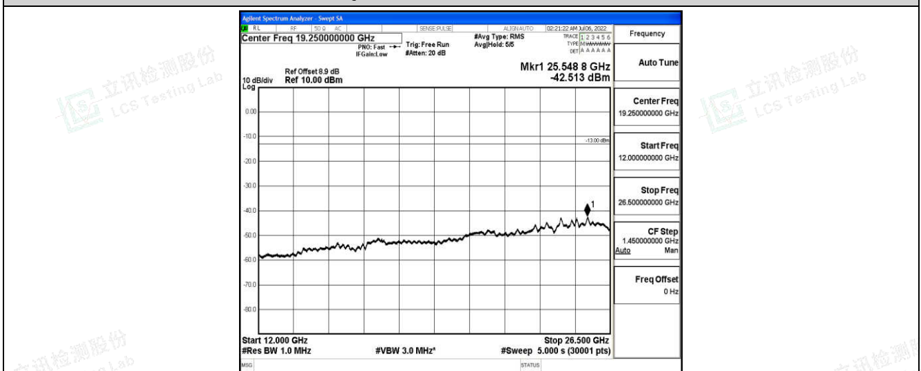
Band25-10MHz-16QAM-26365-1-0-Low-12000-26500--42.51-PASS
