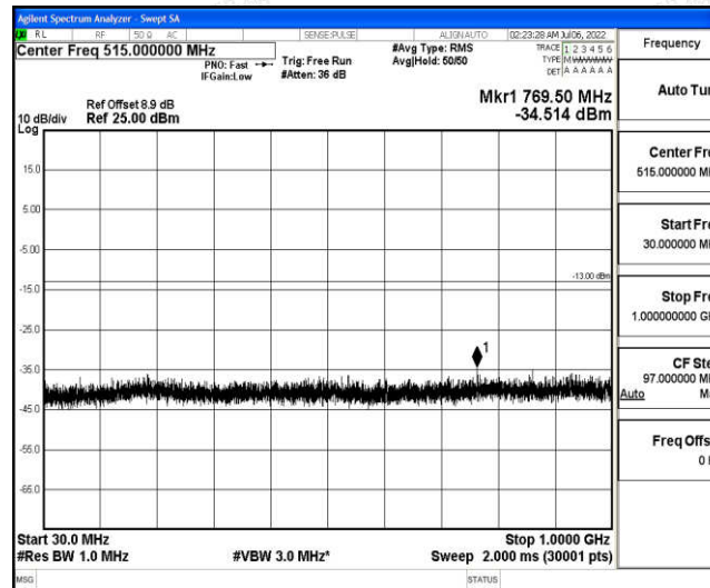
Band25-10MHz-16QAM-26640-1-0-High-30-1000--34.51-PASS
