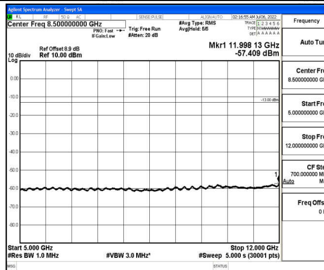
Band25-10MHz-16QAM-26090-1-0-Low-5000-12000--57.41-PASS
