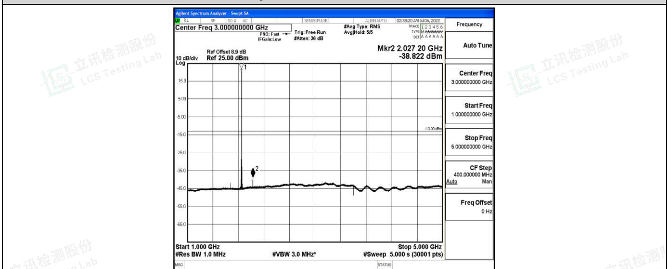
Band25-15MHz-QPSK-26115-1-0-Low-1000-5000--38.82-PASS
