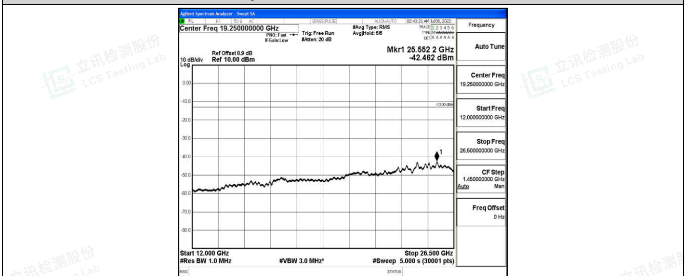
Band25-15MHz-QPSK-26365-1-0-Low-12000-26500--42.46-PASS
