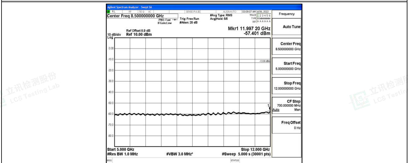
Band25-20MHz-16QAM-26365-1-0-Low-5000-12000--57.4-PASS
