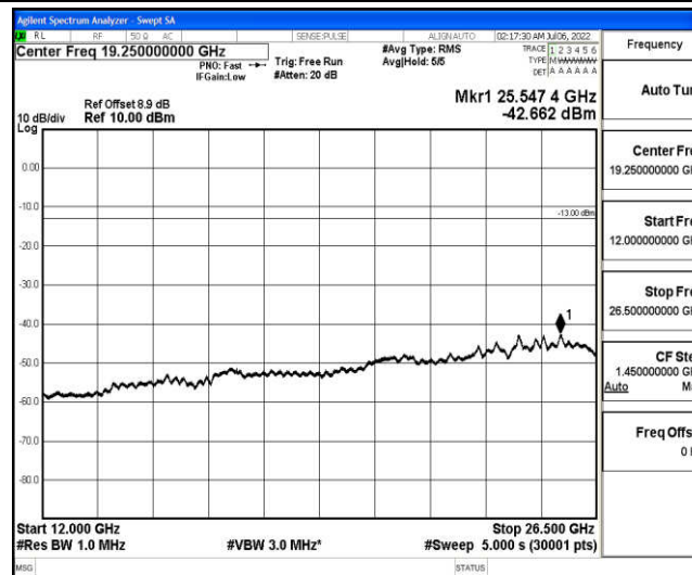
Band25-10MHz-16QAM-26090-1-0-Low-12000-26500--42.66-PASS
