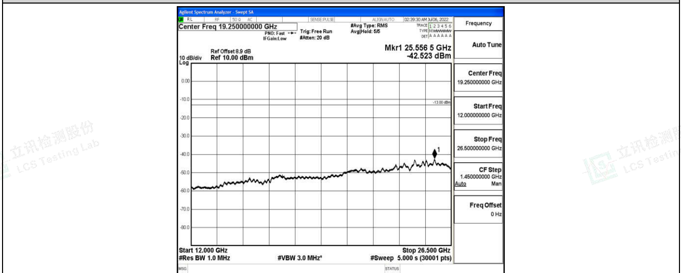
Band25-15MHz-QPSK-26115-1-0-Low-12000-26500--42.52-PASS
