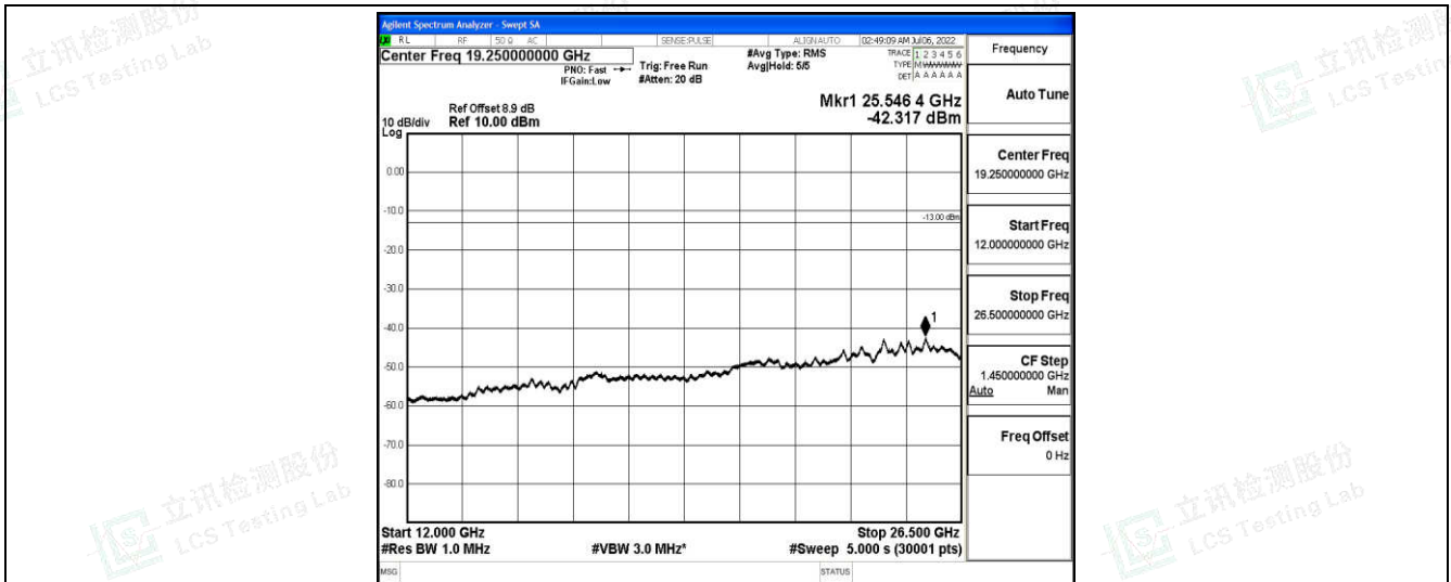
Band25-15MHz-16QAM-26615-1-0-High-12000-26500--42.32-PASS
