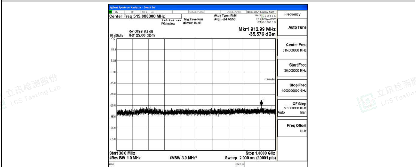
Band25-15MHz-16QAM-26115-1-0-Low-30-1000--35.58-PASS
