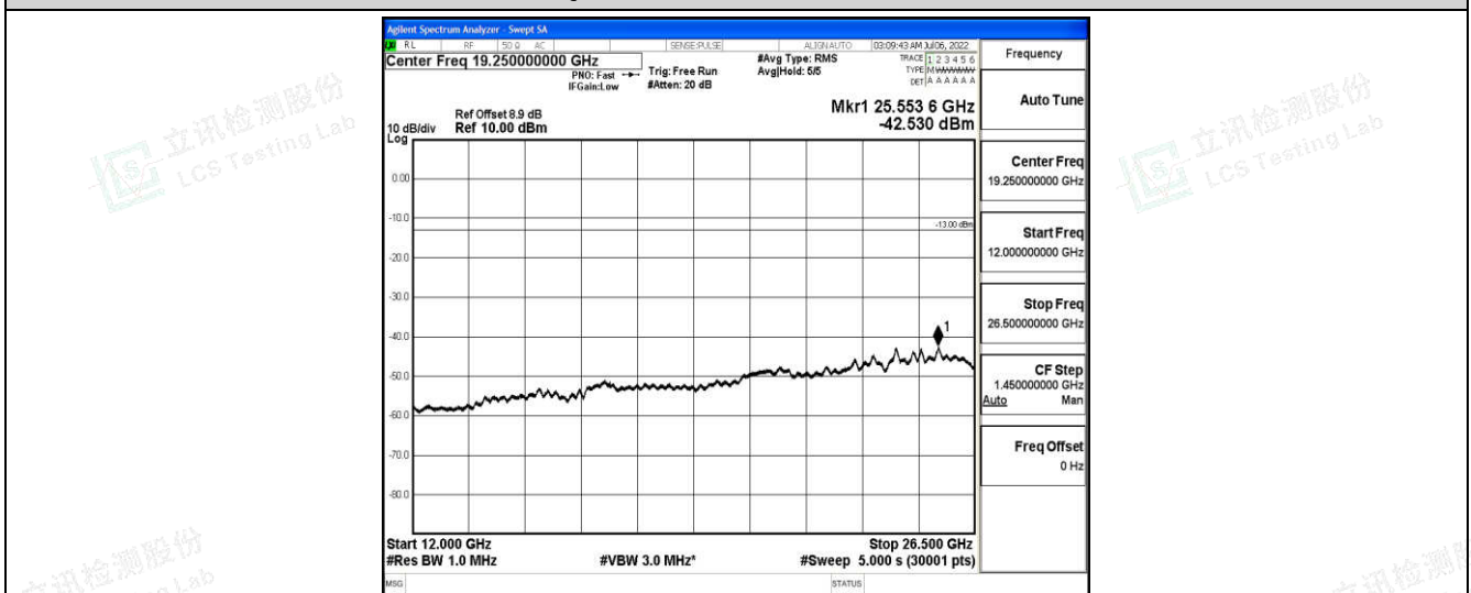
Band25-20MHz-16QAM-26365-1-0-Low-12000-26500--42.53-PASS
