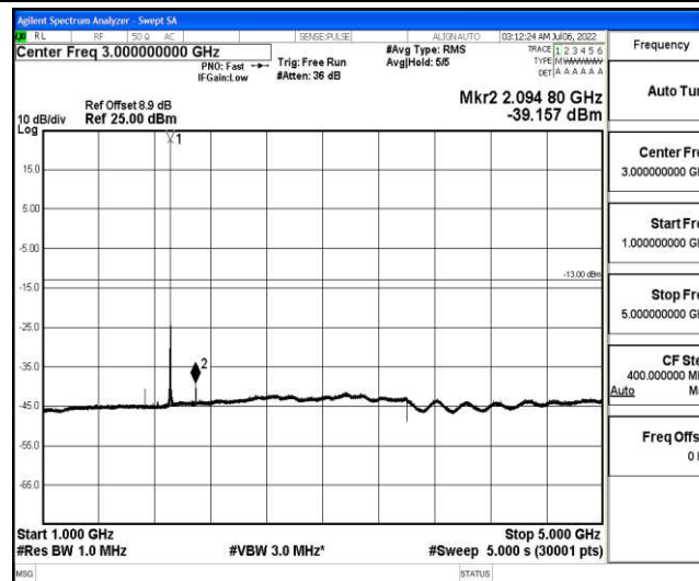
Band25-20MHz-16QAM-26590-1-0-High-1000-5000--39.16-PASS
