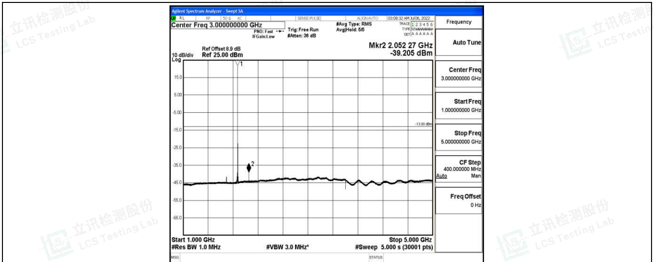
Band25-20MHz-16QAM-26365-1-0-Low-1000-5000--39.21-PASS
