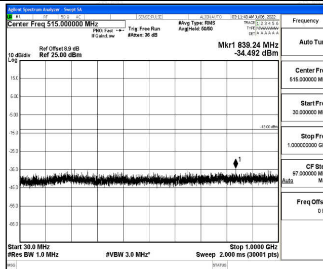
Band25-20MHz-16QAM-26590-1-0-High-30-1000--34.49-PASS
