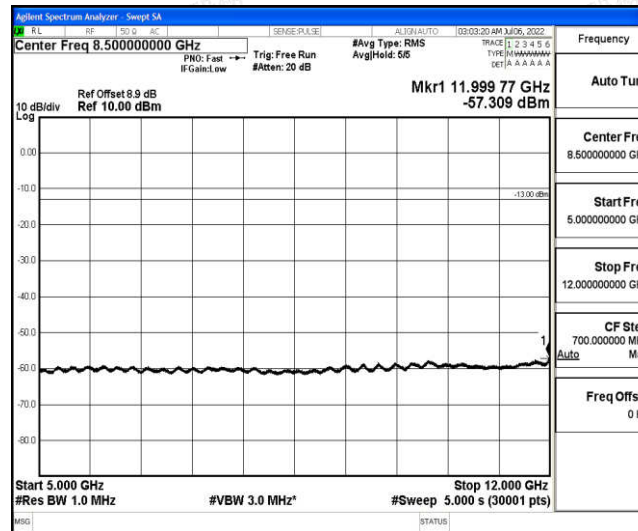
Band25-20MHz-QPSK-26140-1-0-Low-5000-12000--57.31-PASS
