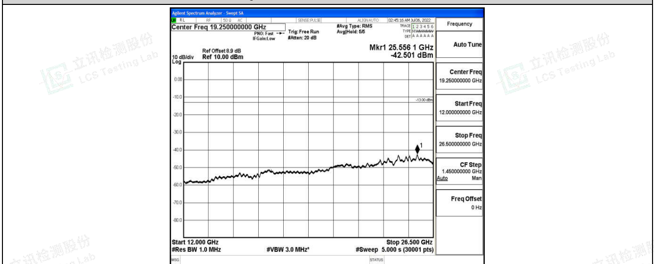
Band25-15MHz-16QAM-26365-1-0-Low-12000-26500--42.5-PASS
