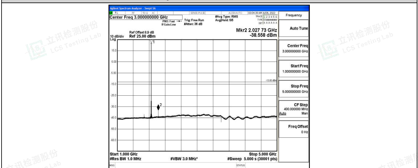
Band25-20MHz-16QAM-26140-1-0-Low-1000-5000--38.56-PASS
