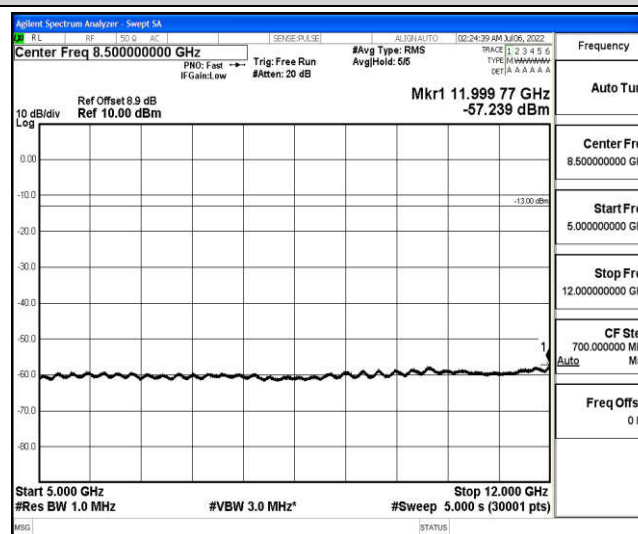
Band25-10MHz-16QAM-26640-1-0-High-5000-12000--57.24-PASS
