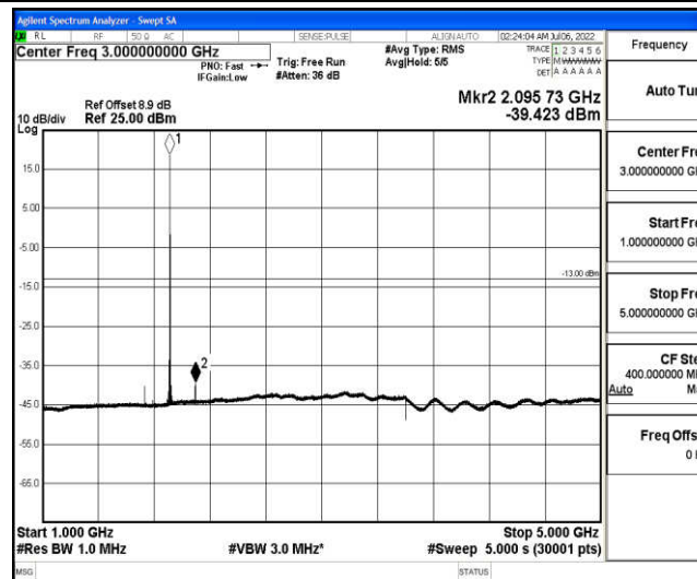
Band25-10MHz-16QAM-26640-1-0-High-1000-5000--39.42-PASS
