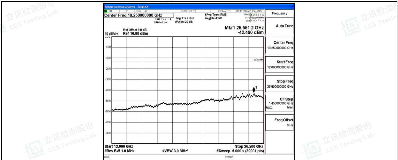
Band25-20MHz-QPSK-26590-1-0-High-12000-26500--42.49-PASS
