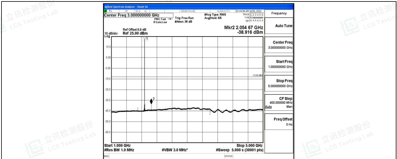
Band25-15MHz-16QAM-26365-1-0-Low-1000-5000--38.92-PASS
