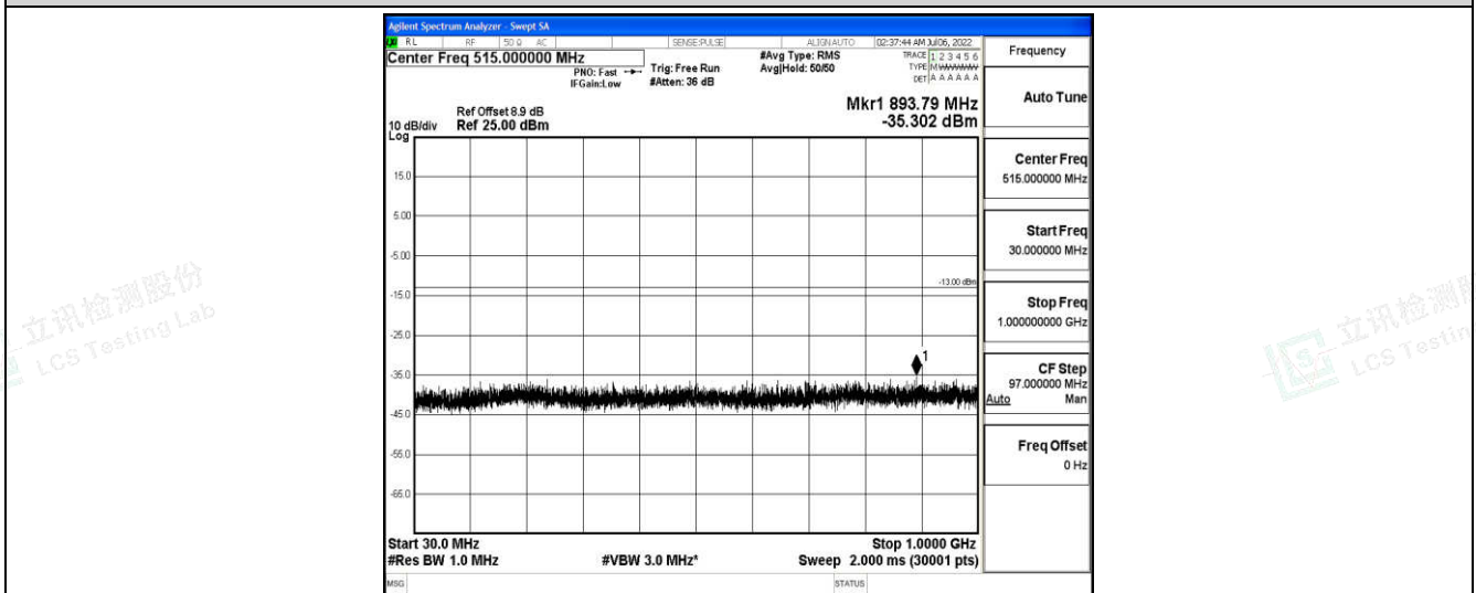
Band25-15MHz-QPSK-26115-1-0-Low-30-1000--35.3-PASS
