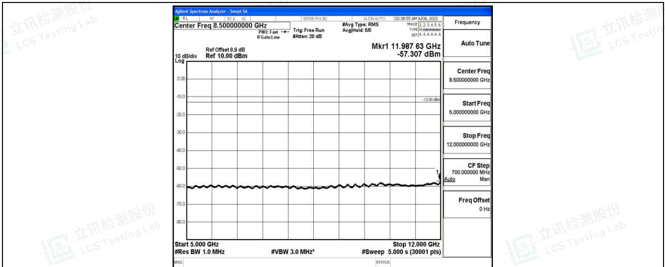
Band25-15MHz-QPSK-26115-1-0-Low-5000-12000--57.31-PASS
