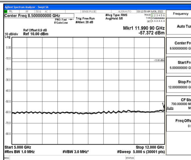
Band25-20MHz-16QAM-26590-1-0-High-5000-12000--57.37-PASS
