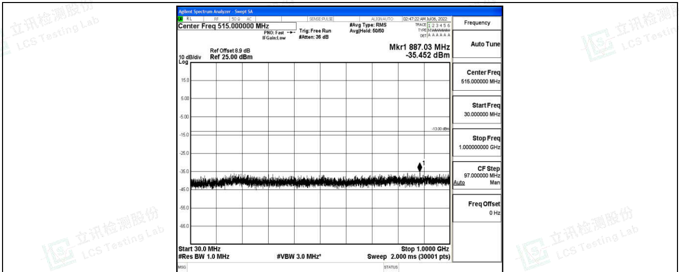
Band25-15MHz-16QAM-26615-1-0-High-30-1000--35.45-PASS
