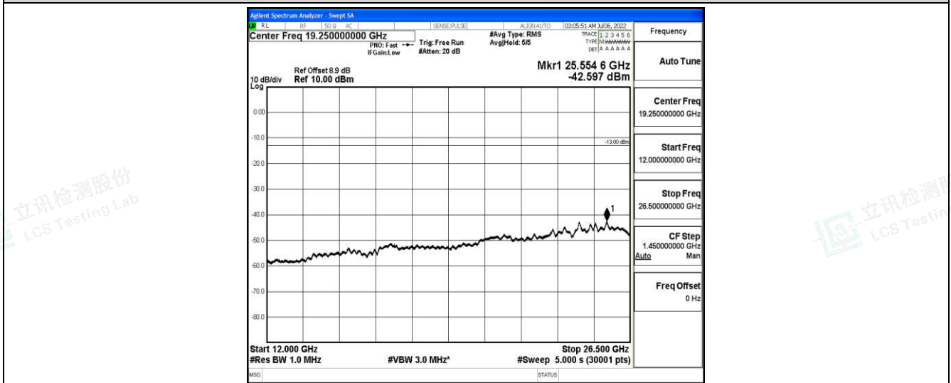
Band25-20MHz-16QAM-26140-1-0-Low-12000-26500--42.6-PASS
