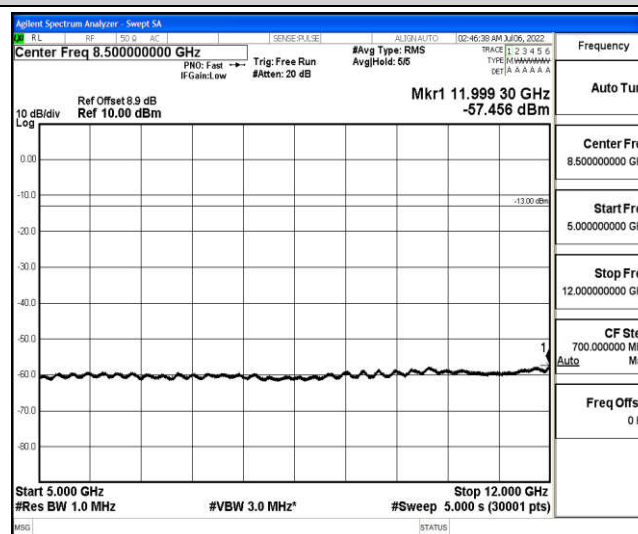
Band25-15MHz-QPSK-26615-1-0-High-5000-12000--57.46-PASS
