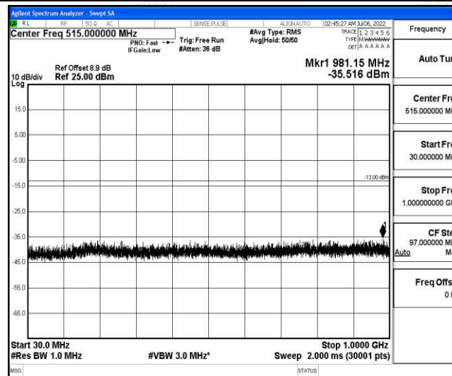
Band25-15MHz-QPSK-26615-1-0-High-30-1000--35.52-PASS
