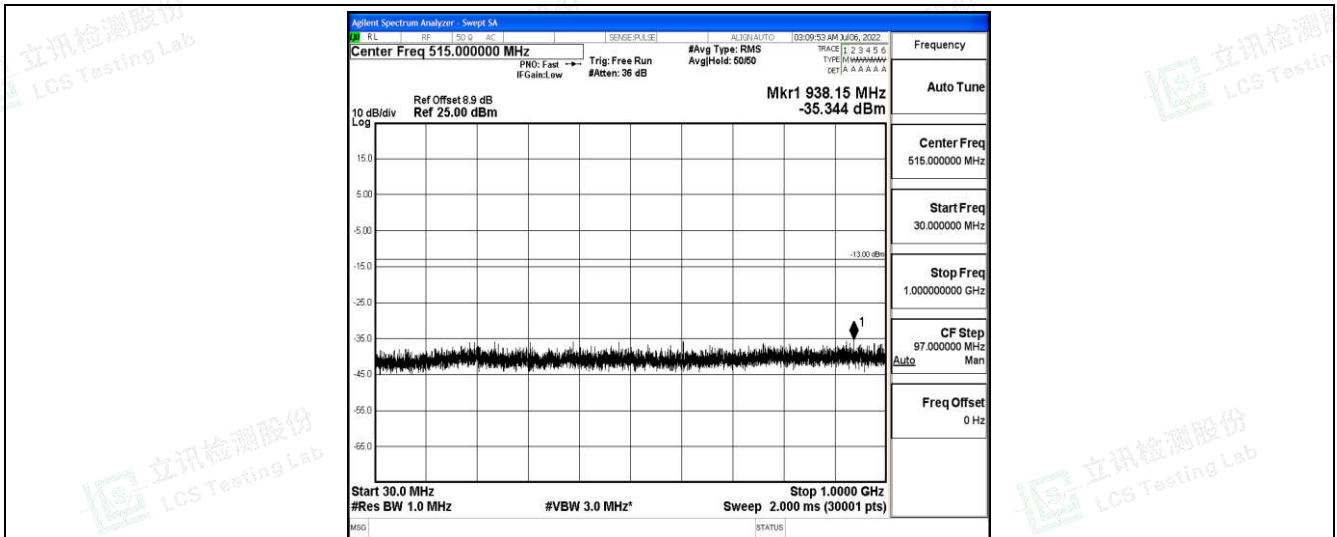
Band25-20MHz-QPSK-26590-1-0-High-30-1000--35.34-PASS
