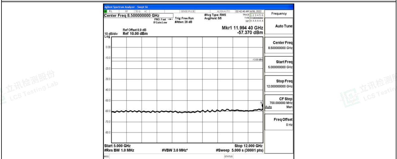
Band25-15MHz-QPSK-26365-1-0-Low-5000-12000--57.37-PASS
