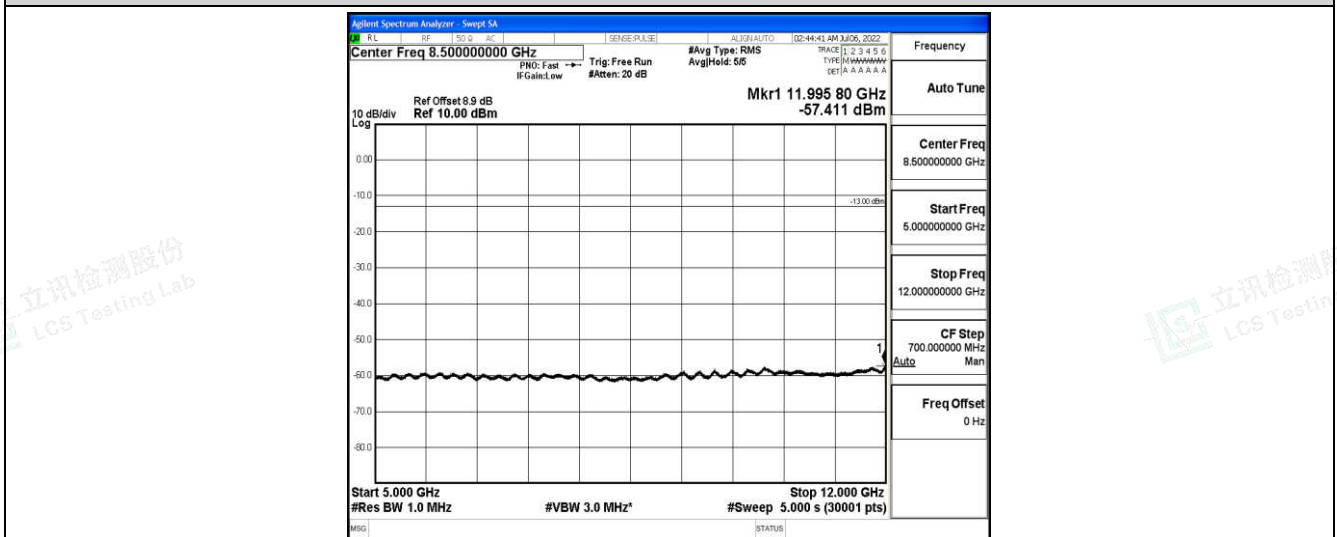
Band25-15MHz-16QAM-26365-1-0-Low-5000-12000--57.41-PASS
