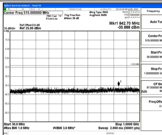
Band25-15MHz-16QAM-26365-1-0-Low-30-1000--35.89-PASS
