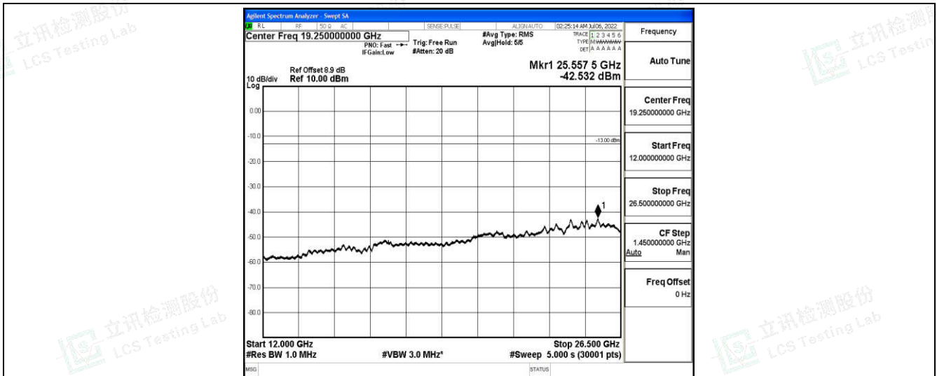
Band25-10MHz-16QAM-26640-1-0-High-12000-26500--42.53-PASS
