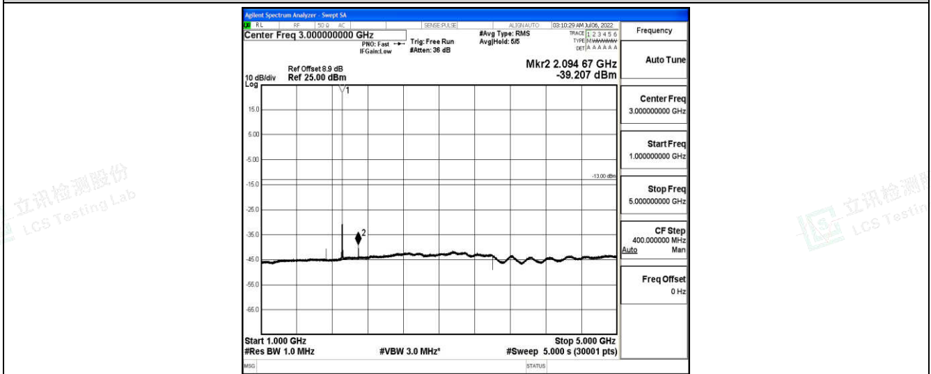
Band25-20MHz-QPSK-26590-1-0-High-1000-5000--39.21-PASS
