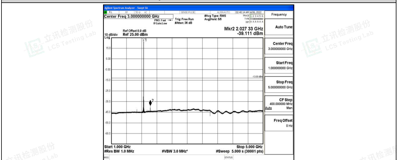
Band25-15MHz-16QAM-26115-1-0-Low-1000-5000--39.11-PASS
