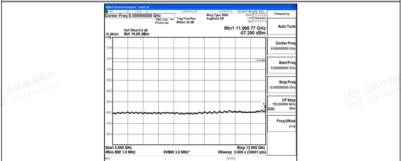
Band25-10MHz-16QAM-26365-1-0-Low-5000-12000--57.29-PASS
