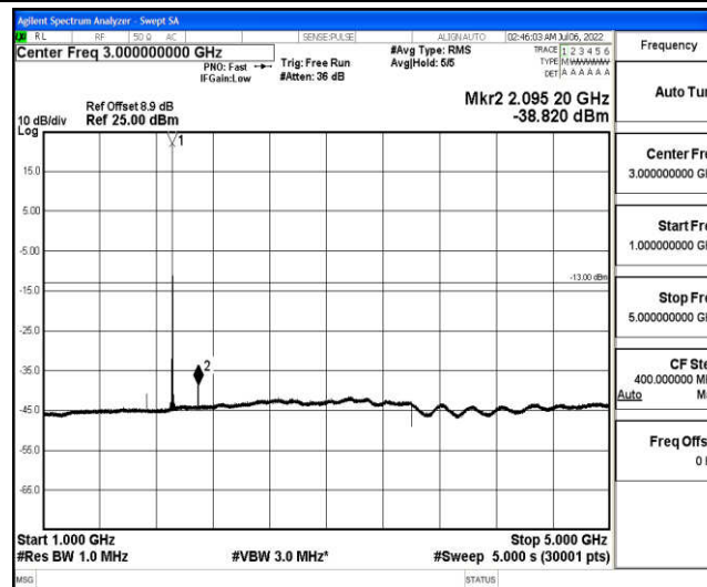
Band25-15MHz-QPSK-26615-1-0-High-1000-5000--38.82-PASS
