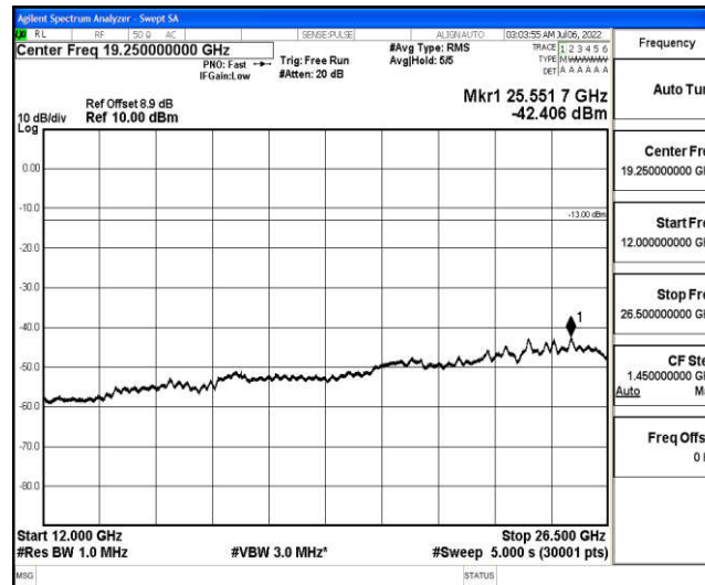
Band25-20MHz-QPSK-26140-1-0-Low-12000-26500--42.41-PASS
