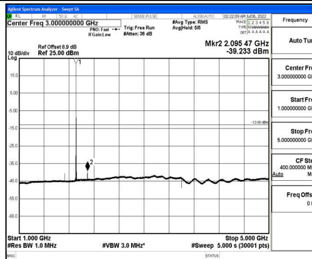
Band25-10MHz-QPSK-26640-1-0-High-1000-5000--39.23-PASS
