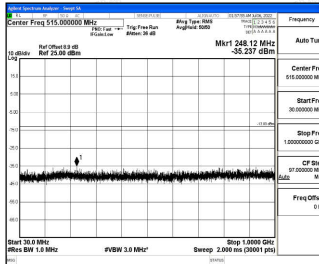
Band25-5MHz-16QAM-26665-1-0-High-30-1000--35.24-PASS
