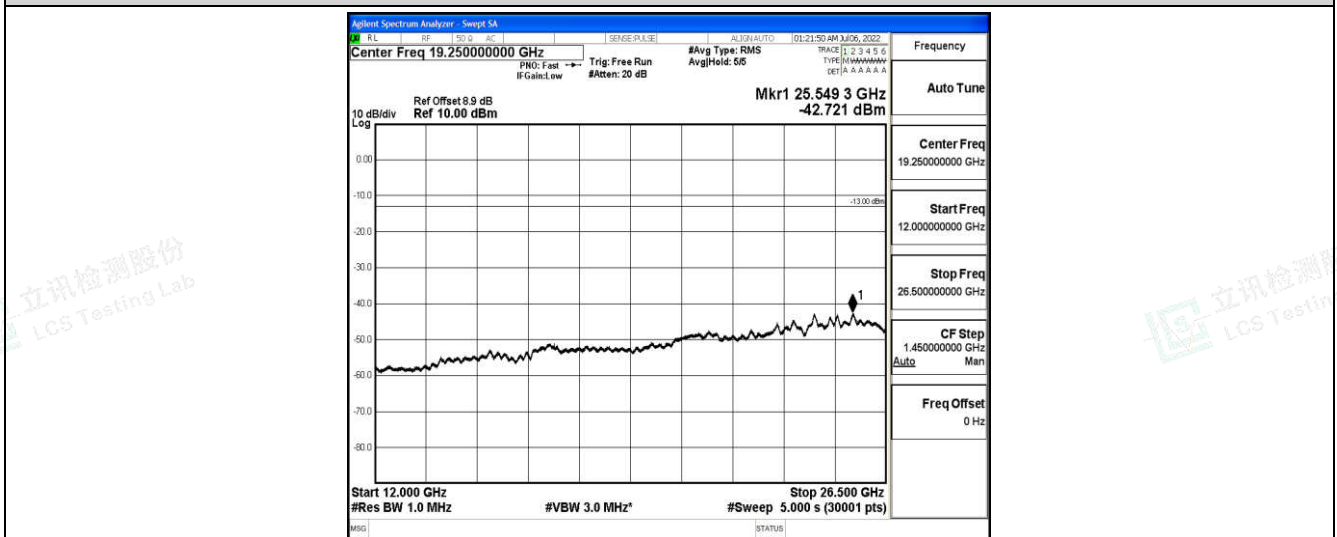
Band25-3MHz-QPSK-26055-1-0-Low-12000-26500--42.72-PASS
