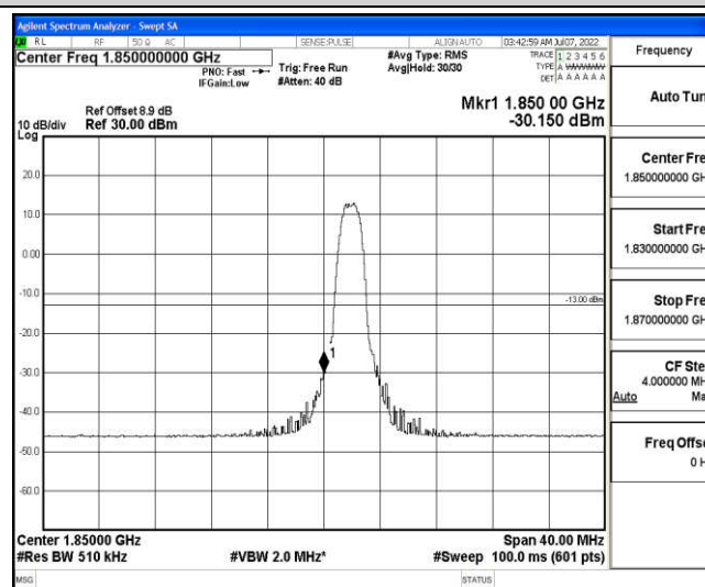
Band25-20MHz-16QAM-26140-6-0-Low--30.15-PASS
