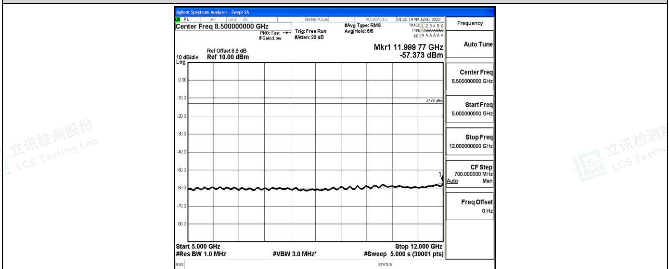
Band25-5MHz-16QAM-26365-1-0-Low-5000-12000--57.37-PASS
