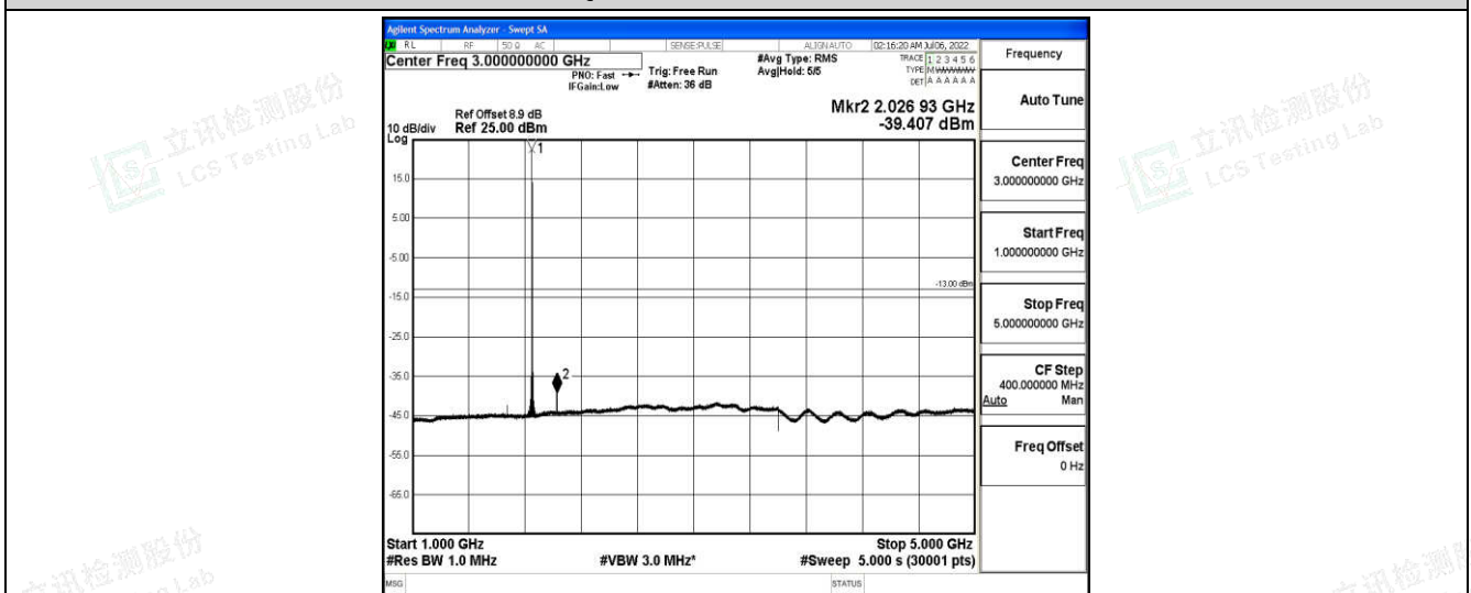
Band25-10MHz-16QAM-26090-1-0-Low-1000-5000--39.41-PASS
