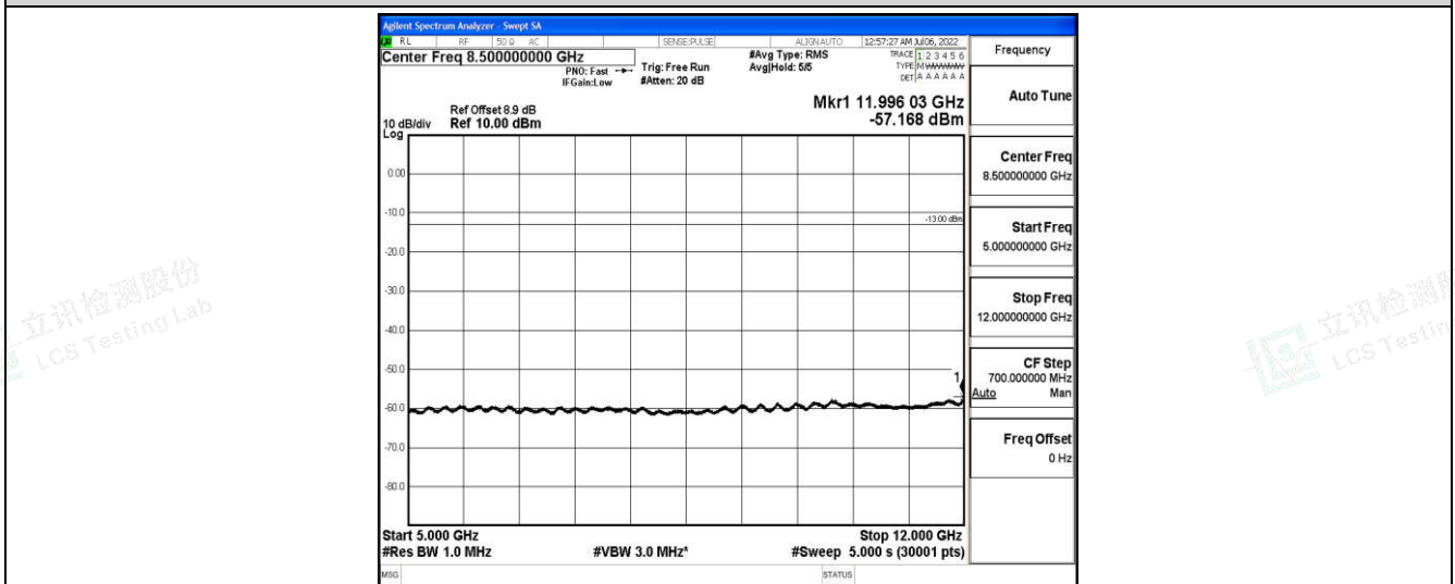
Band25-1.4MHz-16QAM-26365-1-0-Low-5000-12000--57.17-PASS
