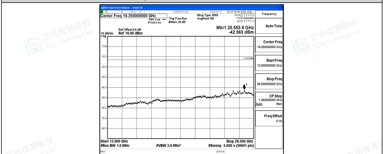
Band25-3MHz-16QAM-26365-1-0-Low-12000-26500--42.36-PASS
