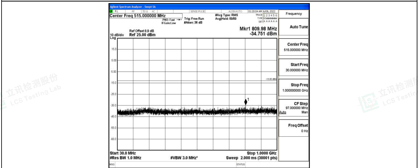
Band25-3MHz-QPSK-26055-1-0-Low-30-1000--34.75-PASS
