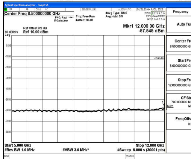
Band25-5MHz-16QAM-26065-1-0-Low-5000-12000--57.55-PASS
