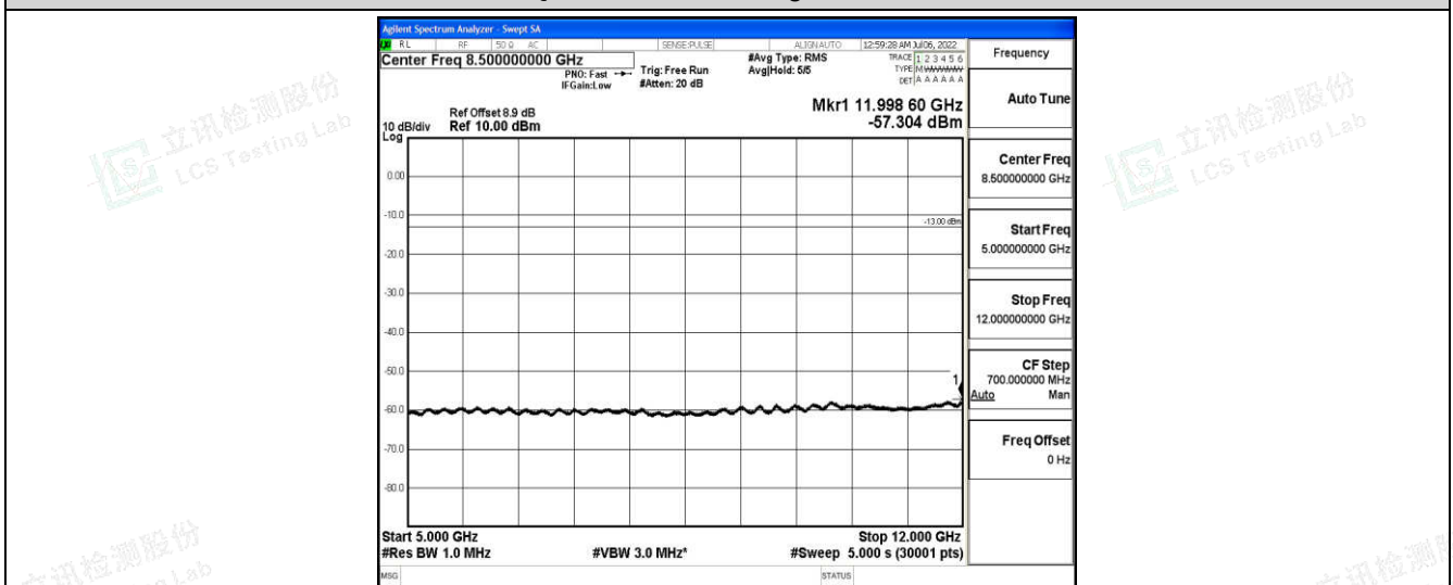
Band25-1.4MHz-QPSK-26683-1-0-High-5000-12000--57.3-PASS
