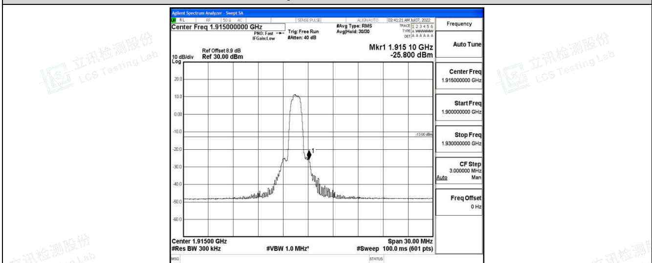
Band25-15MHz-16QAM-26615-6-0-High--25.80-PASS
