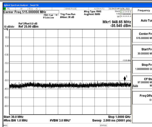
Band25-5MHz-16QAM-26365-1-0-Low-30-1000--35.55-PASS
