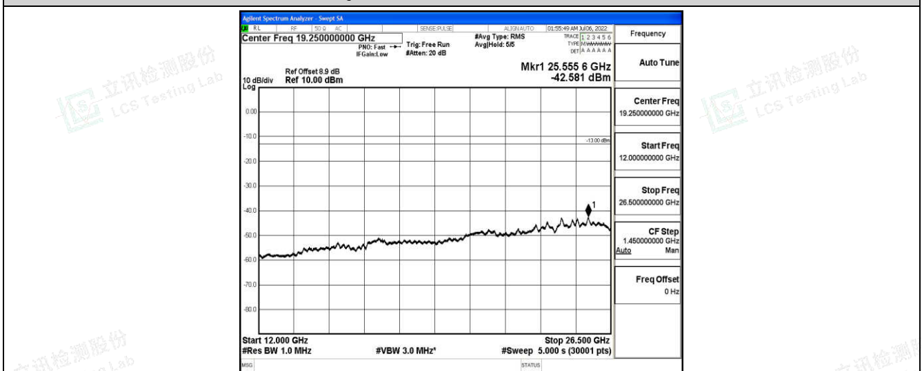
Band25-5MHz-16QAM-26365-1-0-Low-12000-26500--42.58-PASS
