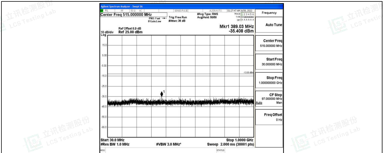
Band25-3MHz-QPSK-26675-1-0-High-30-1000--35.41-PASS
