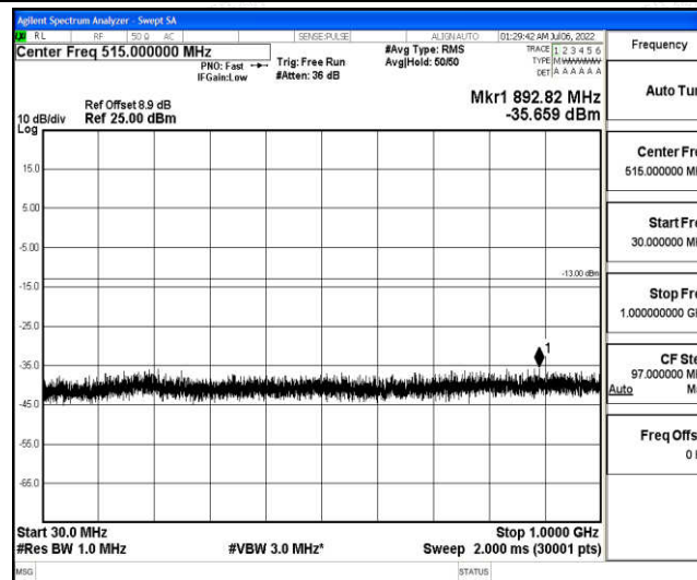
Band25-3MHz-16QAM-26675-1-0-High-30-1000--35.66-PASS
