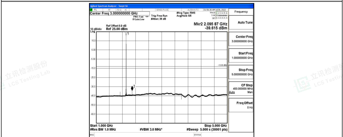
Band25-5MHz-QPSK-26665-1-0-High-1000-5000--39.62-PASS
