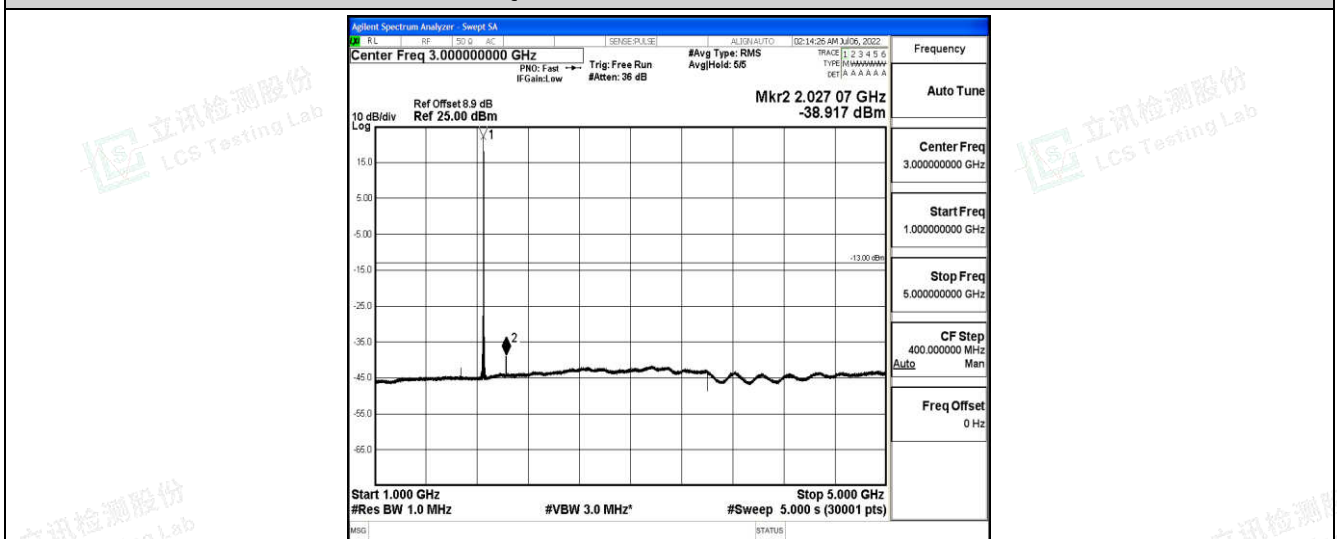
Band25-10MHz-QPSK-26090-1-0-Low-1000-5000--38.92-PASS
