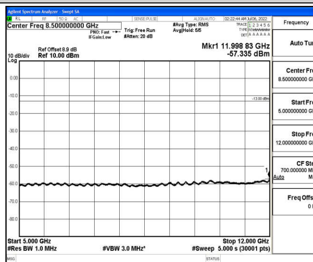
Band25-10MHz-QPSK-26640-1-0-High-5000-12000--57.34-PASS
