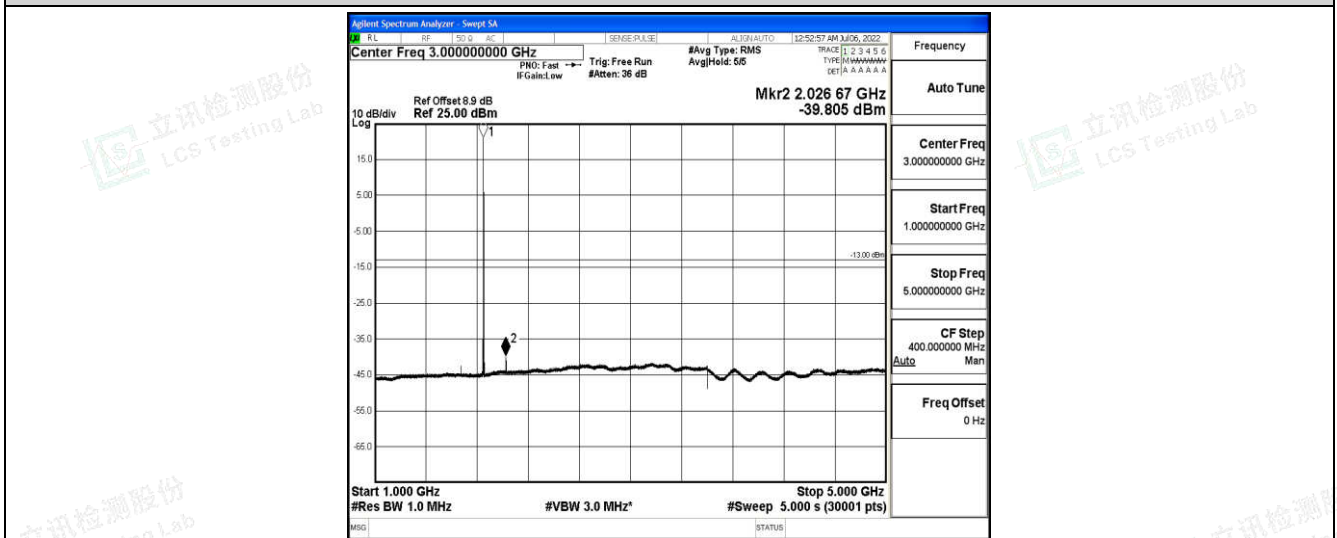
Band25-1.4MHz-16QAM-26047-1-0-Low-1000-5000--39.81-PASS
