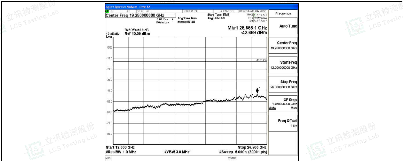
Band25-3MHz-QPSK-26675-1-0-High-12000-26500--42.67-PASS
