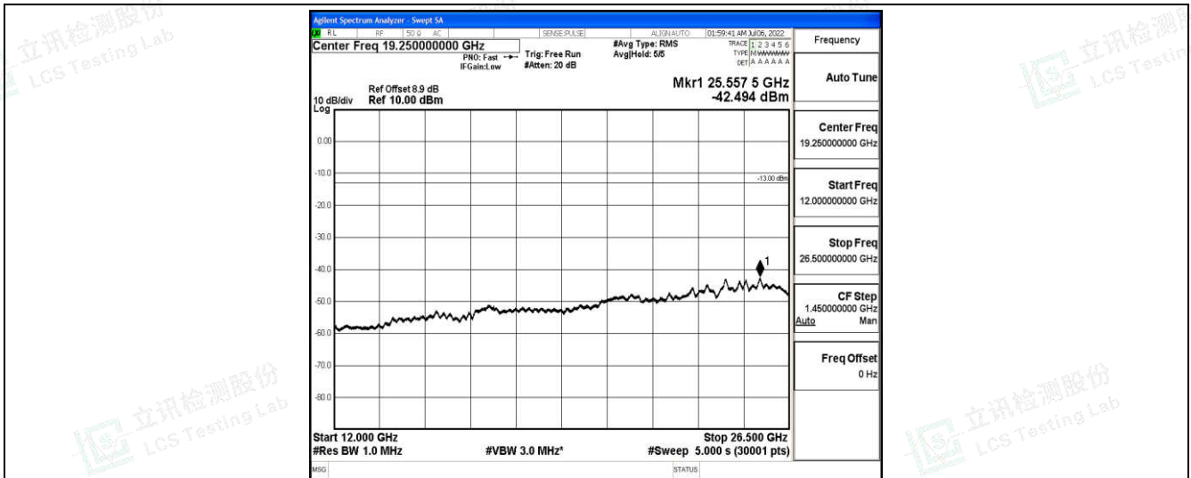
Band25-5MHz-16QAM-26665-1-0-High-12000-26500--42.49-PASS
