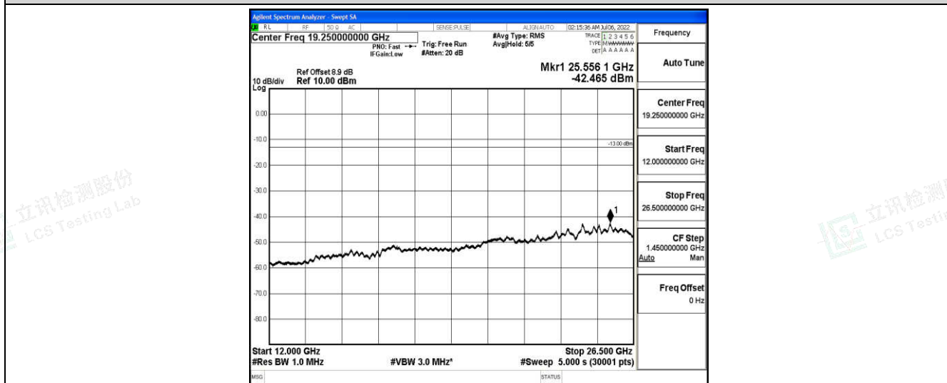
Band25-10MHz-QPSK-26090-1-0-Low-12000-26500--42.47-PASS
