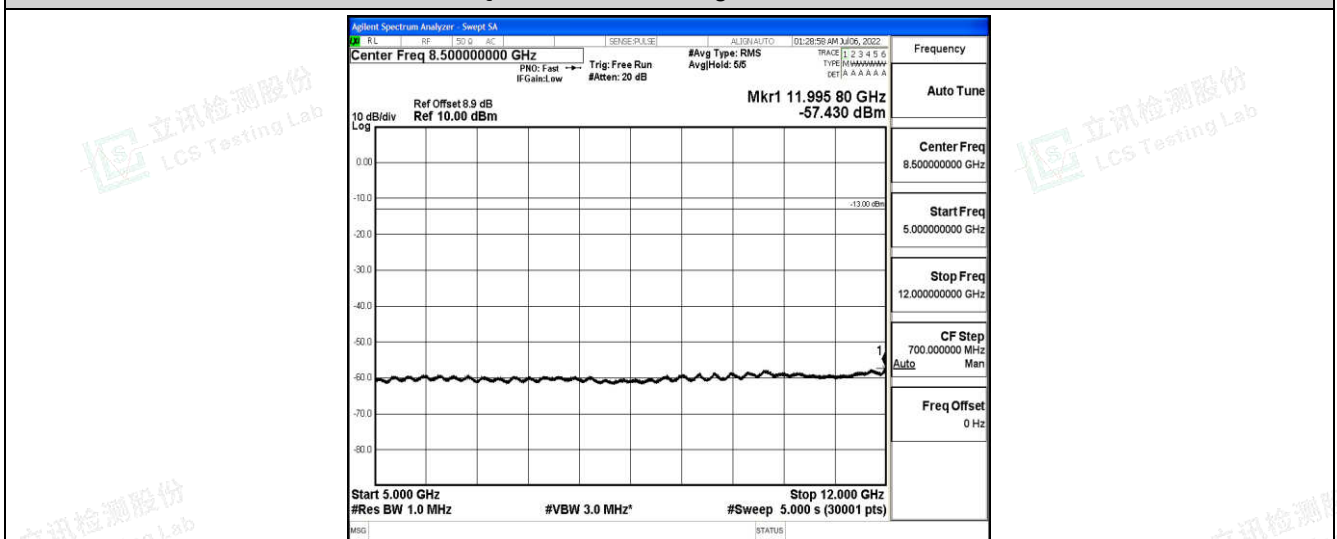
Band25-3MHz-QPSK-26675-1-0-High-5000-12000--57.43-PASS
