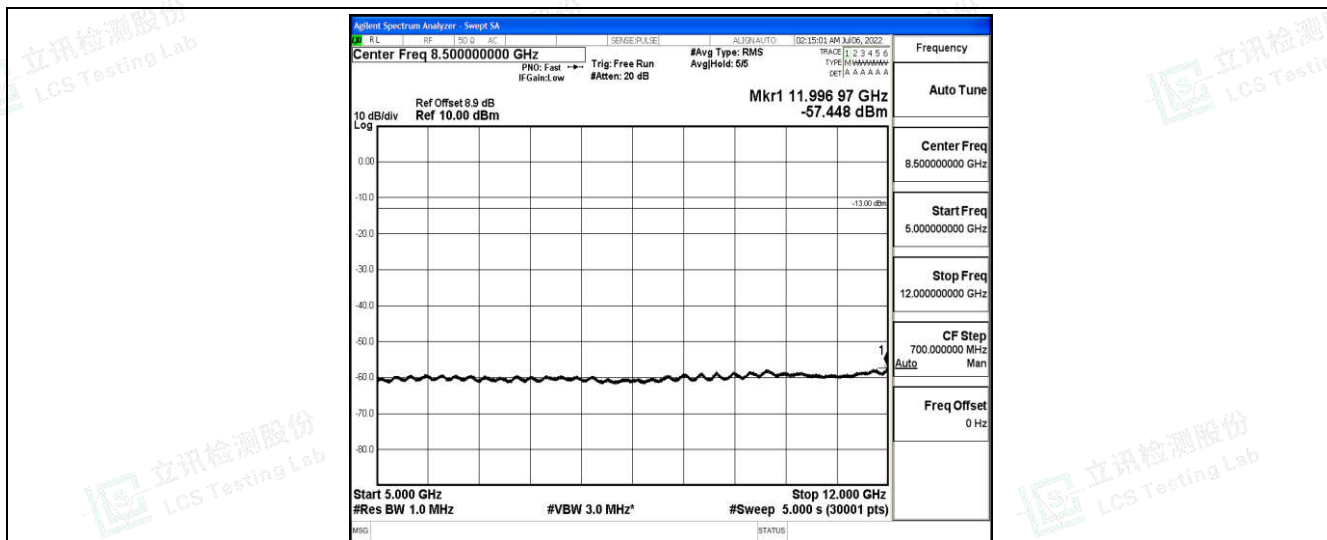
Band25-10MHz-QPSK-26090-1-0-Low-5000-12000--57.45-PASS
