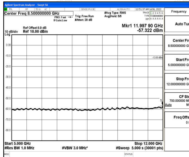
Band25-1.4MHz-QPSK-26047-1-0-Low-5000-12000--57.32-PASS
