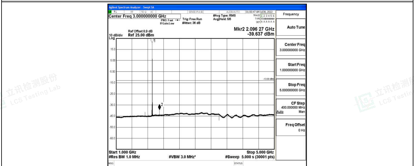
Band25-1.4MHz-16QAM-26683-1-0-High-1000-5000--39.64-PASS
