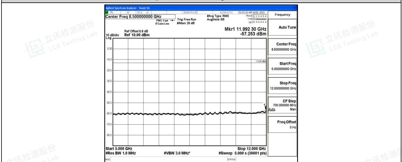
Band25-1.4MHz-16QAM-26683-1-0-High-5000-12000--57.25-PASS
