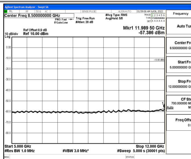
Band25-5MHz-16QAM-26665-1-0-High-5000-12000--57.39-PASS
