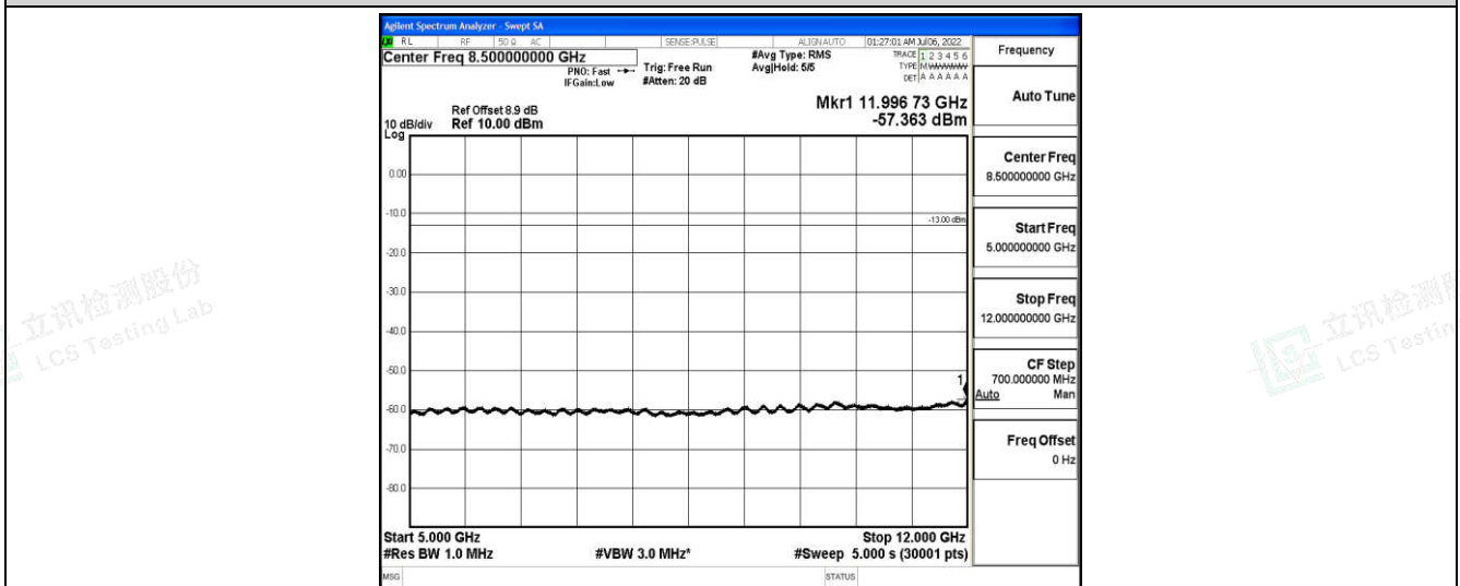
Band25-3MHz-16QAM-26365-1-0-Low-5000-12000--57.36-PASS
