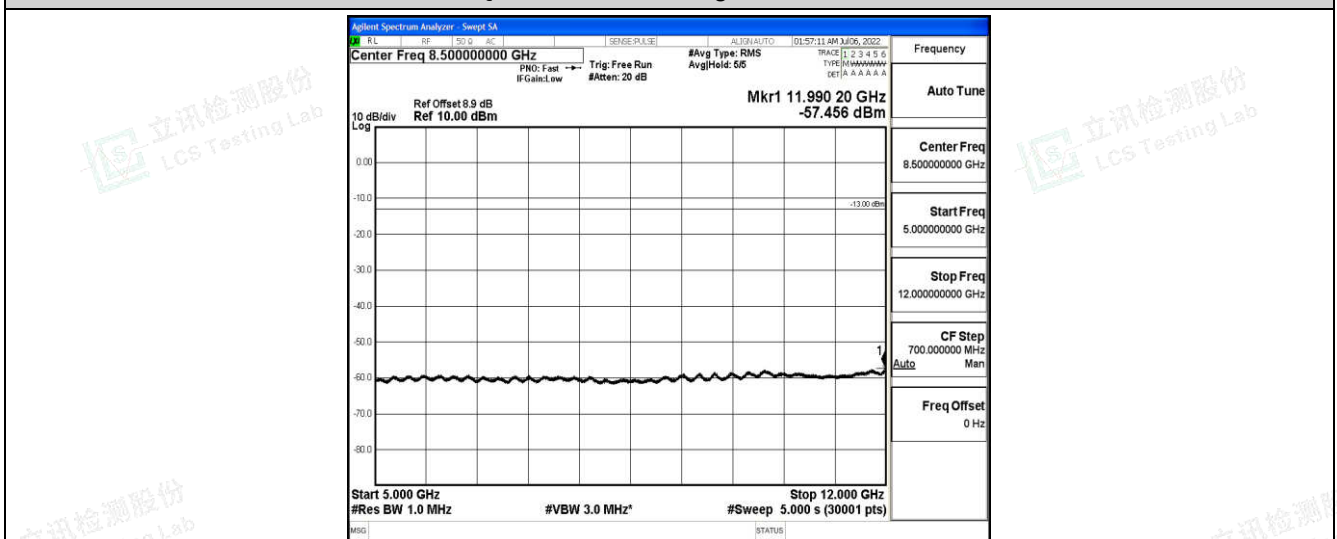
Band25-5MHz-QPSK-26665-1-0-High-5000-12000--57.46-PASS
