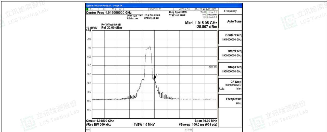
Band25-15MHz-QPSK-26615-6-0-High--25.87-PASS
