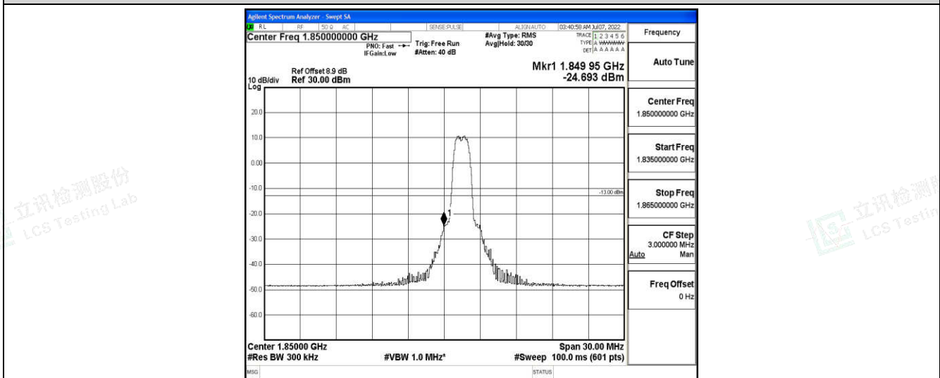
Band25-15MHz-16QAM-26115-6-0-Low--24.69-PASS
