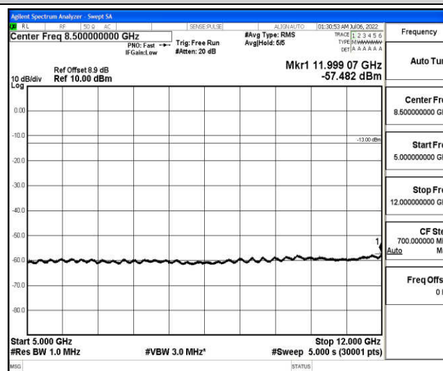
Band25-3MHz-16QAM-26675-1-0-High-5000-12000--57.48-PASS
