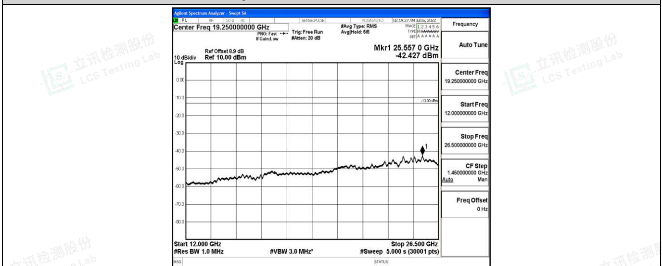
Band25-10MHz-QPSK-26365-1-0-Low-12000-26500--42.43-PASS
