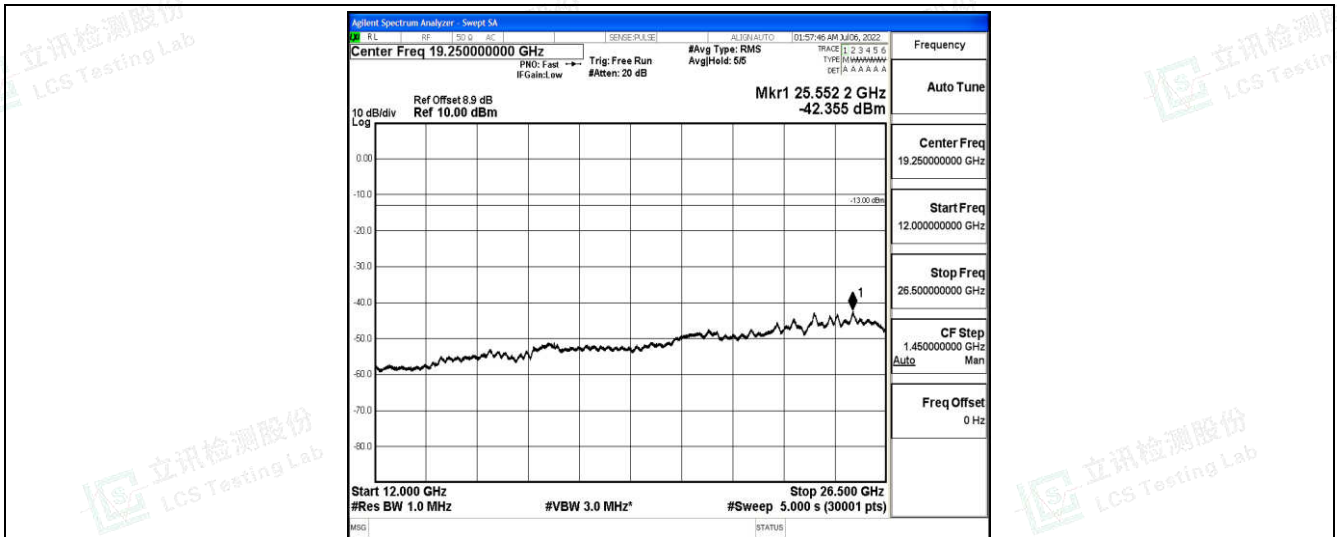
Band25-5MHz-QPSK-26665-1-0-High-12000-26500--42.36-PASS
