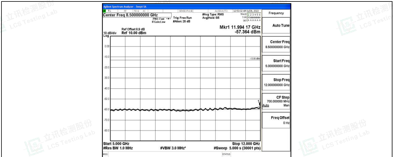
Band25-1.4MHz-16QAM-26047-1-0-Low-5000-12000--57.36-PASS
