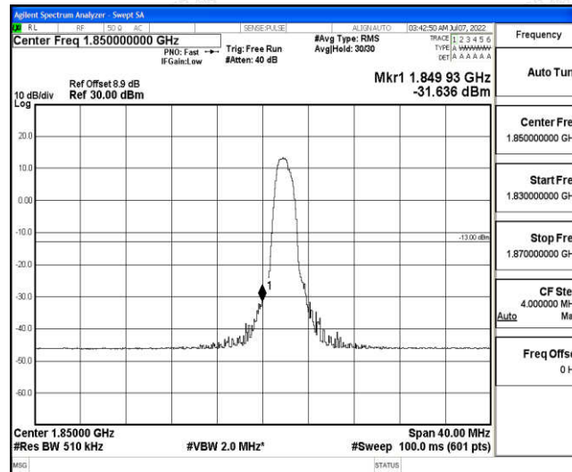
Band25-20MHz-QPSK-26140-6-0-Low--31.64-PASS
