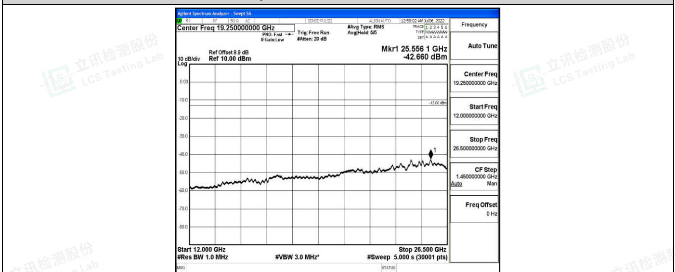
Band25-1.4MHz-16QAM-26365-1-0-Low-12000-26500--42.66-PASS
