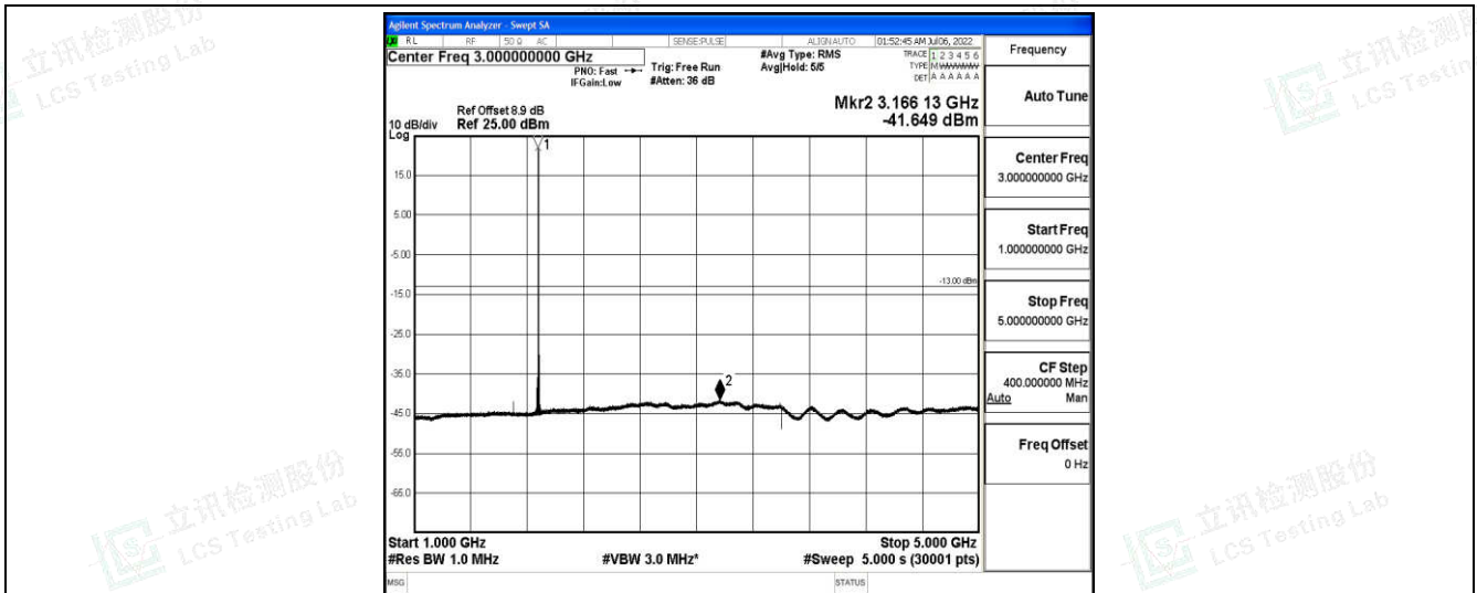
Band25-5MHz-QPSK-26365-1-0-Low-1000-5000--41.65-PASS
