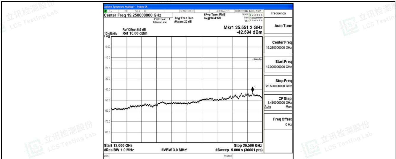
Band25-1.4MHz-QPSK-26683-1-0-High-12000-26500--42.59-PASS
