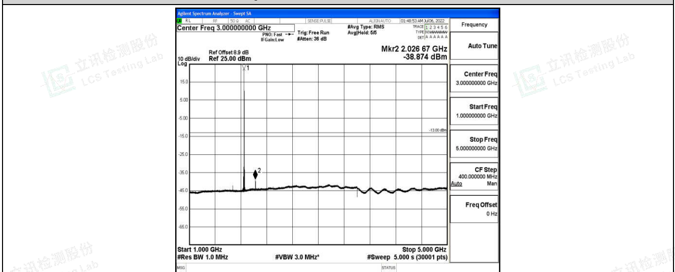
Band25-5MHz-QPSK-26065-1-0-Low-1000-5000--38.87-PASS
