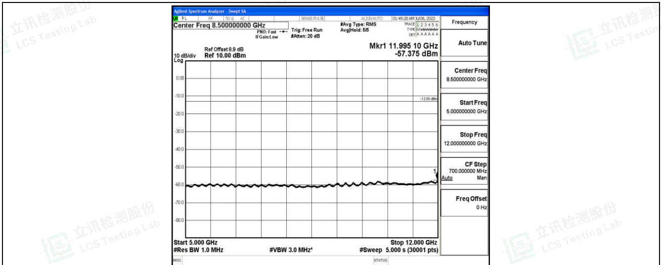
Band25-5MHz-QPSK-26065-1-0-Low-5000-12000--57.38-PASS
