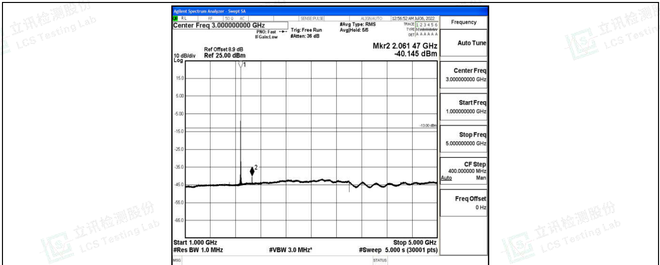
Band25-1.4MHz-16QAM-26365-1-0-Low-1000-5000--40.15-PASS
