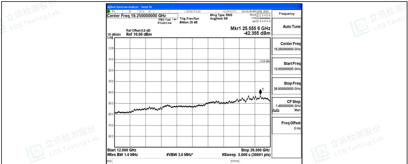
Band25-3MHz-16QAM-26675-1-0-High-12000-26500--42.36-PASS
