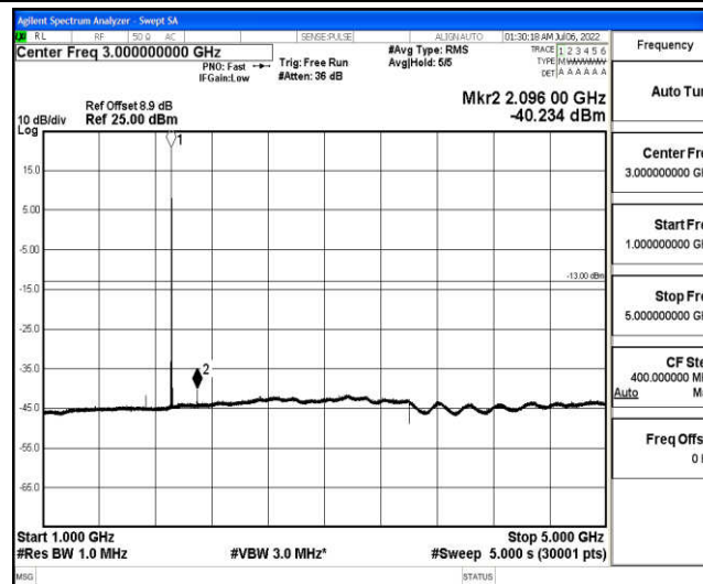
Band25-3MHz-16QAM-26675-1-0-High-1000-5000--40.23-PASS
