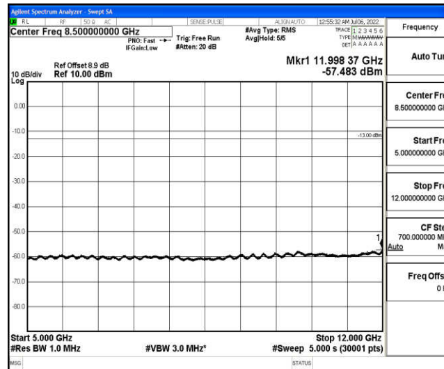
Band25-1.4MHz-QPSK-26365-1-0-Low-5000-12000--57.48-PASS
