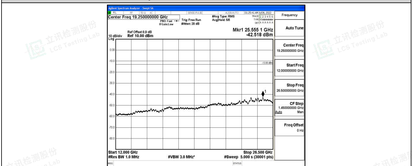
Band25-3MHz-QPSK-26365-1-0-Low-12000-26500--42.52-PASS
