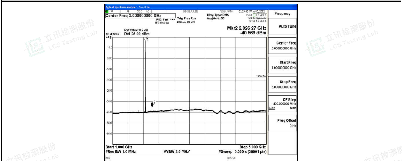
Band25-3MHz-QPSK-26055-1-0-Low-1000-5000--40.57-PASS
