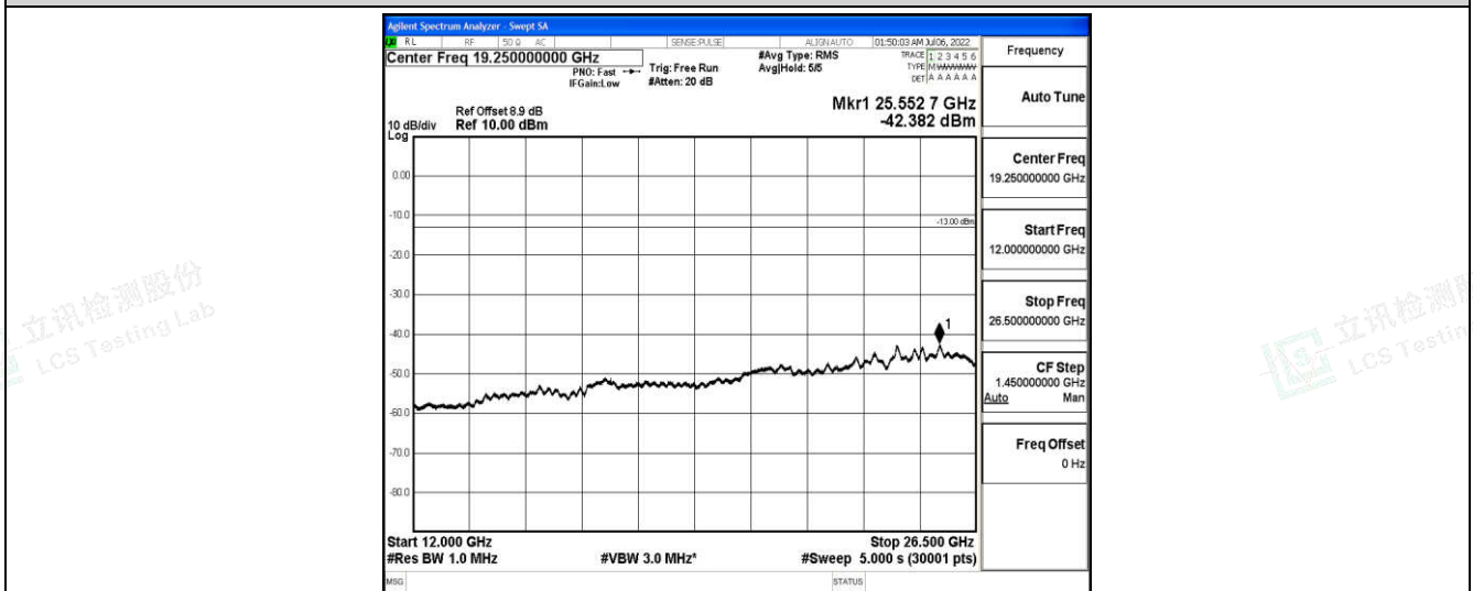
Band25-5MHz-QPSK-26065-1-0-Low-12000-26500--42.38-PASS
