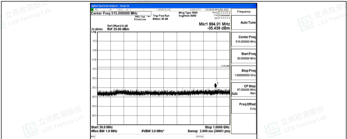
Band25-5MHz-QPSK-26665-1-0-High-30-1000--35.44-PASS
