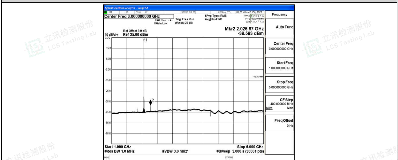
Band25-5MHz-16QAM-26065-1-0-Low-1000-5000--38.58-PASS
