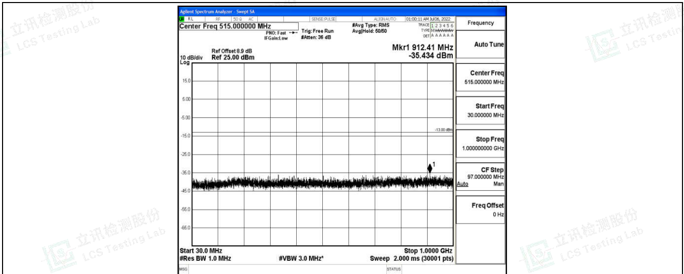
Band25-1.4MHz-16QAM-26683-1-0-High-30-1000--35.43-PASS
