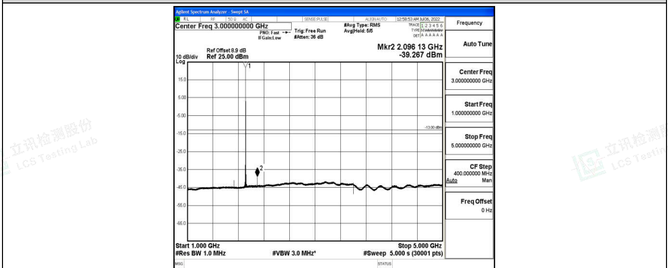
Band25-1.4MHz-QPSK-26683-1-0-High-1000-5000--39.27-PASS
