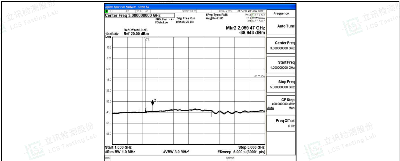
Band25-5MHz-16QAM-26365-1-0-Low-1000-5000--38.94-PASS
