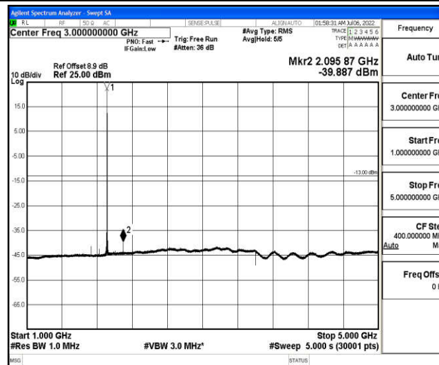
Band25-5MHz-16QAM-26665-1-0-High-1000-5000--39.89-PASS
