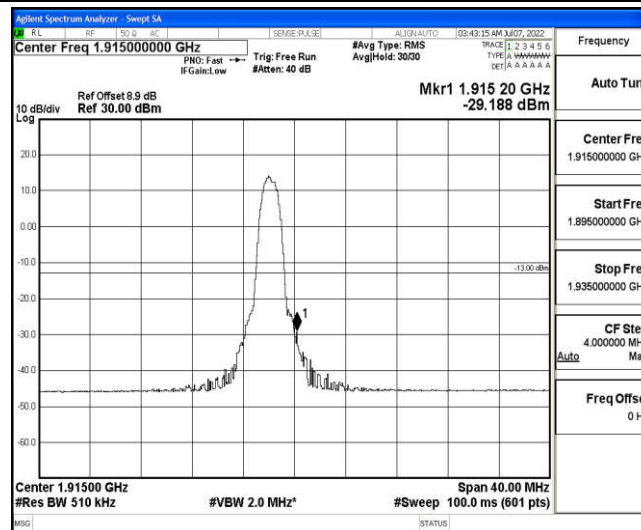
Band25-20MHz-QPSK-26590-6-0-High--29.19-PASS
