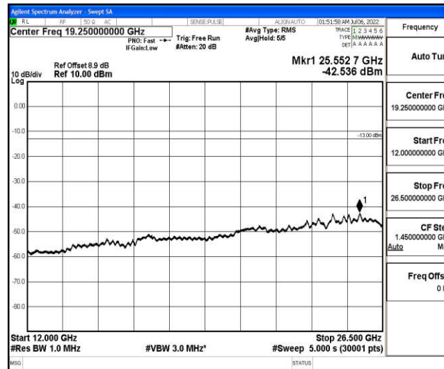
Band25-5MHz-16QAM-26065-1-0-Low-12000-26500--42.54-PASS
