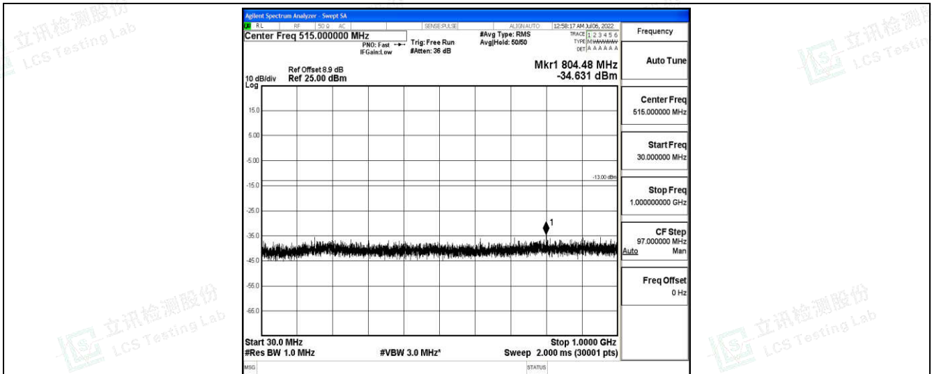
Band25-1.4MHz-QPSK-26683-1-0-High-30-1000--34.63-PASS
