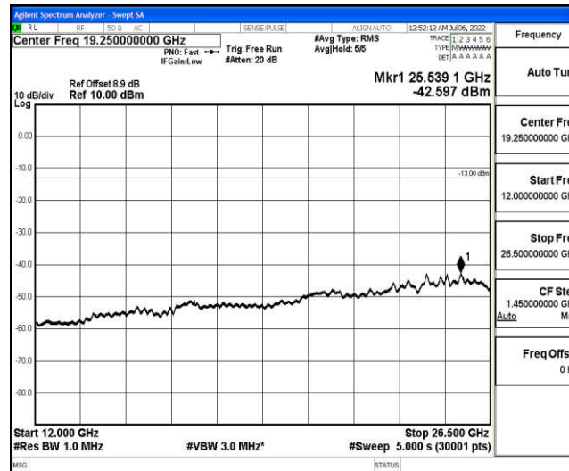
Band25-1.4MHz-QPSK-26047-1-0-Low-12000-26500--42.6-PASS
