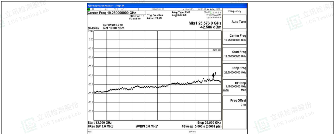
Band25-10MHz-QPSK-26640-1-0-High-12000-26500--42.59-PASS
