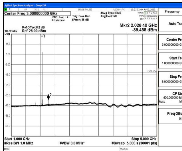
Band25-1.4MHz-QPSK-26047-1-0-Low-1000-5000--39.46-PASS
