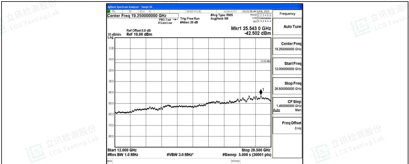
Band25-1.4MHz-16QAM-26683-1-0-High-12000-26500--42.5-PASS
