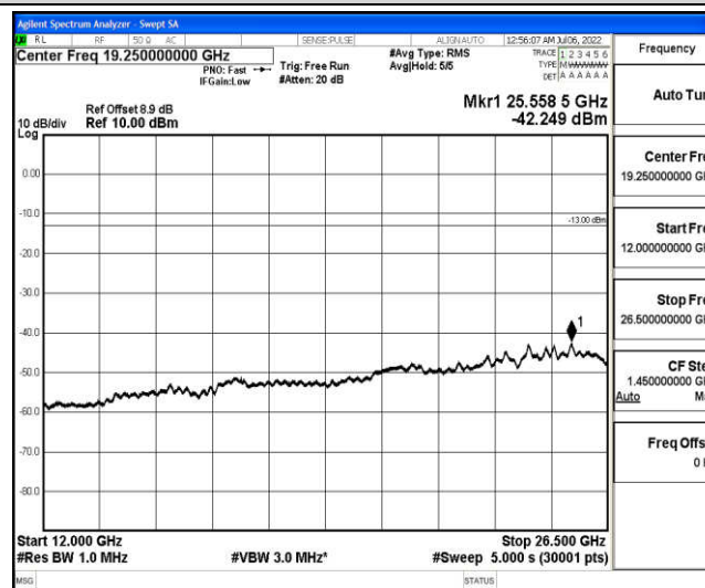
Band25-1.4MHz-QPSK-26365-1-0-Low-12000-26500--42.25-PASS
