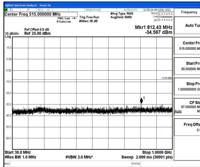
Band25-1.4MHz-QPSK-26047-1-0-Low-30-1000--34.57-PASS
