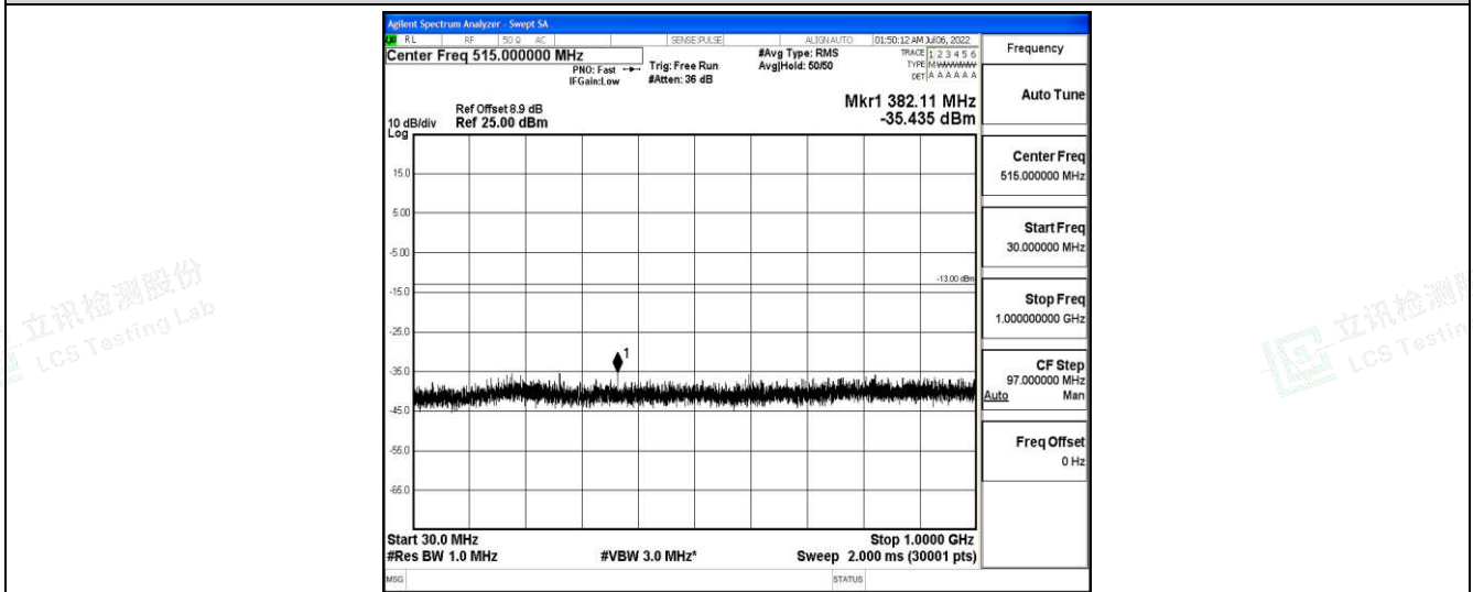
Band25-5MHz-16QAM-26065-1-0-Low-30-1000--35.44-PASS
