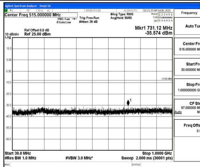
Band25-10MHz-QPSK-26640-1-0-High-30-1000--35.57-PASS
