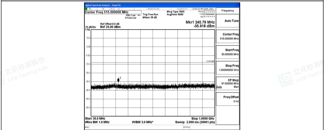
Band25-1.4MHz-16QAM-26047-1-0-Low-30-1000--35.92-PASS
