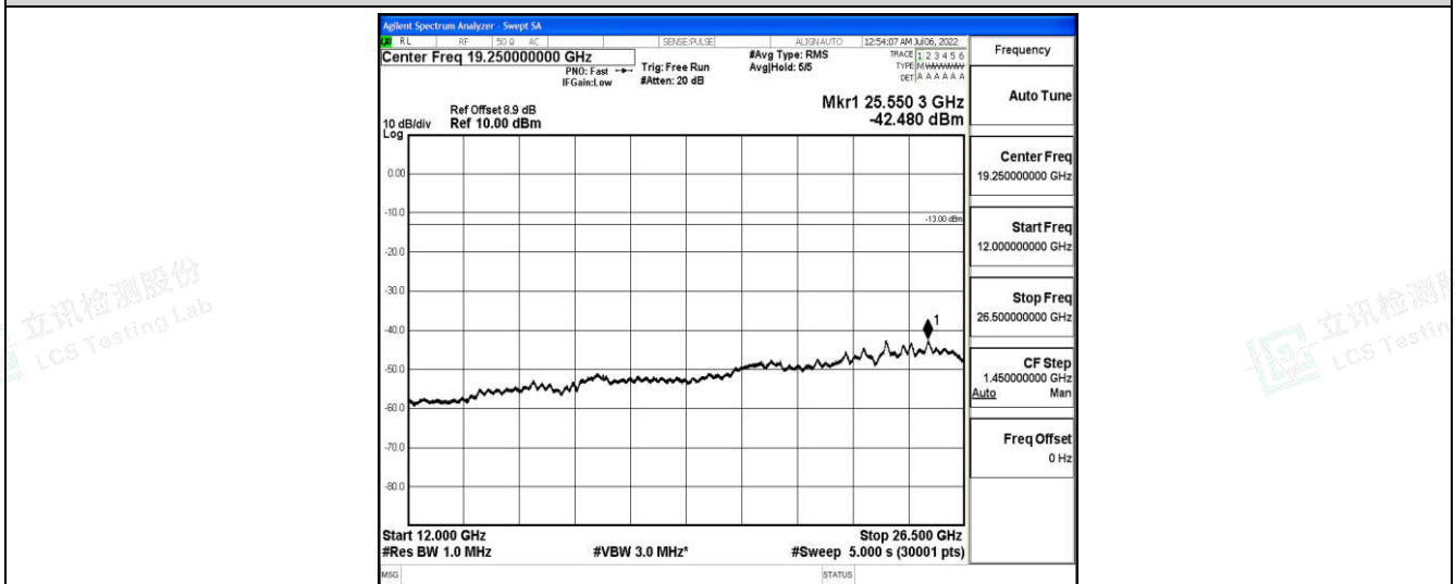
Band25-1.4MHz-16QAM-26047-1-0-Low-12000-26500--42.48-PASS
