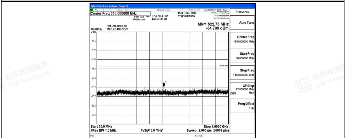
Band25-10MHz-16QAM-26090-1-0-Low-30-1000--34.79-PASS
