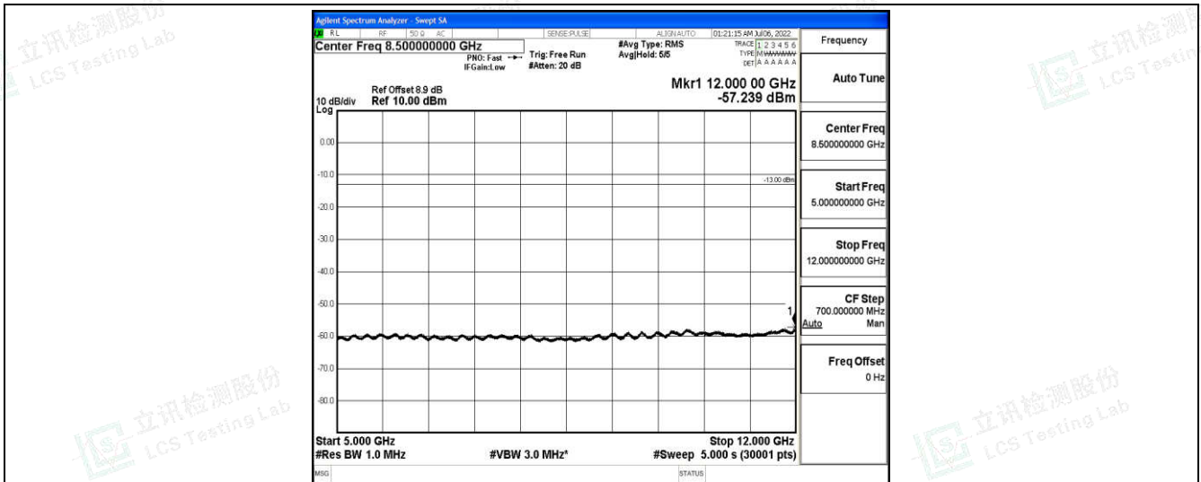
Band25-3MHz-QPSK-26055-1-0-Low-5000-12000--57.24-PASS
