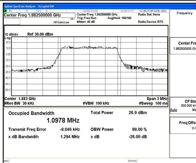
Band25-1.4MHz-QPSK-26365-6-0-Low-1.0978-1.294-PASS
