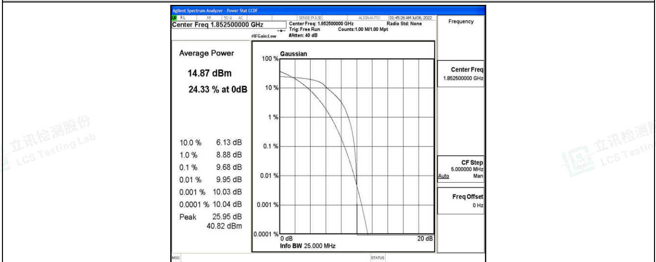
Band25-5MHz-QPSK-26065-6-0-Low-9.68-&lt;=13-PASS
