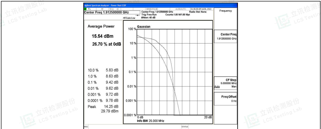
Band25-5MHz-QPSK-26665-6-0-High-9.42-&lt;=13-PASS
