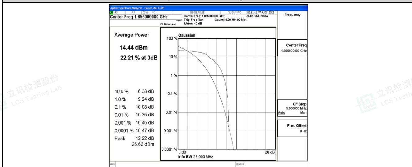
Band25-10MHz-16QAM-26090-6-0-Low-10.08-&lt;=13-PASS
