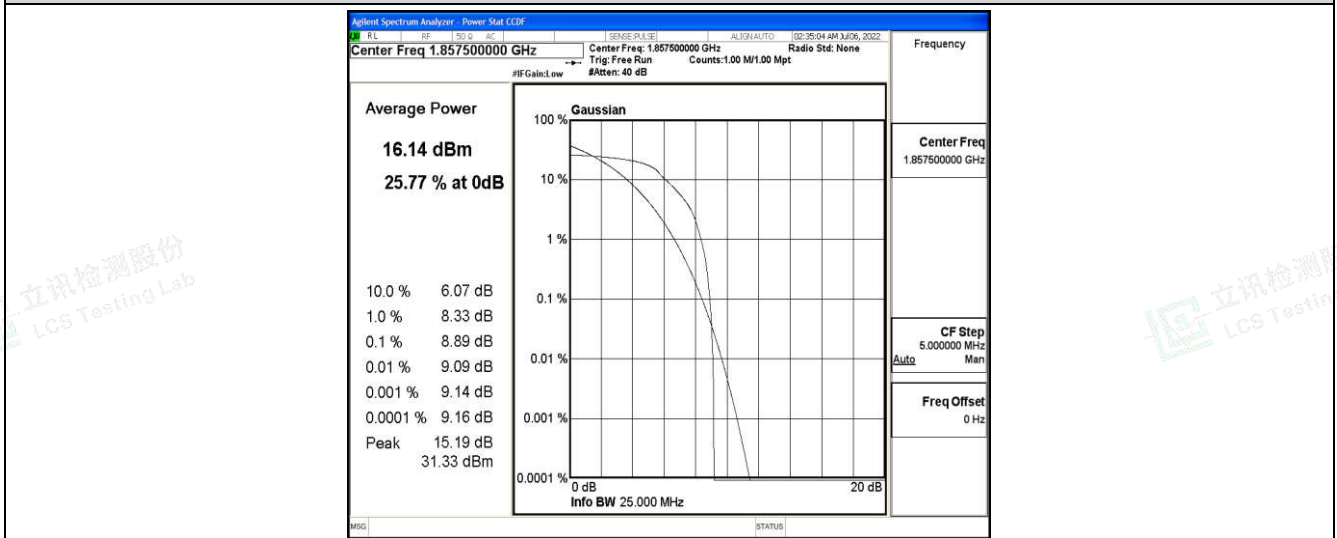
Band25-15MHz-16QAM-26115-6-0-Low-8.89-&lt;=13-PASS
