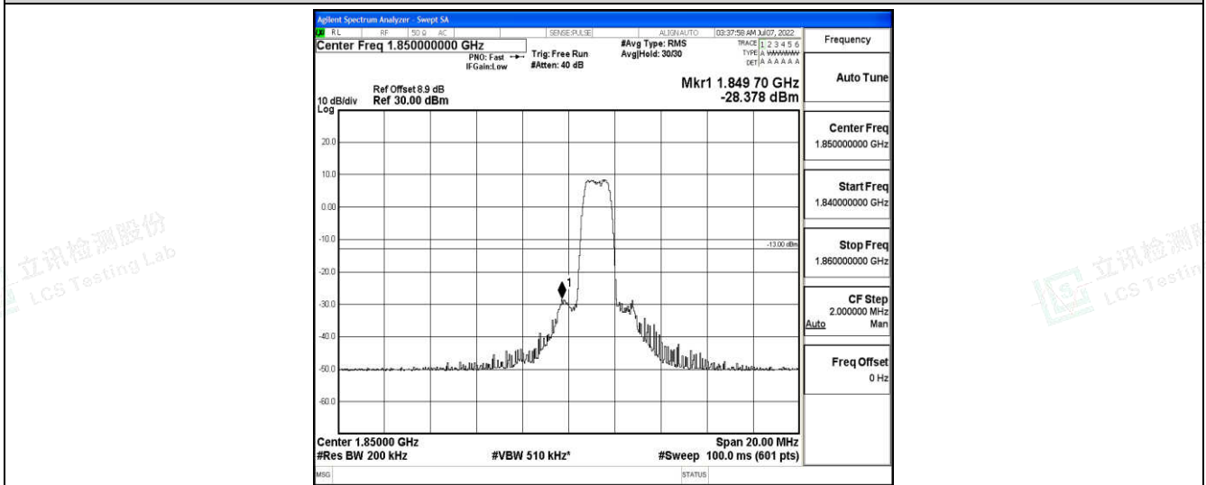
Band25-10MHz-QPSK-26090-6-0-Low--28.38-PASS
