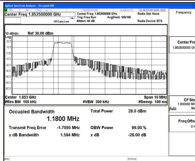
Band25-5MHz-16QAM-26065-6-0-Low-1.1800-1.594-PASS
