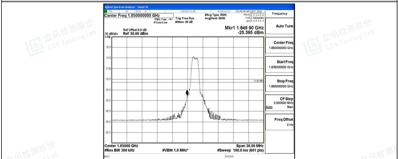
Band25-15MHz-QPSK-26115-6-0-Low--25.39-PASS
