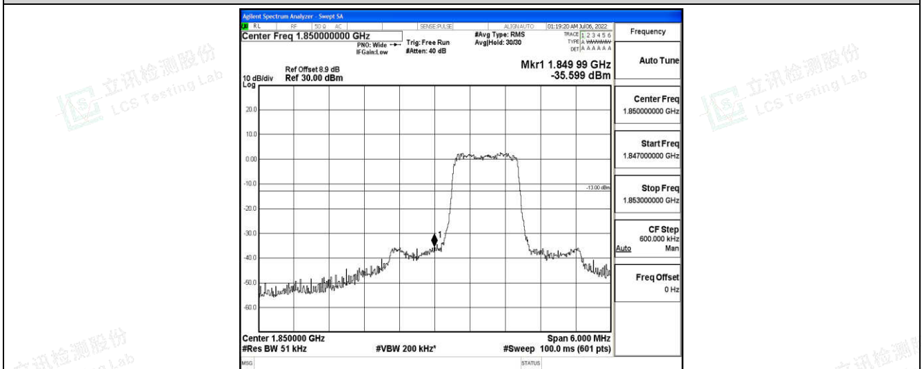
Band25-3MHz-QPSK-26055-6-0-Low--35.60-PASS
