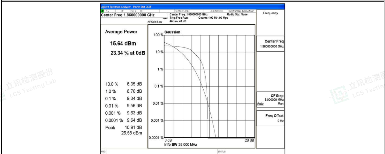
Band25-20MHz-16QAM-26140-6-0-Low-9.34-&lt;=13-PASS
