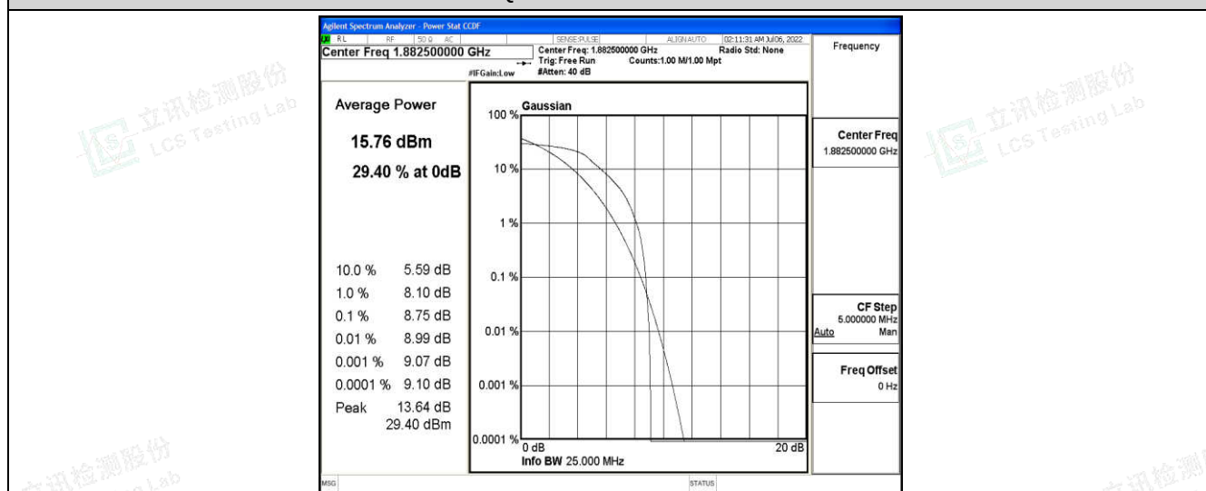
Band25-10MHz-16QAM-26365-6-0-Low-8.75-&lt;=13-PASS
