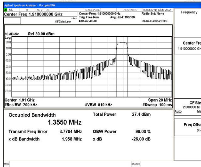
Band25-10MHz-QPSK-26640-6-0-High-1.3550-1.958-PASS
