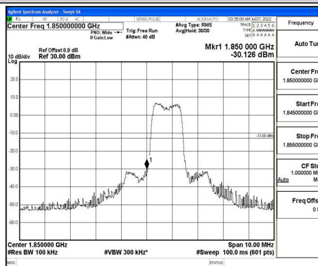
Band25-5MHz-16QAM-26065-6-0-Low--30.13-PASS
