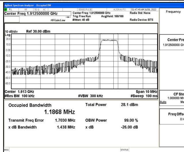
Band25-5MHz-QPSK-26665-6-0-High-1.1868-1.438-PASS
