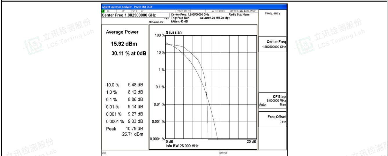
Band25-5MHz-16QAM-26365-6-0-Low-8.86-&lt;=13-PASS
