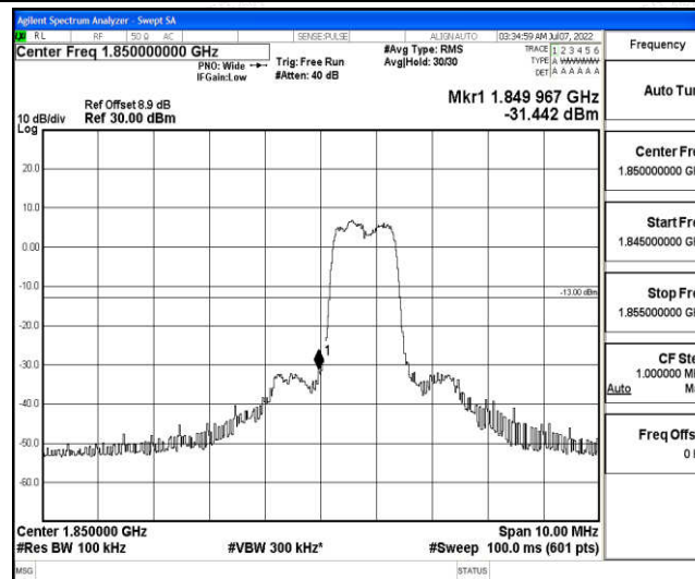
Band25-5MHz-QPSK-26065-6-0-Low--31.44-PASS
