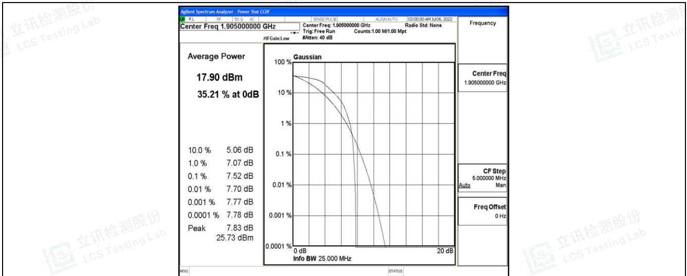
Band25-20MHz-QPSK-26590-6-0-High-7.52-&lt;=13-PASS
