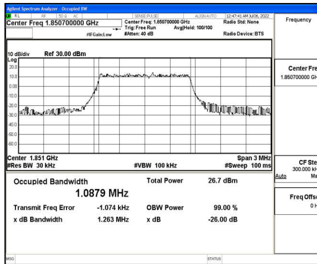
Band25-1.4MHz-QPSK-26047-6-0-Low-1.0879-1.263-PASS
