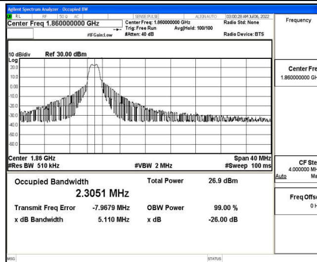
Band25-20MHz-QPSK-26140-6-0-Low-2.3051-5.110-PASS
