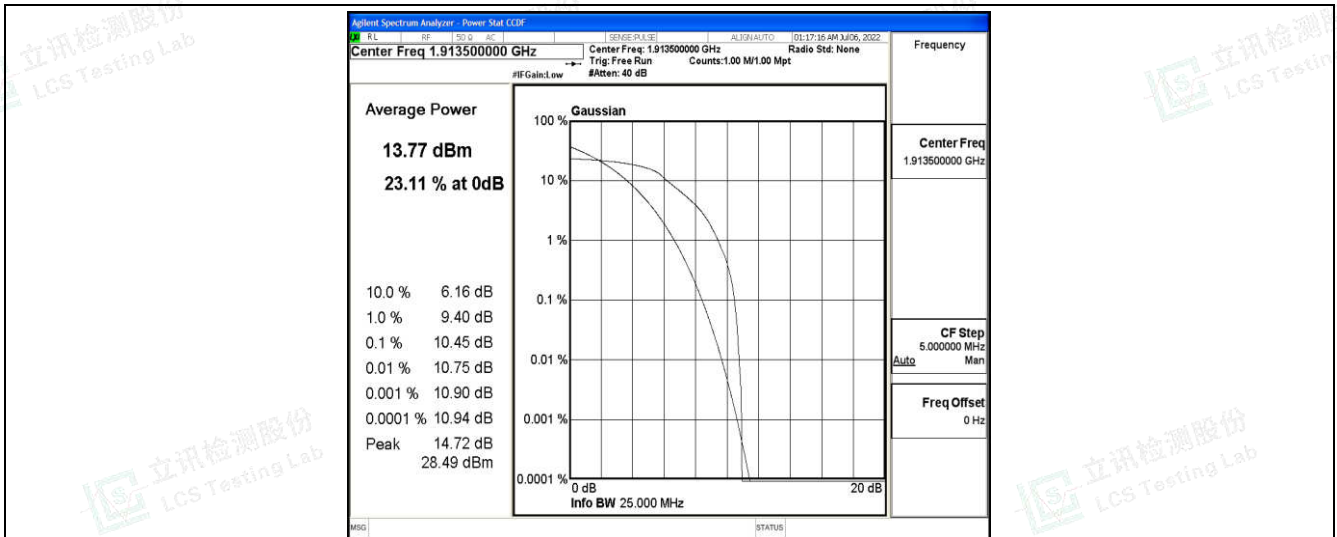
Band25-3MHz-16QAM-26675-6-0-High-10.45-&lt;=13-PASS
