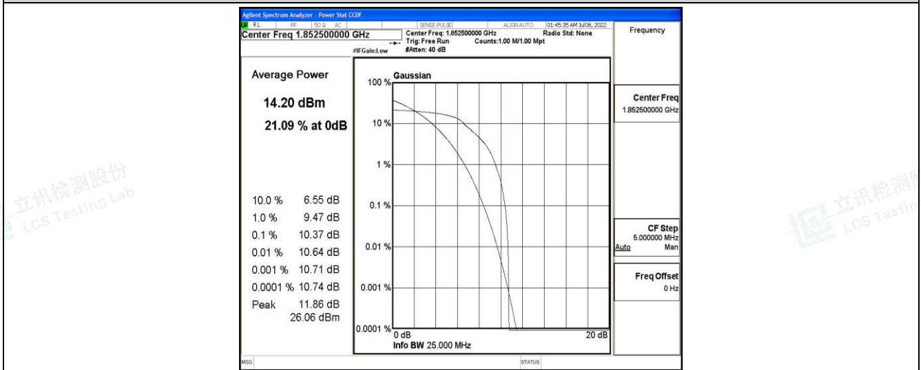
Band25-5MHz-16QAM-26065-6-0-Low-10.37-&lt;=13-PASS
