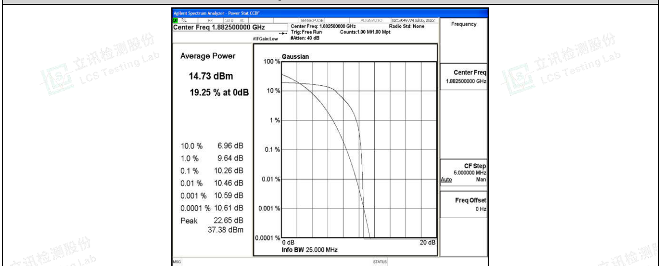
Band25-20MHz-16QAM-26365-6-0-Low-10.26-&lt;=13-PASS
