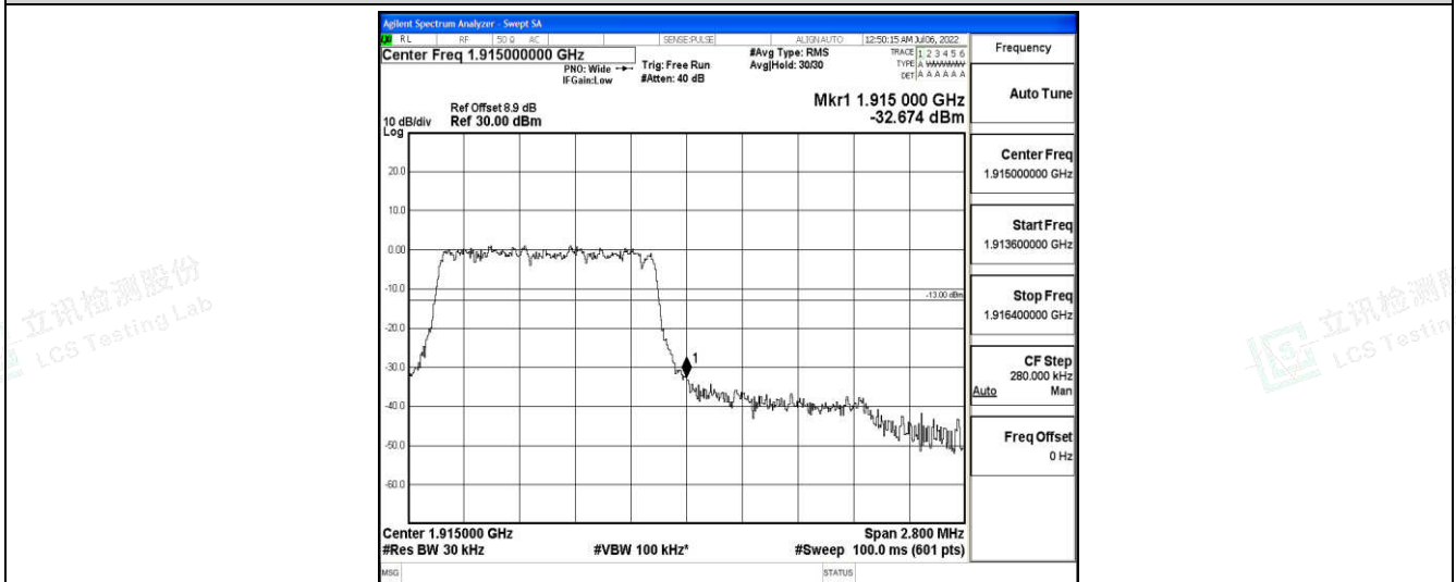
Band25-1.4MHz-16QAM-26683-6-0-High--32.67-PASS
