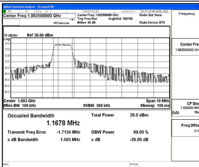
Band25-5MHz-QPSK-26365-6-0-Low-1.1678-1.503-PASS
