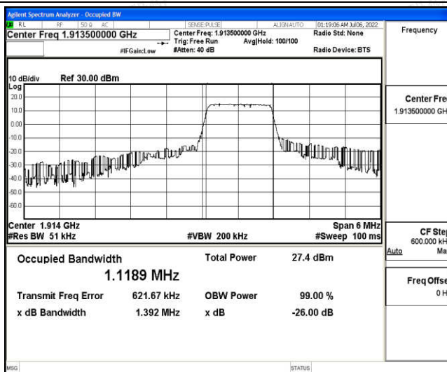
Band25-3MHz-16QAM-26675-6-0-High-1.1189-1.392-PASS
