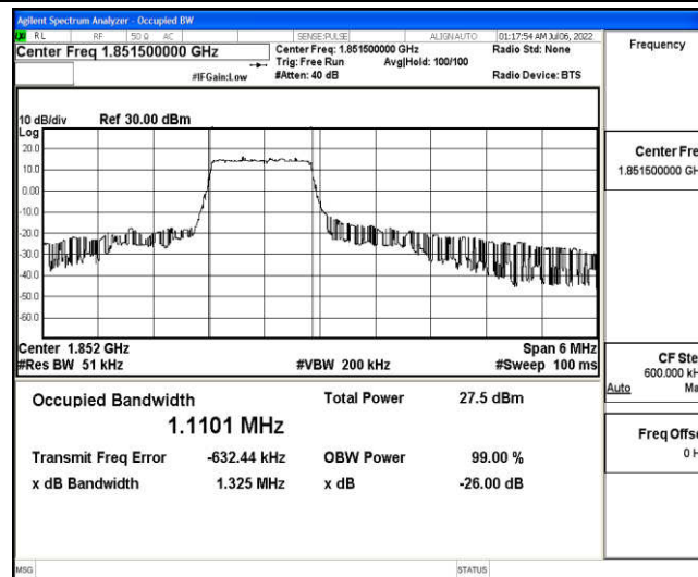
Band25-3MHz-16QAM-26055-6-0-Low-1.1101-1.325-PASS
