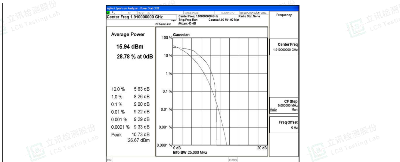
Band25-10MHz-QPSK-26640-6-0-High-9.00-&lt;=13-PASS
