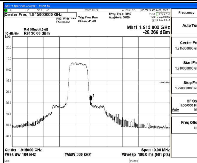
Band25-5MHz-QPSK-26665-6-0-High--28.37-PASS
