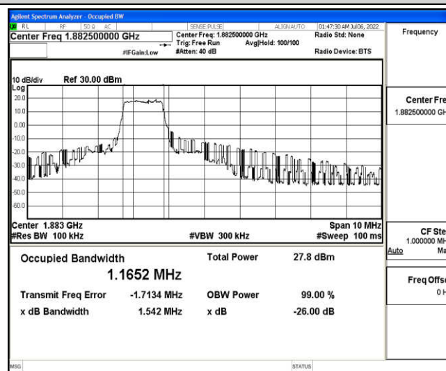
Band25-5MHz-16QAM-26365-6-0-Low-1.1652-1.542-PASS
