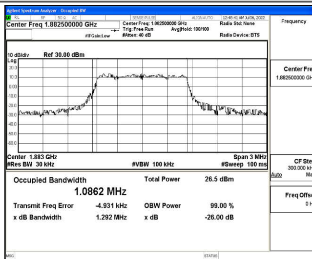
Band25-1.4MHz-16QAM-26365-6-0-Low-1.0862-1.292-PASS
