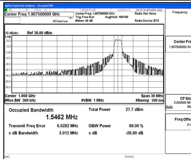
Band25-15MHz-QPSK-26615-6-0-High-1.5462-3.012-PASS
