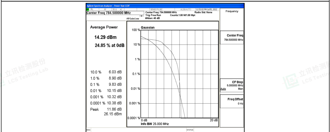
Band13-5MHz-16QAM-23255-6-0-High-9.83-&lt;=13-PASS
