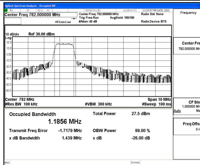
Band13-5MHz-QPSK-23230-6-0-Low-1.1856-1.439-PASS
