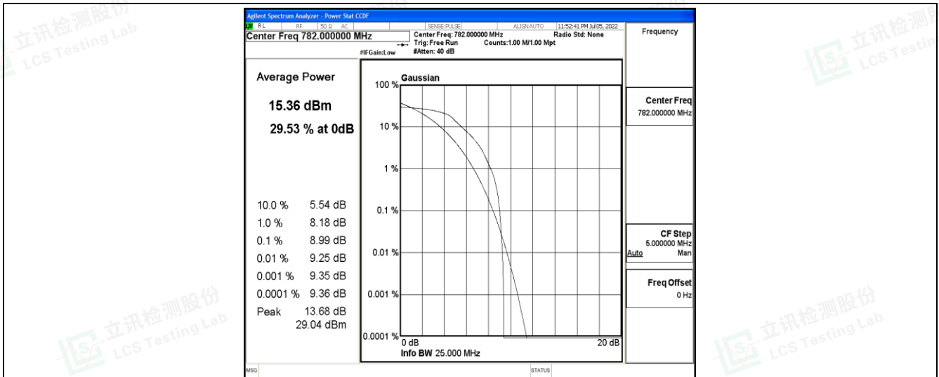
Band13-5MHz-16QAM-23230-6-0-Low-8.99-&lt;=13-PASS
