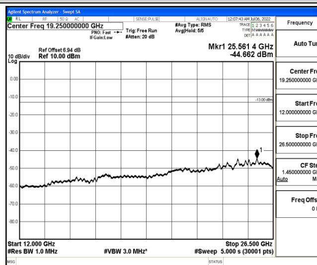
Band13-5MHz-16QAM-23230-1-0-Low-12000-26500--44.66-PASS
