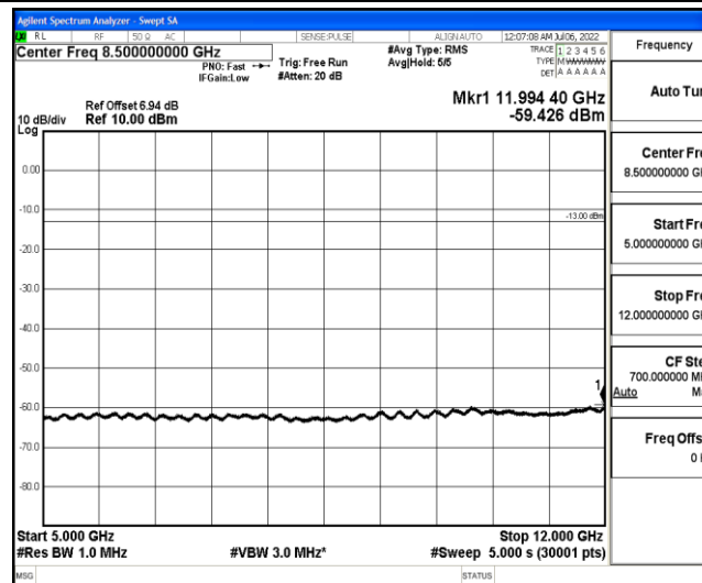
Band13-5MHz-16QAM-23230-1-0-Low-5000-12000--59.43-PASS
