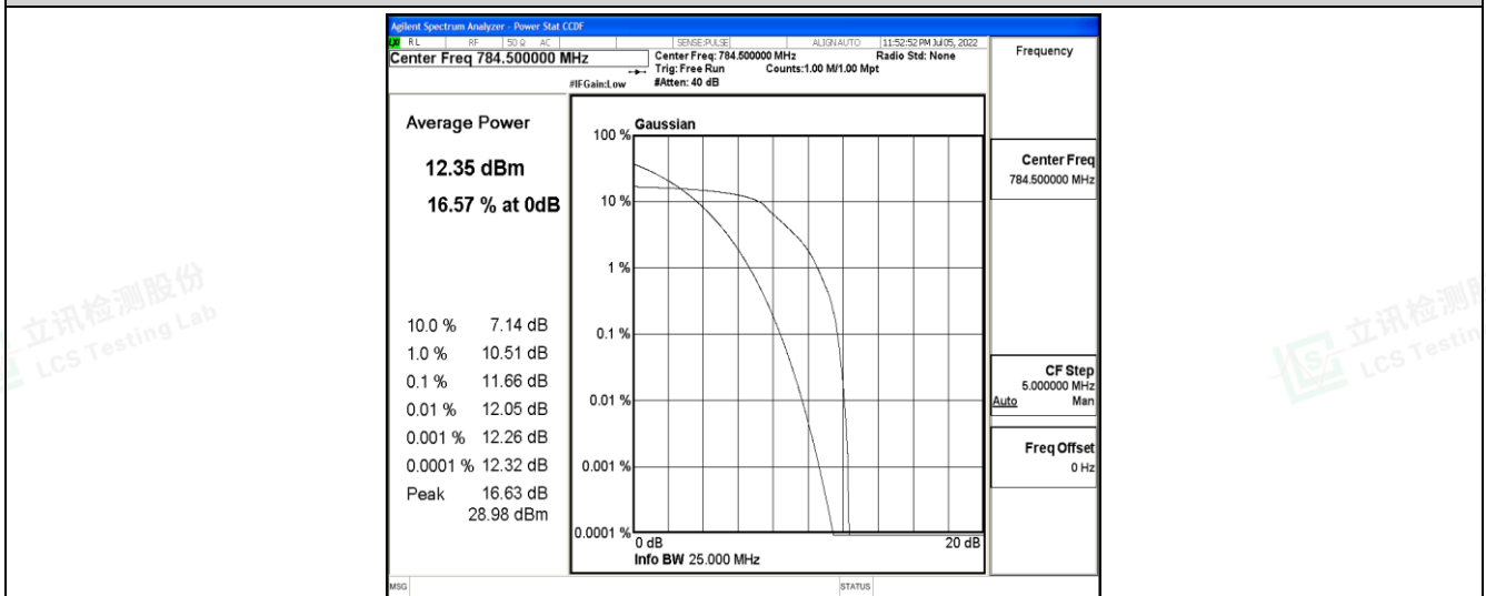
Band13-5MHz-QPSK-23255-6-0-High-11.66-&lt;=13-PASS
