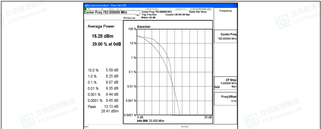
Band13-5MHz-QPSK-23230-6-0-Low-9.07-&lt;=13-PASS
