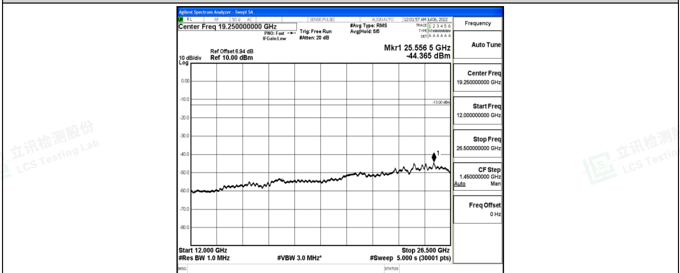
Band13-5MHz-QPSK-23205-1-0-Low-12000-26500--44.37-PASS
