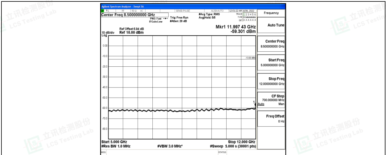
Band13-5MHz-QPSK-23205-1-0-Low-5000-12000--59.3-PASS
