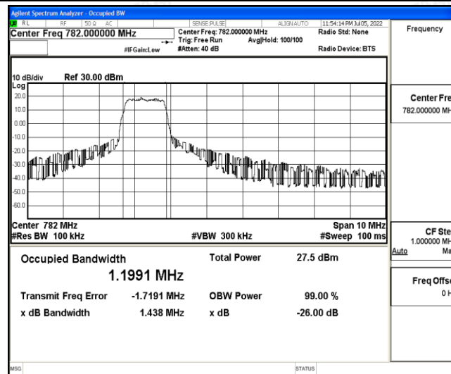
Band13-5MHz-16QAM-23230-6-0-Low-1.1991-1.438-PASS
