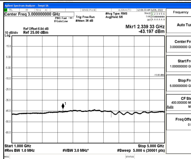
Band13-5MHz-16QAM-23230-1-0-Low-1000-5000--43.2-PASS
