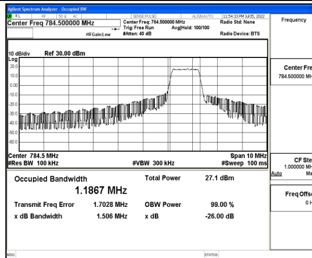
Band13-5MHz-QPSK-23255-6-0-High-1.1867-1.506-PASS
