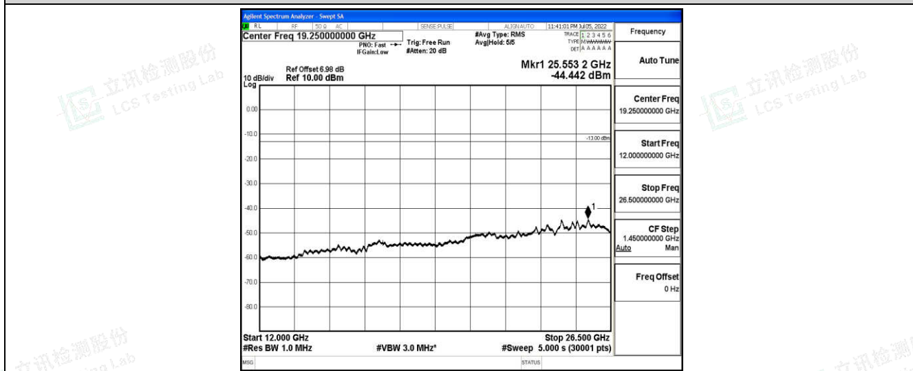
Band12-10MHz-16QAM-23095-1-0-Low-12000-26500--44.44-PASS
