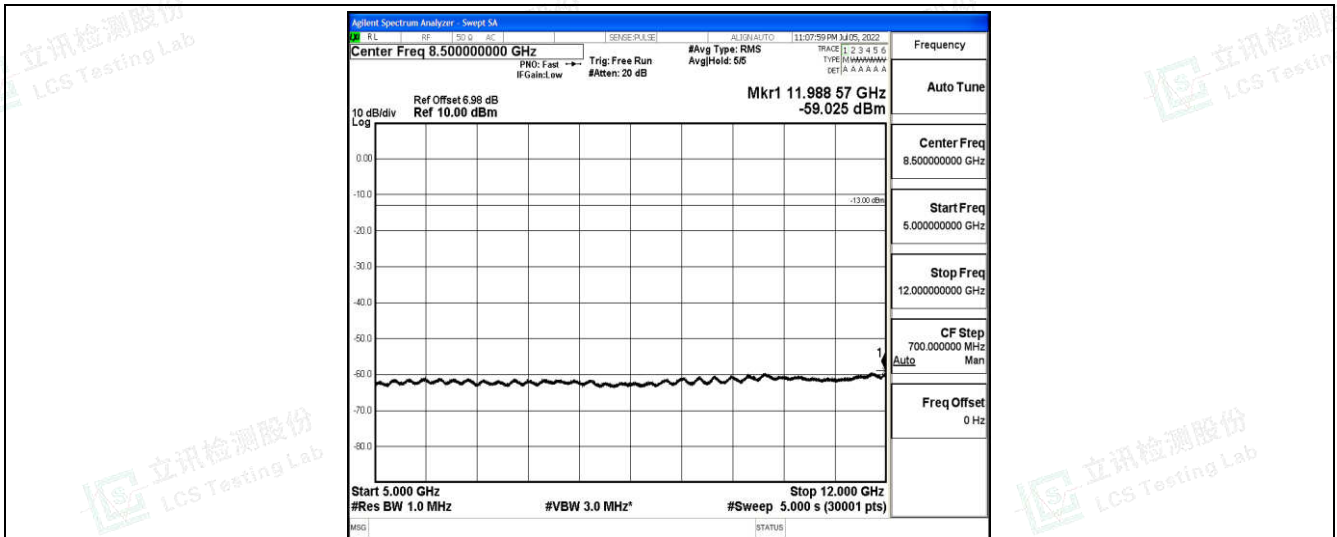
Band12-5MHz-QPSK-23035-1-0-Low-5000-12000--59.03-PASS
