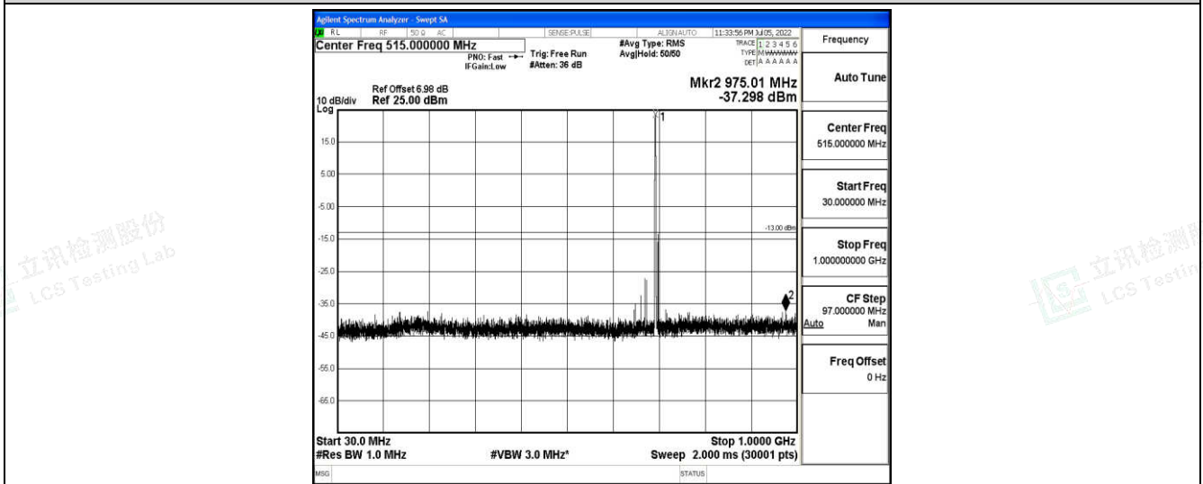
Band12-10MHz-16QAM-23060-1-0-Low-30-1000--37.3-PASS
