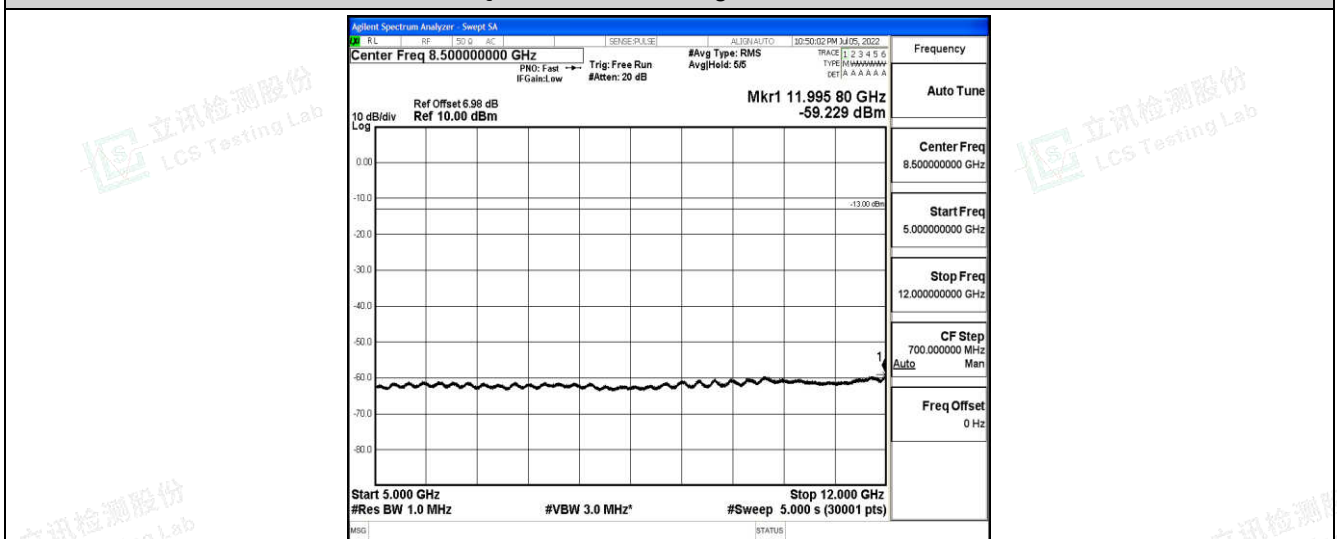
Band12-3MHz-QPSK-23165-1-0-High-5000-12000--59.23-PASS
