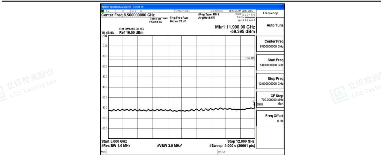
Band12-10MHz-16QAM-23095-1-0-Low-5000-12000--59.4-PASS
