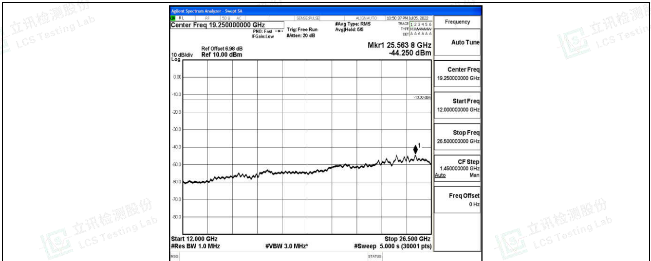
Band12-3MHz-QPSK-23165-1-0-High-12000-26500--44.25-PASS
