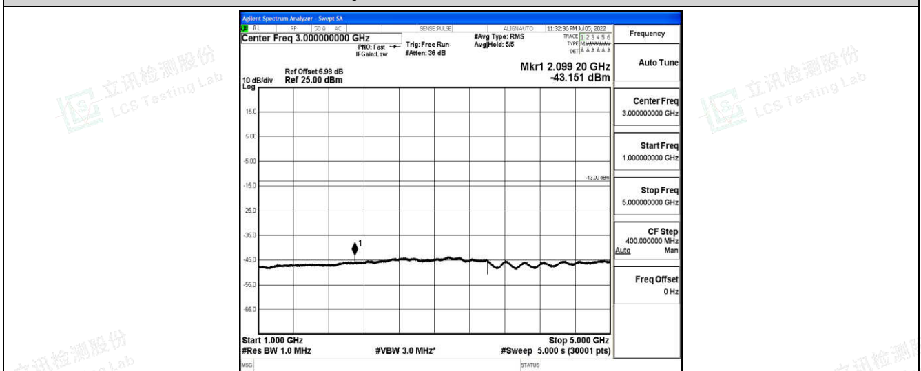
Band12-10MHz-QPSK-23060-1-0-Low-1000-5000--43.15-PASS
