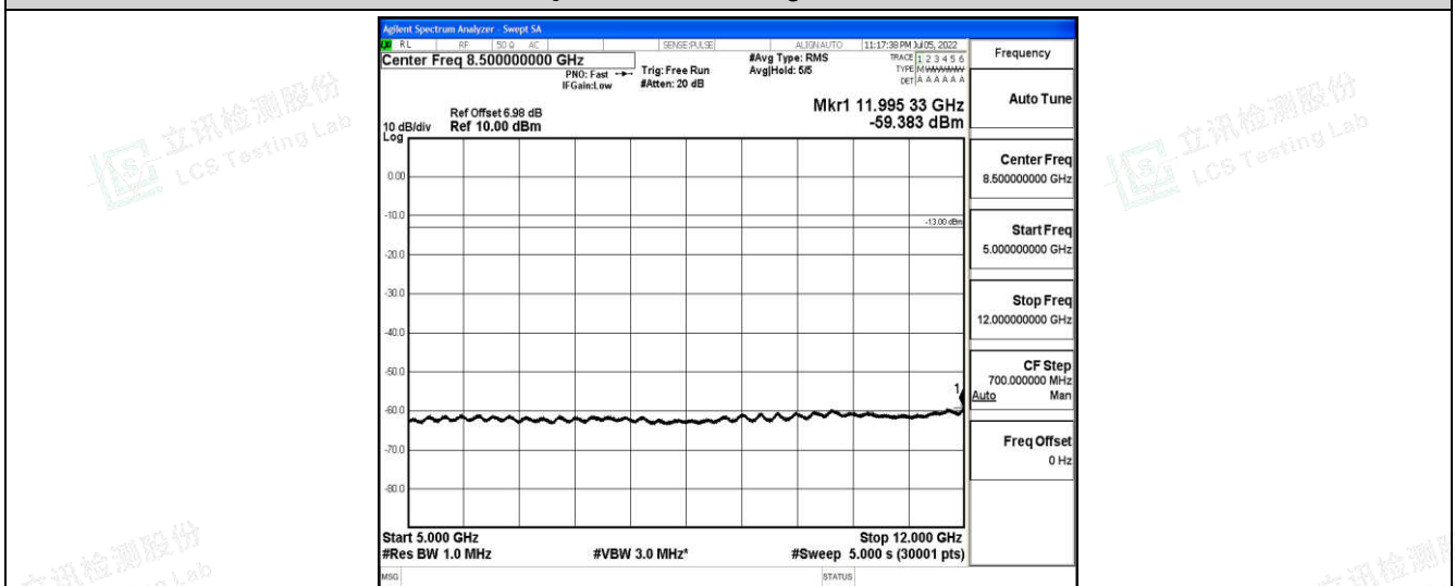
Band12-5MHz-16QAM-23155-1-0-High-5000-12000--59.38-PASS
