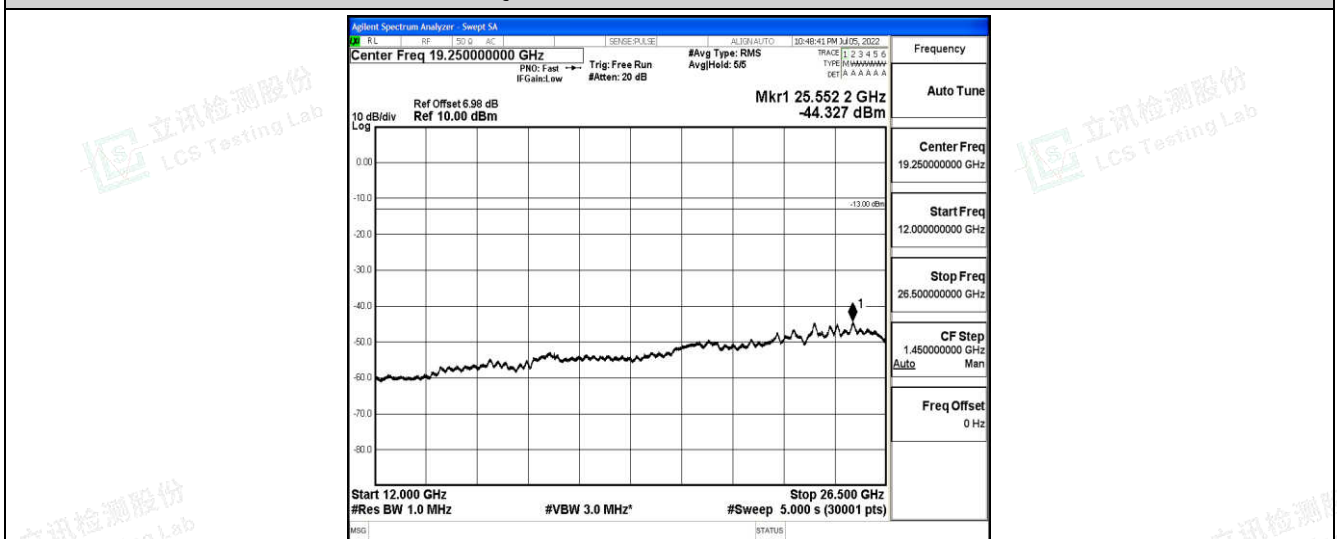
Band12-3MHz-16QAM-23095-1-0-Low-12000-26500--44.33-PASS
