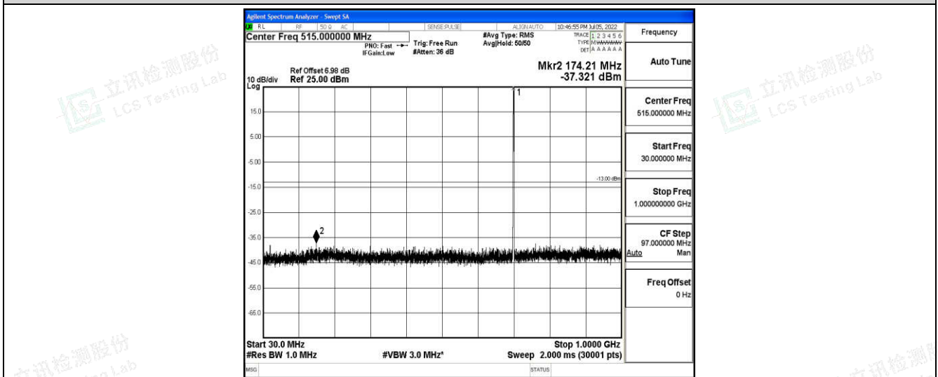
Band12-3MHz-16QAM-23095-1-0-Low-30-1000--37.32-PASS
