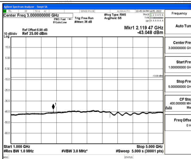
Band12-3MHz-QPSK-23095-1-0-Low-1000-5000--43.05-PASS
