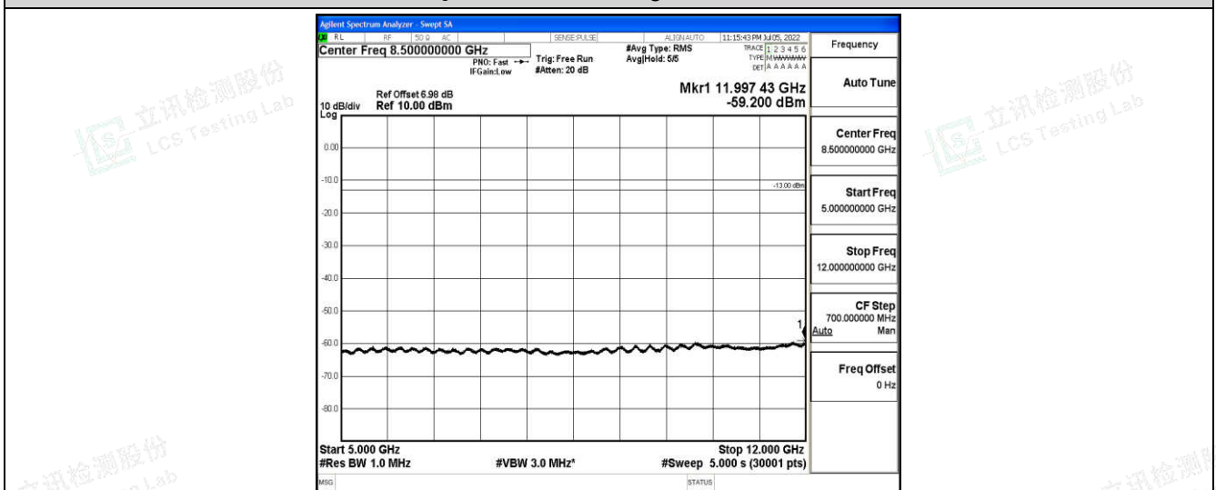
Band12-5MHz-QPSK-23155-1-0-High-5000-12000--59.2-PASS
