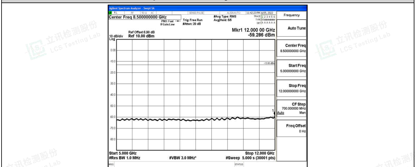
Band12-10MHz-QPSK-23130-1-0-High-5000-12000--59.29-PASS
