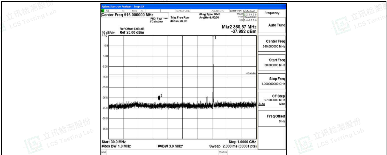
Band12-3MHz-16QAM-23165-1-0-High-30-1000--37.99-PASS
