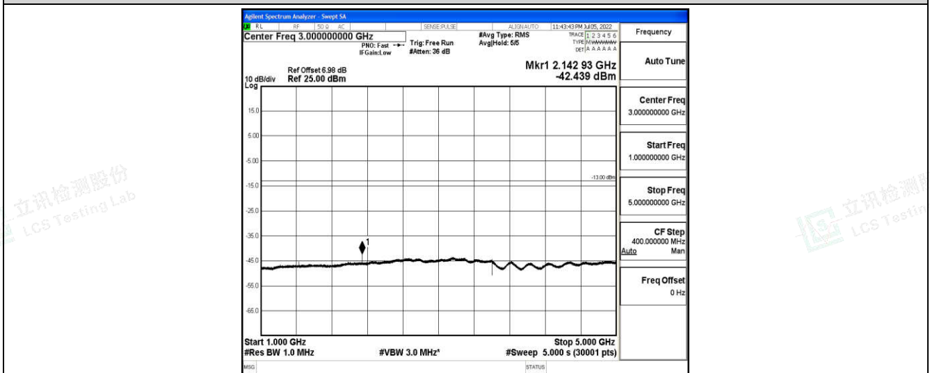
Band12-10MHz-16QAM-23130-1-0-High-1000-5000--42.44-PASS
