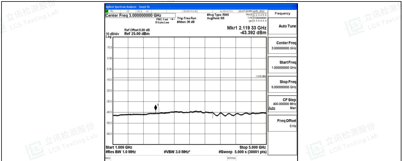
Band12-3MHz-16QAM-23095-1-0-Low-1000-5000--43.39-PASS
