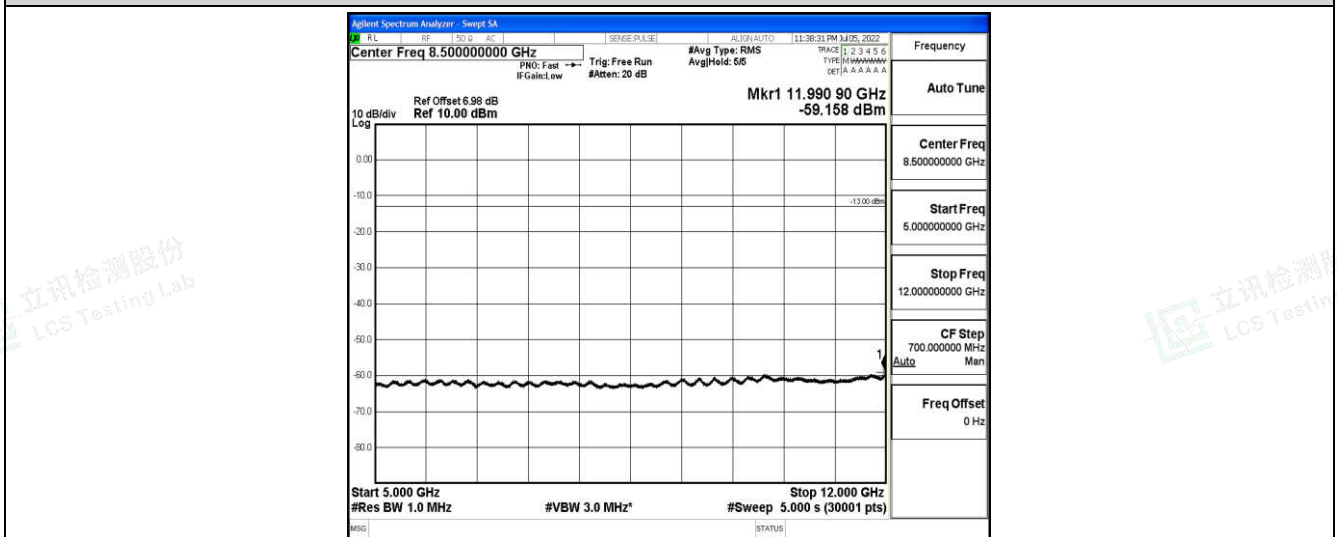
Band12-10MHz-QPSK-23095-1-0-Low-5000-12000--59.16-PASS
