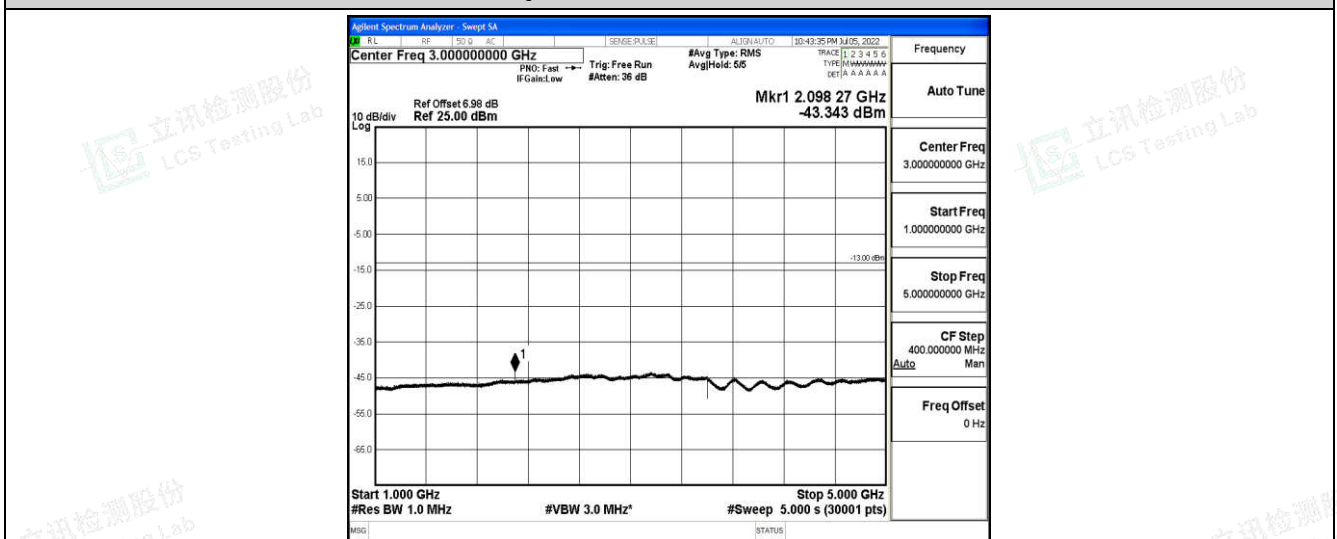
Band12-3MHz-16QAM-23025-1-0-Low-1000-5000--43.34-PASS
