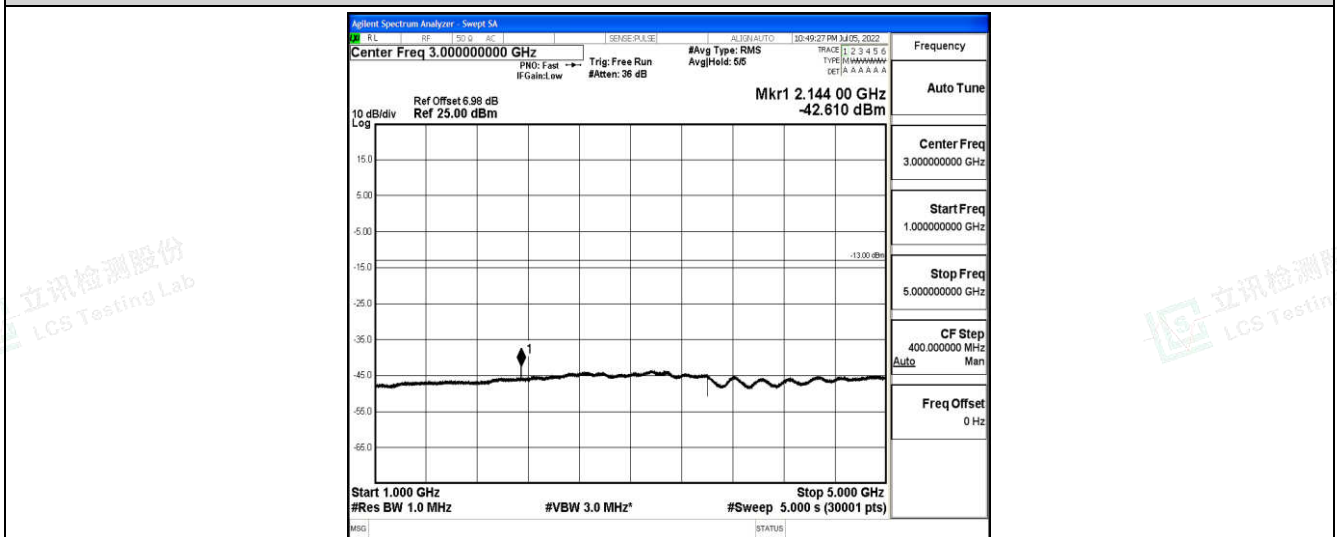
Band12-3MHz-QPSK-23165-1-0-High-1000-5000--42.61-PASS
