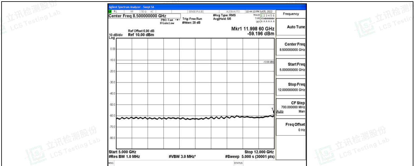
Band12-3MHz-16QAM-23025-1-0-Low-5000-12000--59.2-PASS
