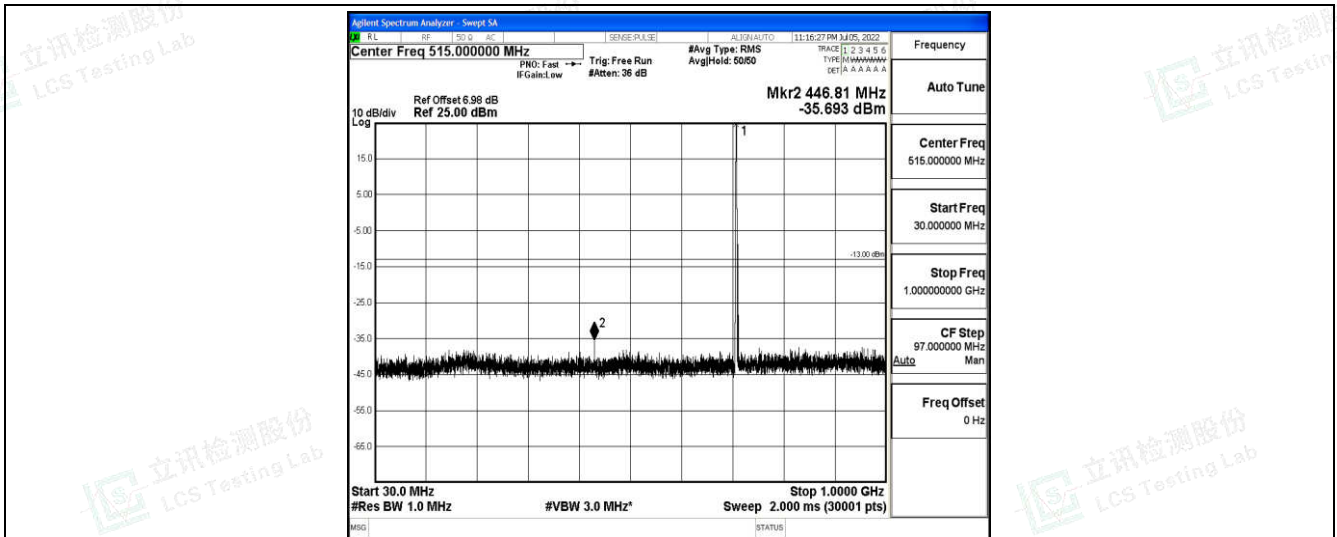
Band12-5MHz-16QAM-23155-1-0-High-30-1000--35.69-PASS
