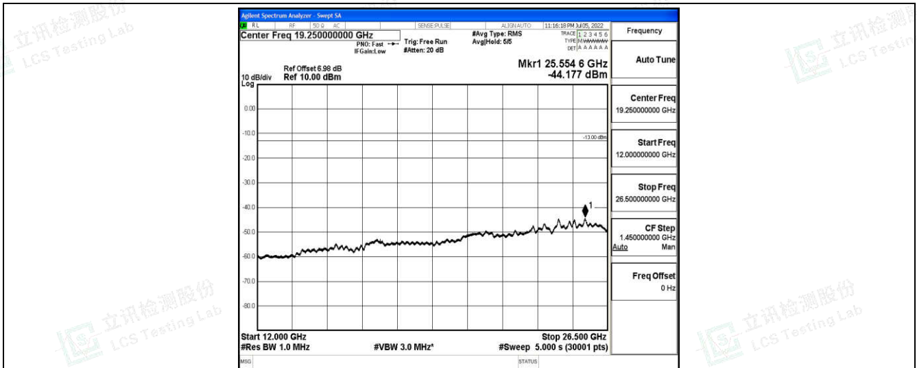
Band12-5MHz-QPSK-23155-1-0-High-12000-26500--44.18-PASS
