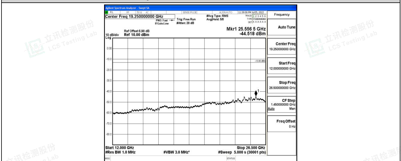
Band12-10MHz-QPSK-23095-1-0-Low-12000-26500--44.52-PASS
