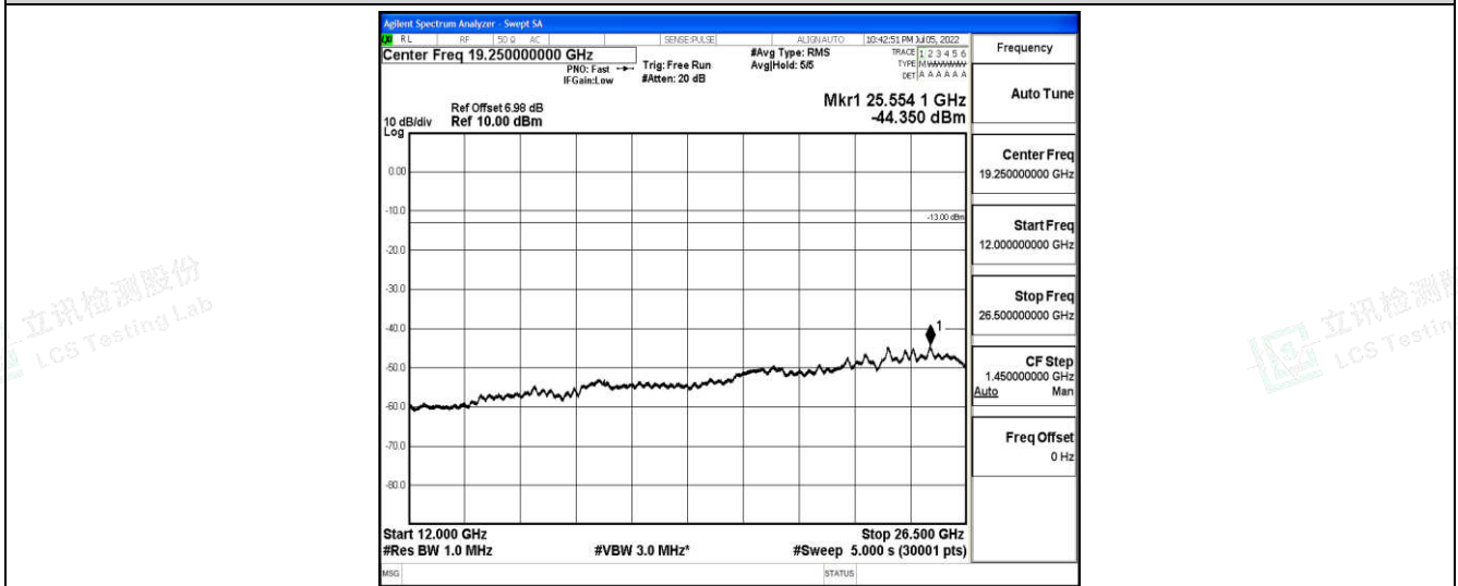
Band12-3MHz-QPSK-23025-1-0-Low-12000-26500--44.35-PASS
