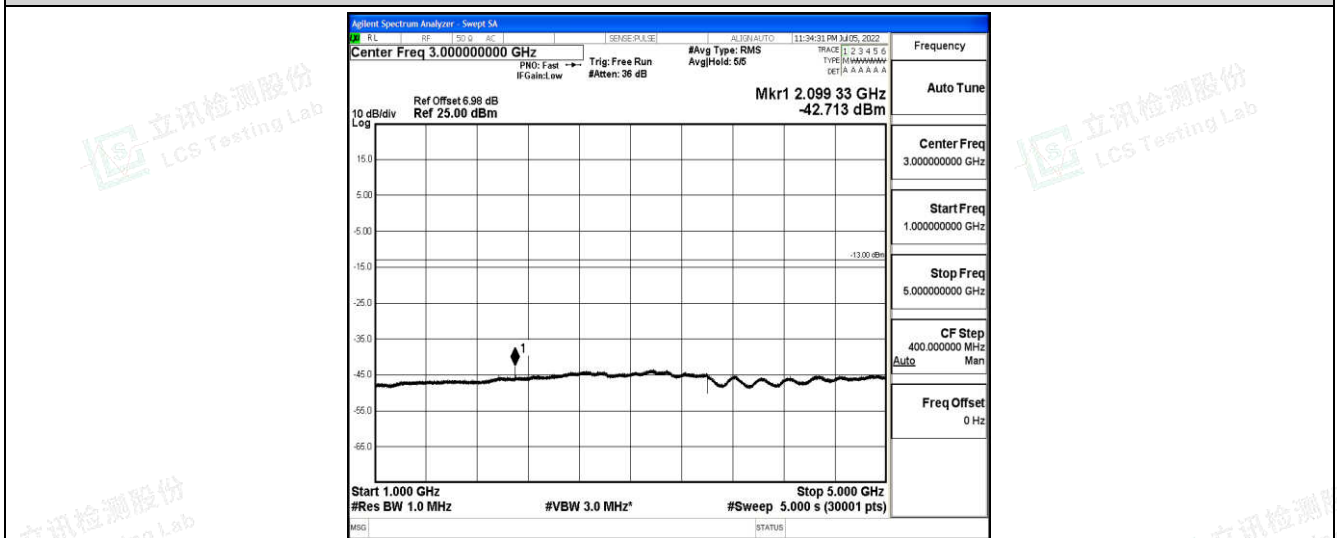
Band12-10MHz-16QAM-23060-1-0-Low-1000-5000--42.71-PASS
