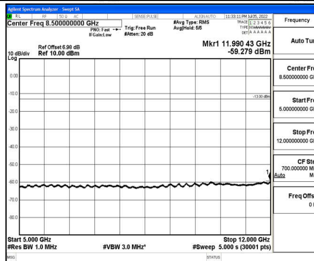
Band12-10MHz-QPSK-23060-1-0-Low-5000-12000--59.28-PASS
