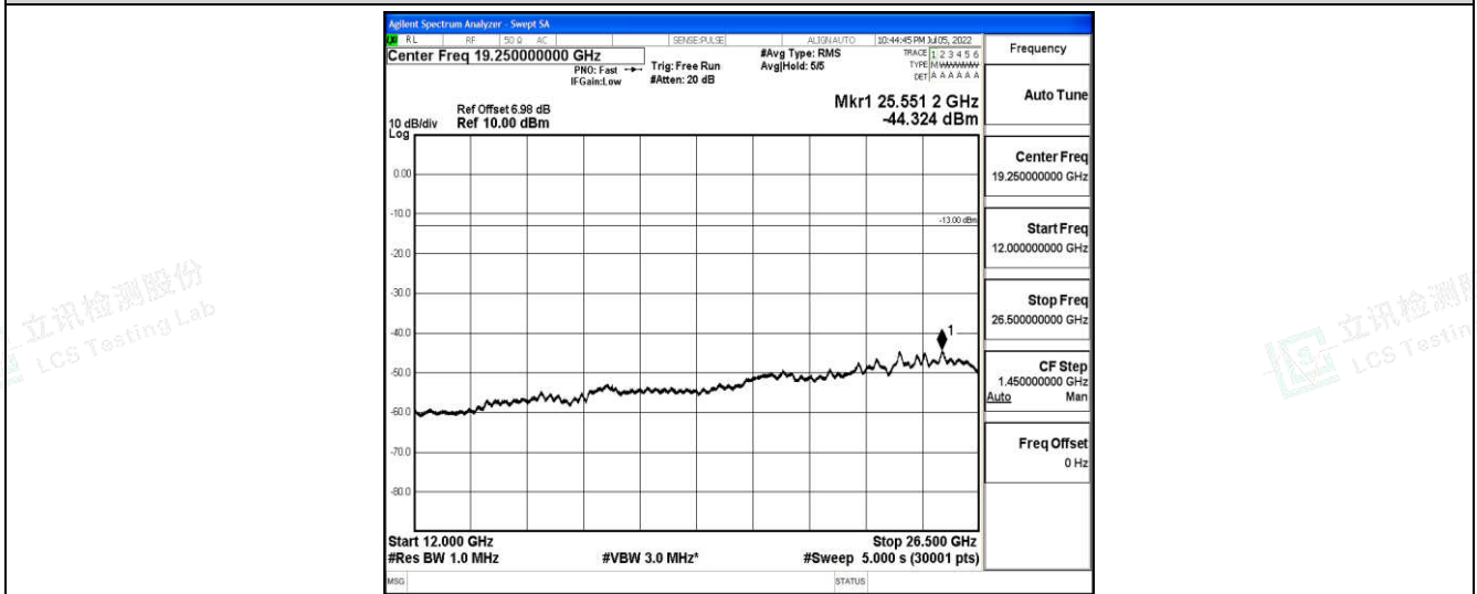
Band12-3MHz-16QAM-23025-1-0-Low-12000-26500--44.32-PASS
