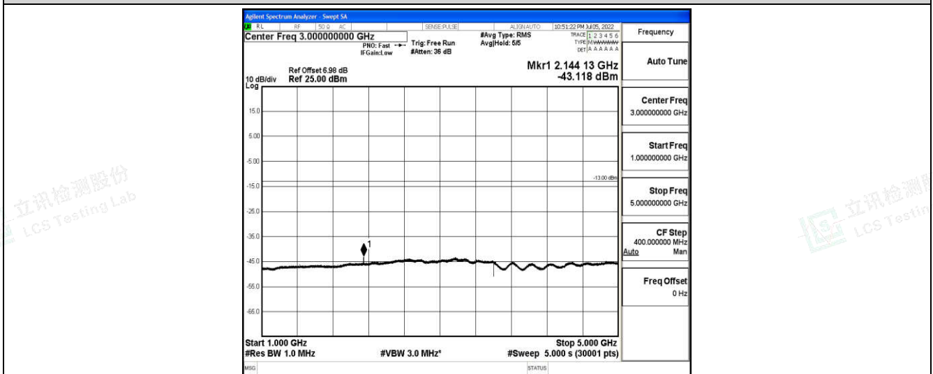
Band12-3MHz-16QAM-23165-1-0-High-1000-5000--43.12-PASS
