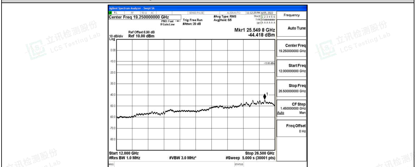
Band12-5MHz-QPSK-23095-1-0-Low-12000-26500--44.42-PASS
