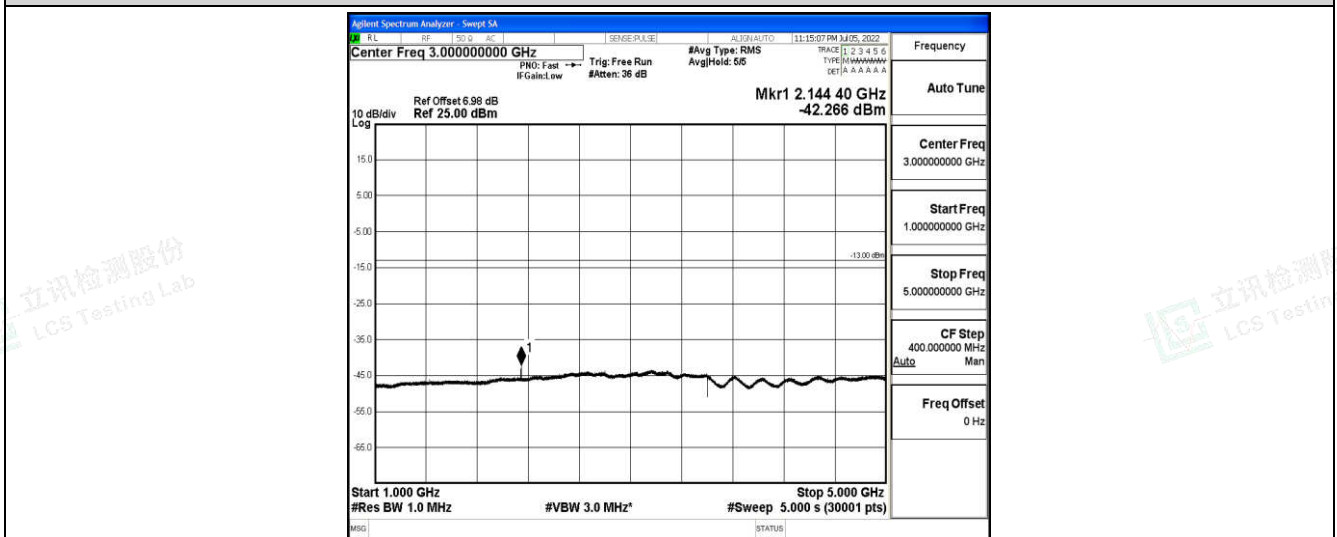
Band12-5MHz-QPSK-23155-1-0-High-1000-5000--42.27-PASS
