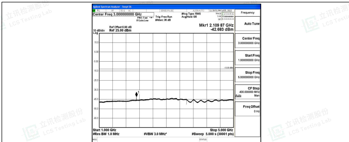
Band12-10MHz-16QAM-23095-1-0-Low-1000-5000--42.68-PASS
