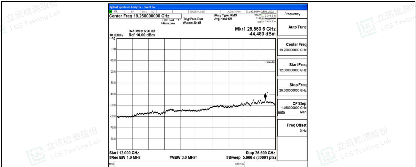
Band12-10MHz-QPSK-23130-1-0-High-12000-26500--44.48-PASS
