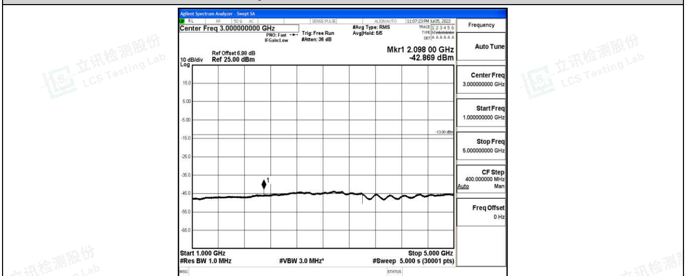
Band12-5MHz-QPSK-23035-1-0-Low-1000-5000--42.87-PASS
