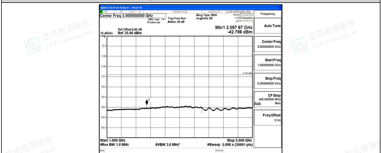
Band12-5MHz-16QAM-23035-1-0-Low-1000-5000--42.8-PASS
