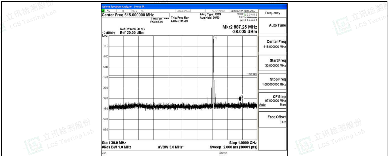
Band12-10MHz-QPSK-23130-1-0-High-30-1000--38.01-PASS
