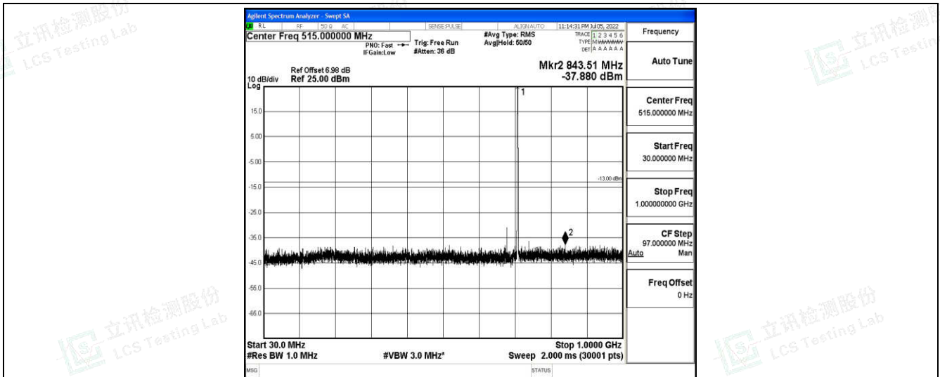
Band12-5MHz-QPSK-23155-1-0-High-30-1000--37.88-PASS
