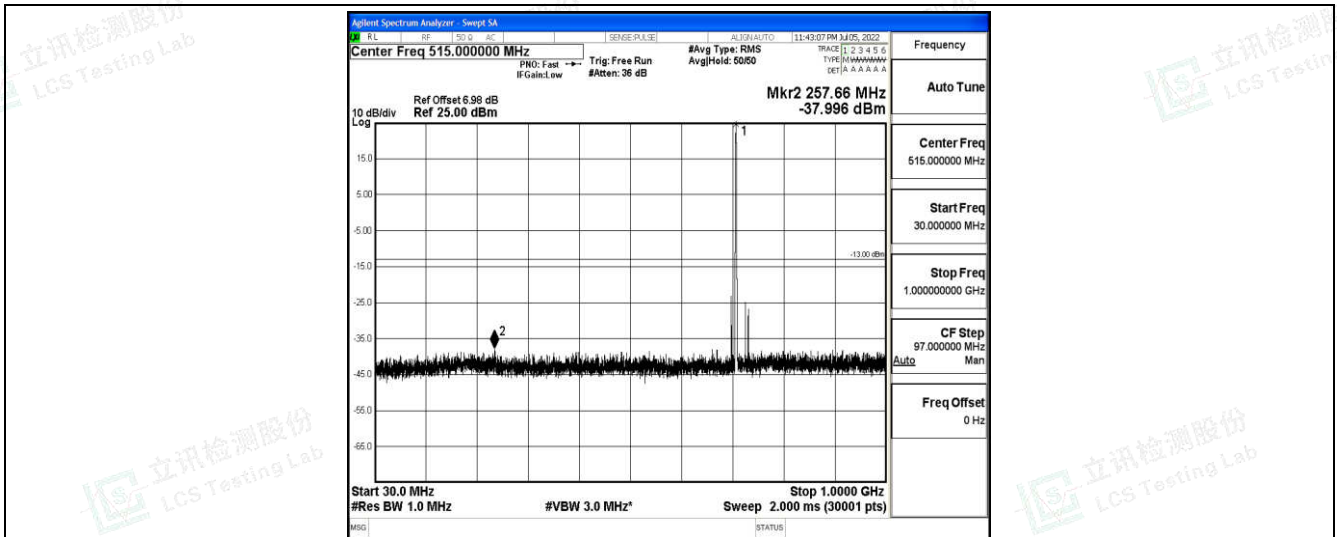
Band12-10MHz-16QAM-23130-1-0-High-30-1000--38-PASS
