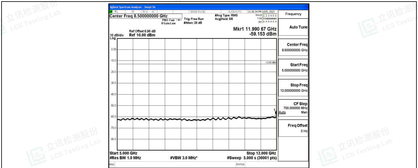
Band12-10MHz-16QAM-23060-1-0-Low-5000-12000--59.15-PASS
