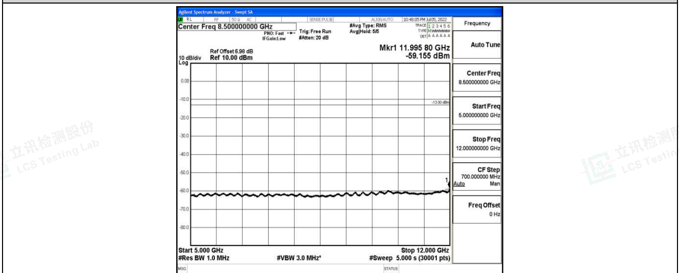
Band12-3MHz-16QAM-23095-1-0-Low-5000-12000--59.16-PASS
