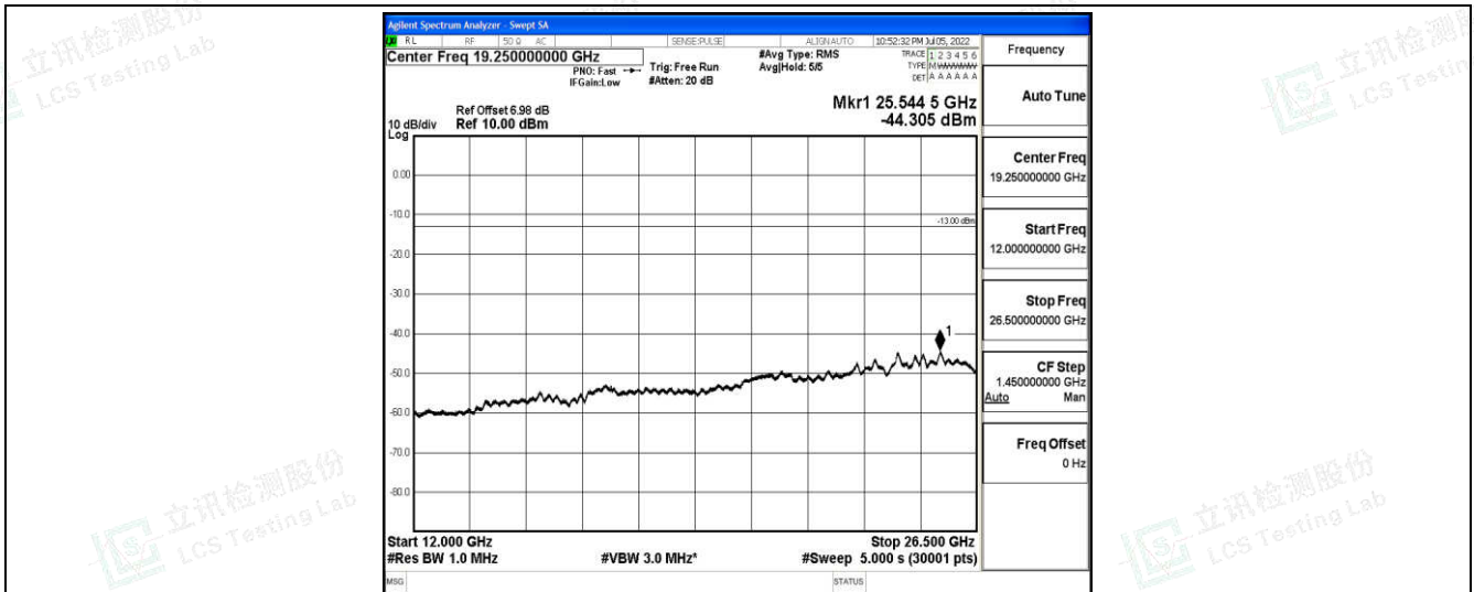
Band12-3MHz-16QAM-23165-1-0-High-12000-26500--44.31-PASS
