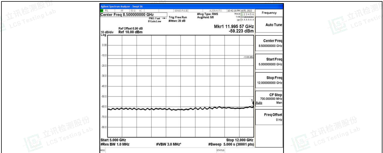
Band12-3MHz-QPSK-23025-1-0-Low-5000-12000--59.22-PASS
