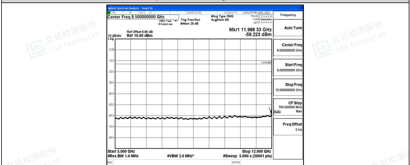
Band12-3MHz-16QAM-23165-1-0-High-5000-12000--59.22-PASS
