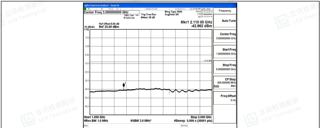
Band12-10MHz-QPSK-23095-1-0-Low-1000-5000--42.86-PASS
