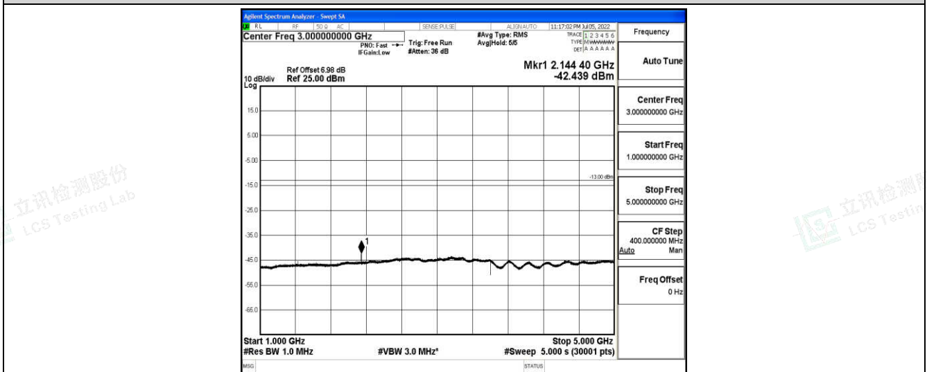
Band12-5MHz-16QAM-23155-1-0-High-1000-5000--42.44-PASS
