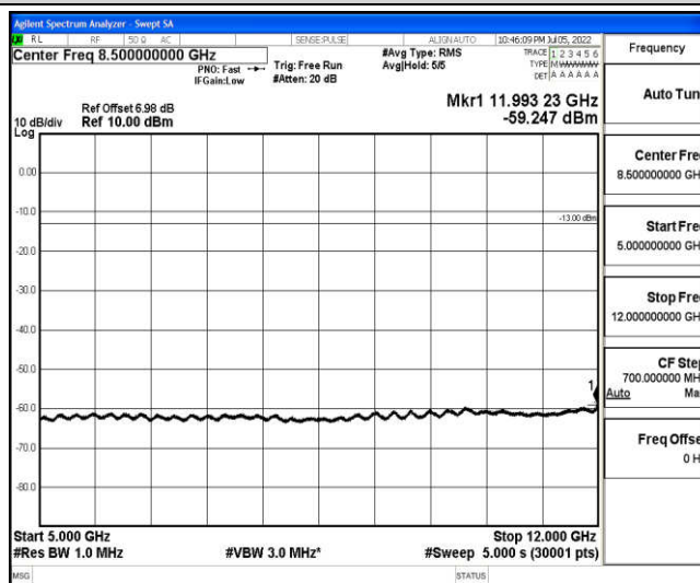
Band12-3MHz-OPSK-23095-1-0-Low-5000-12000--59.25-PASS
