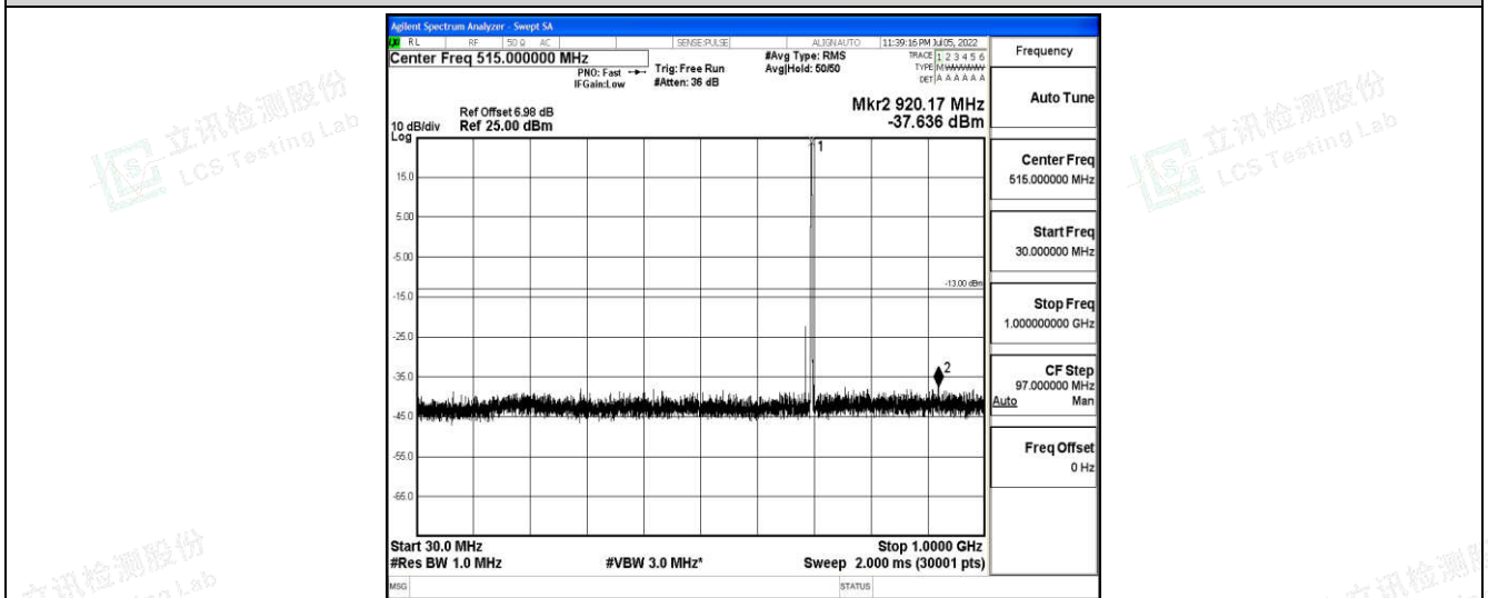
Band12-10MHz-16QAM-23095-1-0-Low-30-1000--37.64-PASS
