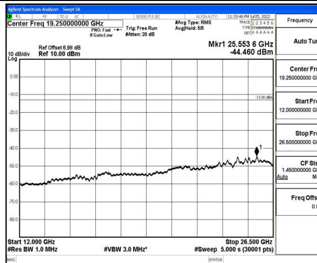
Band12-10MHz-QPSK-23060-1-0-Low-12000-26500--44.46-PASS
