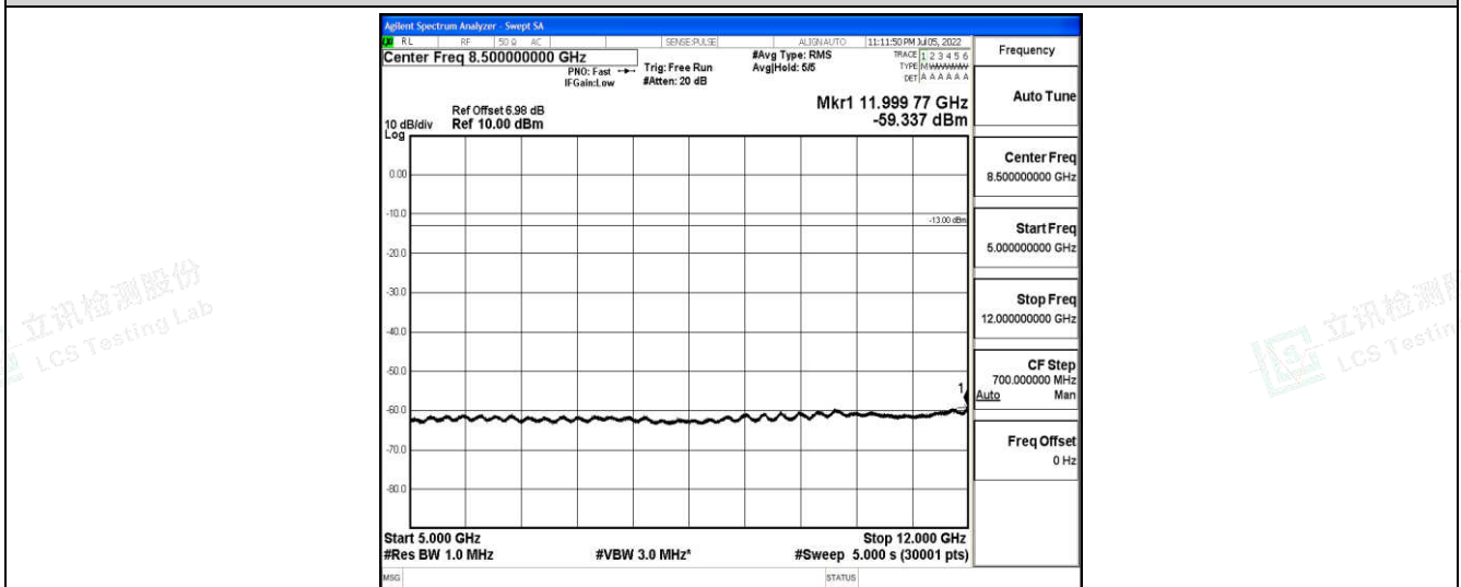
Band12-5MHz-QPSK-23095-1-0-Low-5000-12000--59.34-PASS
