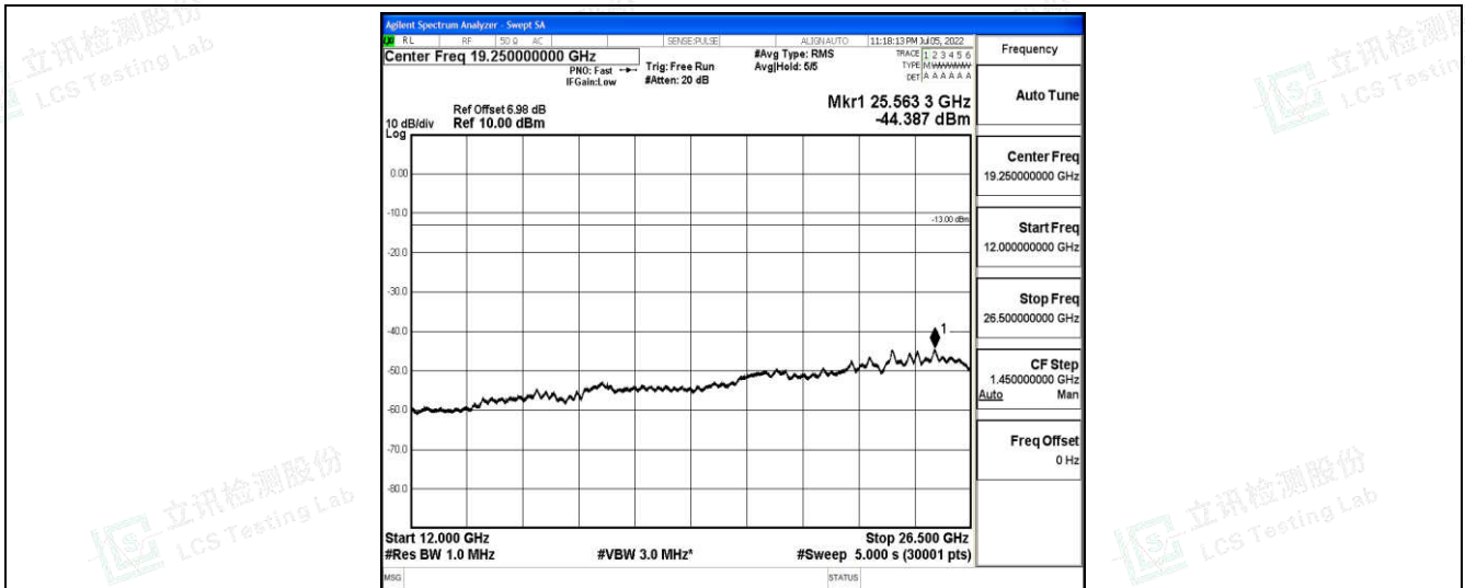
Band12-5MHz-16QAM-23155-1-0-High-12000-26500--44.39-PASS
