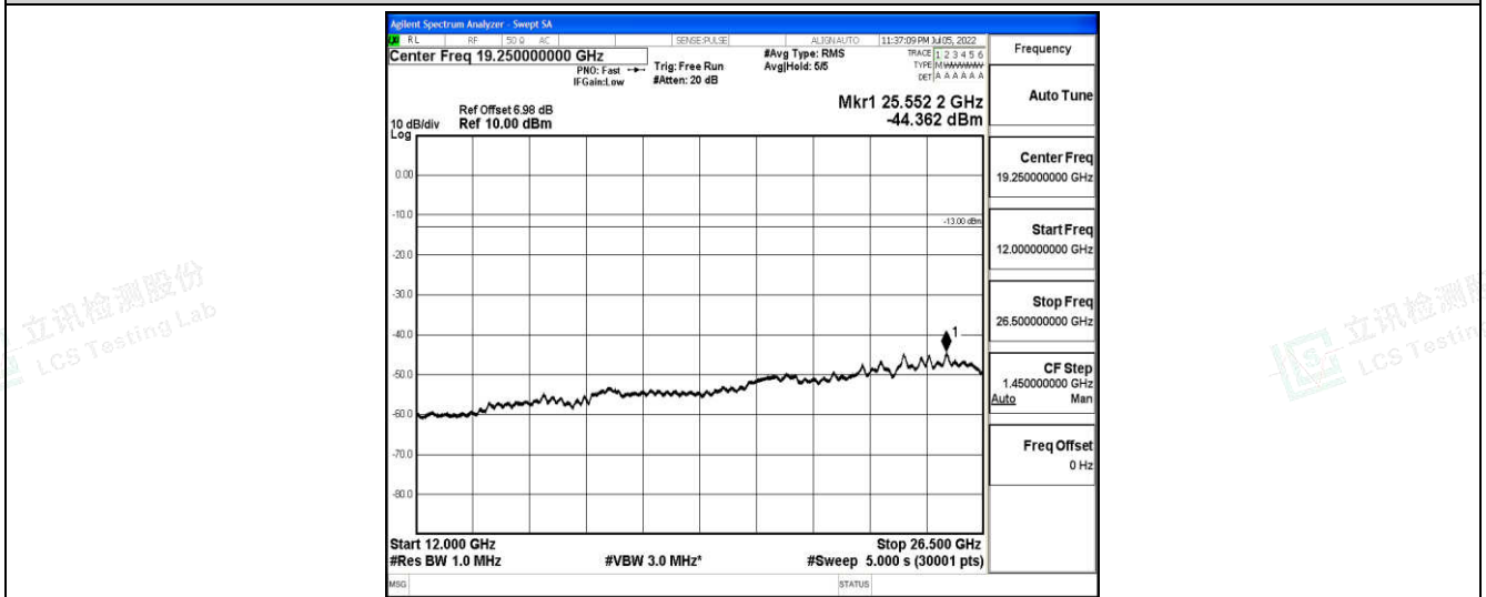
Band12-10MHz-16QAM-23060-1-0-Low-12000-26500--44.36-PASS
