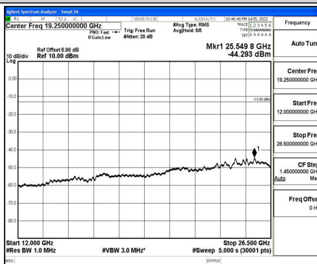
Band12-3MHz-OPSK-23095-1-0-Low-12000-26500--44.29-PASS
