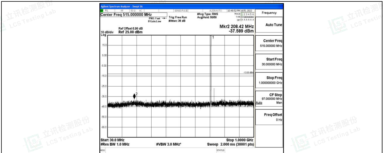
Band12-3MHz-QPSK-23165-1-0-High-30-1000--37.59-PASS
