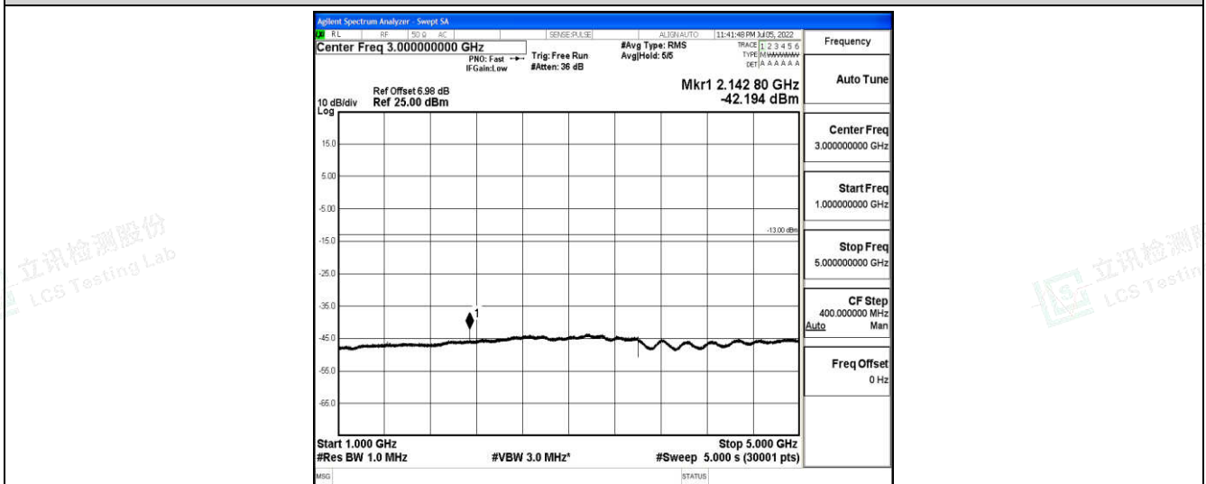
Band12-10MHz-QPSK-23130-1-0-High-1000-5000--42.19-PASS
