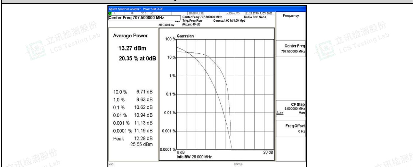
Band12-10MHz-16QAM-23095-6-0-Low-10.62-&lt;=13-PASS
