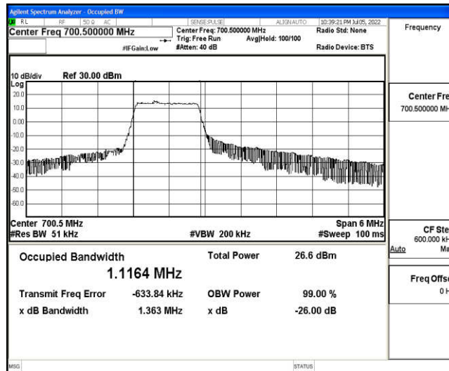
Band12-3MHz-QPSK-23025-6-0-Low-1.1164-1.363-PASS
