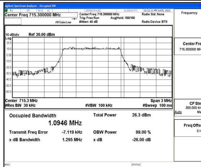
Band12-1.4MHz-QPSK-23173-6-0-High-1.0946-1.295-PASS
