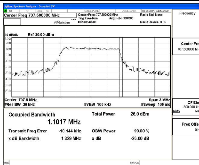
Band12-1.4MHz-QPSK-23095-6-0-Low-1.1017-1.329-PASS
