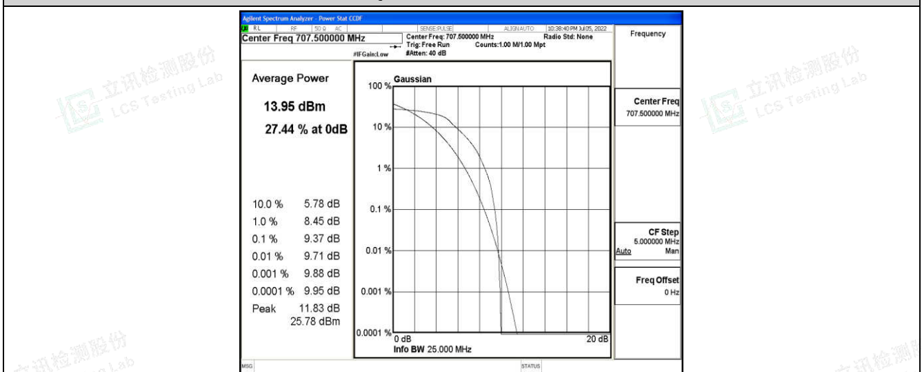
Band12-3MHz-16QAM-23095-6-0-Low-9.37-&lt;=13-PASS
