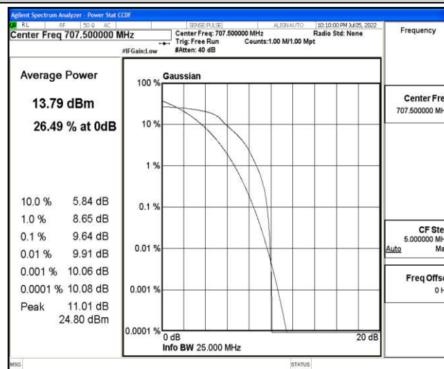
Band12-1.4MHz-16QAM-23095-6-0-Low-9.64-&lt;=13-PASS
