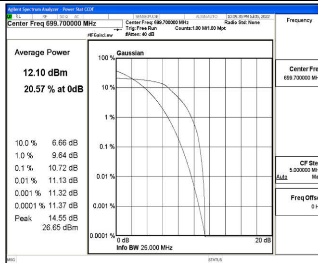
Band12-1.4MHz-16QAM-23017-6-0-Low-10.72-&lt;=13-PASS
