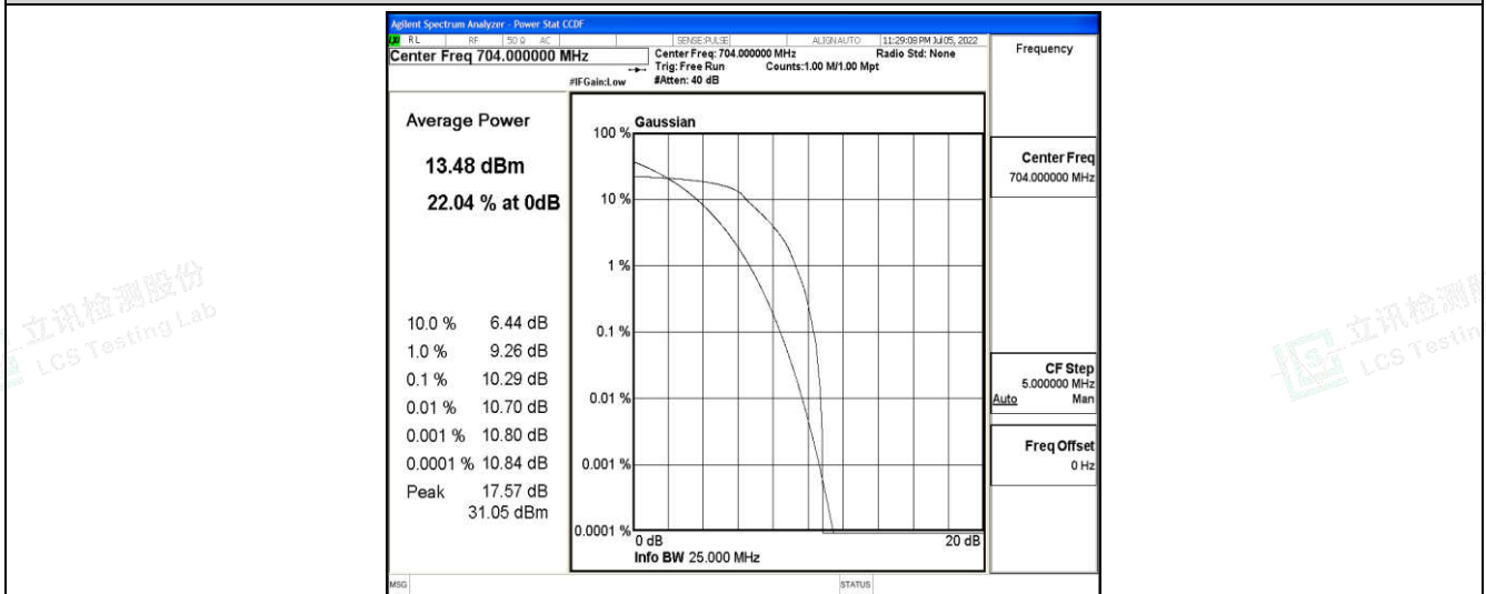
Band12-10MHz-QPSK-23060-6-0-Low-10.29-&lt;=13-PASS
