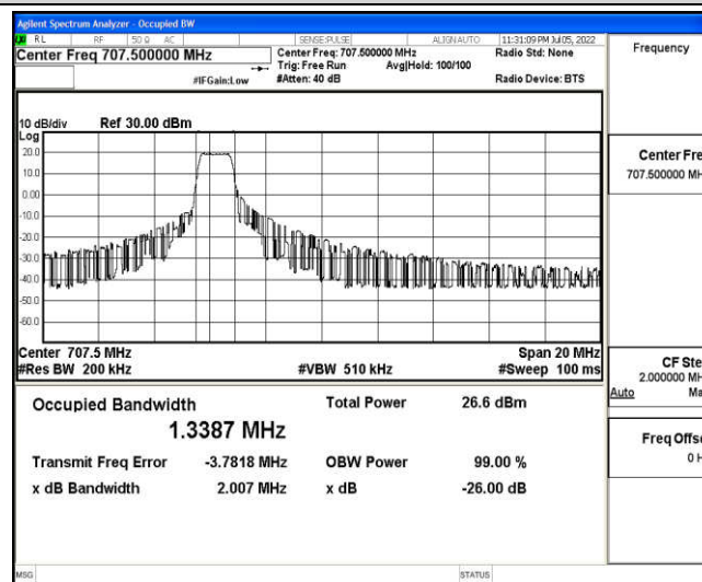
Band12-10MHz-16QAM-23095-6-0-Low-1.3387-2.007-PASS
