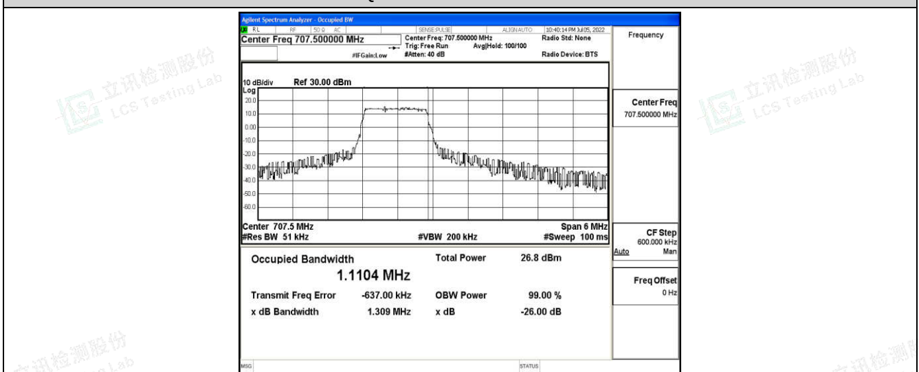
Band12-3MHz-16QAM-23095-6-0-Low-1.1104-1.309-PASS
