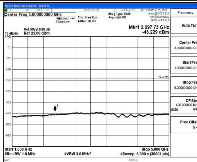
Band12-1.4MHz-QPSK-23017-1-0-Low-1000-5000--43.23-PASS
