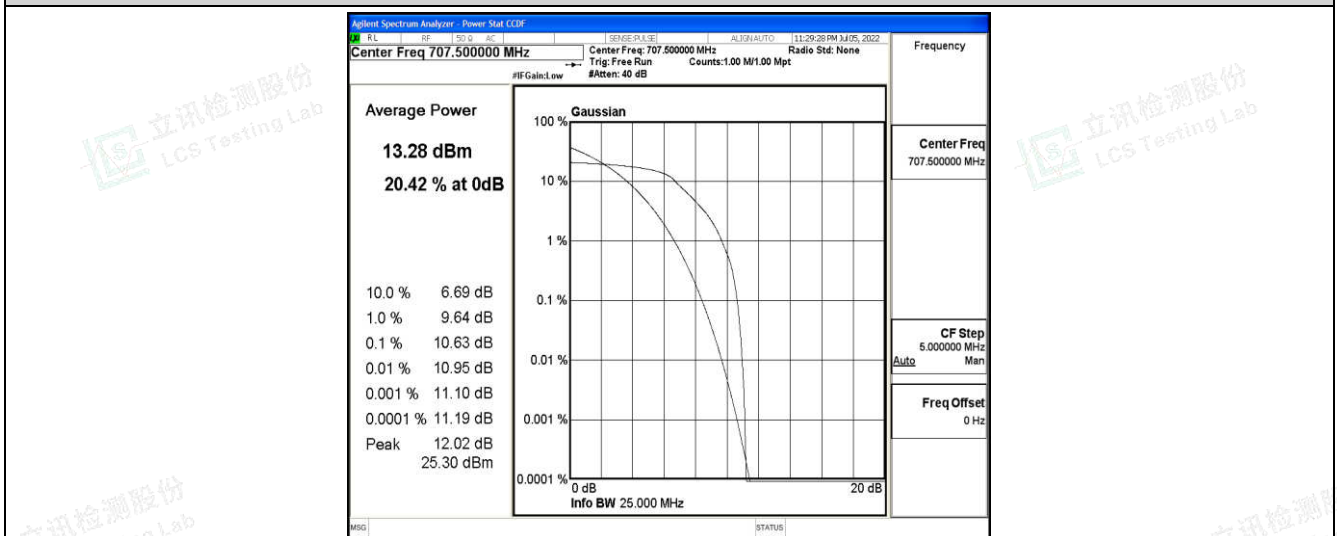
Band12-10MHz-QPSK-23095-6-0-Low-10.63-&lt;=13-PASS
