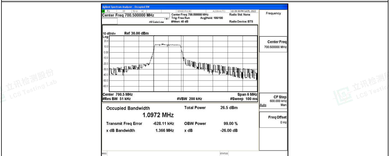
Band12-3MHz-16QAM-23025-6-0-Low-1.0972-1.366-PASS
