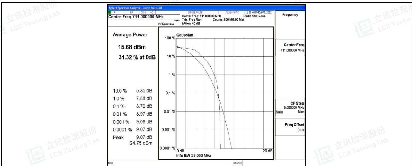
Band12-10MHz-QPSK-23130-6-0-High-8.70-&lt;=13-PASS
