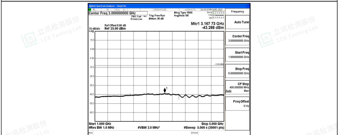
Band12-1.4MHz-16QAM-23017-1-0-Low-1000-5000--43.29-PASS
