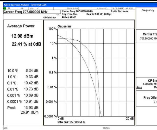
Band12-1.4MHz-QPSK-23095-6-0-Low-10.42-13-PASS
