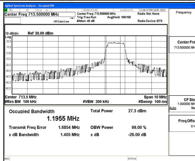
Band12-5MHz-16QAM-23155-6-0-High-1.1955-1.405-PASS
