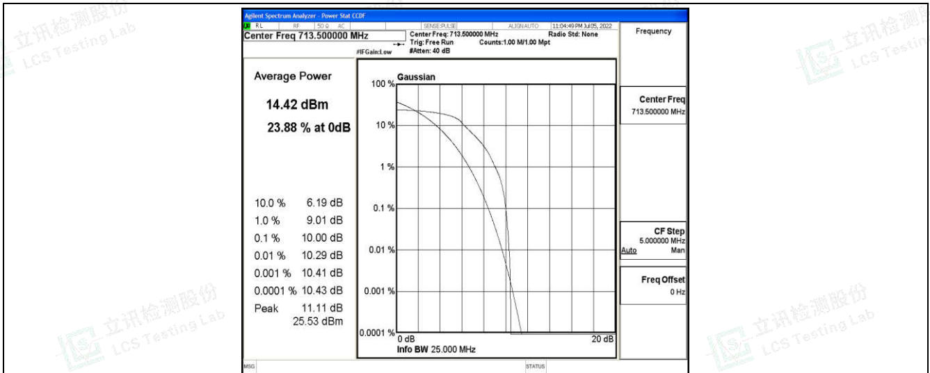
Band12-5MHz-16QAM-23155-6-0-High-10.00-&lt;=13-PASS
