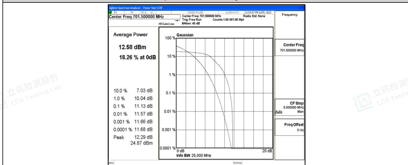
Band12-5MHz-16QAM-23035-6-0-Low-11.13-&lt;=13-PASS
