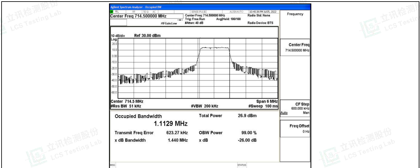
Band12-3MHz-QPSK-23165-6-0-High-1.1129-1.440-PASS
