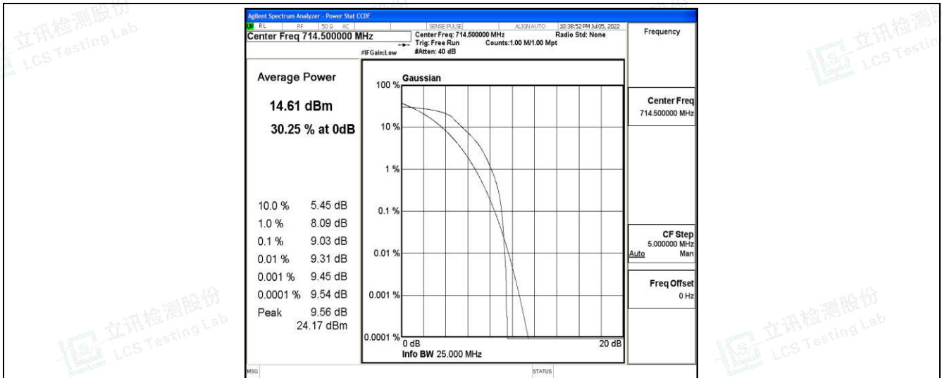
Band12-3MHz-QPSK-23165-6-0-High-9.03-&lt;=13-PASS
