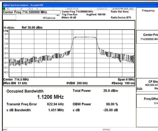
Band12-3MHz-16QAM-23165-6-0-High-1.1206-1.451-PASS
