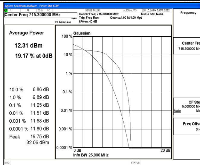
Band12-1.4MHz-QPSK-23173-6-0-High-11.05-&lt;=13-PASS
