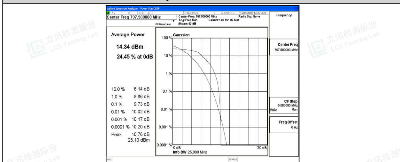
Band12-5MHz-16QAM-23095-6-0-Low-9.73-&lt;=13-PASS
