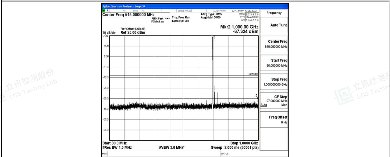
Band12-3MHz-QPSK-23025-1-0-Low-30-1000--37.32-PASS
