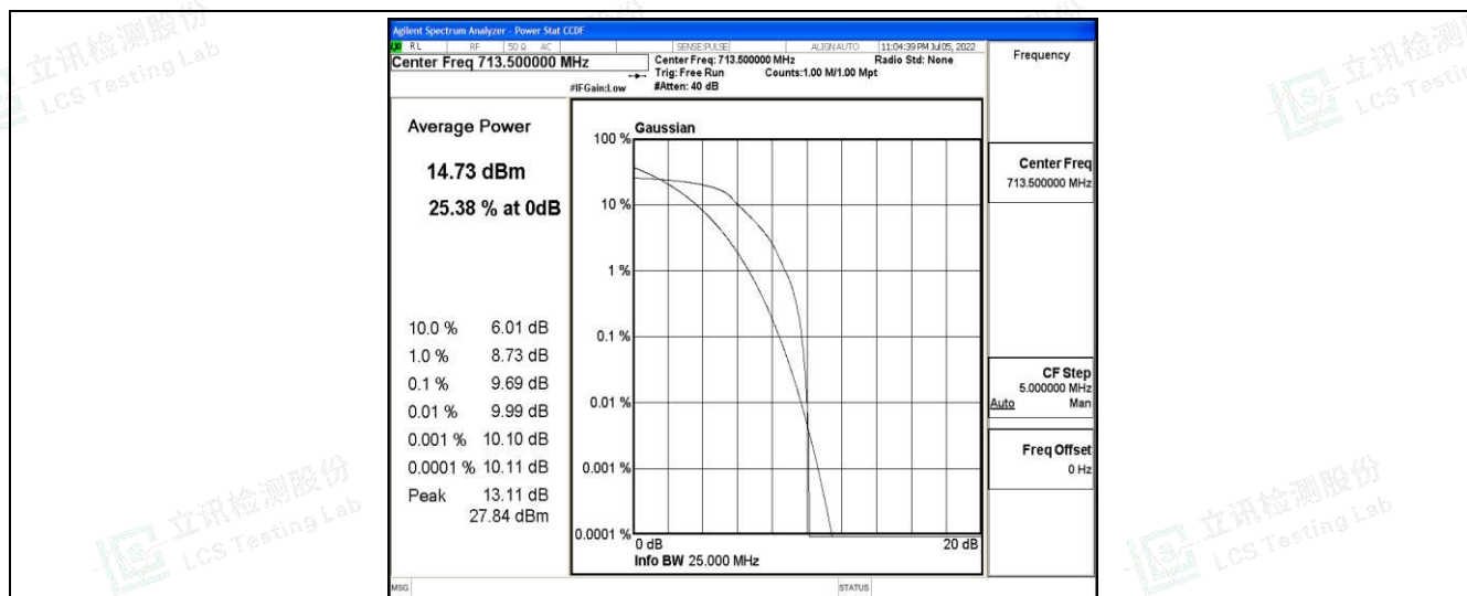
Band12-5MHz-QPSK-23155-6-0-High-9.69-&lt;=13-PASS
