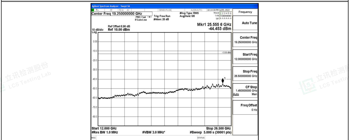
Band12-1.4MHz-QPSK-23017-1-0-Low-12000-26500--44.45-PASS
