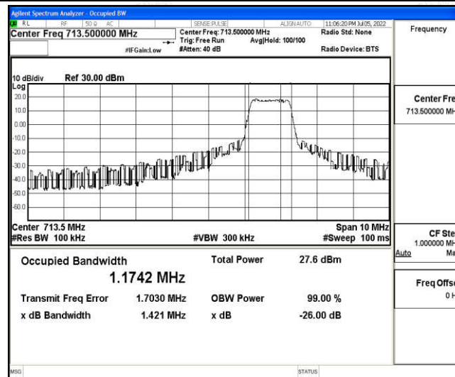
Band12-5MHz-QPSK-23155-6-0-High-1.1742-1.421-PASS
