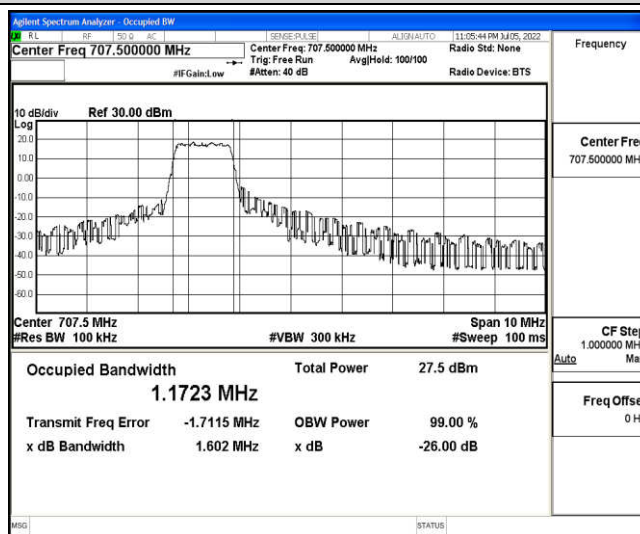
Band12-5MHz-QPSK-23095-6-0-Low-1.1723-1.602-PASS
