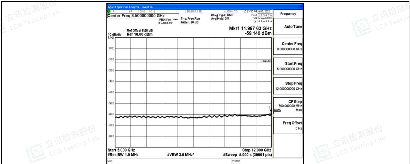
Band12-1.4MHz-QPSK-23017-1-0-Low-5000-12000--59.14-PASS
