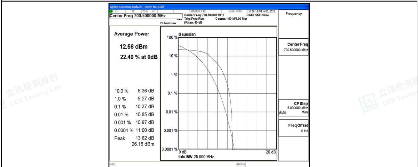
Band12-3MHz-16QAM-23025-6-0-Low-10.37-&lt;=13-PASS
