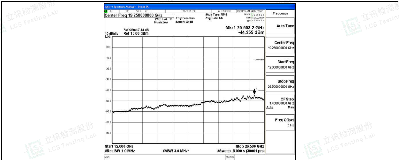
Band5-5MHz-16QAM-20525-1-0-Low-12000-26500--44.26-PASS
