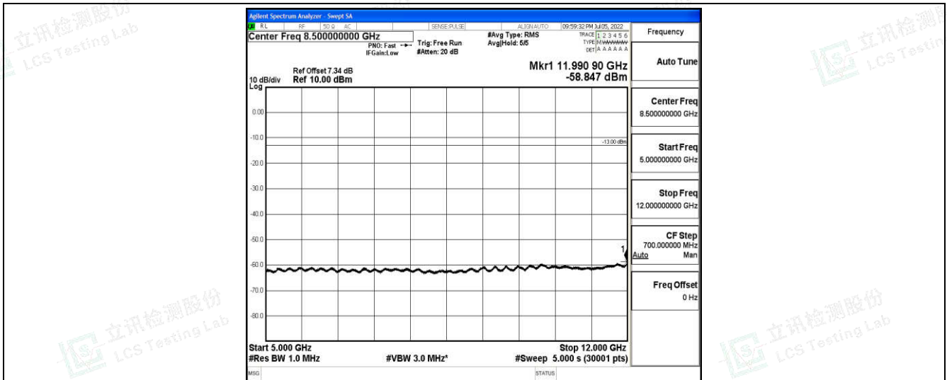
Band5-10MHz-QPSK-20600-1-0-High-5000-12000--58.85-PASS
