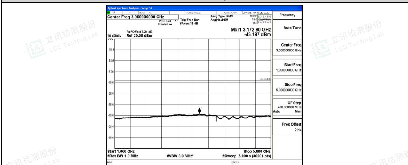
Band5-10MHz-QPSK-20600-1-0-High-1000-5000--43.19-PASS
