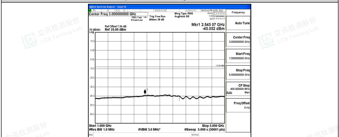
Band5-3MHz-QPSK-20635-1-0-High-1000-5000--43.03-PASS
