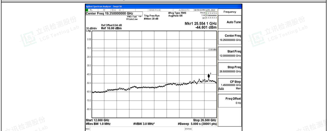
Band5-3MHz-16QAM-20415-1-0-Low-12000-26500--44.6-PASS
