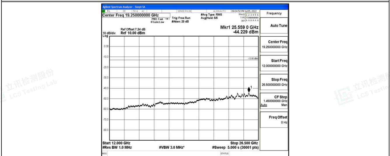
Band5-3MHz-QPSK-20635-1-0-High-12000-26500--44.23-PASS
