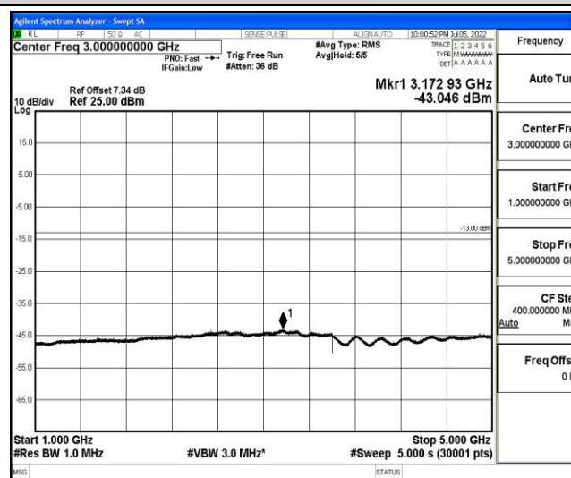
Band5-10MHz-16QAM-20600-1-0-High-1000-5000--43.05-PASS
