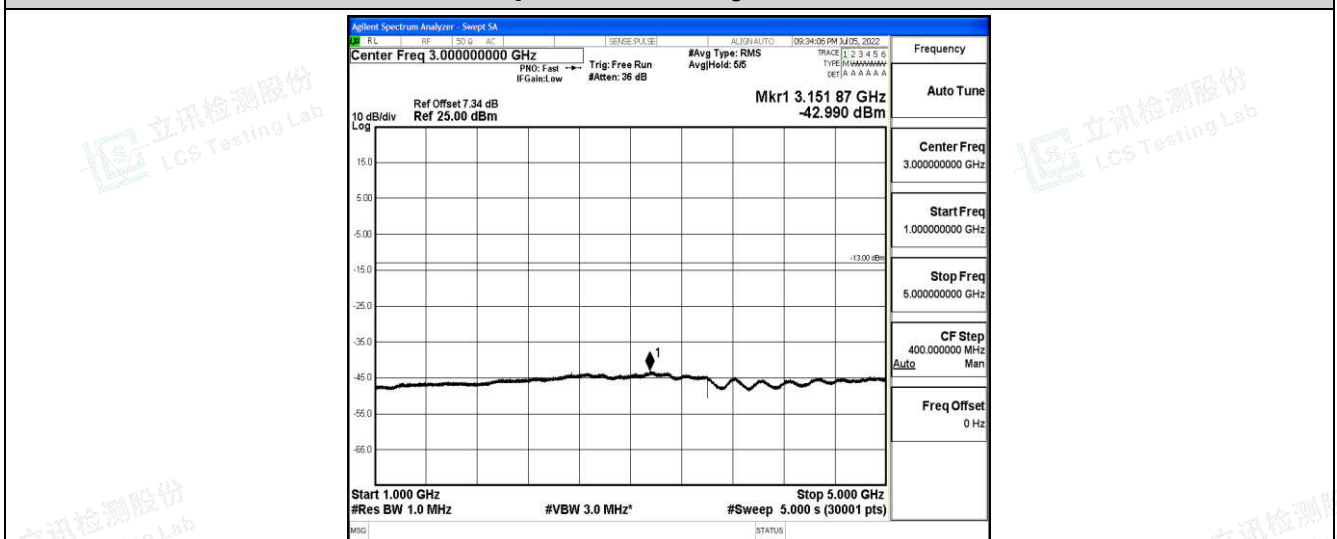
Band5-5MHz-16QAM-20625-1-0-High-1000-5000--42.99-PASS
