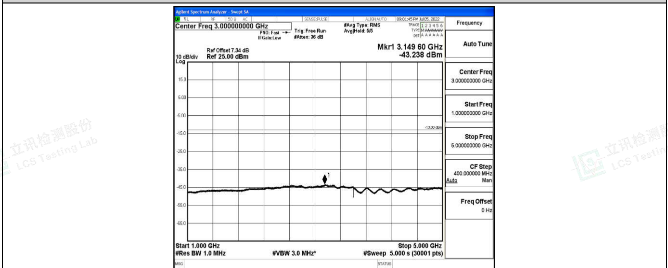
Band5-3MHz-16QAM-20525-1-0-Low-1000-5000--43.24-PASS
