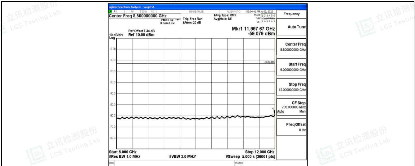
Band5-5MHz-16QAM-20625-1-0-High-5000-12000--59.08-PASS
