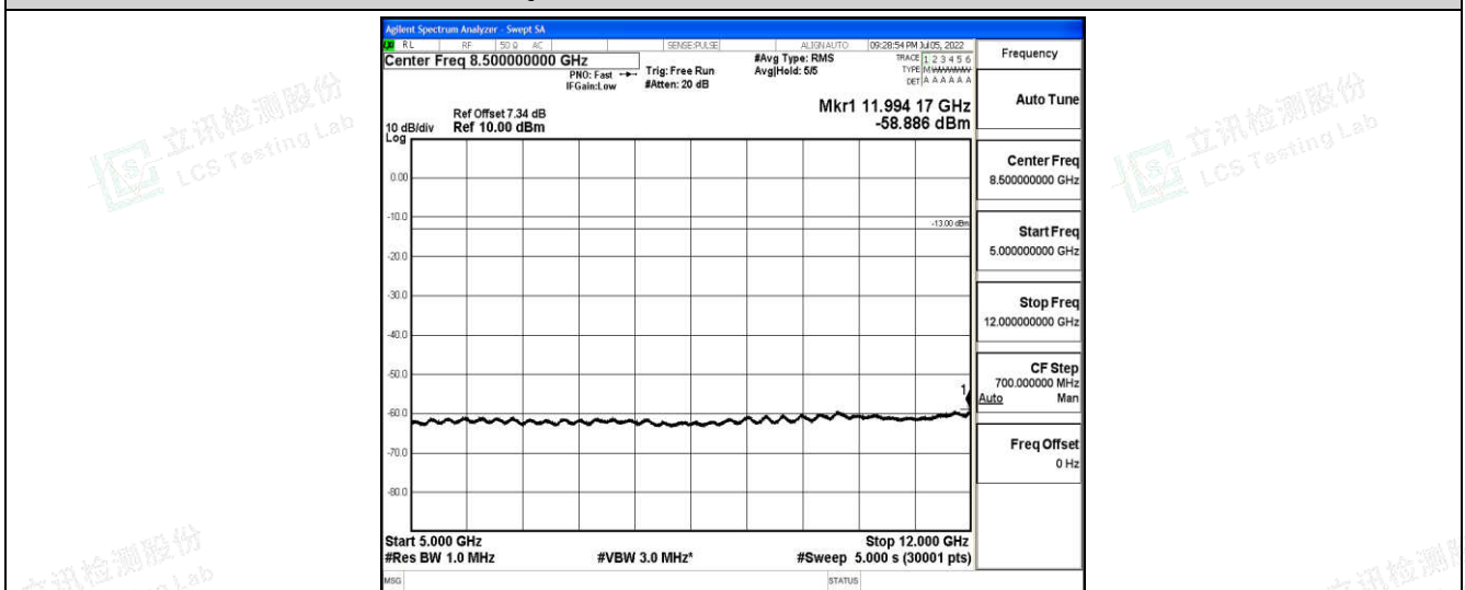
Band5-5MHz-QPSK-20525-1-0-Low-5000-12000--58.89-PASS
