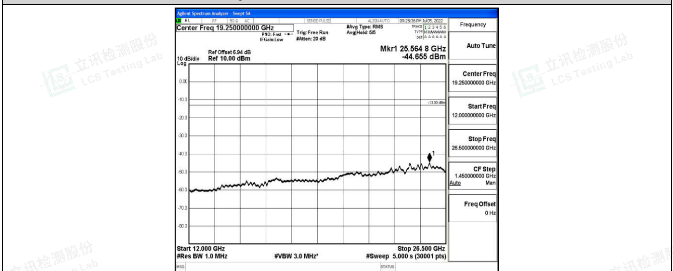
Band5-5MHz-QPSK-20425-1-0-Low-12000-26500--44.66-PASS
