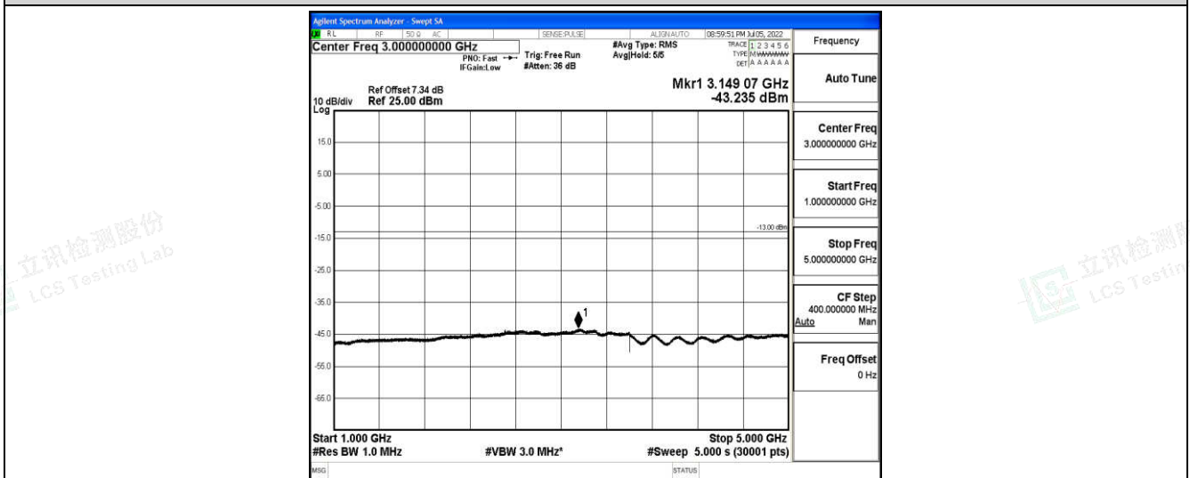
Band5-3MHz-QPSK-20525-1-0-Low-1000-5000--43.24-PASS
