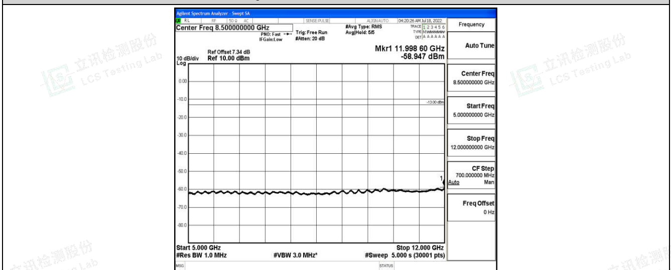
Band5-10MHz-16QAM-20525-1-0-Low-5000-12000--58.95-PASS
