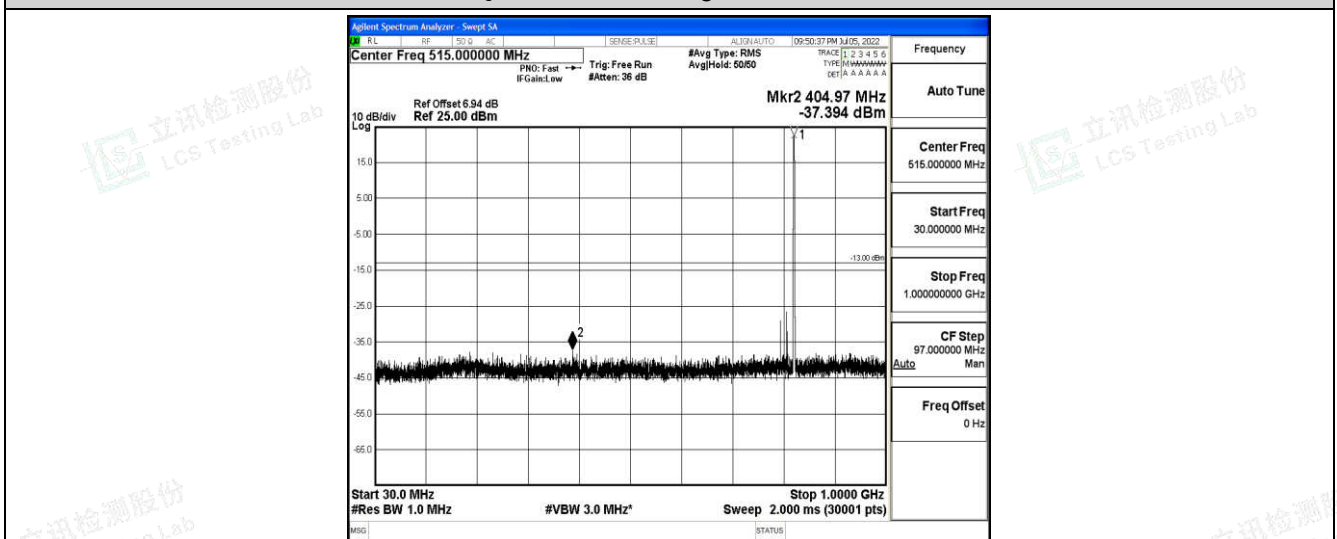
Band5-10MHz-QPSK-20450-1-0-Low-30-1000--37.39-PASS
