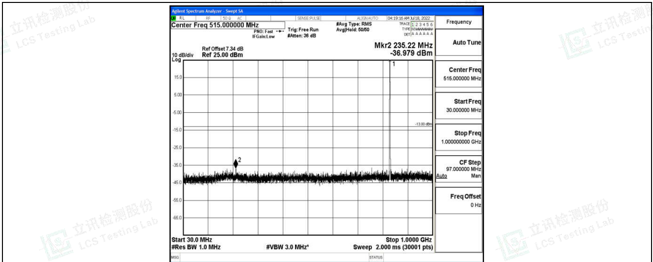
Band5-10MHz-16QAM-20525-1-0-Low-30-1000--36.98-PASS
