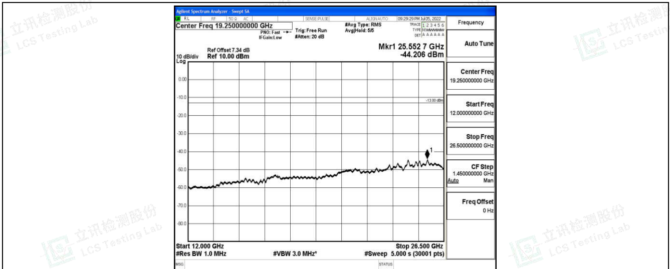
Band5-5MHz-QPSK-20525-1-0-Low-12000-26500--44.21-PASS
