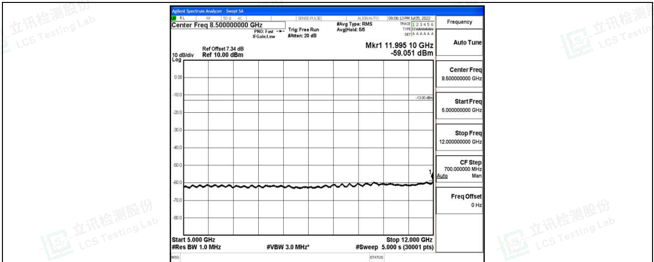
Band5-3MHz-16QAM-20635-1-0-High-5000-12000--59.05-PASS
