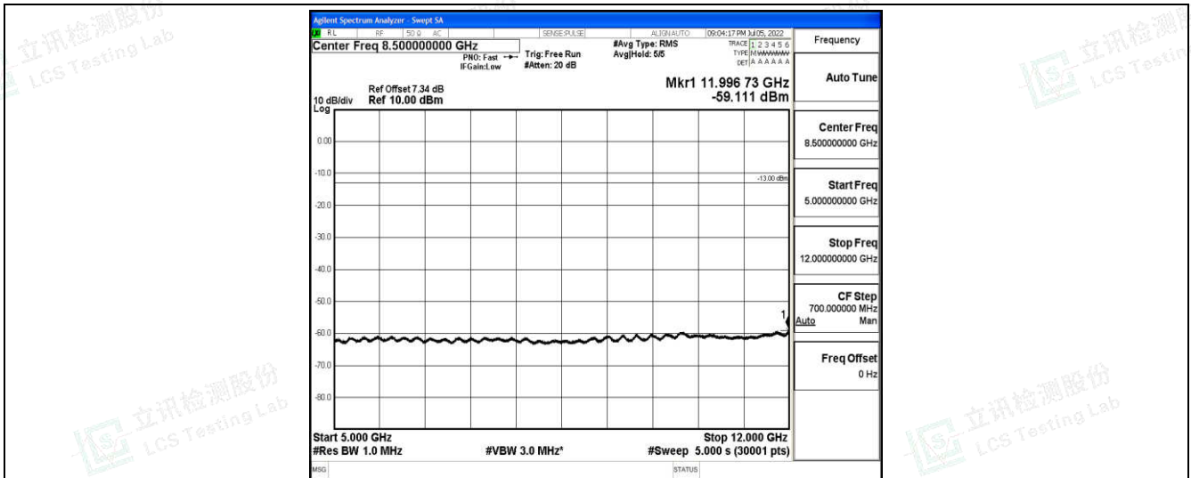
Band5-3MHz-QPSK-20635-1-0-High-5000-12000--59.11-PASS
