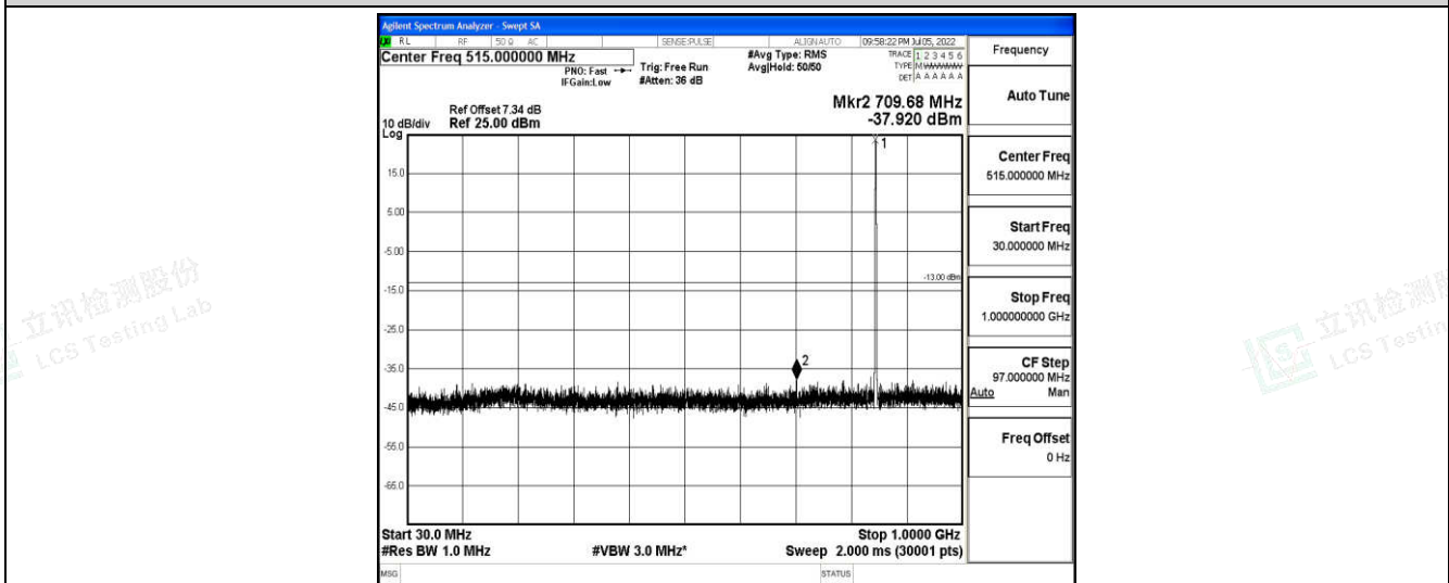
Band5-10MHz-QPSK-20600-1-0-High-30-1000--37.92-PASS
