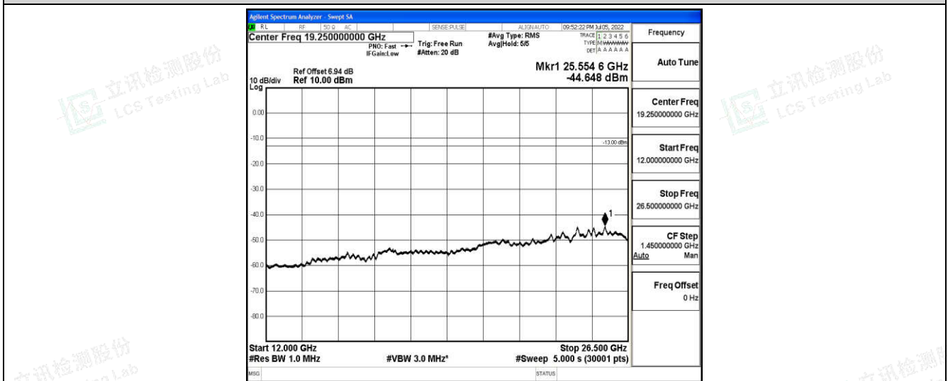
Band5-10MHz-QPSK-20450-1-0-Low-12000-26500--44.65-PASS
