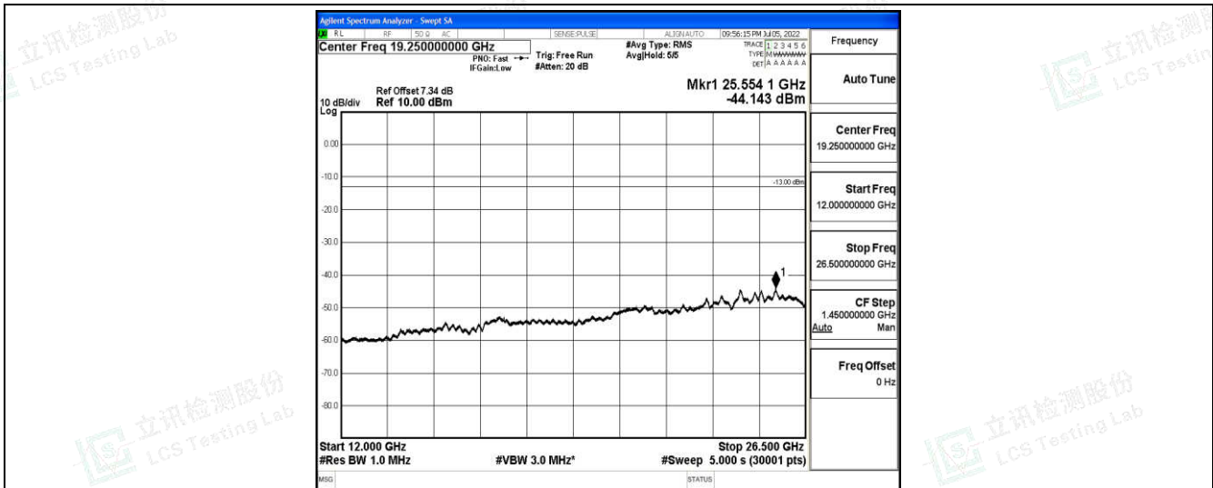
Band5-10MHz-QPSK-20525-1-0-Low-12000-26500--44.14-PASS
