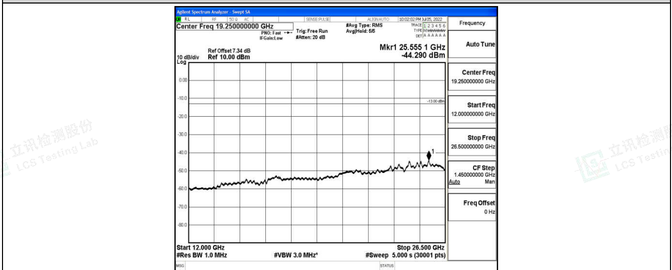
Band5-10MHz-16QAM-20600-1-0-High-12000-26500--44.29-PASS
