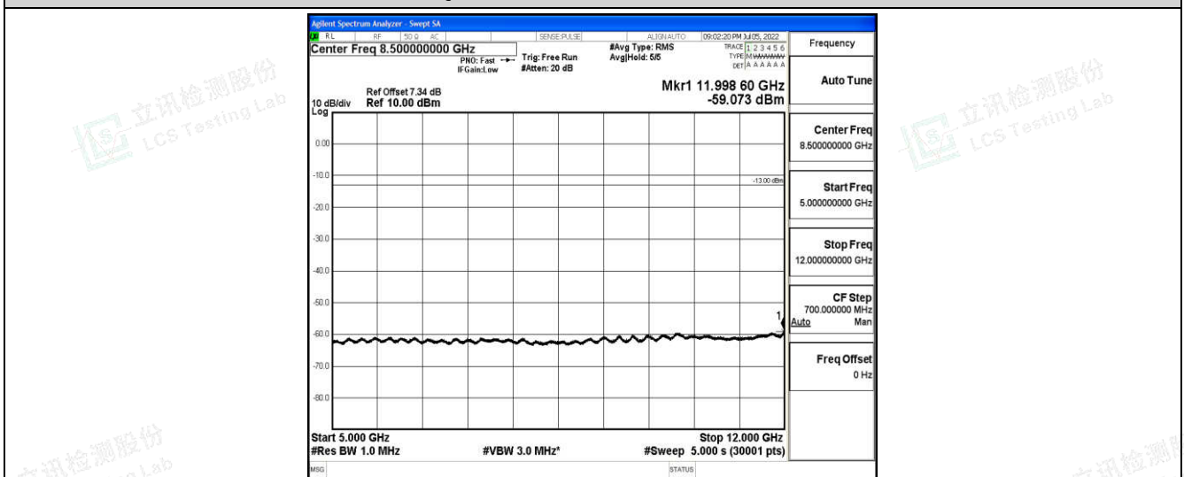
Band5-3MHz-16QAM-20525-1-0-Low-5000-12000--59.07-PASS
