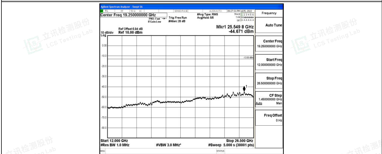
Band5-5MHz-16QAM-20425-1-0-Low-12000-26500--44.67-PASS
