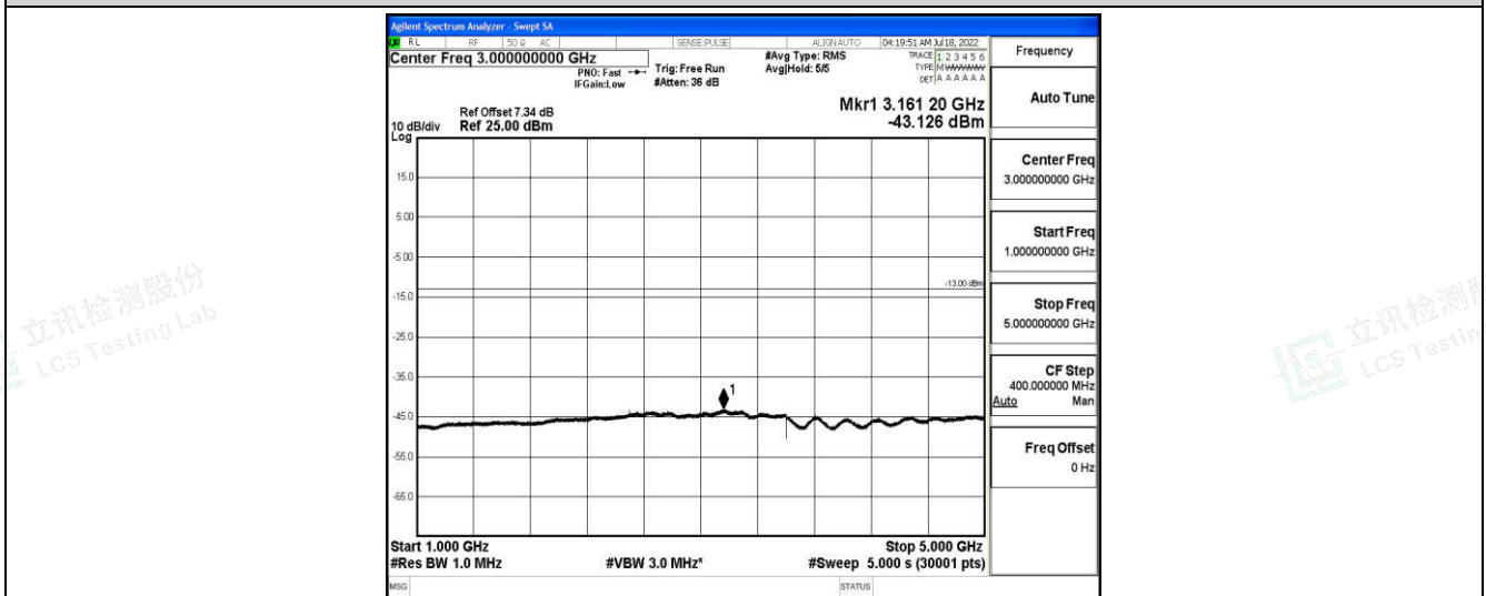
Band5-10MHz-16QAM-20525-1-0-Low-1000-5000--43.13-PASS
