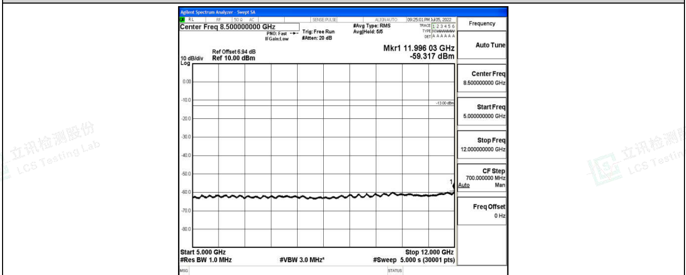
Band5-5MHz-QPSK-20425-1-0-Low-5000-12000--59.32-PASS
