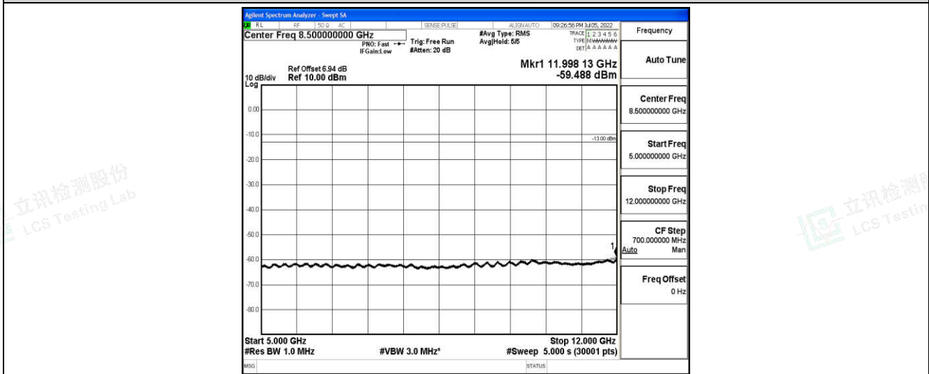
Band5-5MHz-16QAM-20425-1-0-Low-5000-12000--59.49-PASS
