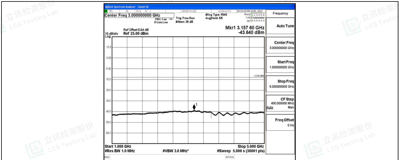
Band5-5MHz-QPSK-20425-1-0-Low-1000-5000--43.64-PASS
