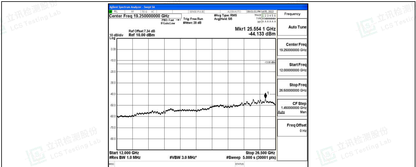
Band5-3MHz-QPSK-20525-1-0-Low-12000-26500--44.13-PASS
