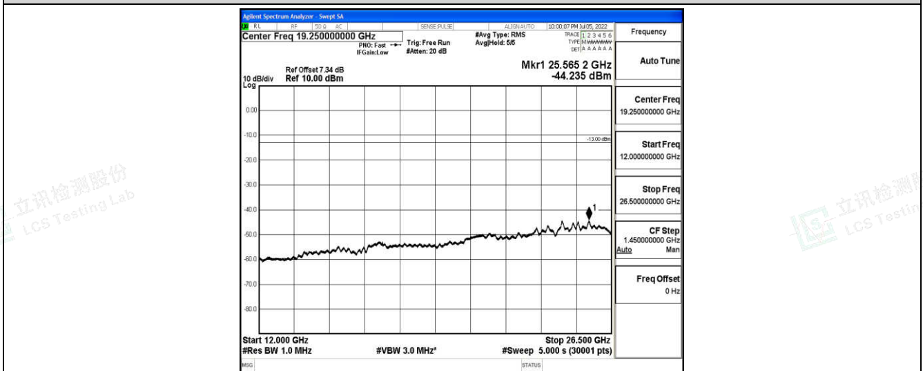
Band5-10MHz-QPSK-20600-1-0-High-12000-26500--44.24-PASS
