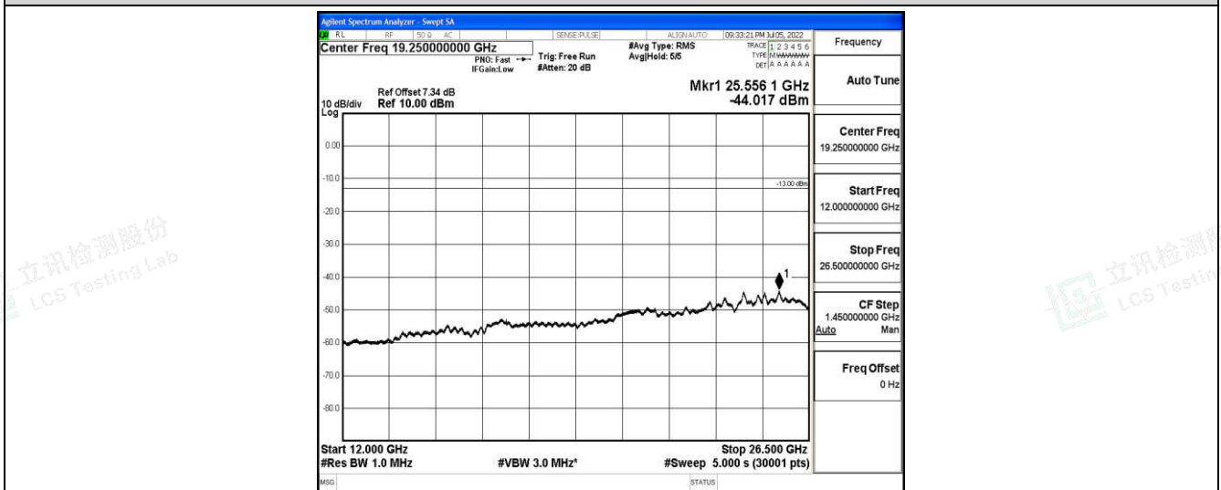
Band5-5MHz-QPSK-20625-1-0-High-12000-26500--44.02-PASS
