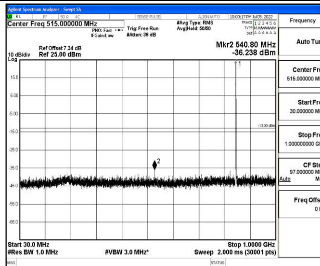
Band5-10MHz-16QAM-20600-1-0-High-30-1000--36.24-PASS
