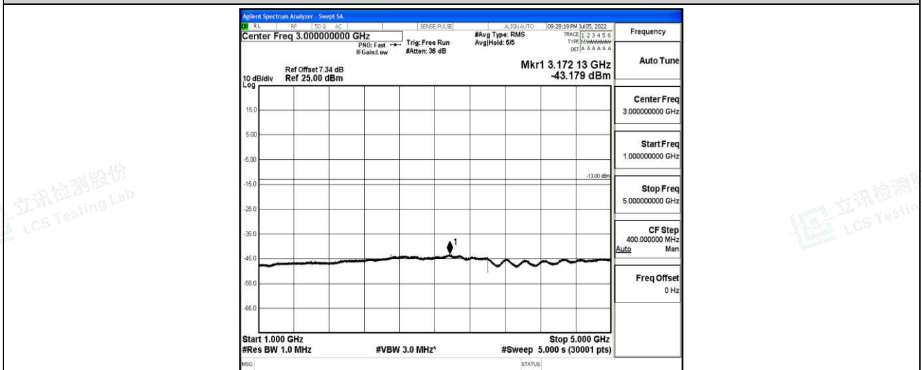
Band5-5MHz-QPSK-20525-1-0-Low-1000-5000--43.18-PASS
