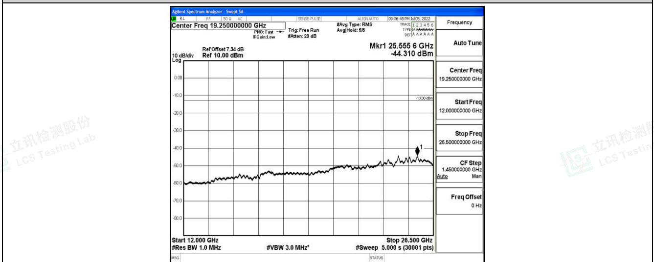
Band5-3MHz-16QAM-20635-1-0-High-12000-26500--44.31-PASS
