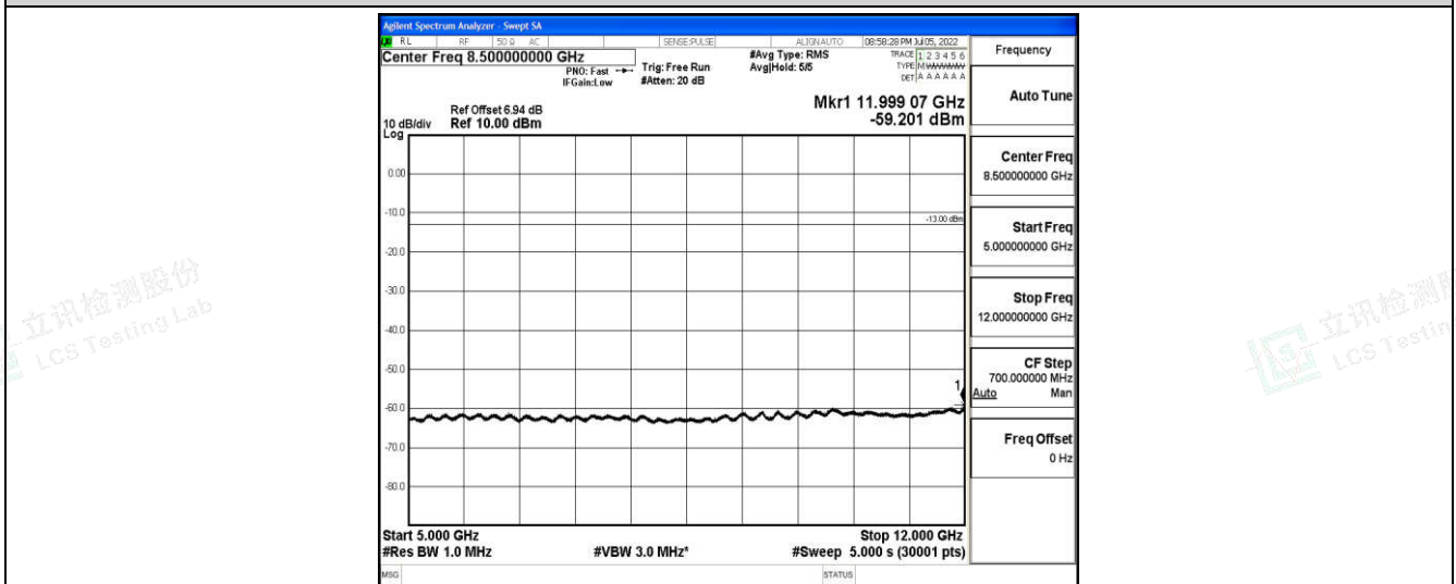
Band5-3MHz-16QAM-20415-1-0-Low-5000-12000--59.2-PASS
