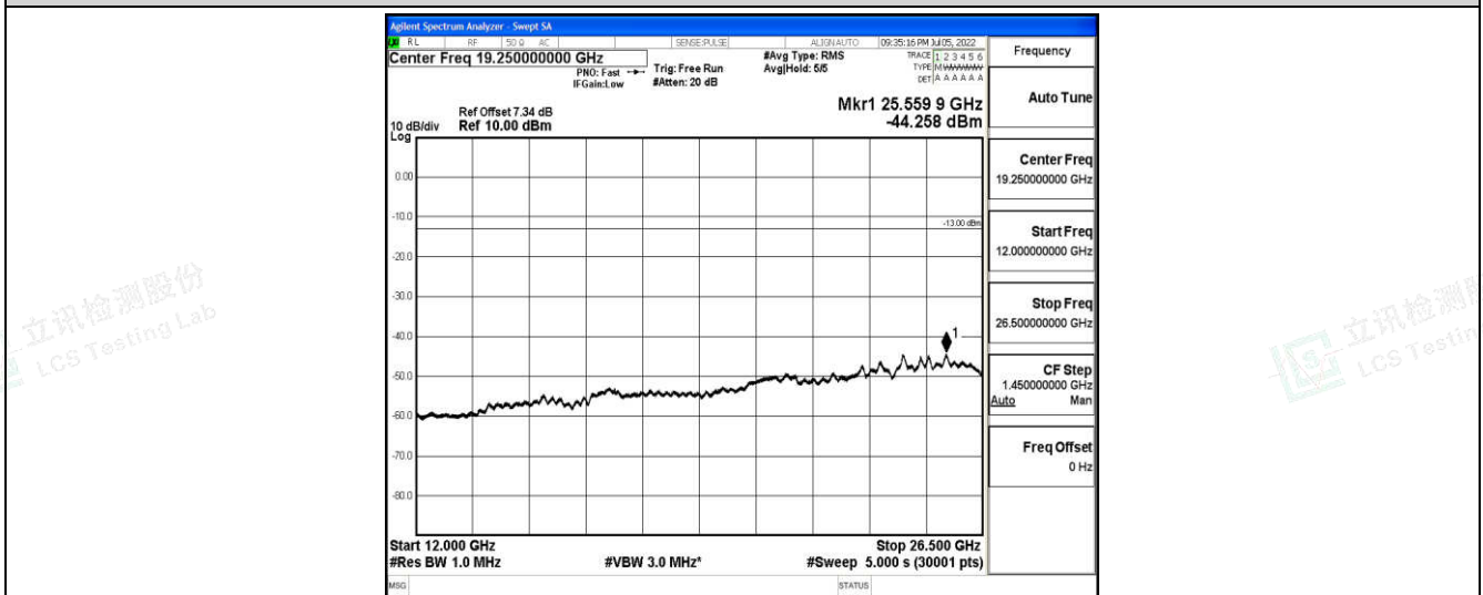
Band5-5MHz-16QAM-20625-1-0-High-12000-26500--44.26-PASS
