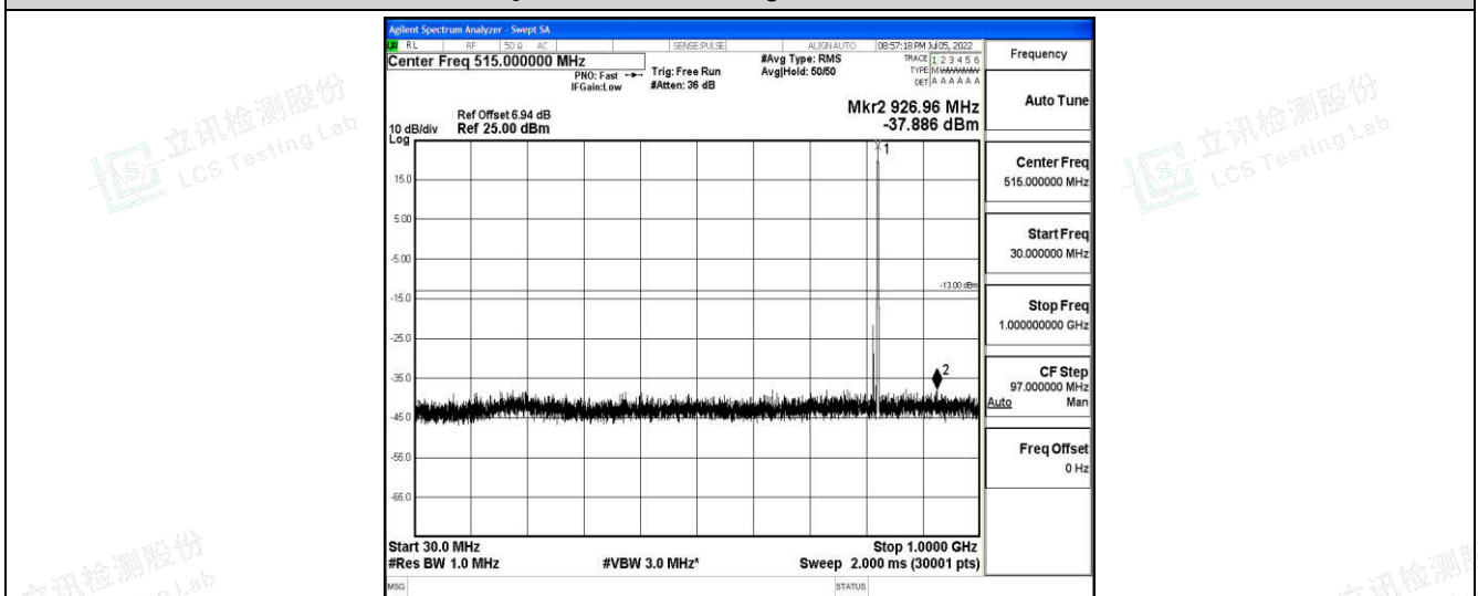
Band5-3MHz-16QAM-20415-1-0-Low-30-1000--37.89-PASS
