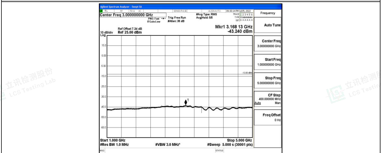
Band5-5MHz-16QAM-20525-1-0-Low-1000-5000--43.24-PASS
