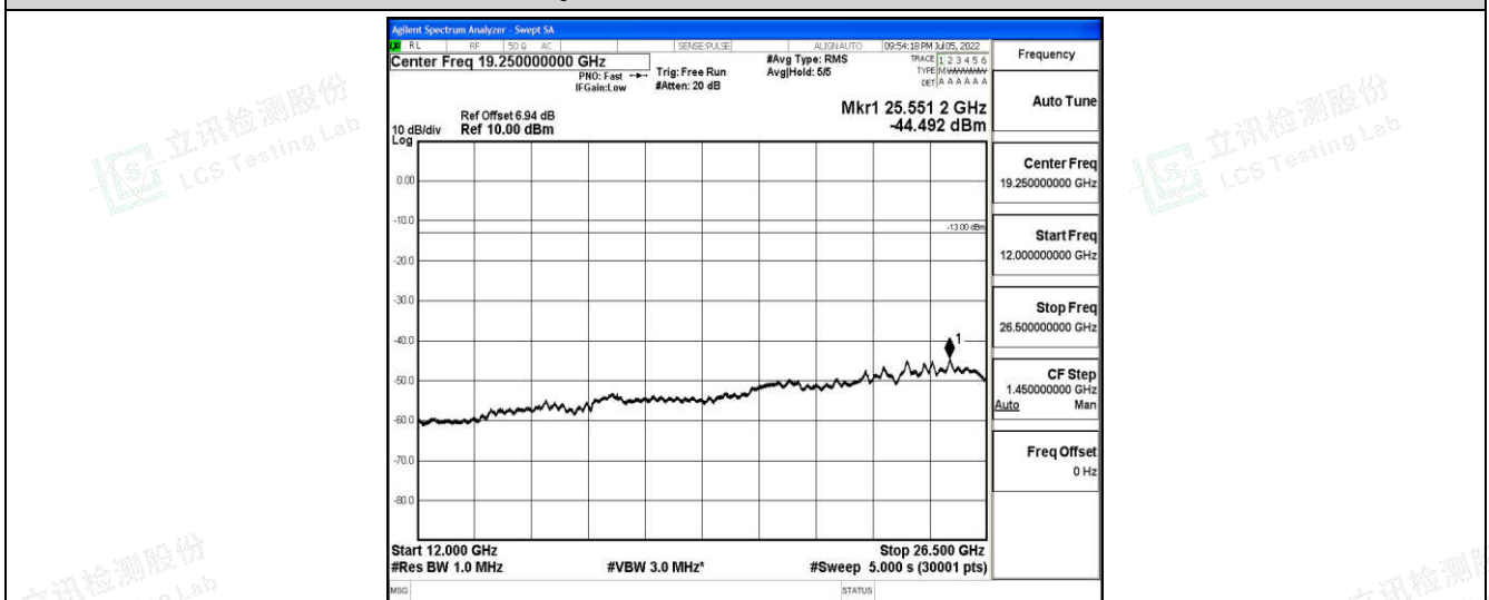
Band5-10MHz-16QAM-20450-1-0-Low-12000-26500--44.49-PASS
