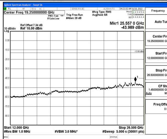
Band5-10MHz-16QAM-20525-1-0-Low-12000-26500--43.99-PASS
