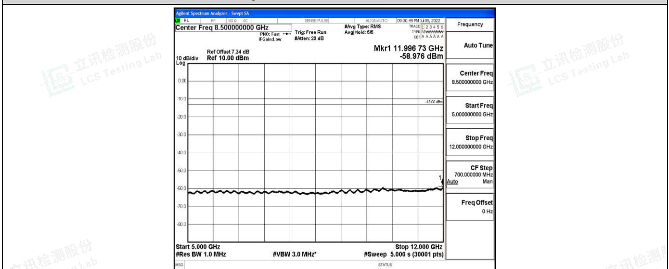
Band5-5MHz-16QAM-20525-1-0-Low-5000-12000--58.98-PASS
