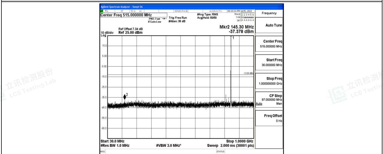
Band5-5MHz-16QAM-20625-1-0-High-30-1000--37.38-PASS
