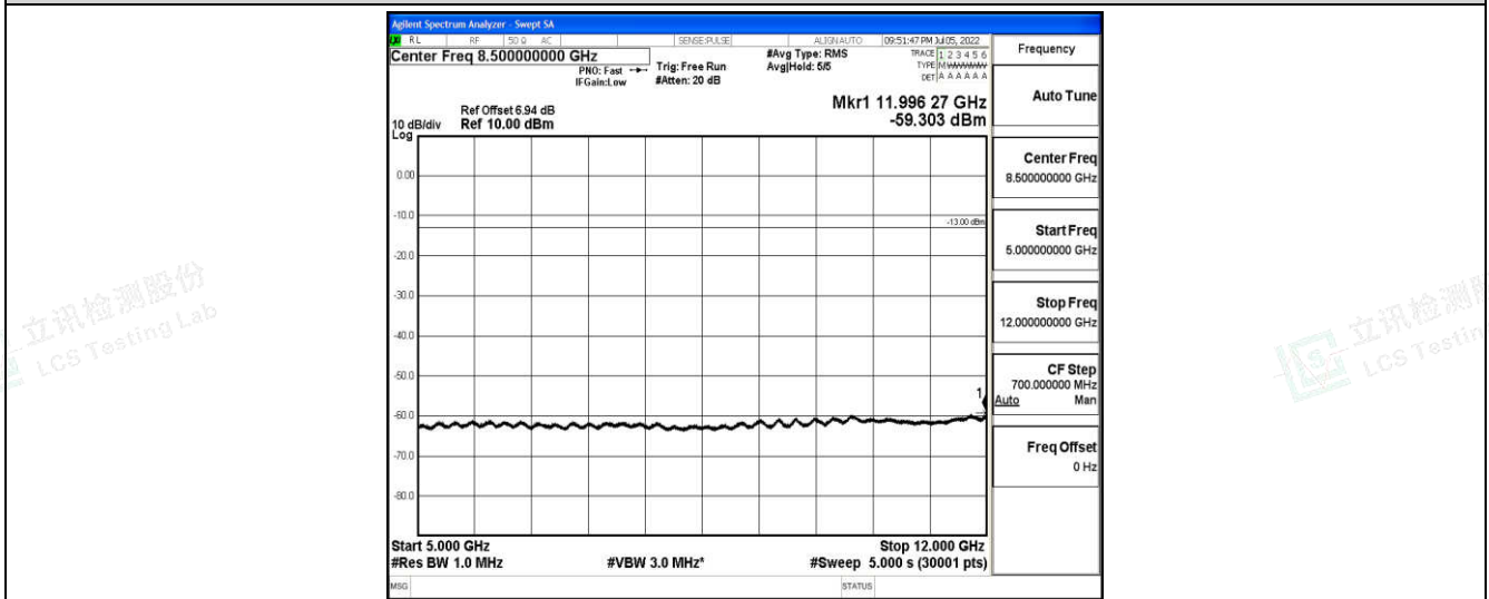
Band5-10MHz-QPSK-20450-1-0-Low-5000-12000--59.3-PASS
