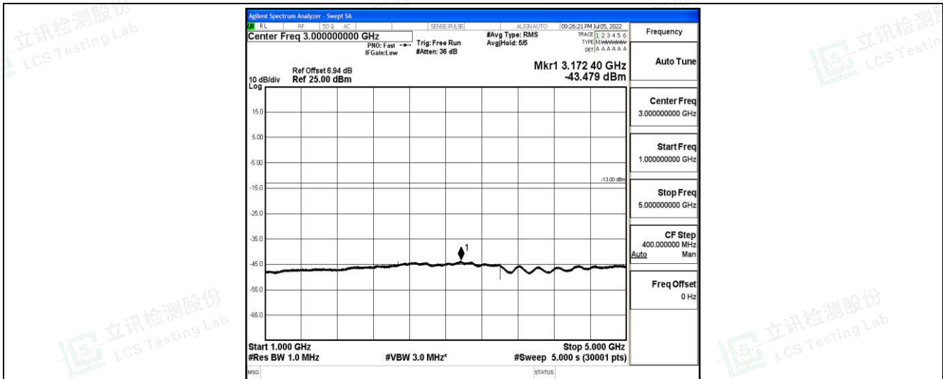
Band5-5MHz-16QAM-20425-1-0-Low-1000-5000--43.48-PASS
