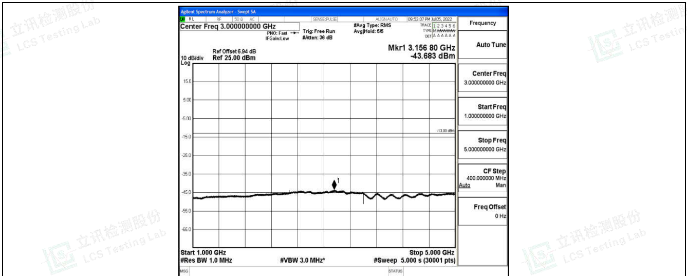
Band5-10MHz-16QAM-20450-1-0-Low-1000-5000--43.68-PASS
