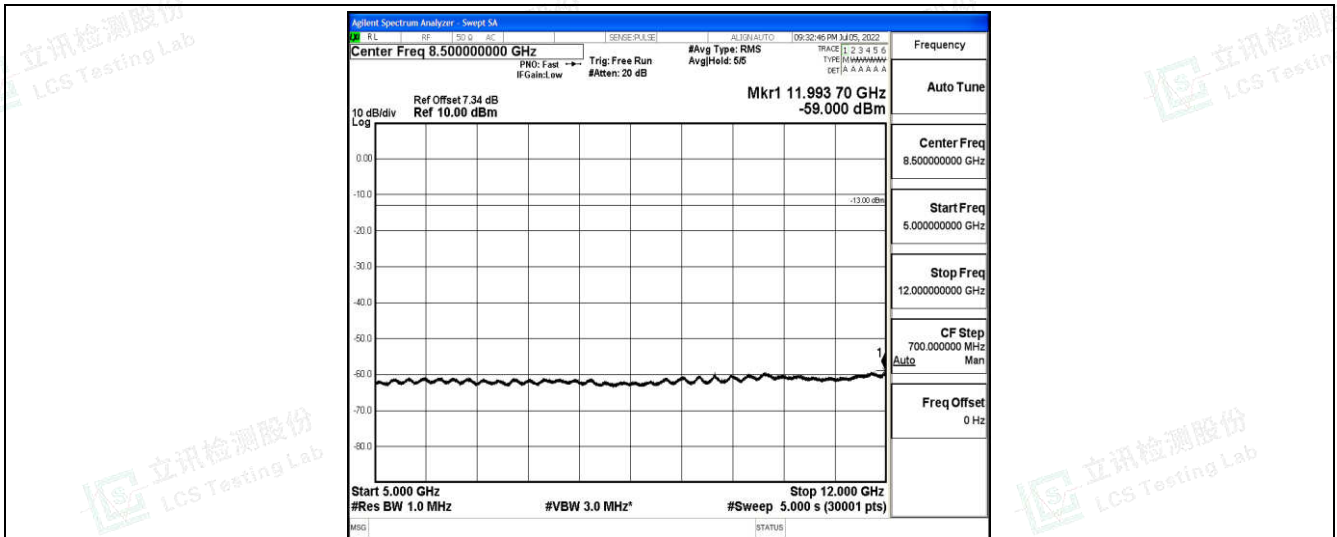
Band5-5MHz-QPSK-20625-1-0-High-5000-12000--59-PASS
