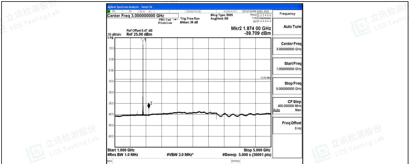
Band4-20MHz-QPSK-20175-1-0-Low-1000-5000--39.71-PASS
