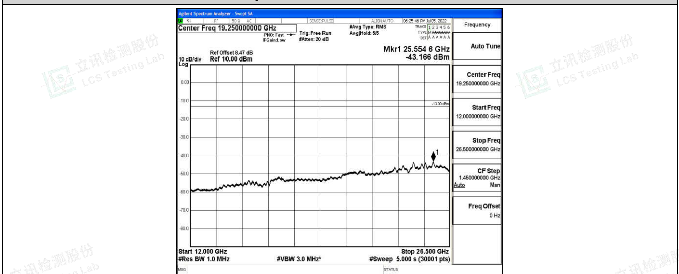
Band4-10MHz-16QAM-20175-1-0-Low-12000-26500--43.17-PASS
