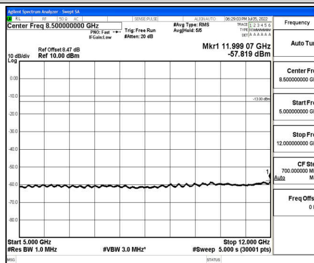
Band4-10MHz-16QAM-20350-1-0-High-5000-12000--57.82-PASS
