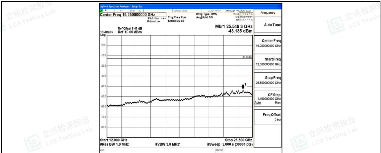
Band4-15MHz-QPSK-20325-1-0-High-12000-26500--43.14-PASS
