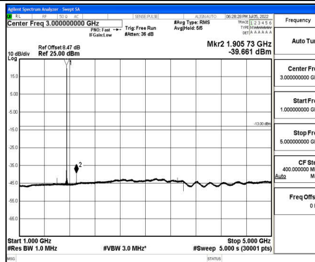
Band4-10MHz-16QAM-20350-1-0-High-1000-5000--39.66-PASS
