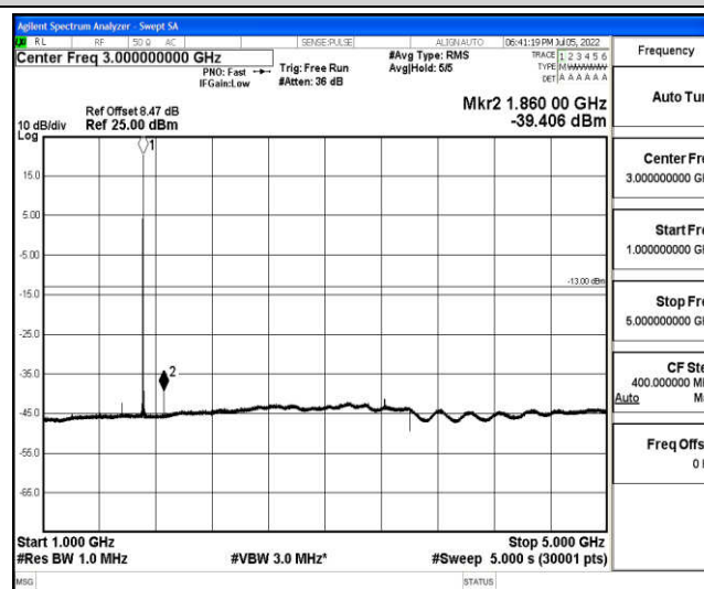
Band4-15MHz-QPSK-20025-1-0-Low-1000-5000--39.41-PASS
