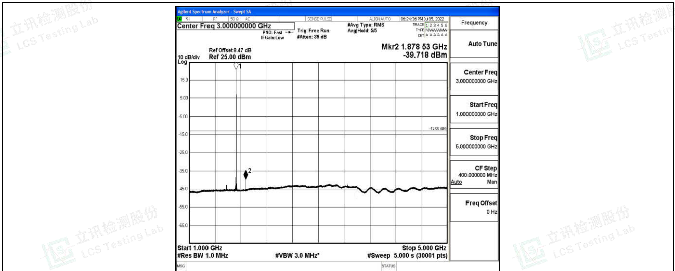
Band4-10MHz-16QAM-20175-1-0-Low-1000-5000--39.72-PASS
