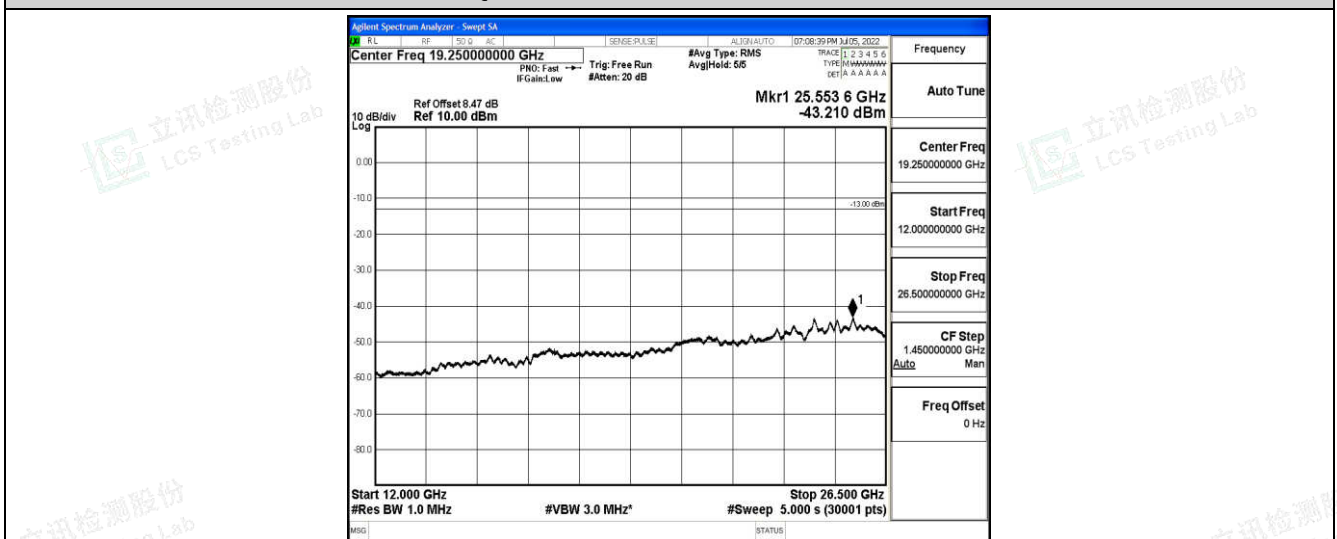
Band4-20MHz-QPSK-20175-1-0-Low-12000-26500--43.21-PASS
