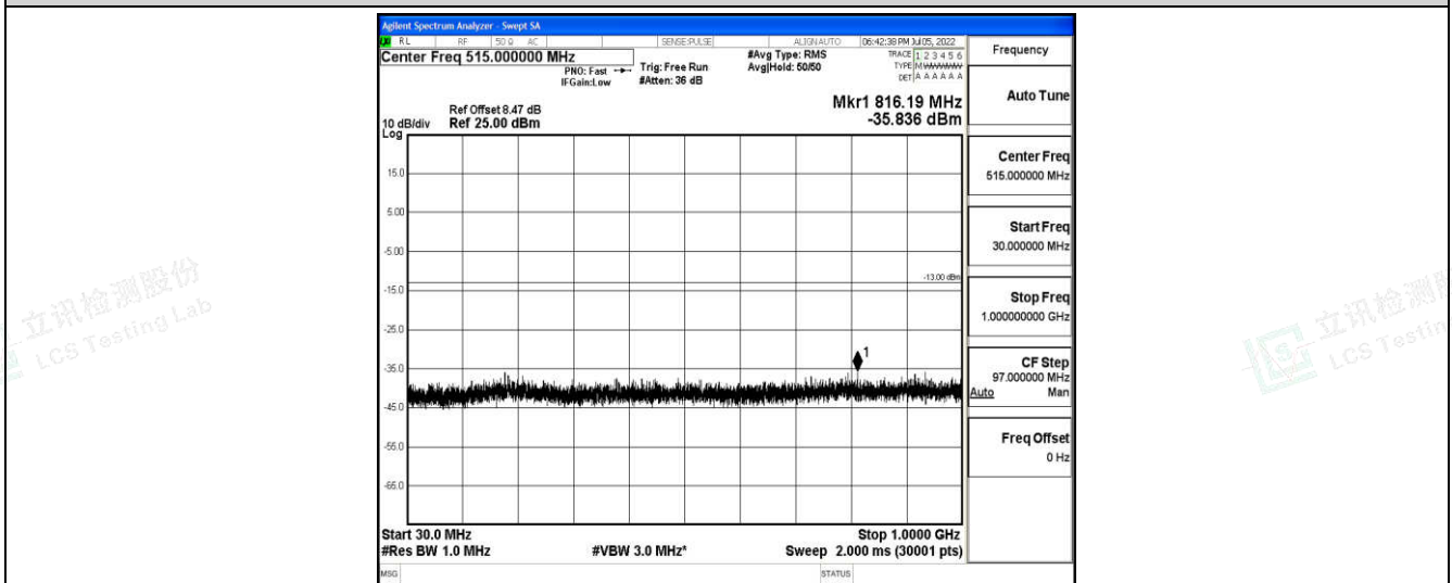
Band4-15MHz-16QAM-20025-1-0-Low-30-1000--35.84-PASS
