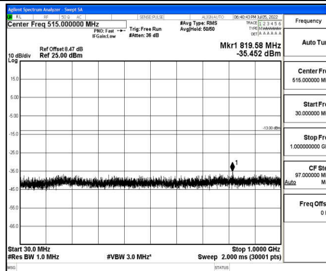
Band4-15MHz-QPSK-20025-1-0-Low-30-1000--35.45-PASS
