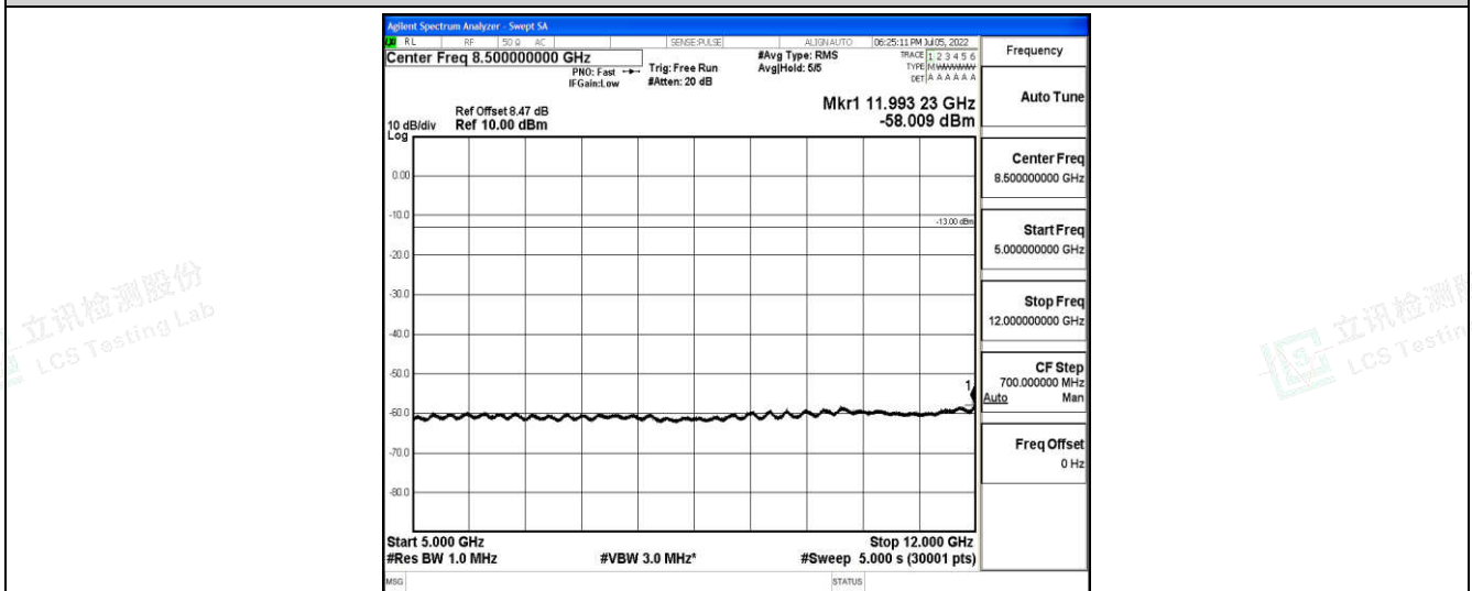
Band4-10MHz-16QAM-20175-1-0-Low-5000-12000--58.01-PASS
