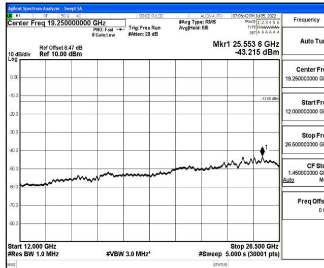
Band4-20MHz-16QAM-20050-1-0-Low-12000-26500--43.22-PASS
