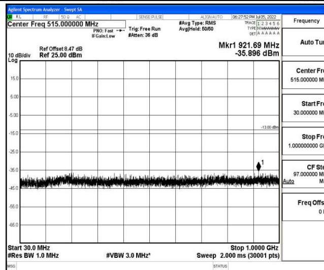
Band4-10MHz-16QAM-20350-1-0-High-30-1000--35.9-PASS
