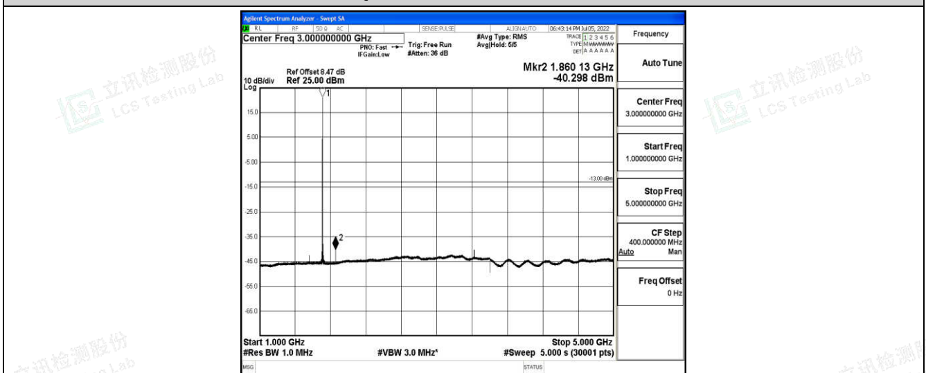
Band4-15MHz-16QAM-20025-1-0-Low-1000-5000--40.3-PASS
